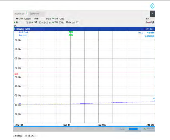
1-N41-PC2-30-100-M-1-DFT-PI2BPSK-Inner_1RB_L eft-1@1-0.15-30-Ant1--76.85--45-PASS
