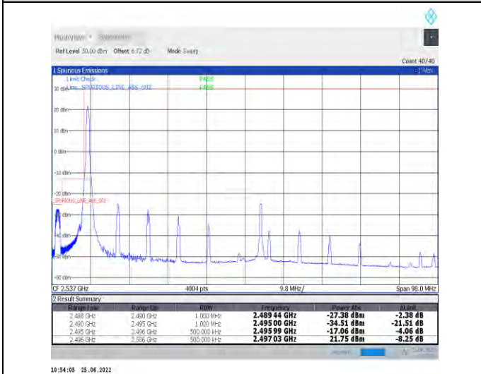
1-N41-PC2-30-90-L-4-CP-QPSK-Edge_1RB_Left-1@0-Ant1-PASS-see graph
