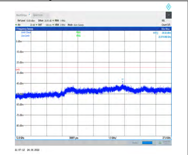
1-N41-PC2-30-100-L-1-DFT-PI2BPSK-Inner_1RB_L eft-1@1-12000-27000-Ant1--39.54--25-PASS
