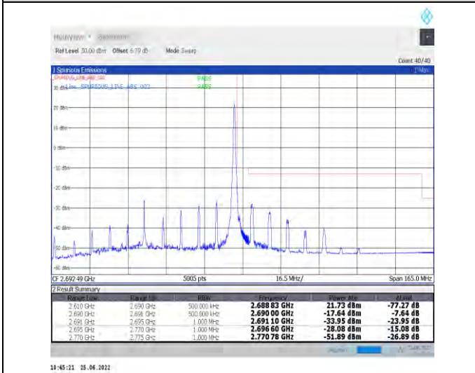
1-N41-PC2-30-80-H-5-CP-QPSK-Edge_1RB_Right-1@216-Ant1-PASS-see graph
