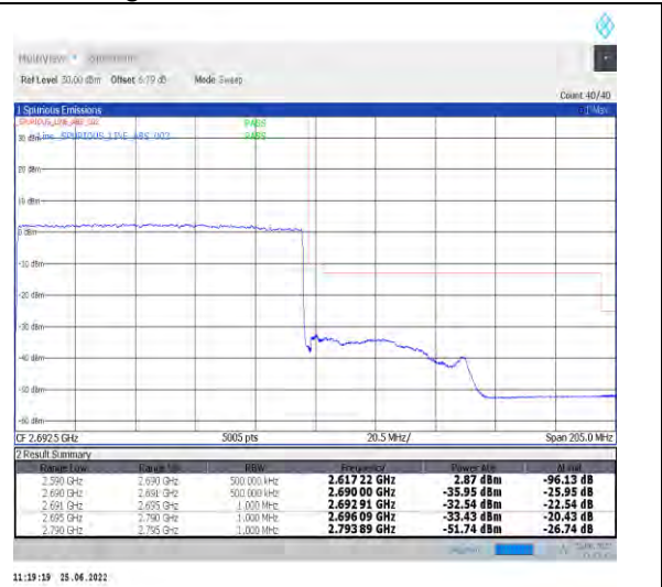
1-N41-PC2-30-100-H-3-DFT-PI2BPSK-Outer_Full-270@0-Ant1-PASS-see graph
