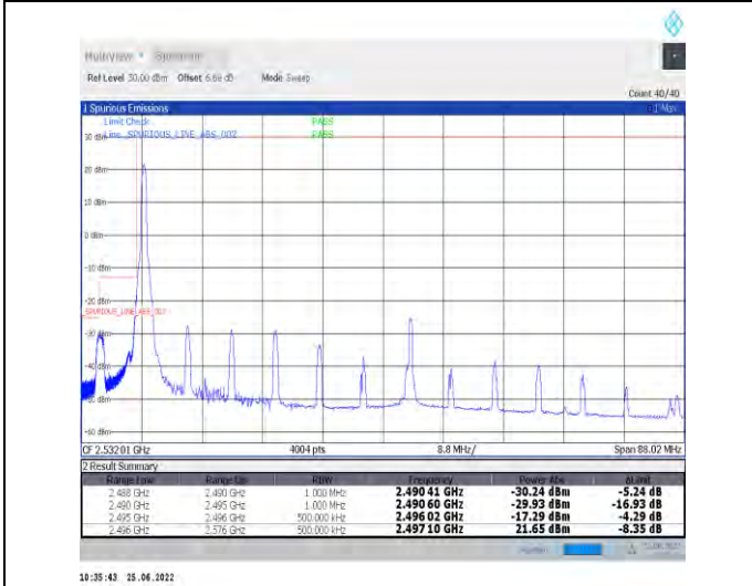
1-N41-PC2-30-80-L-4-CP-QPSK-Edge_1RB_Left-1@0-Ant1-PASS-see graph
