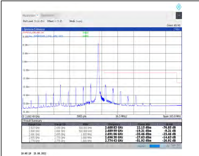
1-N41-PC2-30-80-H-2-DFT-PI2BPSK-Edge_1RB_Right-t-1@216-Ant1-PASS-see graph
