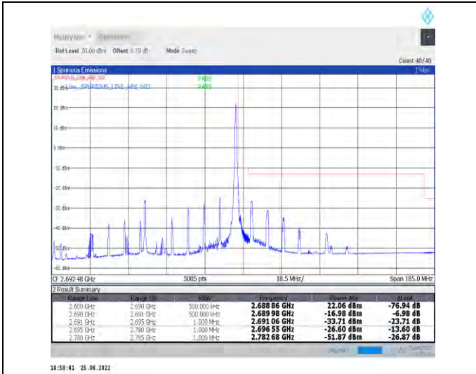
1-N41-PC2-30-90-H-2-DFT-PI2BPSK-Edge_1RB_Righ t-1@244-Ant1-PASS-see graph
