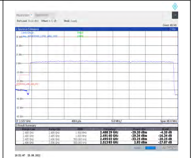
1-N41-PC2-30-90-L-3-DFT-PI2BPSK-Outer_Full-240@0-Ant1-PASS-see graph
