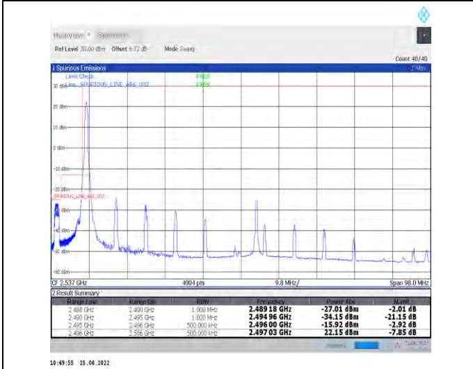
1-N41-PC2-30-90-L-1-DFT-PI2BPSK-Edge_1RB_Left-1@0-Ant1-PASS-see graph
