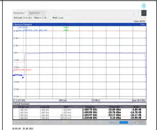
1-N41-PC2-30-90-L-6-CP-QPSK-Outer_Full-245@0-Ant1-PASS-see graph
