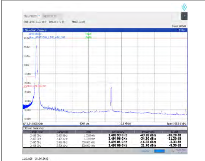
1-N41-PC2-30-100-L-4-CP-QPSK-Edge_1RB_Left-1@0-Ant1-PASS-see graph
