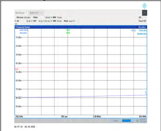
1-N41-PC2-30-100-H-1-DFT-PI2BPSK-Inner_1RB_L eft-1@1-0.15-30-Ant1--76.82--45-PASS
