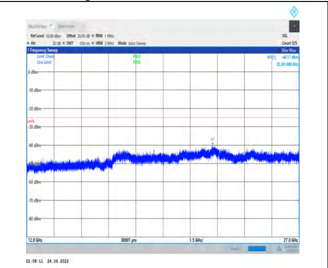
1-N41-PC2-30-100-H-1-DFT-PI2BPSK-Inner_1RB_L eft-1@1-12000-27000-Ant1--40.17--25-PASS
