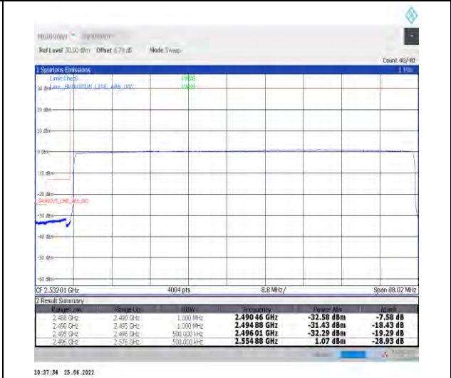
1-N41-PC2-30-80-L-6-CP-QPSK-Outer_Full-217@0-Ant1-PASS-see graph
