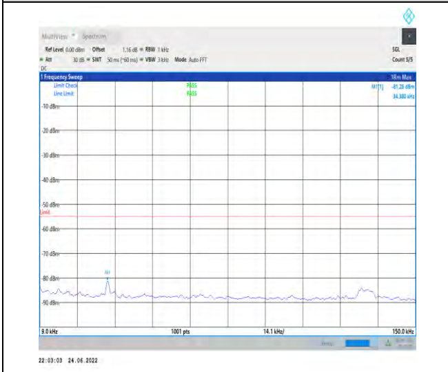
1-N41-PC2-30-100-M-1-DFT-PI2BPSK-Inner_1RB_L Left-1@1-0.009-0.15-Ant1--81.28--55-PASS
