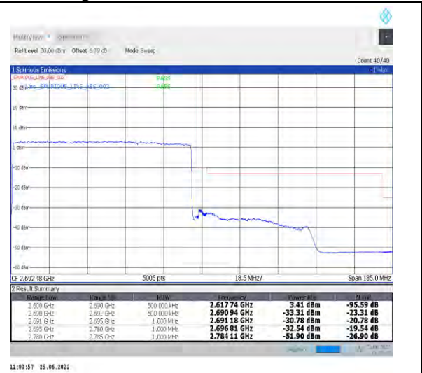
1-N41-PC2-30-90-H-3-DFT-PI2BPSK-Outer_Full-2 40@0-Ant1-PASS-see graph
