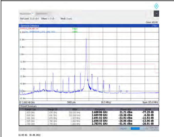
1-N41-PC2-30-90-H-5-CP-QPSK-Edge_1RB_Righ t-1@244-Ant1-PASS-see graph
