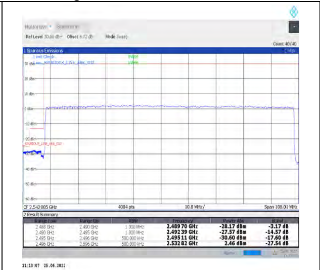
1-N41-PC2-30-100-L-3-DFT-PI2BPSK-Outer_Full-270@0-Ant1-PASS-see graph
