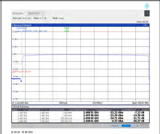
1-N41-PC2-30-100-L-6-CP-QPSK-Outer_Full-273@0-Ant1-PASS-see graph
