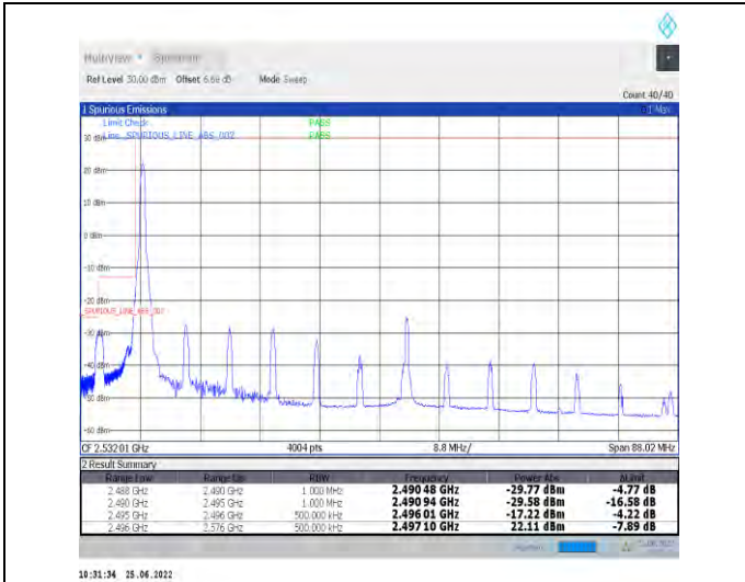
1-N41-PC2-30-80-L-1-DFT-PI2BPSK-Edge_1RB_Left-1@0-Ant1-PASS-see graph
