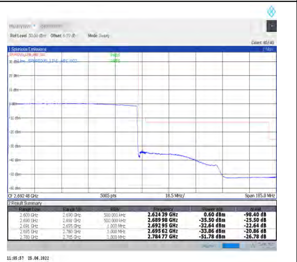
1-N41-PC2-30-90-H-6-CP-QPSK-Outer_Full-245 @0-Ant1-PASS-see graph
