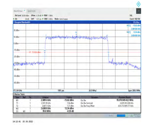
1-N41-PC2-30-100-H-5-DFT-256QAM-Outer_Full-2700@0-Ant1-95.91-99.800-≤100-PASS
