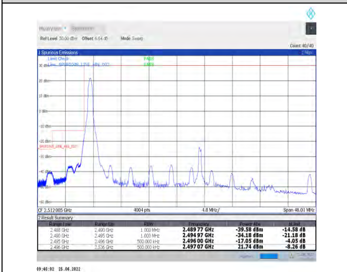
1-N41-PC2-30-40-L-4-CP-QPSK-Edge_1RB_Left-1@0-Ant1-PASS-see graph
