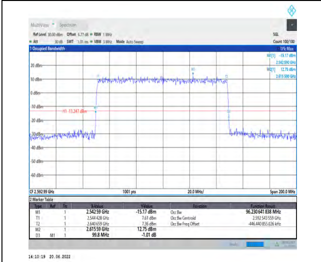
1-N41-PC2-30-100-M-5-DFT-256QAM-Outer_Full-270 @0-Ant1-96.231-99.800-≤100-PASS
