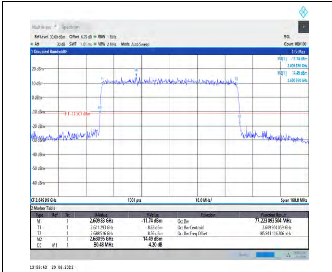
1-N41-PC2-30-80-H-8-CP-64QAM-Outer_Full-217@ 0-Ant1-77.223-80.480-≤80-PASS
