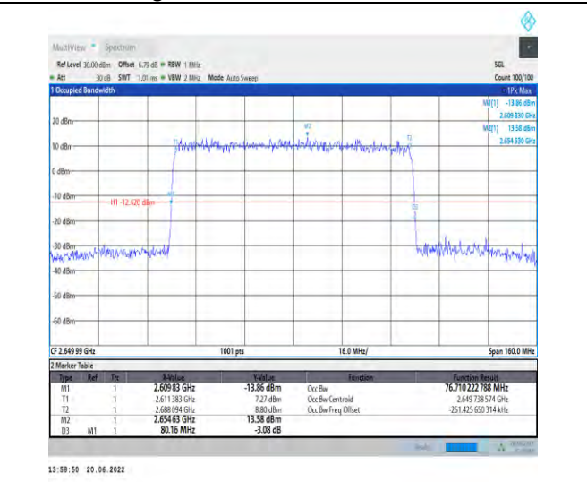
1-N41-PC2-30-80-H-5-DFT-256QAM-Outer_Full-216 @0-Ant1-76.71-80.160-≤80-PASS
