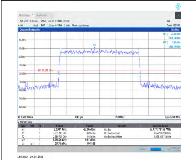
1-N41-PC2-30-60-H-9-CP-256QAM-Outer_Full-162 @0-Ant1-57.478-59.760-≤60-PASS
