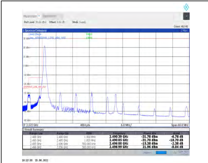
1-N41-PC2-30-60-L-1-DFT-PI2BPSK-Edge_1RB_Left-1@0-Ant1-PASS-see graph
