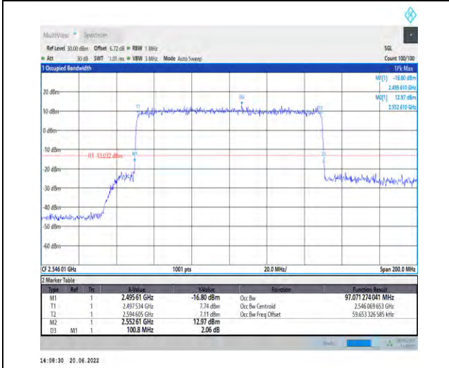
1-N41-PC2-30-100-L-6-CP-QPSK-Outer_Full-273 @0-Ant1-97.071-100.800-≤100-PASS
