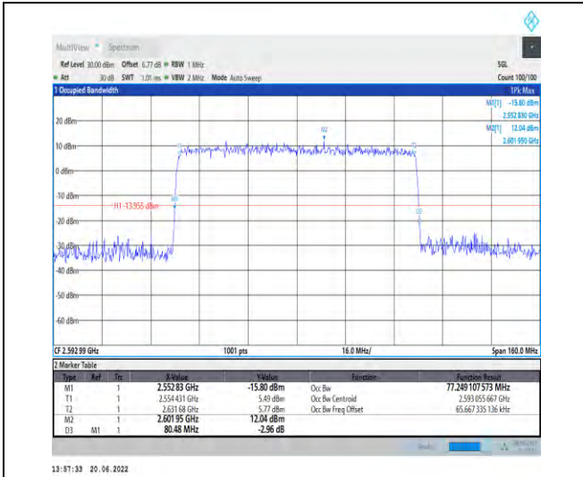
1-N41-PC2-30-80-M-9-CP-256QAM-Outer_Full-217 @0-Ant1-77.249-80.480-≤80-PASS
