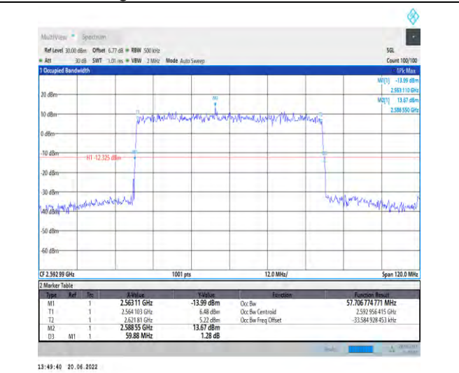
1-N41-PC2-30-60-M-5-DFT-256QAM-Outer_Full-162 @0-Ant1-57.707-59.880-≤60-PASS
