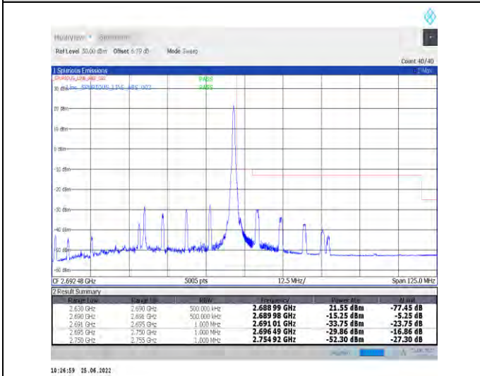
1-N41-PC2-30-60-H-5-CP-QPSK-Edge_1RB_Right-1@161-Ant1-PASS-see graph
