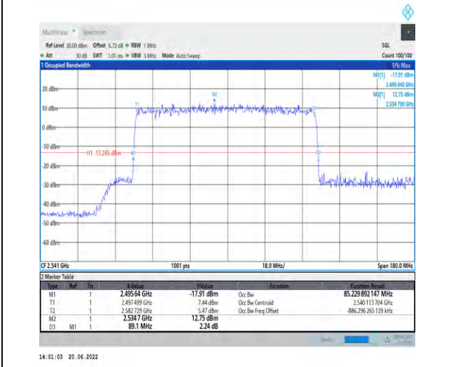
1-N41-PC2-30-90-L-5-DFT-256QAM-Outer_Full-240 @0-Ant1-85.23-89.100-≤90-PASS
