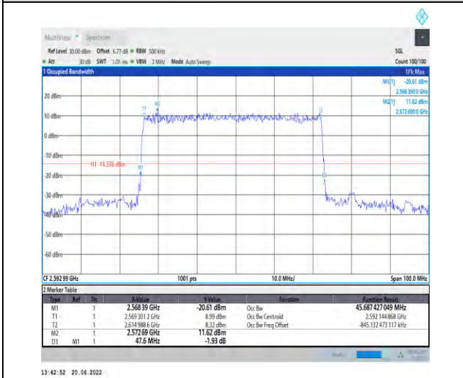
1-N41-PC2-30-50-M-5-DFT-256QAM-Outer_Full-128 @0-Ant1-45.687-47.600-≤50-PASS
