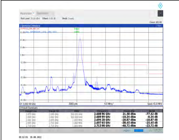
1-N41-PC2-30-20-H-5-CP-QPSK-Edge_1RB_Right-1@50-Ant1-PASS-see graph
