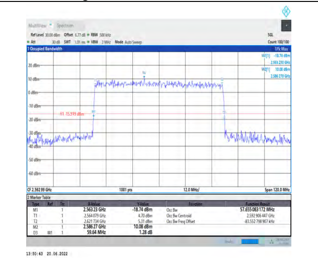
1-N41-PC2-30-60-M-9-CP-256QAM-Outer_Full-162 @0-Ant1-57.655-59.640-≤60-PASS
