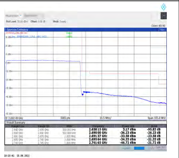
1-N41-PC2-30-50-H-6-CP-QPSK-Outer_Full-133@0-Ant1-PASS-see graph
