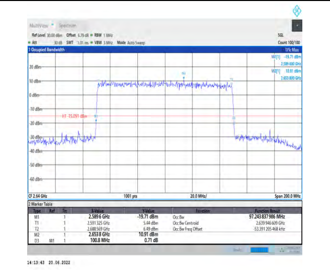
1-N41-PC2-30-100-H-9-CP-256QAM-Outer_Full-273 @0-Ant1-97.244-100.800-≤100-PASS
