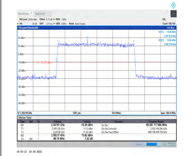
1-N41-PC2-30-90-M-4-DFT-64QAM-Outer_Full-240 @0-Ant1-85.582-88.740-<=90-PASS
