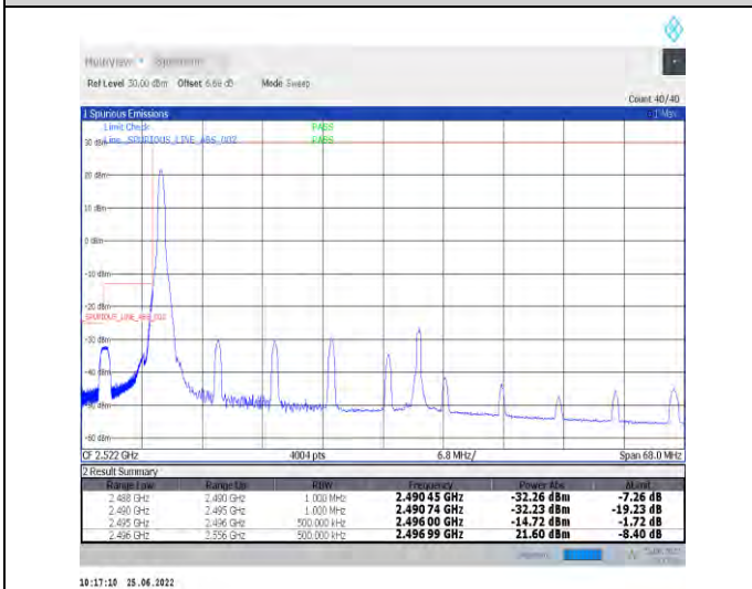
1-N41-PC2-30-60-L-4-CP-QPSK-Edge_1RB_Left-1@0-Ant1-PASS-see graph
