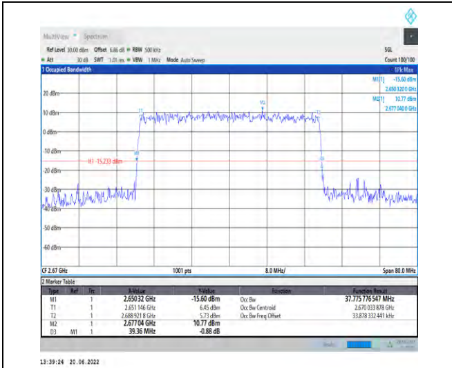
1-N41-PC2-30-40-H-9-CP-256QAM-Outer_Full-106 @0-Ant1-37.776-39.360-≤40-PASS
