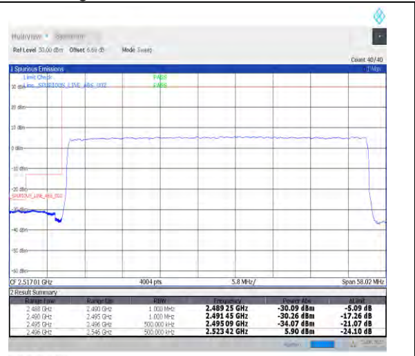
1-N41-PC2-30-50-L-3-DFT-PI2BPSK-Outer_Full-128@0-Ant1-PASS-see graph
