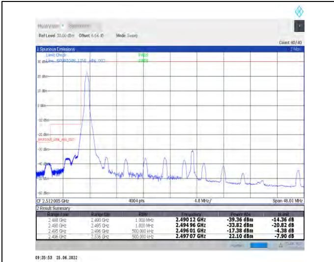
1-N41-PC2-30-40-L-1-DFT-PI2BPSK-Edge_1RB_Left-1@0-Ant1-PASS-see graph
