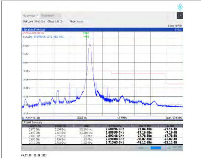
1-N41-PC2-30-20-H-2-DFT-PI2BPSK-Edge_1RB_Right-t1@50-Ant1-PASS-see graph
