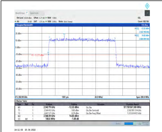
1-N41-PC2-30-100-M-7-CP-16QAM-Outer_Full-273 @0-Ant1-97.16-100.600-≤100-PASS
