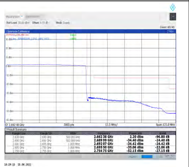
1-N41-PC2-30-60-H-6-CP-QPSK-Outer_Full-162@0-Ant1-PASS-see graph
