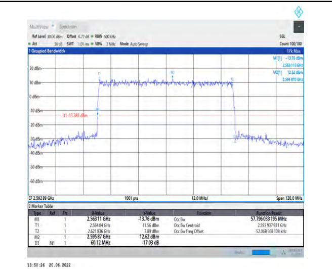
1-N41-PC2-30-60-M-7-CP-16QAM-Outer_Full-162@0 -Ant1-57.796-60.120-≤60-PASS
