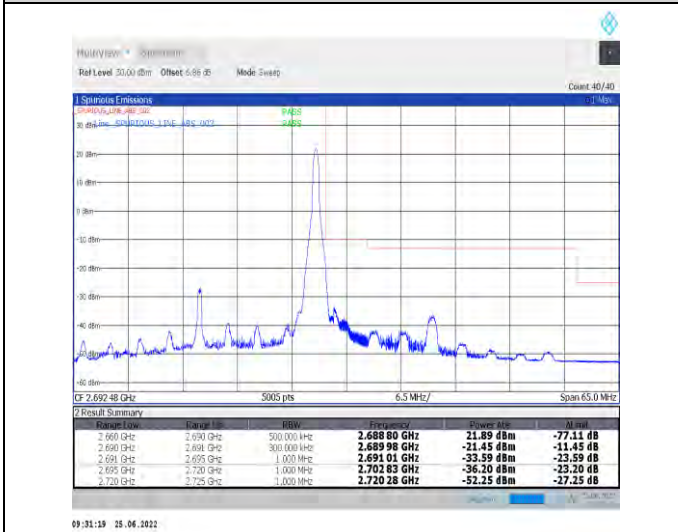
1-N41-PC2-30-30-H-5-CP-QPSK-Edge_1RB_Right-1@77-Ant1-PASS-see graph
