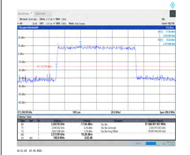
1-N41-PC2-30-100-M-9-CP-256QAM-Outer_Full-27 3@0-Ant1-97.306-100.800-≤100-PASS
