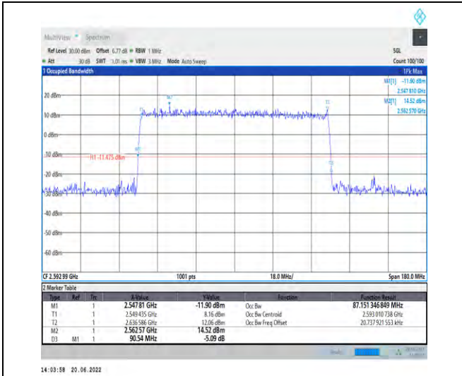
1-N41-PC2-30-90-M-6-CP-QPSK-Outer_Full-245@0 -Ant1-87.151-90.540-≤90-PASS
