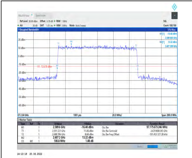
1-N41-PC2-30-100-H-6-CP-QPSK-Outer_Full-273@ 0-Ant1-97.176-100.800-≤100-PASS
