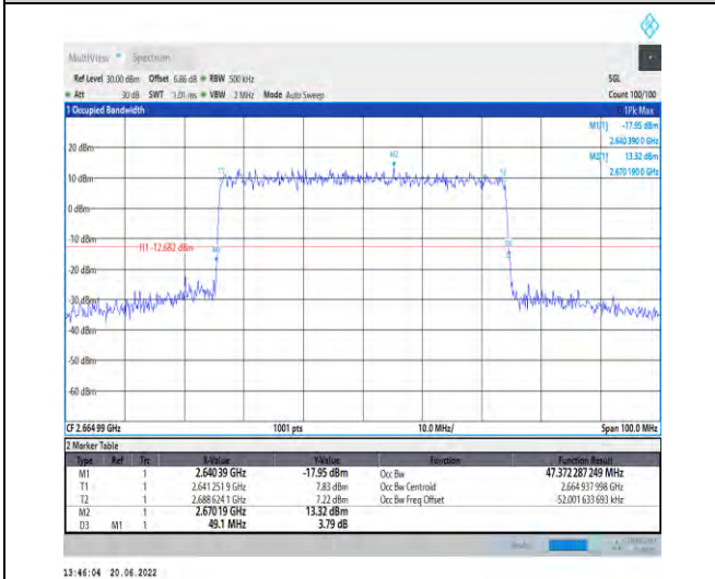
1-N41-PC2-30-50-H-8-CP-64QAM-Outer_Full-133@0 -Ant1-47.372-49.100-≤50-PASS
