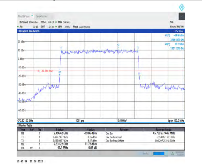
1-N41-PC2-30-50-L-5-DFT-256QAM-Outer_Full-128 @0-Ant1-45.77-47.400-≤50-PASS
