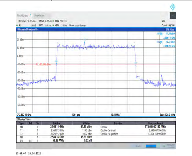
1-N41-PC2-30-60-M-1-DFT-QPSK-Outer_Full-162 @0-Ant1-57.869-59.880-≤60-PASS
