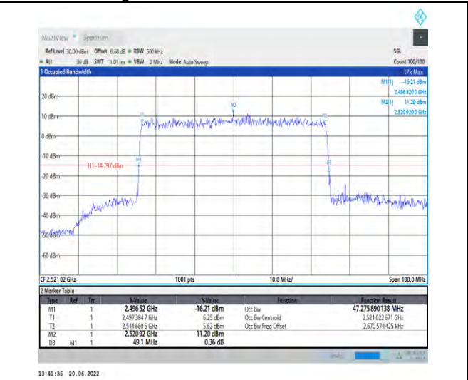
1-N41-PC2-30-50-L-9-CP-256QAM-Outer_Full-133 @0-Ant1-47.276-49.100-≤50-PASS
