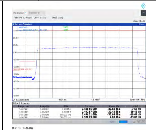
1-N41-PC2-30-40-L-3-DFT-PI2BPSK-Outer_Full-100@0-Ant1-PASS-see graph
