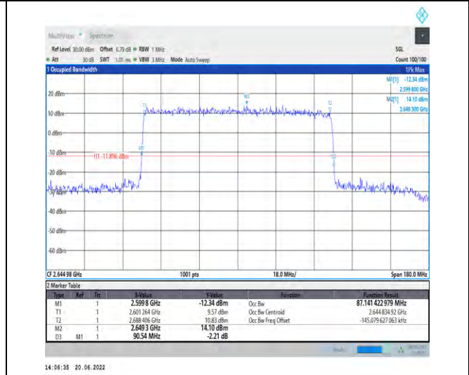
1-N41-PC2-30-90-H-8-CP-64QAM-Outer_Full-245@0-Ant1-87.141-90.540-≤90-PASS
