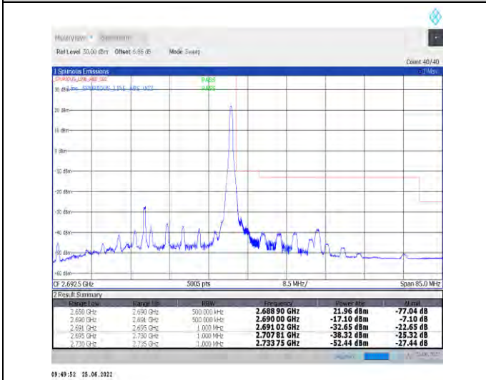
1-N41-PC2-30-40-H-5-CP-QPSK-Edge_1RB_Right-1@105-Ant1-PASS-see graph
