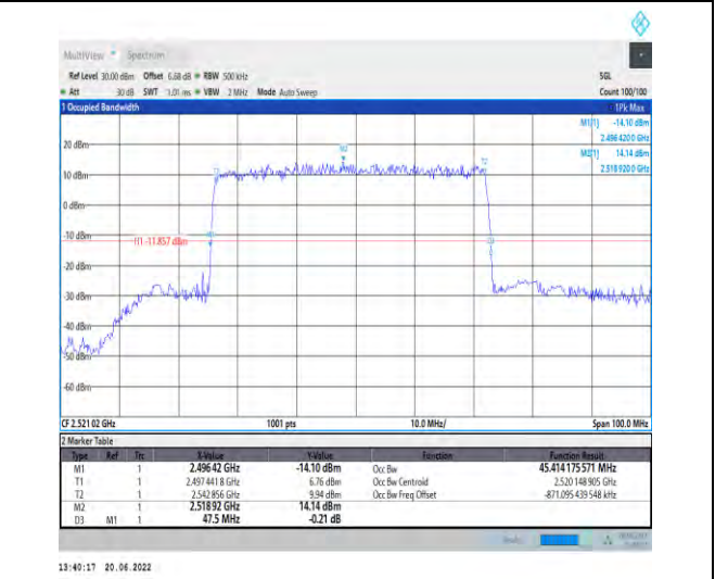
1-N41-PC2-30-50-L-3-DFT-16QAM-Outer_Full-128 @0-Ant1-45.414-47.500-≤50-PASS
