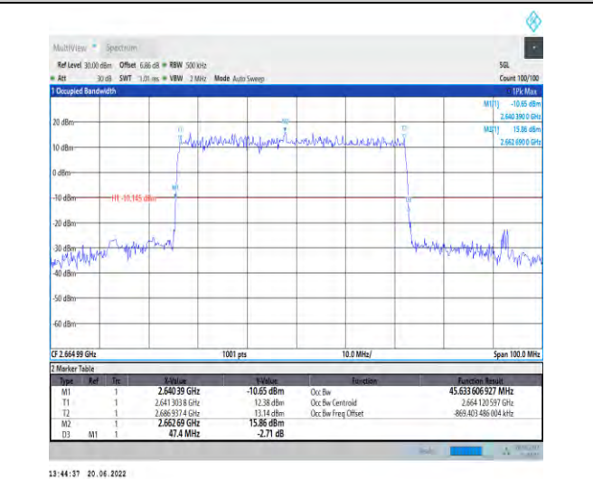
1-N41-PC2-30-50-H-1-DFT-QPSK-Outer_Full-128@ 0-Ant1-45.634-47.400-≤50-PASS
