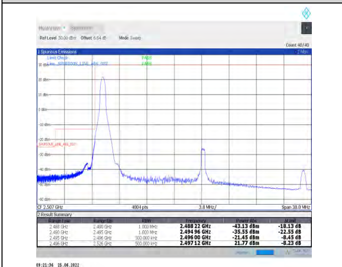
1-N41-PC2-30-30-L-4-CP-QPSK-Edge_1RB_Left-1@0-Ant1-PASS-see graph
