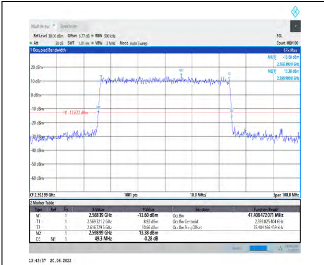
1-N41-PC2-30-50-M-7-CP-16QAM-Outer_Full-133@ 0-Ant1-47.408-49.300-≤50-PASS
