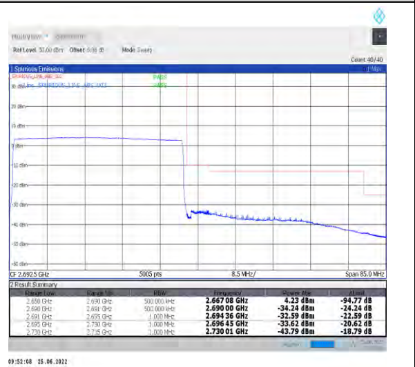
1-N41-PC2-30-40-H-6-CP-QPSK-Outer_Full-106@0-Ant1-PASS-see graph
