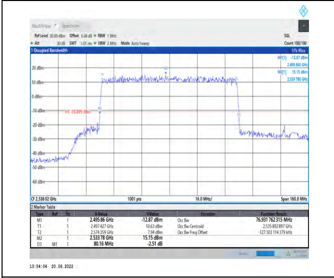
1-N41-PC2-30-80-L-4-DFT-64QAM-Outer_Full-216 @0-Ant1-76.932-80.160-≤80-PASS
