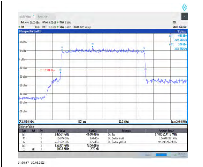
1-N41-PC2-30-100-L-8-CP-64QAM-Outer_Full-273 @0-Ant1-97.005-100.800-≤100-PASS
