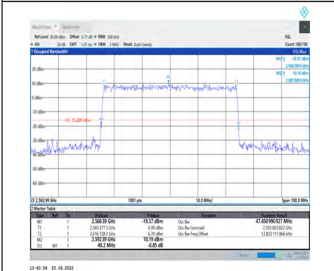
1-N41-PC2-30-50-M-9-CP-256QAM-Outer_Full-133 @0-Ant1-47.451-49.200-≤50-PASS
