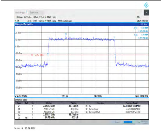
1-N41-PC2-30-90-M-8-CP-64QAM-Outer_Full-245@0 -Ant1-87.319-90.720-≤90-PASS
