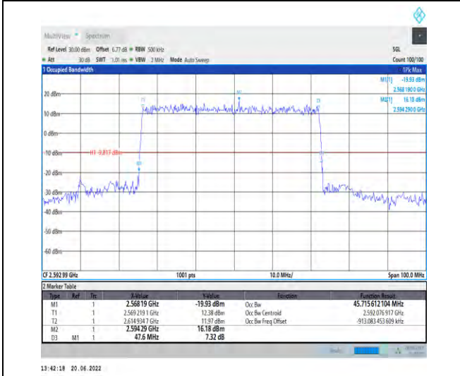
1-N41-PC2-30-50-M-1-DFT-QPSK-Outer_Full-128@ 0-Ant1-45.716-47.600-≤50-PASS
