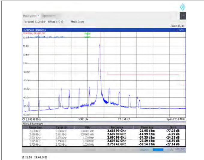
1-N41-PC2-30-60-H-2-DFT-PI2BPSK-Edge_1RB_Right-t-1@161-Ant1-PASS-see graph
