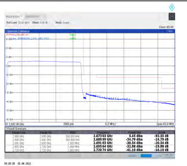
1-N41-PC2-30-30-H-6-CP-QPSK-Outer_Full-78@0-Ant1-PASS-see graph
