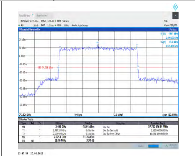
1-N41-PC2-30-60-L-6-CP-QPSK-Outer_Full-162@0-Ant1-57.721-59.760-≤60-PASS
