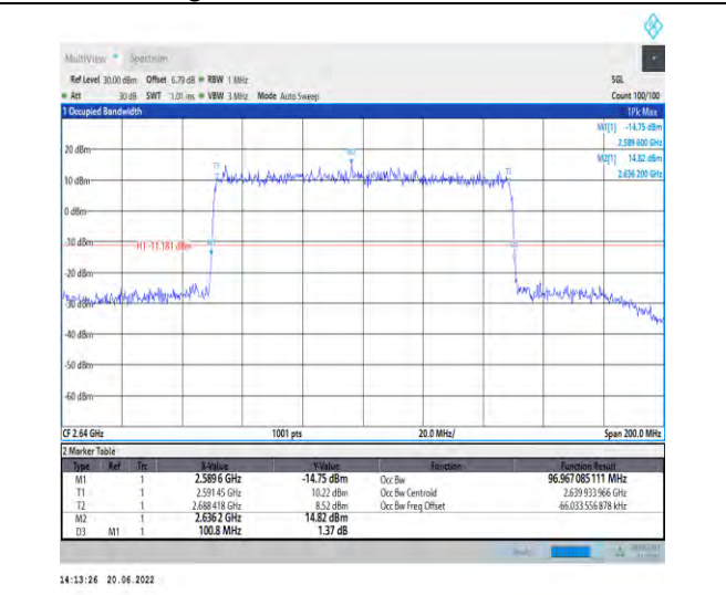
1-N41-PC2-30-100-H-7-CP-16QAM-Outer_Full-273 @0-Ant1-96.967-100.800-≤100-PASS
