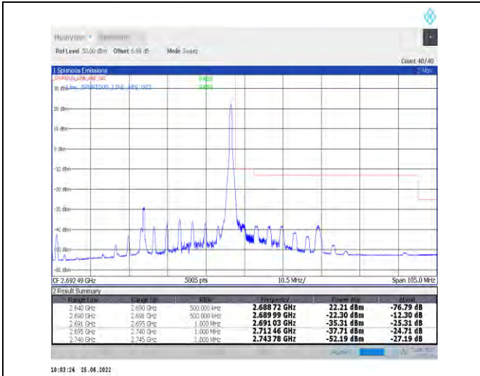
1-N41-PC2-30-50-H-2-DFT-PI2BPSK-Edge_1RB_Right-t-1@132-Ant1-PASS-see graph
