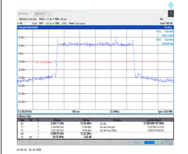
1-N41-PC2-30-60-M-2-DFT-PI2BPSK-Outer_Full-162 @0-Ant1-57.839-59.760-≤60-PASS
