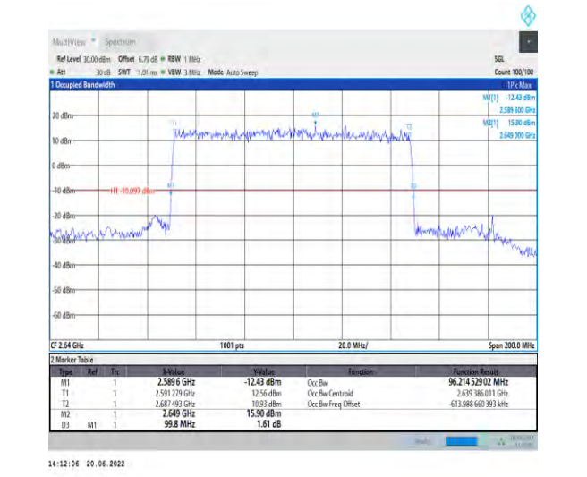
1-N41-PC2-30-100-H-1-DFT-QPSK-Outer_Full-270 @0-Ant1-96.215-99.800-≤100-PASS
