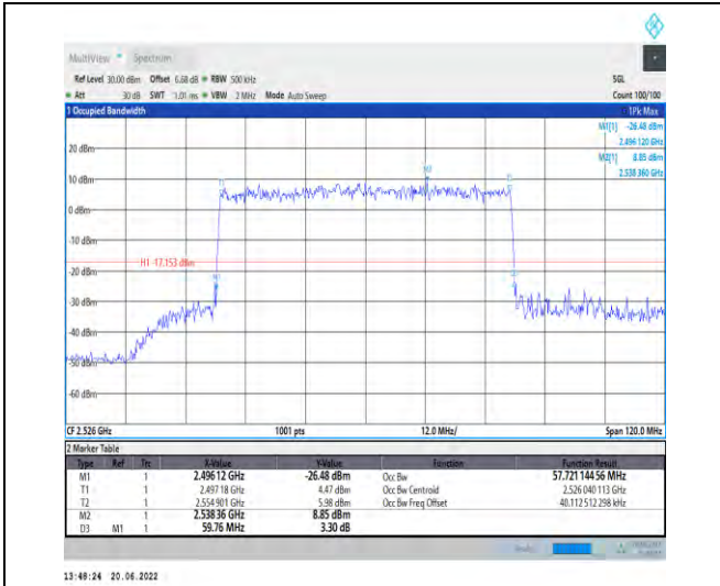
1-N41-PC2-30-60-L-9-CP-256QAM-Outer_Full-162 @0-Ant1-57.721-59.760-≤60-PASS
