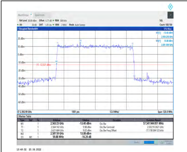
1-N41-PC2-30-60-M-4-DFT-64QAM-Outer_Full-162 @0-Ant1-57.542-59.880-≤60-PASS
