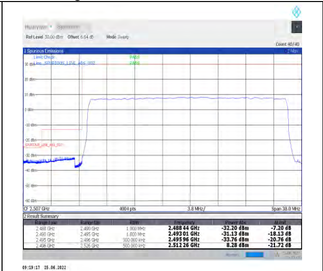
1-N41-PC2-30-30-L-3-DFT-PI2BPSK-Outer_Full-75@0-Ant1-PASS-see graph
