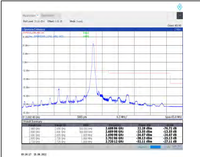
1-N41-PC2-30-30-H-2-DFT-PI2BPSK-Edge_1RB_Right-t1@77-Ant1-PASS-see graph
