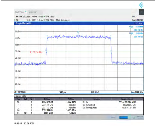
1-N41-PC2-30-80-M-7-CP-16QAM-Outer_Full-217@0-Ant1-77.474-80.640-≤80-PASS
