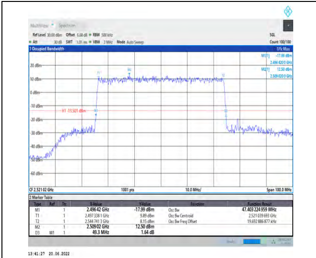
1-N41-PC2-30-50-L-8-CP-64QAM-Outer_Full-133@ 0-Ant1-47.403-49.300-≤50-PASS
