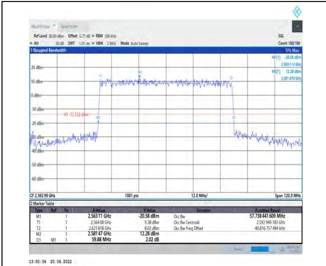
1-N41-PC2-30-60-M-8-CP-64QAM-Outer_Full-162@ 0-Ant1-57.738-59.880-≤60-PASS
