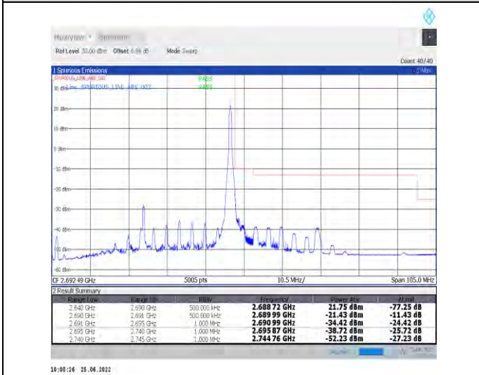
1-N41-PC2-30-50-H-5-CP-QPSK-Edge_1RB_Right-1@132-Ant1-PASS-see graph
