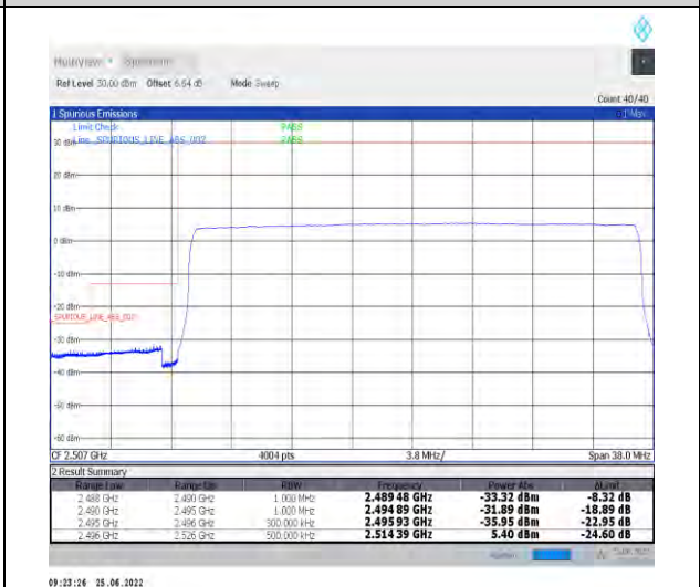
1-N41-PC2-30-30-L-6-CP-QPSK-Outer_Full-78@0-Ant1-PASS-see graph
