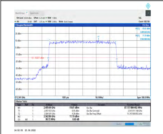
1-N41-PC2-30-90-L-9-CP-256QAM-Outer_Full-245 @0-Ant1-87.158-90.720-≤90-PASS
