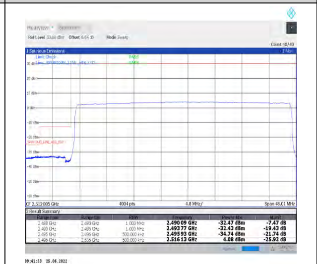
1-N41-PC2-30-40-L-6-CP-QPSK-Outer_Full-106@0-Ant1-PASS-see graph
