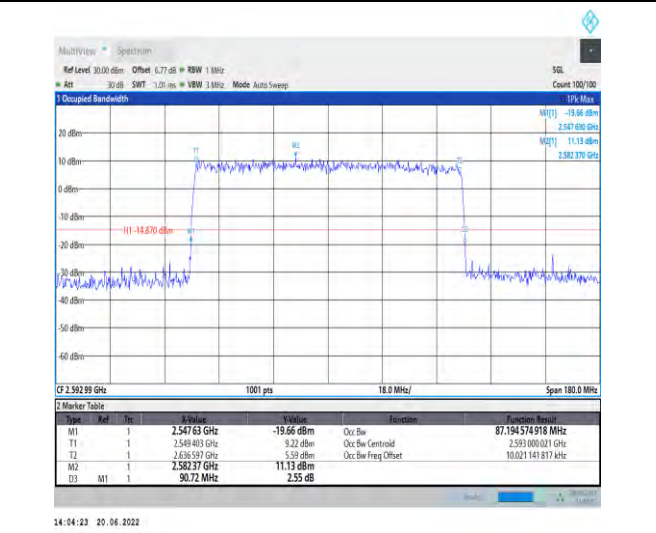
1-N41-PC2-30-90-M-9-CP-256QAM-Outer_Full-245@0 -Ant1-87.195-90.720-≤90-PASS
