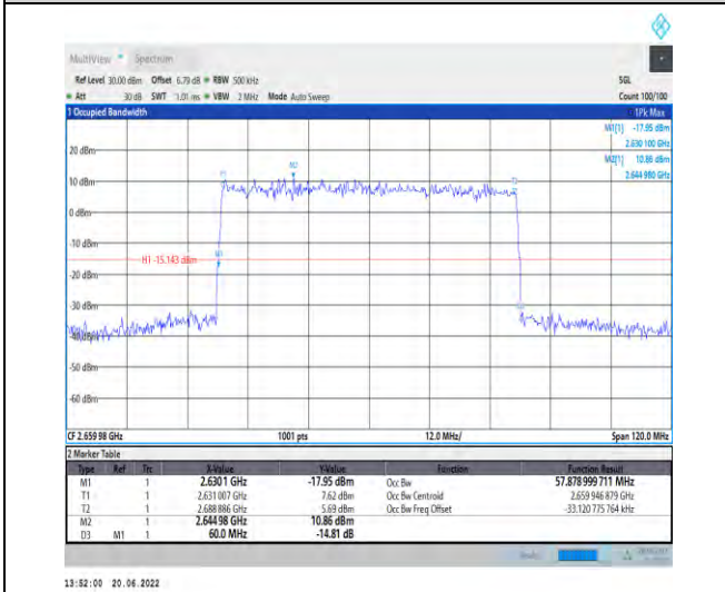
1-N41-PC2-30-60-H-5-DFT-256QAM-Outer_Full-162 @0-Ant1-57.879-60.000-≤60-PASS
