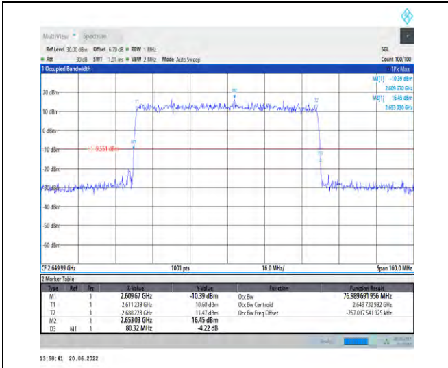
1-N41-PC2-30-80-H-4-DFT-64QAM-Outer_Full-216 @0-Ant1-76.99-80.320-≤80-PASS
