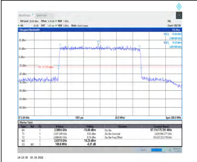
1-N41-PC2-30-100-H-8-CP-64QAM-Outer_Full-273 @0-Ant1-97.114-100.800-≤100-PASS
