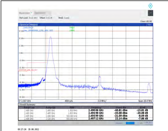
1-N41-PC2-30-30-L-1-DFT-PI2BPSK-Edge_1RB_Left-1@0-Ant1-PASS-see graph
