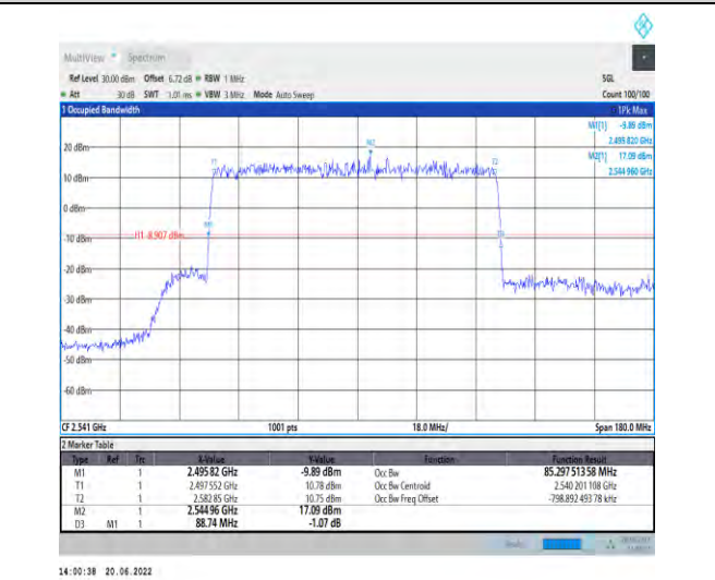
1-N41-PC2-30-90-L-2-DFT-PI2BPSK-Outer_Full-240 @0-Ant1-85.298-88.740-≤90-PASS
