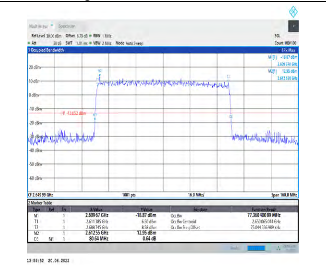
1-N41-PC2-30-80-H-9-CP-256QAM-Outer_Full-217 @0-Ant1-77.36-80.640-≤80-PASS
