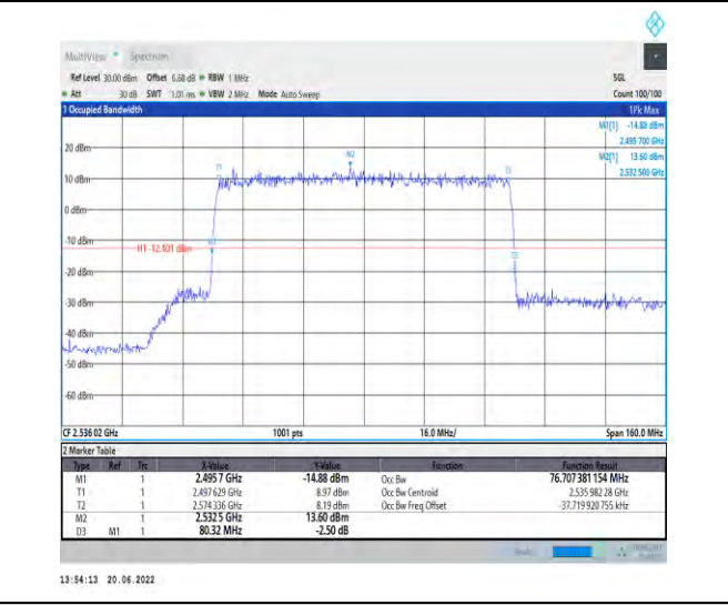
1-N41-PC2-30-80-L-5-DFT-256QAM-Outer_Full-216 @0-Ant1-76.707-80.320-≤80-PASS
