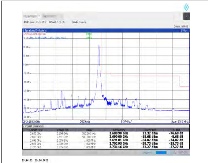
1-N41-PC2-30-40-H-2-DFT-PI2BPSK-Edge_1RB_Right-t-1@105-Ant1-PASS-see graph
