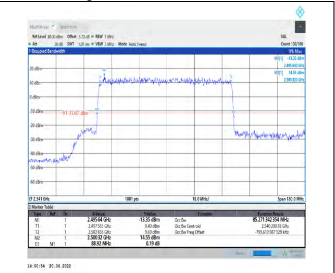
1-N41-PC2-30-90-L-4-DFT-64QAM-Outer_Full-240 @0-Ant1-85.271-88.920-≤90-PASS
