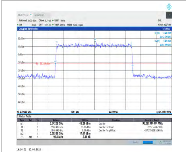
1-N41-PC2-30-100-M-3-DFT-16QAM-Outer_Full-270 @0-Ant1-96.287-99.800-≤100-PASS
