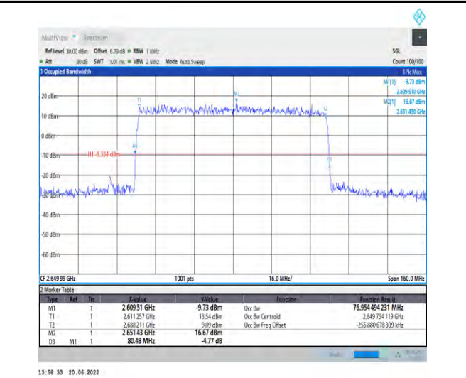
1-N41-PC2-30-80-H-3-DFT-16QAM-Outer_Full-216 @0-Ant1-76.954-80.480-≤80-PASS
