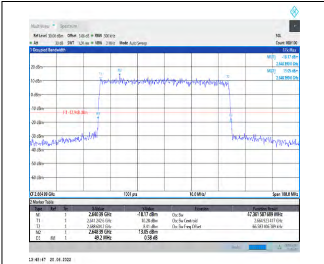
1-N41-PC2-30-50-H-6-CP-QPSK-Outer_Full-133@0 -Ant1-47.362-49.200-≤50-PASS
