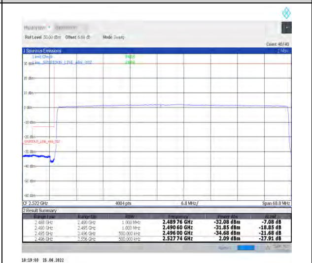
1-N41-PC2-30-60-L-6-CP-QPSK-Outer_Full-162@0-Ant1-PASS-see graph
