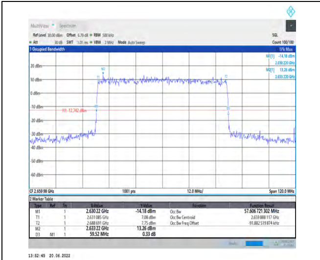
1-N41-PC2-30-60-H-7-CP-16QAM-Outer_Full-162@ 0-Ant1-57.607-59.520-≤60-PASS
