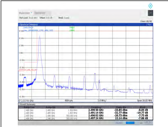
1-N41-PC2-30-50-L-1-DFT-PI2BPSK-Edge_1RB_Left-1@0-Ant1-PASS-see graph
