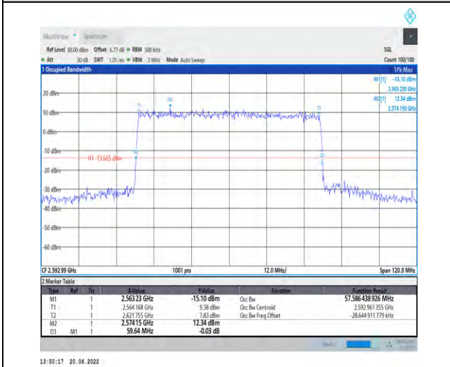
1-N41-PC2-30-60-M-6-CP-QPSK-Outer_Full-162@0 -Ant1-57.586-59.640-≤60-PASS
