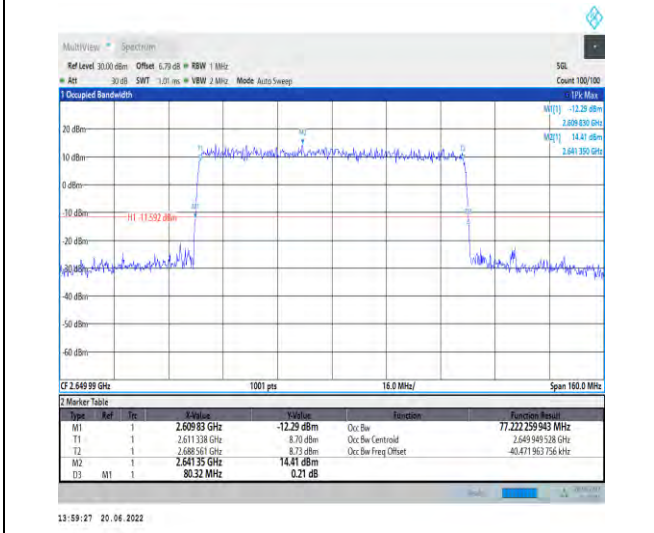
1-N41-PC2-30-80-H-6-CP-QPSK-Outer_Full-217@0 -Ant1-77.222-80.320-≤80-PASS
