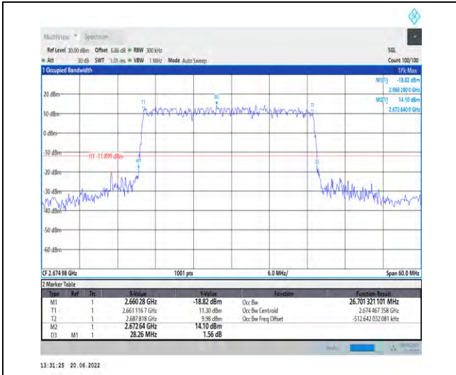
1-N41-PC2-30-30-H-4-DFT-64QAM-Outer_Full-75@ 0-Ant1-26.701-28.260-≤30-PASS
