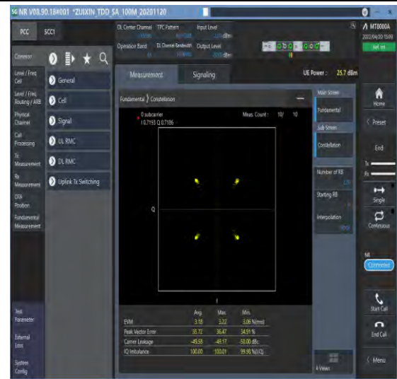
1-N41--30-100-M-2-DFT-QPSK-Outer_Full-270@0- Ant1-see graph-PASS
