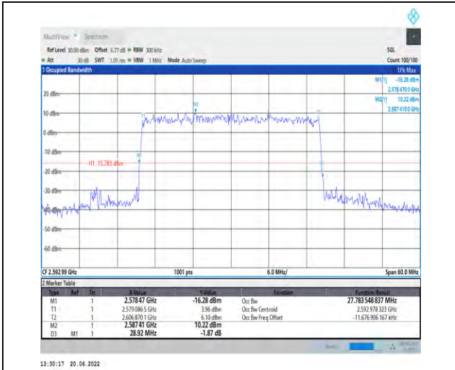
1-N41-PC2-30-30-M-9-CP-256QAM-Outer_Full-78@ 0-Ant1-27.784-28.920-≤30-PASS
