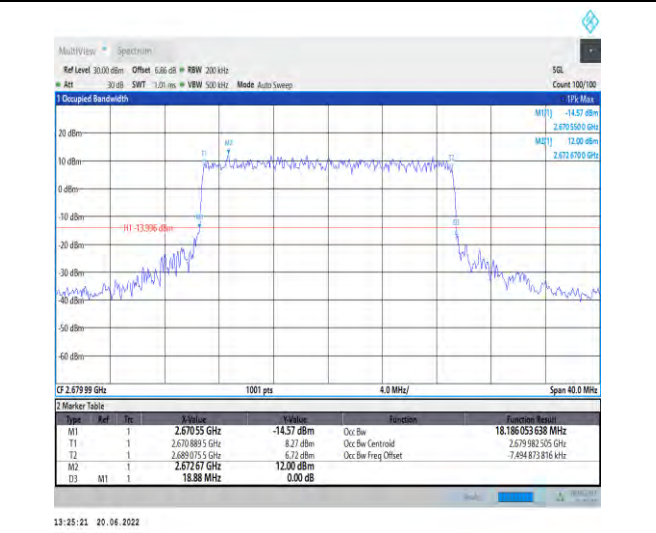
1-N41-PC2-30-20-H-6-CP-QPSK-Outer_Full-51@0- Ant1-18.186-18.880-≤20-PASS
