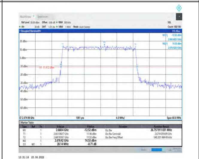
1-N41-PC2-30-30-H-3-DFT-16QAM-Outer_Full-75@ 0-Ant1-26.758-28.140-≤30-PASS
