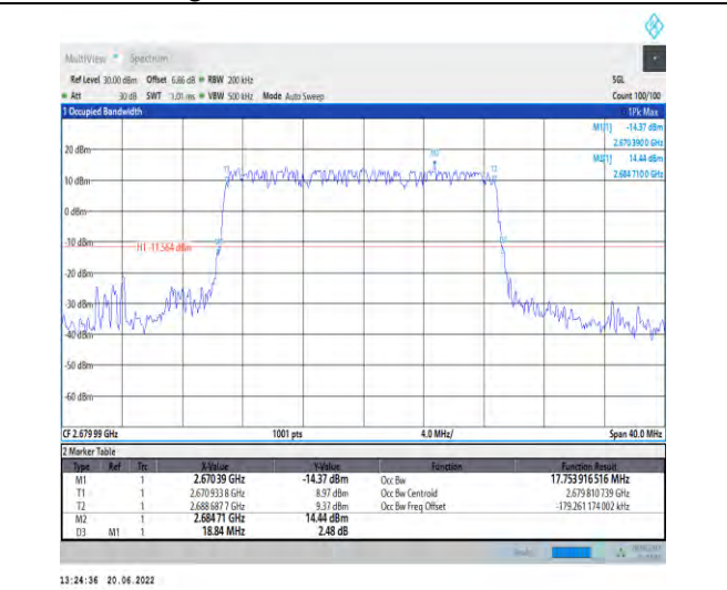
1-N41-PC2-30-20-H-4-DFT-64QAM-Outer_Full-50@ 0-Ant1-17.754-18.840-≤20-PASS
