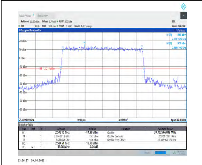
1-N41-PC2-30-40-M-8-CP-64QAM-Outer_Full-106@0 -Ant1-37.763-39.760-≤40-PASS
