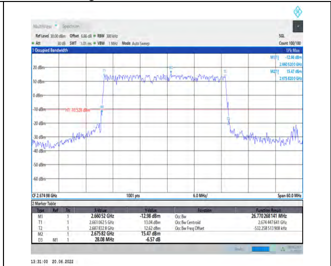
1-N41-PC2-30-30-H-1-DFT-QPSK-Outer_Full-75@0- Ant1-26.77-28.080-≤30-PASS
