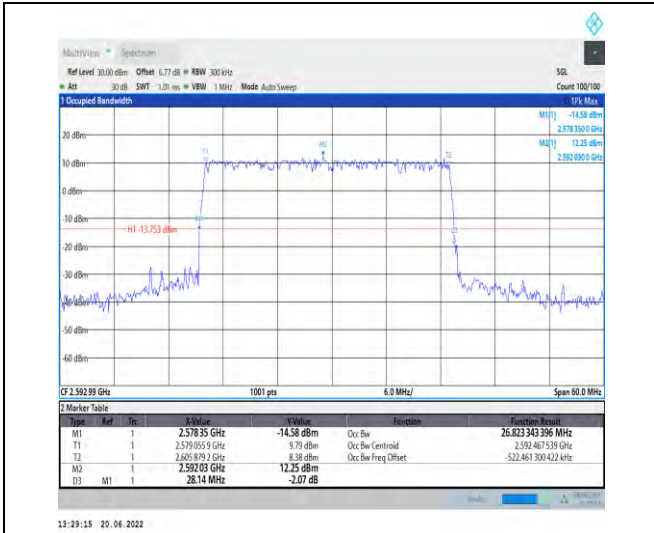
1-N41-PC2-30-30-M-5-DFT-256QAM-Outer_Full-75 @0-Ant1-26.823-28.140-≤30-PASS
