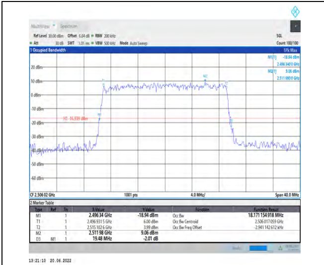
1-N41-PC2-30-20-L-9-CP-256QAM-Outer_Full-51@ 0-Ant1-18.171-19.480-≤20-PASS
