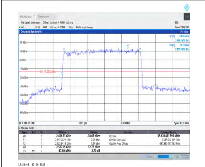
1-N41-PC2-30-40-L-5-DFT-256QAM-Outer_Full-100 @0-Ant1-35.639-37.360-≤40-PASS
