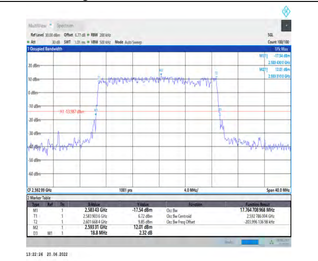
1-N41-PC2-30-20-M-5-DFT-256QAM-Outer_Full-50@ 0-Ant1-17.765-18.800-<20-PASS
