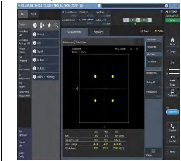
1-N41--30-100-M-6-CP-QPSK-Outer_Full-273@0-Ant1-see graph-PASS
