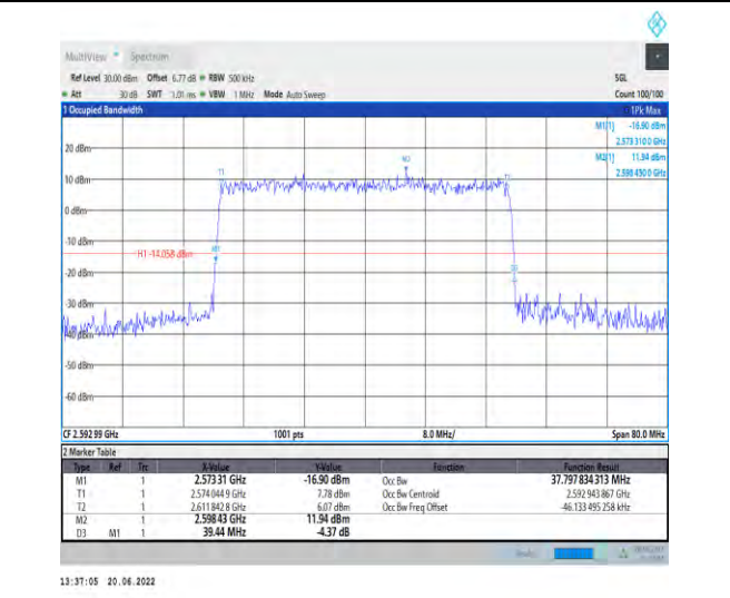
1-N41-PC2-30-40-M-9-CP-256QAM-Outer_Full-106@0 -Ant1-37.798-39.440-≤40-PASS
