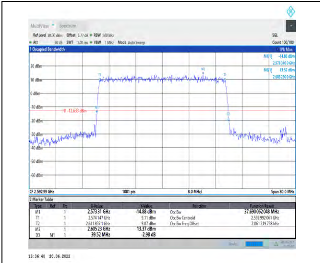
1-N41-PC2-30-40-M-6-CP-QPSK-Outer_Full-106@0 -Ant1-37.69-39.520-≤40-PASS
