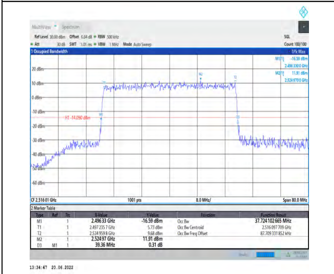
1-N41-PC2-30-40-L-9-CP-256QAM-Outer_Full-106 @0-Ant1-37.724-39.360-≤40-PASS
