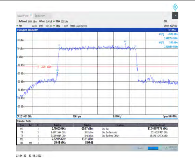
1-N41-PC2-30-40-L-6-CP-QPSK-Outer_Full-106@0-Ant1-37.744-39.440-≤40-PASS
