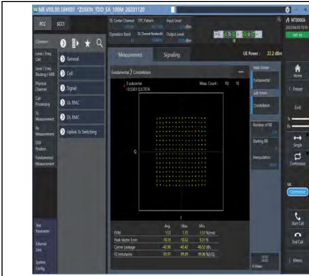
1-N41--30-100-M-5-DFT-256QAM-Outer_Full-270@0-Ant1-see graph-PASS
