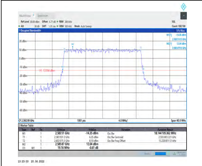
1-N41-PC2-30-20-M-6-CP-QPSK-Outer_Full-51@0- Ant1-18.144-19.160-<20-PASS
