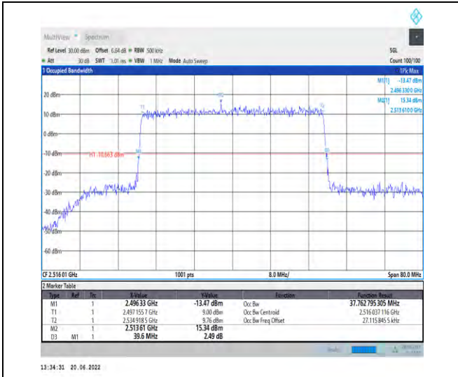
1-N41-PC2-30-40-L-7-CP-16QAM-Outer_Full-106@ 0-Ant1-37.763-39.600-≤40-PASS
