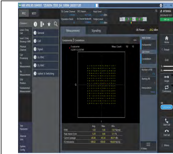
1-N41--30-100-M-9-CP-256QAM-Outer_Full-273@0-Ant1-see graph-PASS
