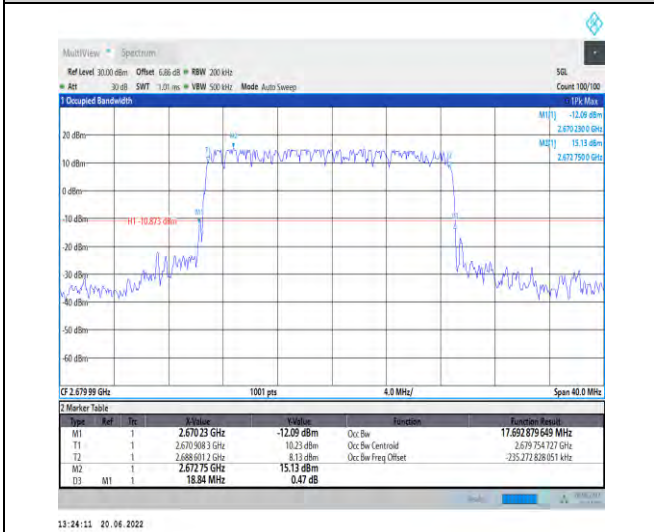
1-N41-PC2-30-20-H-1-DFT-QPSK-Outer_Full-50@0 -Ant1-17.693-18.840-≤20-PASS
