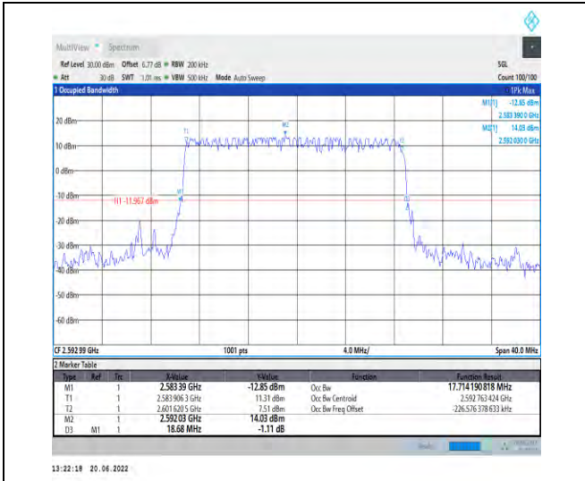
1-N41-PC2-30-20-M-4-DFT-64QAM-Outer_Full-50@ 0-Ant1-17.714-18.680-<20-PASS
