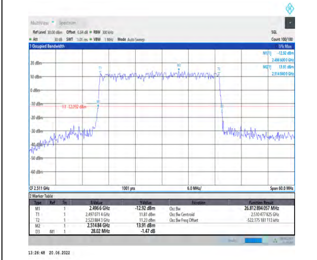
1-N41-PC2-30-30-L-4-DFT-64QAM-Outer_Full-75 @0-Ant1-26.813-28.020-≤30-PASS
