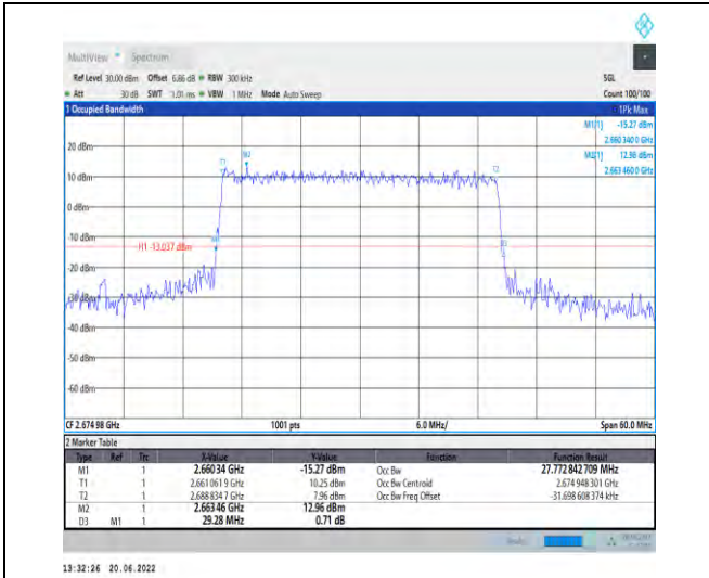
1-N41-PC2-30-30-H-8-CP-64QAM-Outer_Full-78@0 -Ant1-27.773-29.280-≤30-PASS
