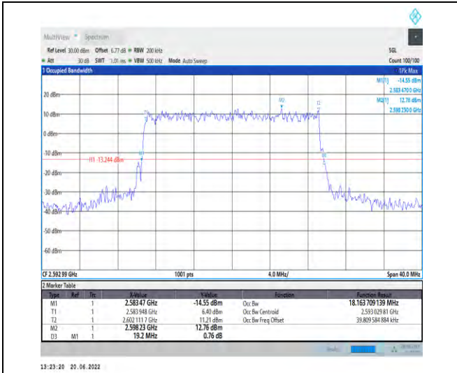
1-N41-PC2-30-20-M-8-CP-64QAM-Outer_Full-51@0 -Ant1-18.164-19.200-≤20-PASS
