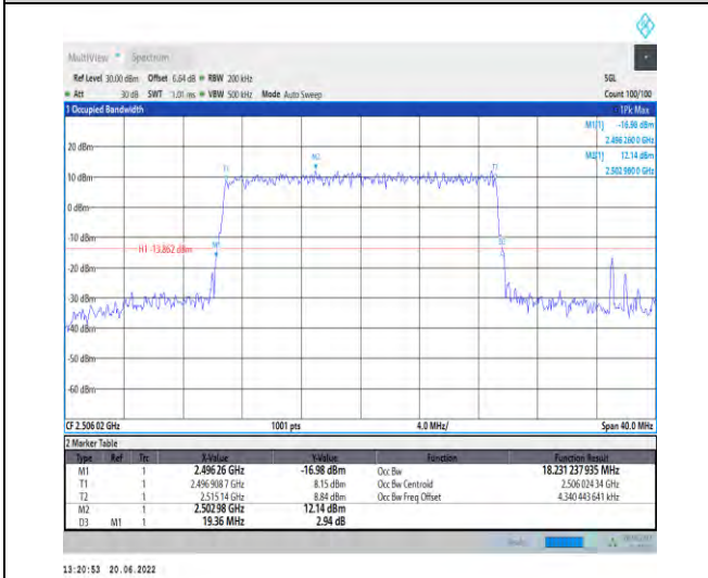
1-N41-PC2-30-20-L-7-CP-16QAM-Outer_Full-51@0-Ant1-18.231-19.360-≤20-PASS
