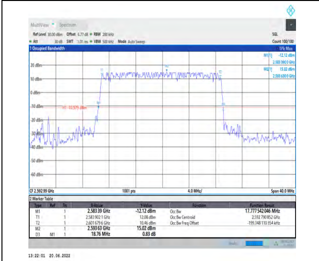
1-N41-PC2-30-20-M-2-DFT-PI2BPSK-Outer_Full-50 @0-Ant1-17.778-18.760-≤20-PASS
