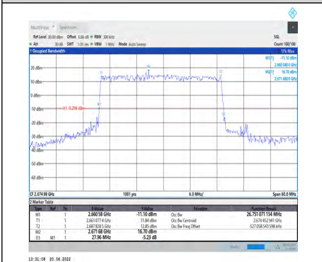
1-N41-PC2-30-30-H-2-DFT-PI2BPSK-Outer_Full-75 @0-Ant1-26.751-27.960-≤30-PASS
