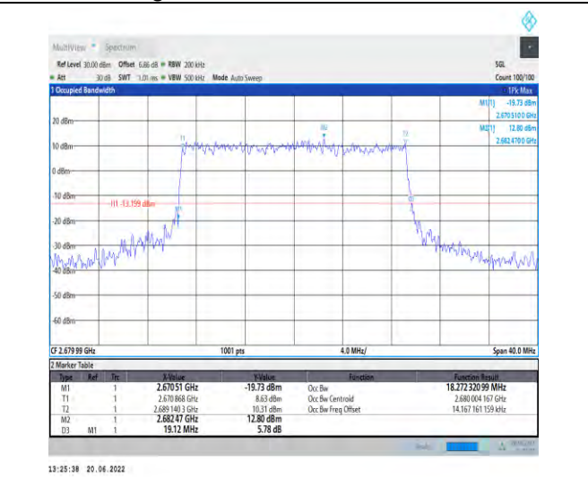
1-N41-PC2-30-20-H-8-CP-64QAM-Outer_Full-51@0 -Ant1-18.272-19.120-≤20-PASS
