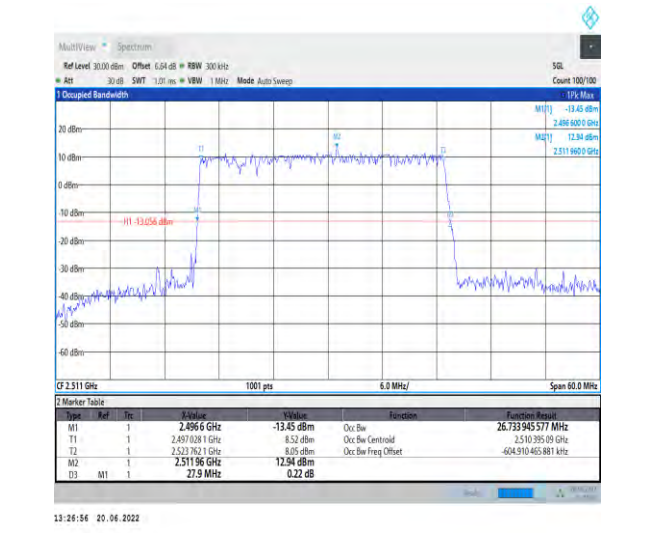
1-N41-PC2-30-30-L-5-DFT-256QAM-Outer_Full-75 @0-Ant1-26.734-27.900-≤30-PASS
