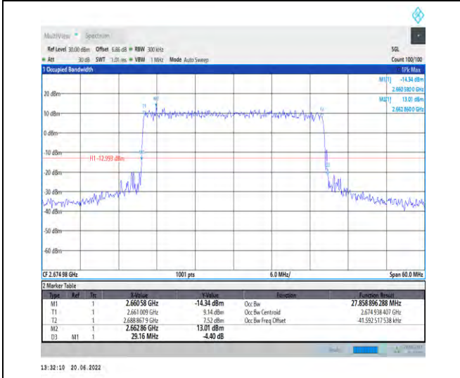
1-N41-PC2-30-30-H-6-CP-QPSK-Outer_Full-78@0- Ant1-27.859-29.160-≤30-PASS
