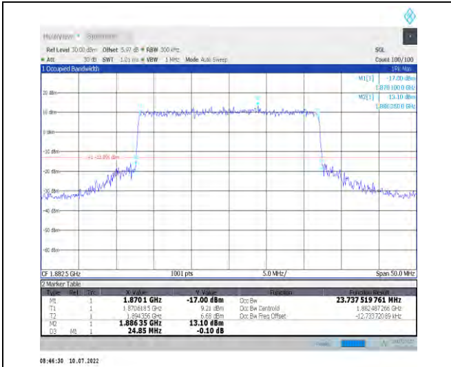
1-N25-PC3-15-25-M-8-CP-64QAM-Outer_Full-133@ 0-Ant1-23.738-24.850-≤25-PASS
