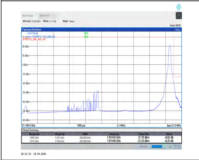
1-N25--15-20-H-5-CP-QPSK-Edge_1RB_Right-1@105 -Ant1-seegraph-PASS-see graph
