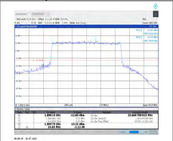
1-N25-PC3-15-25-H-8-CP-64QAM-Outer_Full-133@ 0-Ant1-23.67-24.650-≤25-PASS
