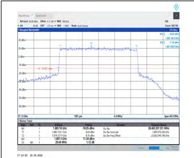
1-N25-PC3-15-30-H-8-CP-64QAM-Outer_Full-160@ 0-Ant1-28.483-29.640-≤30-PASS
