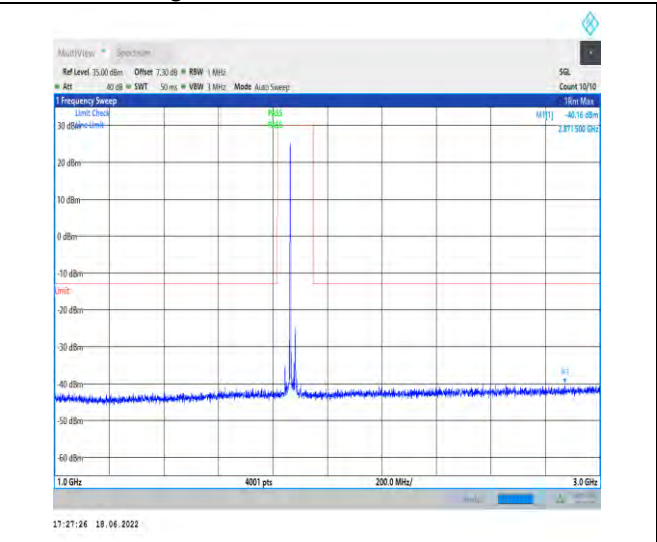
1-N25--15-40-M-1-DFT-PI2BPSK-Inner_1RB_Left-1 @1-1000-3000-Ant1--40.16--13-PASS
