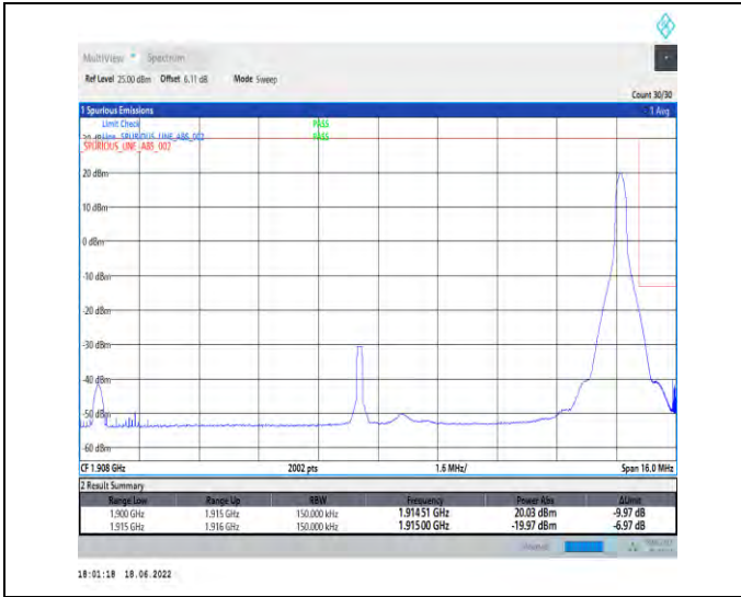
1-N25--15-15-H-2-DFT-PI2BPSK-Edge_1RB_Right-1@78-Ant1-seegraph-PASS-see graph
