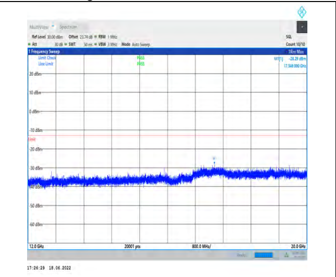
1-N25--15-40-L-1-DFT-PI2BPSK-Inner_1RB_Left-1@ 1-12000-20000-Ant1--28.29--13-PASS
