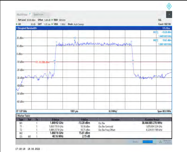
1-N25-PC3-15-40-L-2-DFT-PI2BPSK-Outer_Full-216 @0-Ant1-38.467-40.160-≤40-PASS
