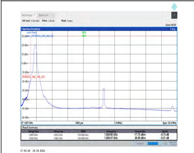
1-N25--15-15-L-4-CP-QPSK-Edge_1RB_Left-1@0-Ant1-seegraph-PASS-see graph
