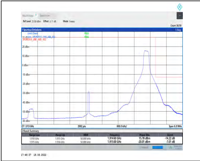
1-N25--15-5-H-2-DFT-PI2BPSK-Edge_1RB_Right-1@24-Ant1-seegraph-PASS-see graph
