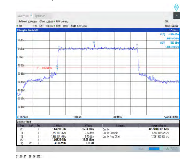
1-N25-PC3-15-40-L-8-CP-64QAM-Outer_Full-216@ 0-Ant1-38.574-40.160-≤40-PASS
