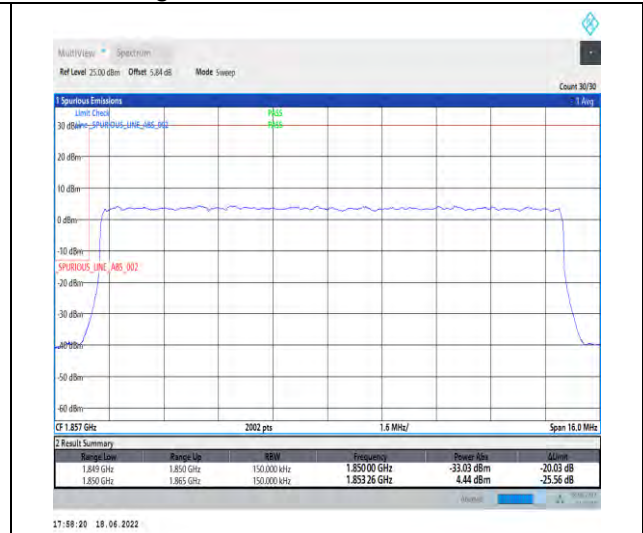
1-N25--15-15-L-3-DFT-PI2BPSK-Outer_Full-75@0-Ant1-seegraph-PASS-see graph
