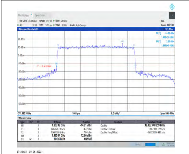
1-N25-PC3-15-40-M-8-CP-64QAM-Outer_Full-216@0 -Ant1-38.433-40.160-≤40-PASS
