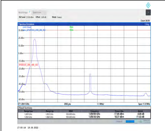
1-N25--15-10-L-1-DFT-PI2BPSK-Edge_1RB_Left-1@0 -Ant1-seegraph-PASS-see graph
