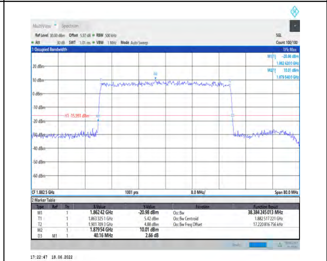
1-N25-PC3-15-40-M-9-CP-256QAM-Outer_Full-216@0 -Ant1-38.384-40.160-≤40-PASS
