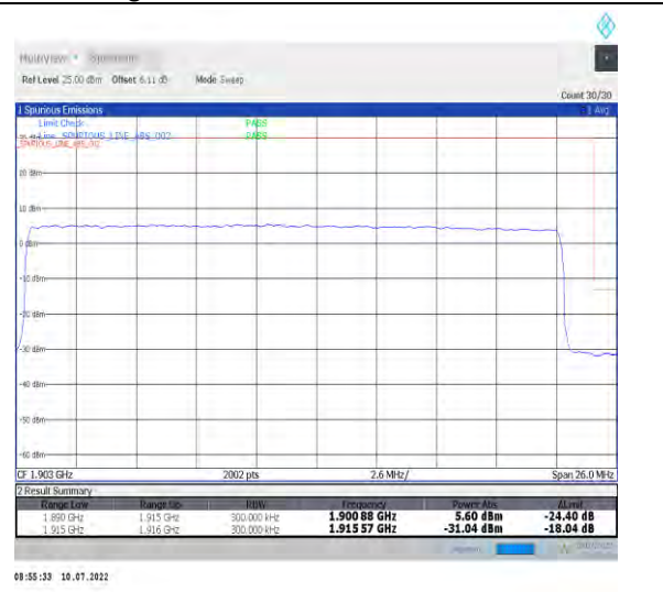
1-N25-PC3-15-25-H-3-DFT-PI2BPSK-Outer_Full-128@0-Ant1-seegraph-PASS-see graph
