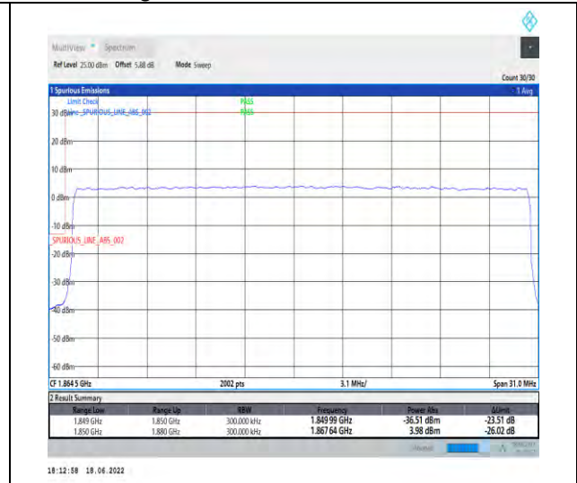
1-N25--15-30-L-3-DFT-PI2BPSK-Outer_Full-160@0-Ant1-seegraph-PASS-see graph
