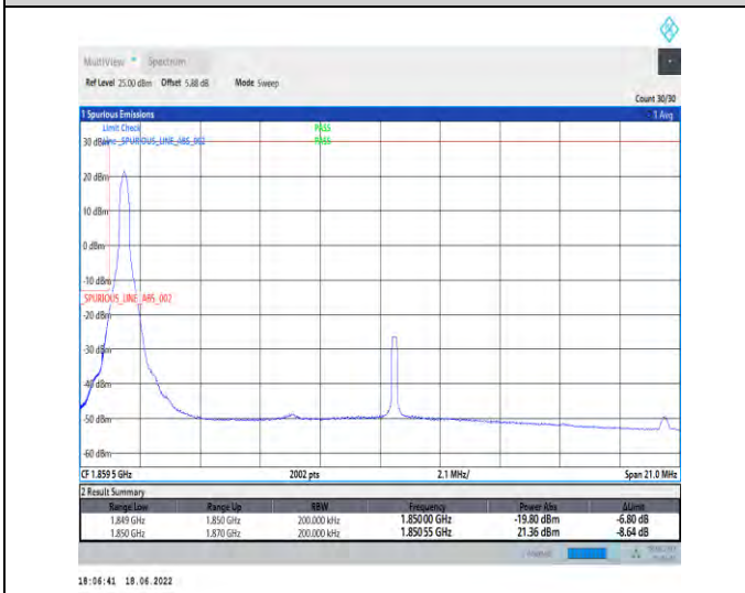
1-N25--15-20-L-4-CP-QPSK-Edge_1RB_Left-1@0-Ant1-seegraph-PASS-see graph
