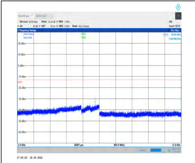
1-N25--15-40-L-1-DFT-PI2BPSK-Inner_1RB_Left-1 @1-3000-12000-Ant1--33.66--13-PASS
