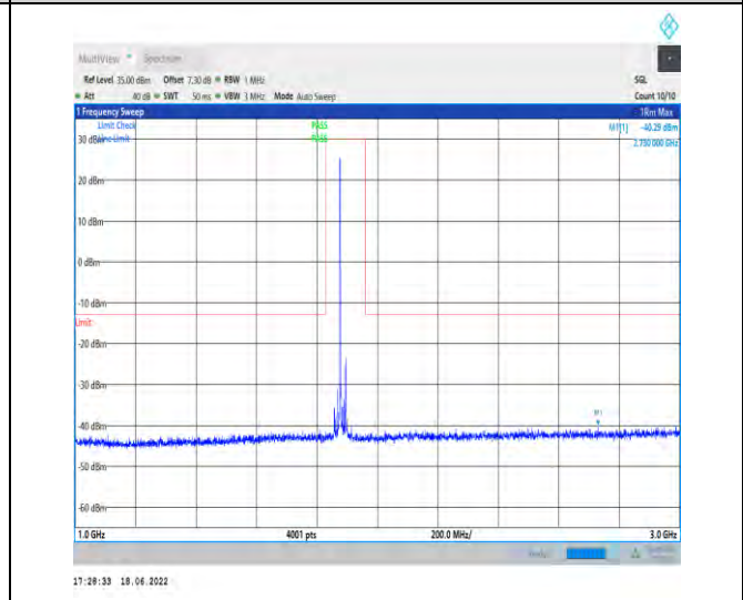
1-N25--15-40-H-1-DFT-PI2BPSK-Inner_1RB_Left-1 @1-1000-3000-Ant1--40.29--13-PASS
