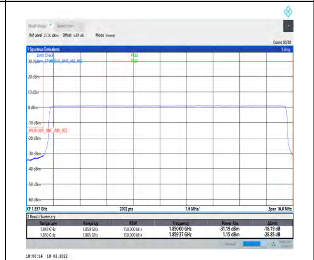
1-N25--15-15-L-6-CP-QPSK-Outer_Full-79@0-Ant1-seegraph-PASS-see graph
