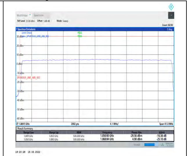
1-N25--15-40-L-3-DFT-PI2BPSK-Outer_Full-216@0-Ant1-seegraph-PASS-see graph
