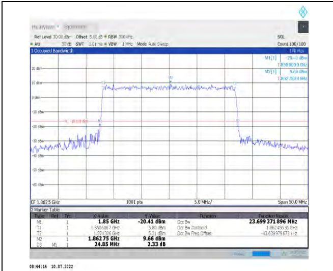
1-N25-PC3-15-25-L-9-CP-256QAM-Outer_Full-133 @0-Ant1-23.699-24.850-≤25-PASS
