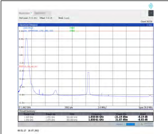
1-N25-PC3-15-25-L-1-DFT-PI2BPSK-Edge_1RB_Left-1@0-Ant1-seegraph-PASS-see graph
