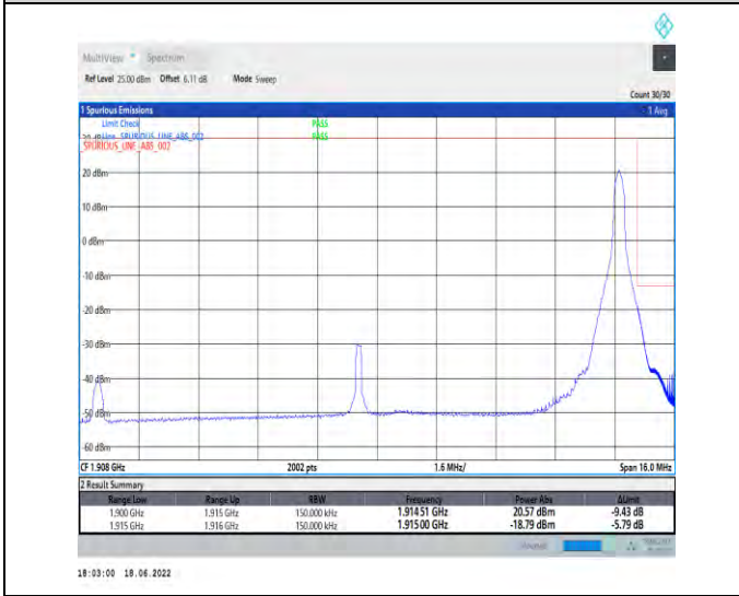
1-N25--15-15-H-5-CP-QPSK-Edge_1RB_Right-1@78-Ant1-seegraph-PASS-see graph
