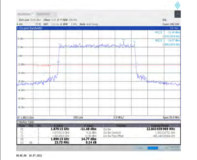
1-N25-PC3-15-25-M-3-DFT-16QAM-Outer_Full-128 @0-Ant1-22.844-23.750-≤25-PASS
