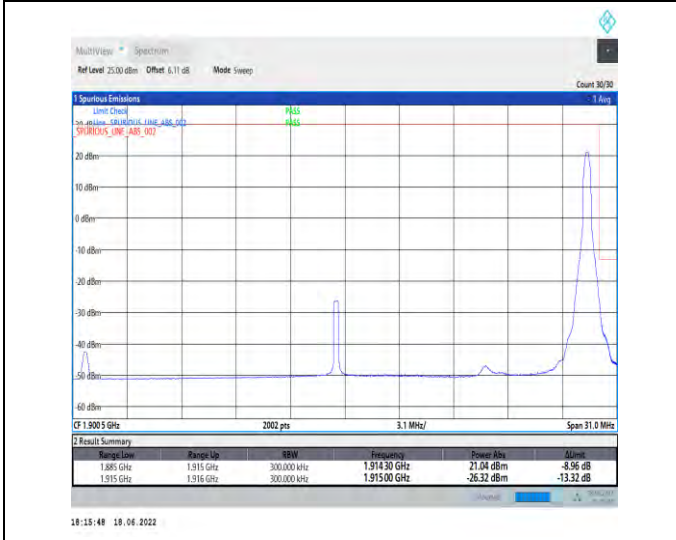
1-N25--15-30-H-2-DFT-PI2BPSK-Edge_1RB_Right-1 @159-Ant1-seegraph-PASS-see graph
