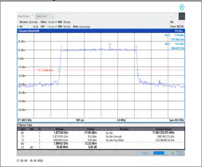
1-N25-PC3-15-20-M-4-DFT-64QAM-Outer_Full-100 @0-Ant1-17.861-18.680-≤20-PASS
