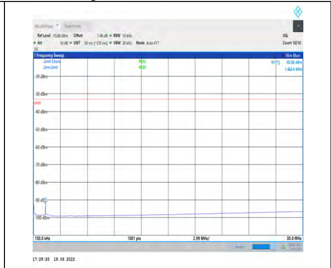
1-N25--15-40-H-1-DFT-PI2BPSK-Inner_1RB_Left-1 @1-0.15-30-Ant1--92.85--33-PASS
