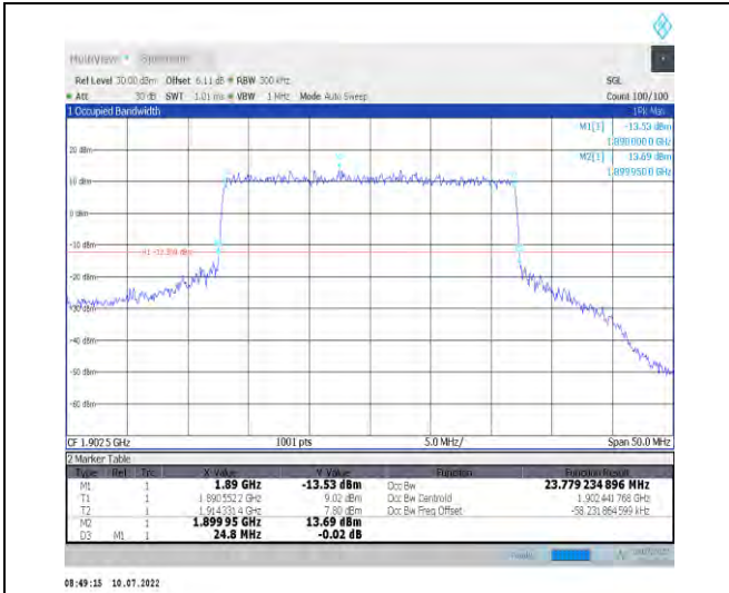
1-N25-PC3-15-25-H-7-CP-16QAM-Outer_Full-133@ 0-Ant1-23.779-24.800-≤25-PASS
