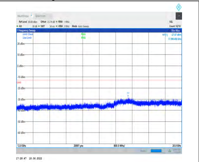
1-N25--15-40-H-1-DFT-PI2BPSK-Inner_1RB_Left-1 @1-12000-20000-Ant1--27.87--13-PASS
