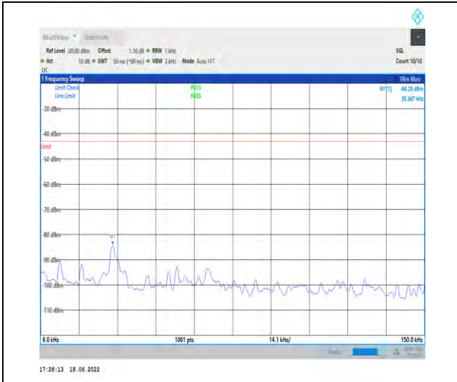
1-N25--15-40-H-1-DFT-PI2BPSK-Inner_1RB_Left-1 @1-0.009-0.15-Ant1--84.28--43-PASS
