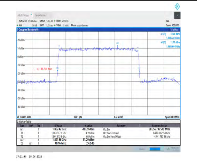
1-N25-PC3-15-40-M-5-DFT-256QAM-Outer_Full-216 @0-Ant1-38.357-40.160-≤40-PASS
