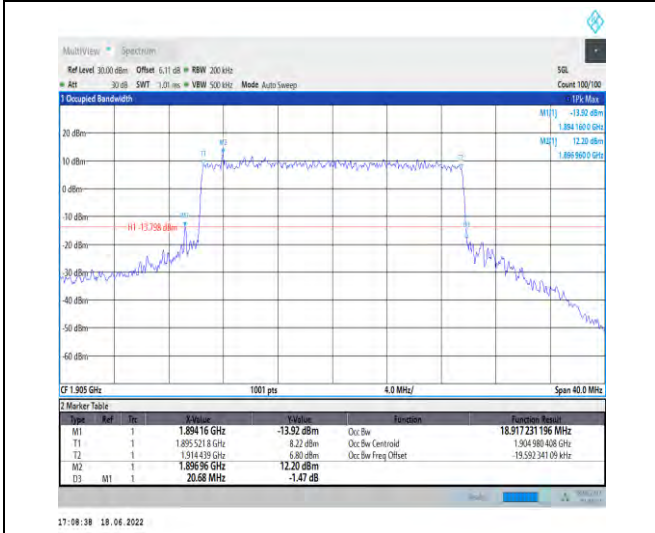
1-N25-PC3-15-20-H-8-CP-64QAM-Outer_Full-106@0 -Ant1-18.917-20.680-≤20-PASS
