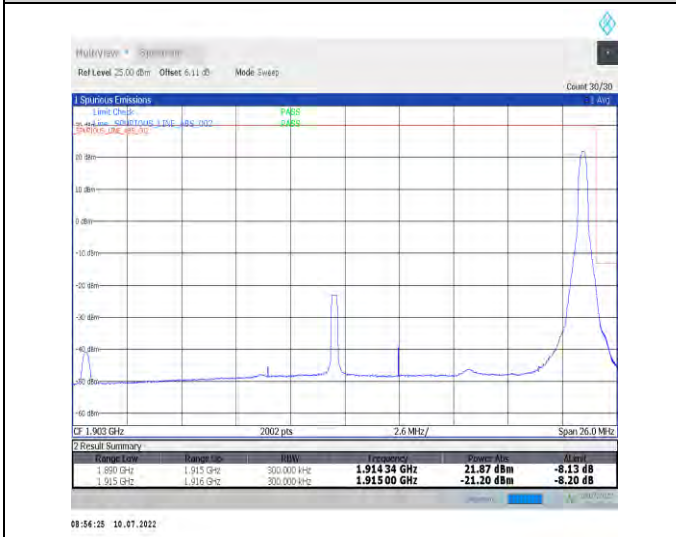
1-N25-PC3-15-25-H-5-CP-QPSK-Edge_1RB_Right-1@132-Ant1-seegraph-PASS-see graph
