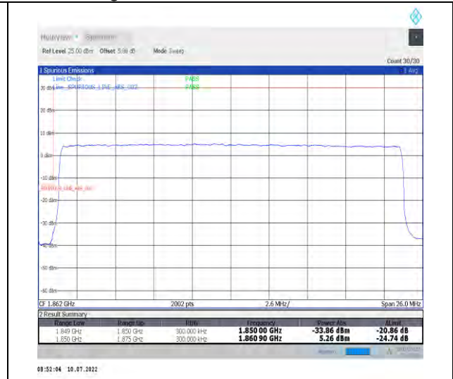
1-N25-PC3-15-25-L-3-DFT-PI2BPSK-Outer_Full-128@0-Ant1-seegraph-PASS-see graph
