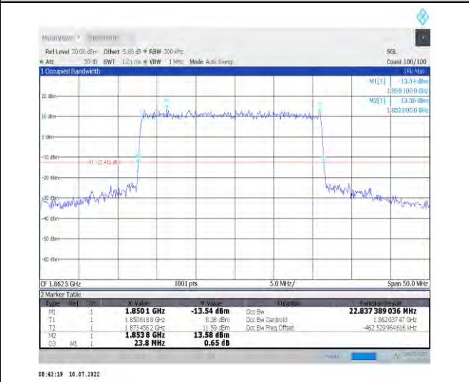
1-N25-PC3-15-25-L-4-DFT-64QAM-Outer_Full-128 @0-Ant1-22.837-23.800-≤25-PASS
