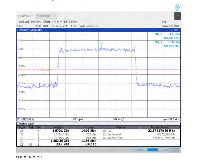
1-N25-PC3-15-25-M-5-DFT-256QAM-Outer_Full-128 @0-Ant1-22.874-23.900-≤25-PASS
