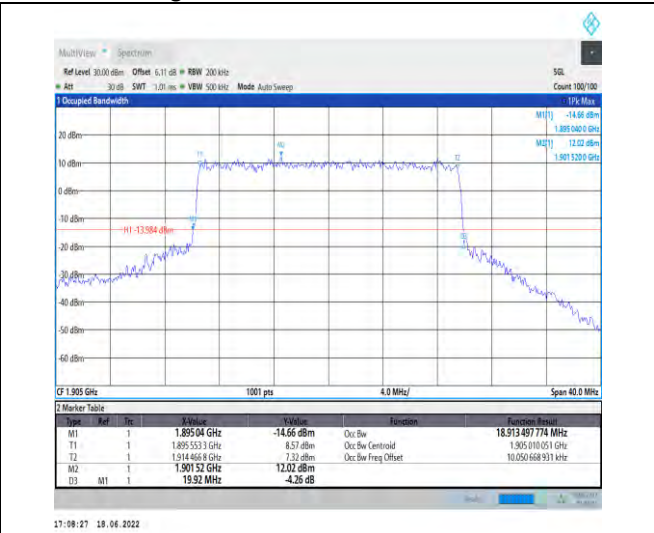
1-N25-PC3-15-20-H-7-CP-16QAM-Outer_Full-106@0 -Ant1-18.913-19.920-≤20-PASS
