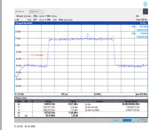
1-N25-PC3-15-40-L-5-DFT-256QAM-Outer_Full-216 @0-Ant1-38.49-40.160-≤40-PASS
