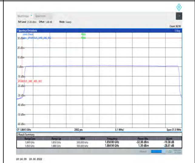
1-N25--15-30-L-6-CP-QPSK-Outer_Full-160@0-Ant1-seegraph-PASS-see graph
