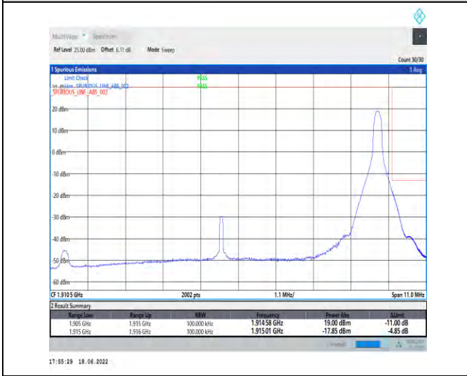
1-N25--15-10-H-5-CP-QPSK-Edge_1RB_Right-1@51-Ant1-seegraph-PASS-see graph
