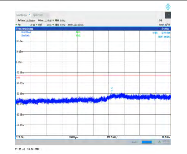
1-N25--15-40-M-1-DFT-PI2BPSK-Inner_1RB_Left-1 @1-12000-20000-Ant1--28.11--13-PASS
