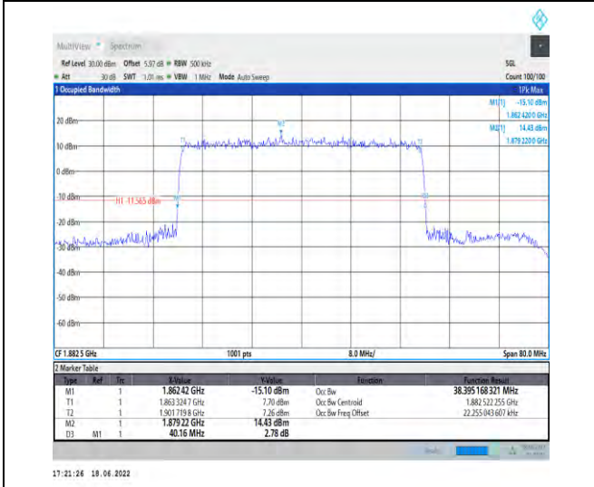
1-N25-PC3-15-40-M-4-DFT-64QAM-Outer_Full-216 @0-Ant1-38.395-40.160-≤40-PASS
