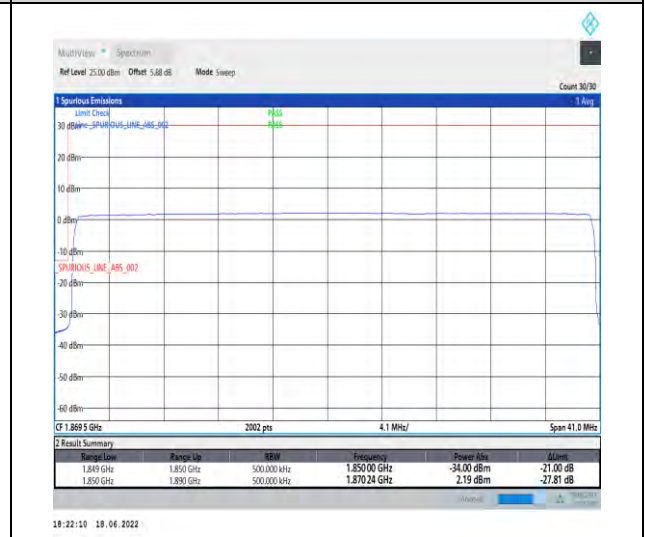
1-N25--15-40-L-6-CP-QPSK-Outer_Full-216@0-Ant1-seegraph-PASS-see graph
