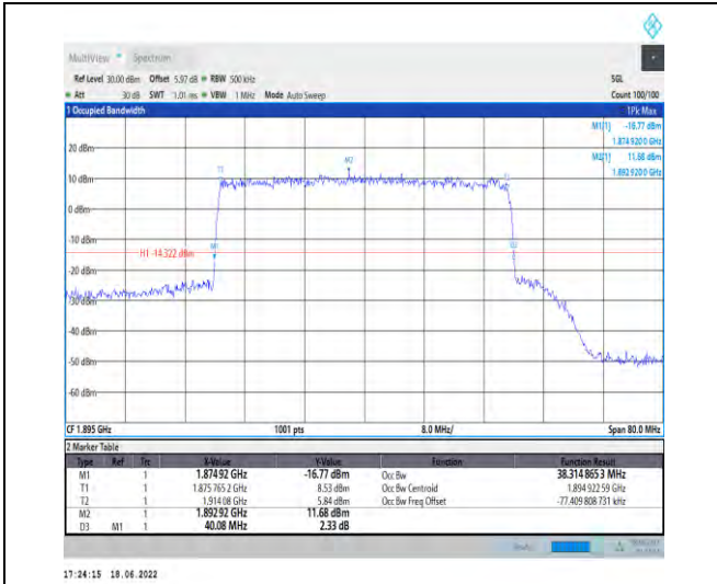
1-N25-PC3-15-40-H-5-DFT-256QAM-Outer_Full-216 @0-Ant1-38.315-40.080-≤40-PASS
