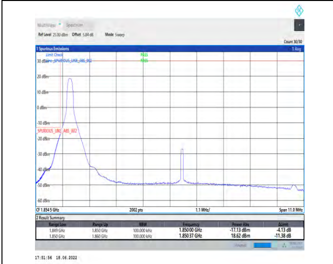
1-N25--15-10-L-4-CP-QPSK-Edge_1RB_Left-1@0-Ant1 1-seegraph-PASS-see graph
