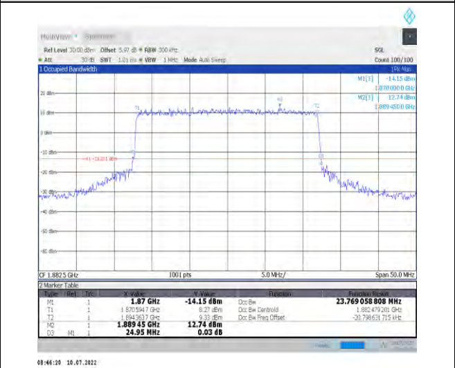
1-N25-PC3-15-25-M-7-CP-16QAM-Outer_Full-133@0 -Ant1-23.769-24.950-≤25-PASS
