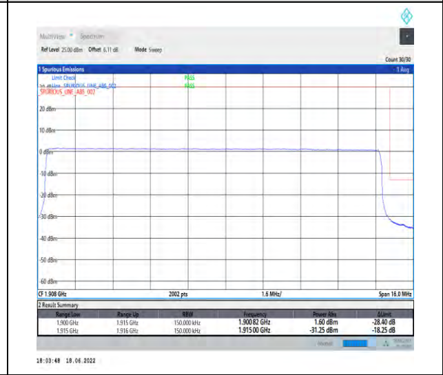
1-N25--15-15-H-6-CP-QPSK-Outer_Full-79@0-Ant1-seegraph-PASS-see graph
