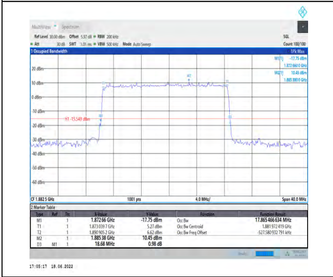
1-N25-PC3-15-20-M-5-DFT-256QAM-Outer_Full-100 @0-Ant1-17.865-18.680-≤20-PASS
