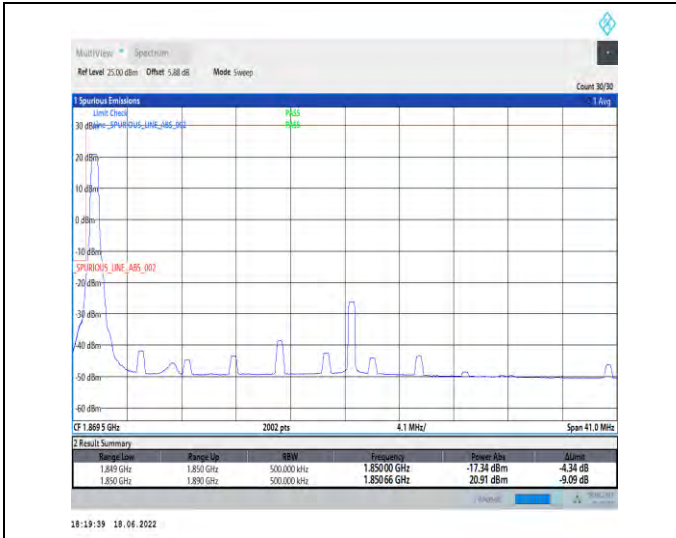
1-N25--15-40-L-1-DFT-PI2BPSK-Edge_1RB_Left-1@0-Ant1-seegraph-PASS-see graph
