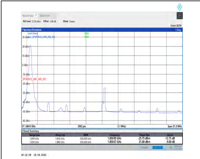
1-N25--15-30-L-1-DFT-PI2BPSK-Edge_1RB_Left-1@0-Ant1-seegraph-PASS-see graph
