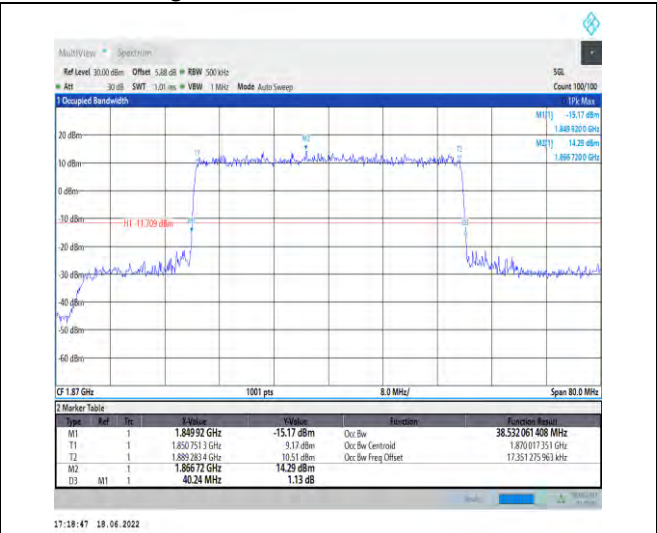
1-N25-PC3-15-40-L-4-DFT-64QAM-Outer_Full-216 @0-Ant1-38.532-40.240-≤40-PASS
