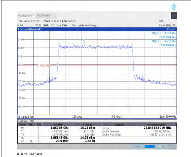
1-N25-PC3-15-25-L-3-DFT-16QAM-Outer_Full-128 @0-Ant1-22.847-23.900-≤25-PASS
