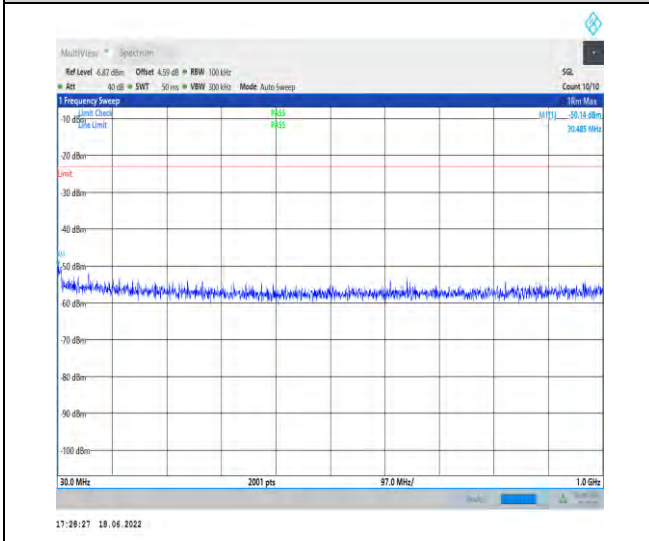
1-N25--15-40-H-1-DFT-PI2BPSK-Inner_1RB_Left-1 @1-30-1000-Ant1--50.14--23-PASS
