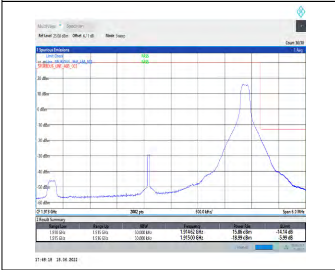
1-N25--15-5-H-5-CP-QPSK-Edge_1RB_Right-1@24-Ant1-seegraph-PASS-see graph
