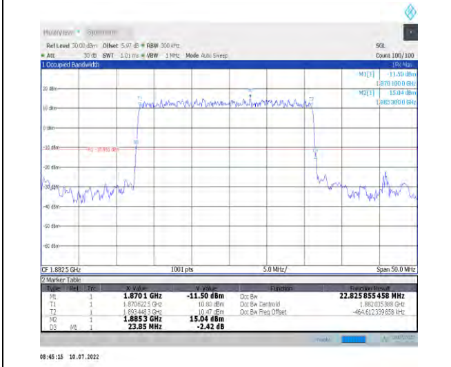
1-N25-PC3-15-25-M-2-DFT-PI2BPSK-Outer_Full-12 8@0-Ant1-22.826-23.850-≤25-PASS
