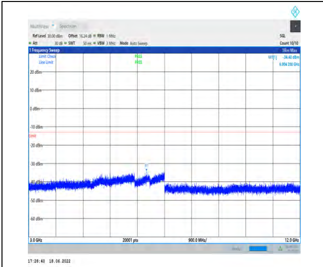
1-N25--15-40-H-1-DFT-PI2BPSK-Inner_1RB_Left-1 @1-3000-12000-Ant1--34.40--13-PASS
