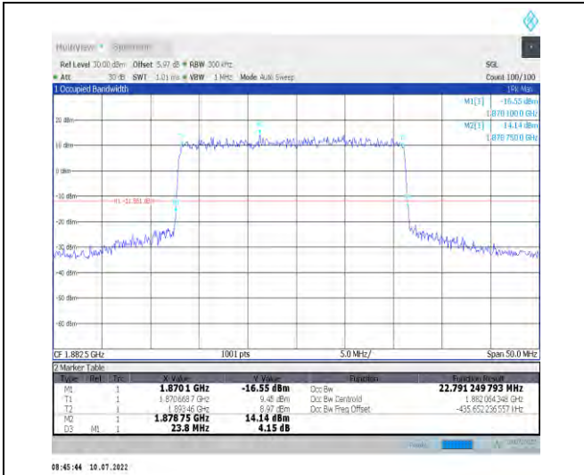
1-N25-PC3-15-25-M-4-DFT-64QAM-Outer_Full-128 @0-Ant1-22.791-23.800-≤25-PASS
