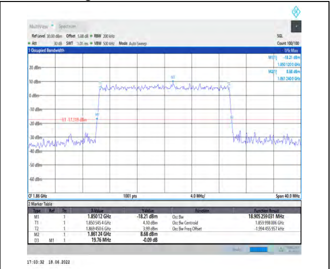
1-N25-PC3-15-20-L-9-CP-256QAM-Outer_Full-106@0-Ant1-18.905-19.760-≤20-PASS
