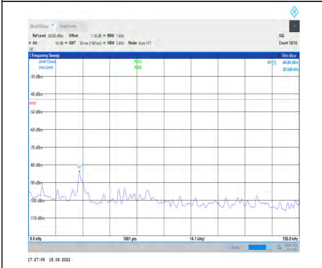
1-N25--15-40-M-1-DFT-PI2BPSK-Inner_1RB_Left-1 @1-0.009-0.15-Ant1--84.80--43-PASS
