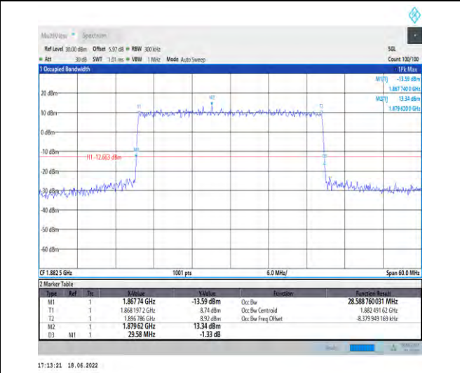
1-N25-PC3-15-30-M-4-DFT-64QAM-Outer_Full-160@0-Ant1-28.589-29.580-≤30-PASS
