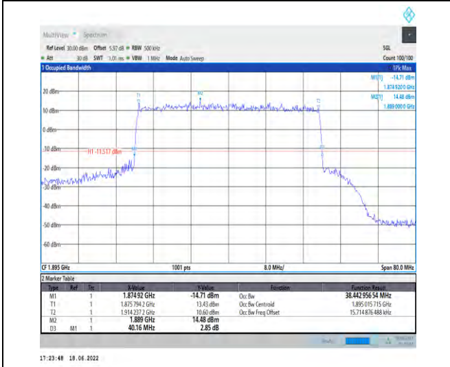
1-N25-PC3-15-40-H-3-DFT-16QAM-Outer_Full-216 @0-Ant1-38.443-40.160-≤40-PASS
