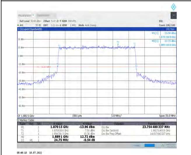
1-N25-PC3-15-25-M-6-CP-QPSK-Outer_Full-133@0 -Ant1-23.754-24.750-≤25-PASS
