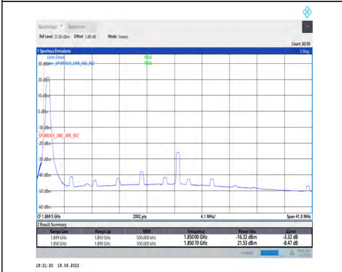
1-N25--15-40-L-4-CP-QPSK-Edge_1RB_Left-1@0-Ant1-seegraph-PASS-see graph
