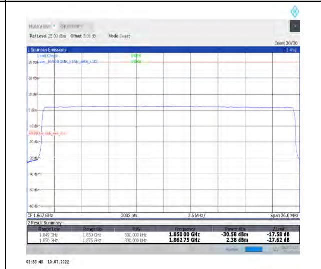
1-N25-PC3-15-25-L-6-CP-QPSK-Outer_Full-133@0-Ant1-seegraph-PASS-see graph
