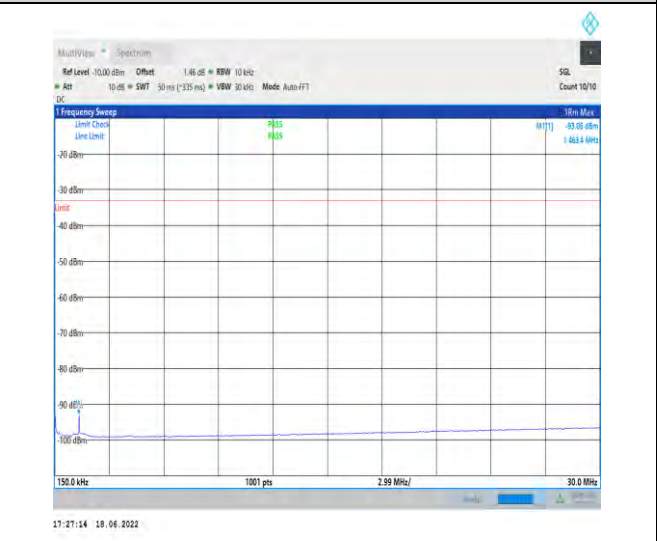
1-N25--15-40-M-1-DFT-PI2BPSK-Inner_1RB_Left-1 @1-0.15-30-Ant1--93.06--33-PASS
