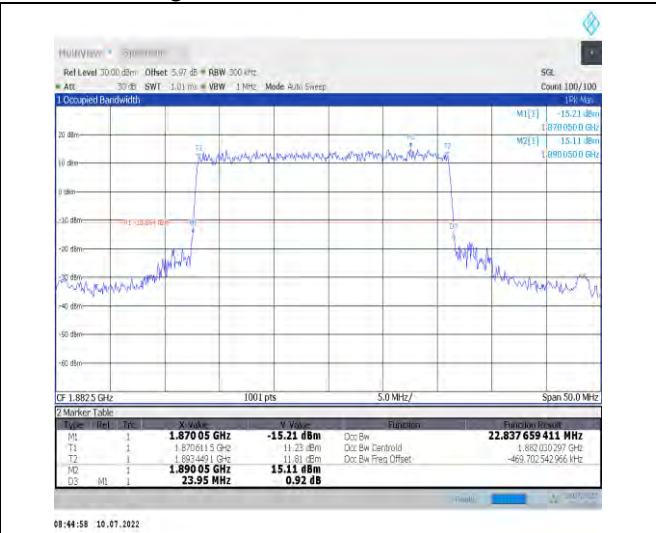
1-N25-PC3-15-25-M-1-DFT-QPSK-Outer_Full-128 @0-Ant1-22.838-23.950-≤25-PASS
