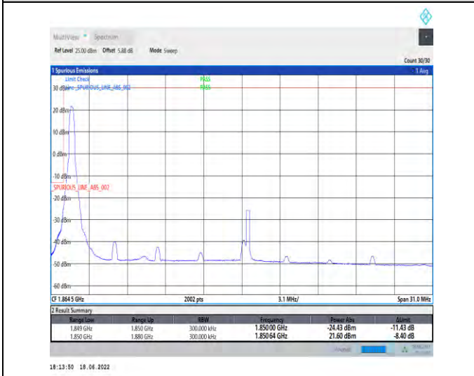
1-N25--15-30-L-4-CP-QPSK-Edge_1RB_Left-1@0-Ant1-seegraph-PASS-see graph
