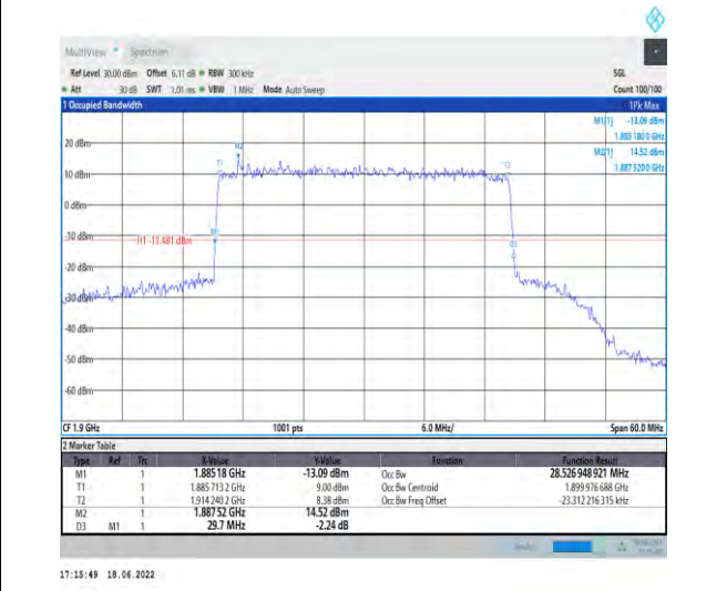
1-N25-PC3-15-30-H-3-DFT-16QAM-Outer_Full-160 @0-Ant1-28.527-29.700-≤30-PASS
