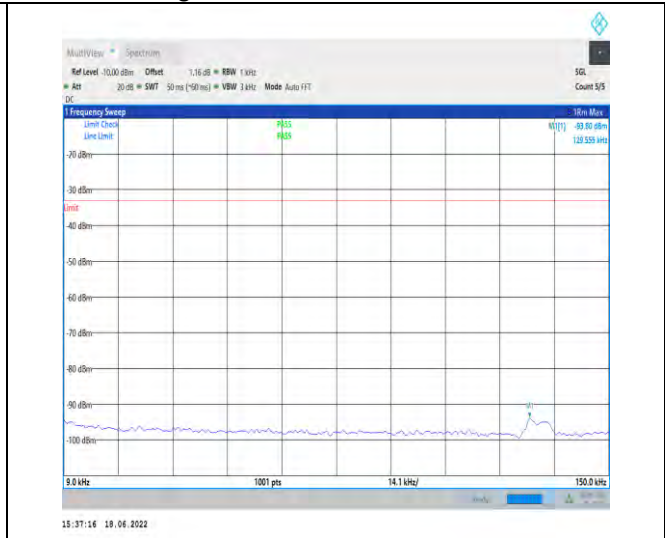
1-N5--15-20-M-1-DFT-PI2BPSK-Inner_1RB_Left-1@ 1-0.009-0.15-Ant1--93.80--33-PASS
