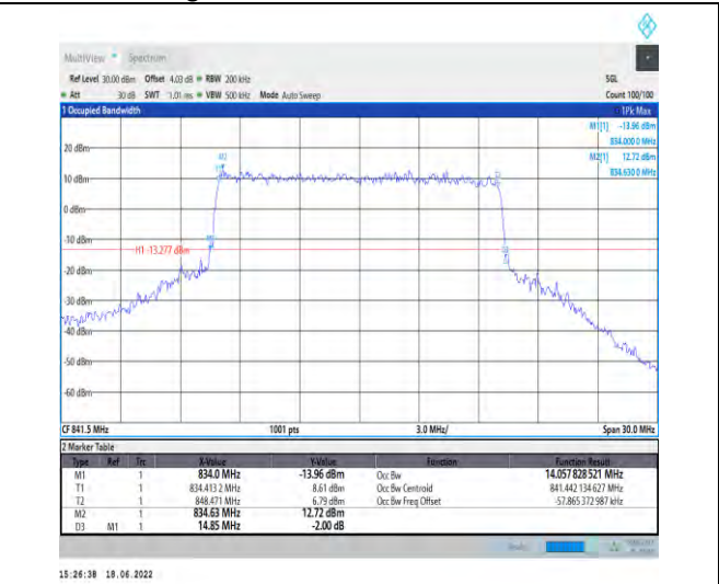
1-N5--15-15-H-6-CP-QPSK-Outer_Full-79@0-Ant1-1 4.058-14.850-≤15-PASS
