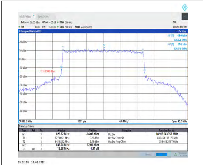
1-N5--15-20-M-7-CP-16QAM-Outer_Full-106@0-Ant 1-18.918-19.680-≤20-PASS
