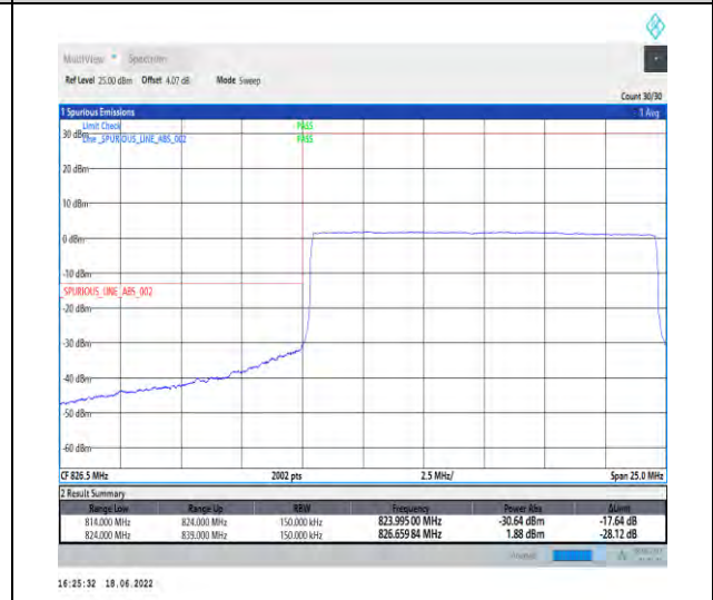
1-N5--15-15-L-6-CP-QPSK-Outer_Full-79@0-Ant1-seegraph-PASS-see graph
