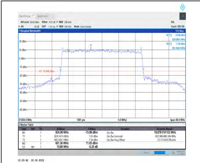
1-N5--15-20-L-8-CP-64QAM-Outer_Full-106@0-Ant 1-18.879-19.840-≤20-PASS
