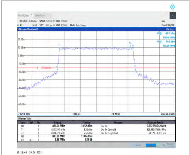
1-N5--15-10-L-6-CP-QPSK-Outer_Full-52@0-Ant1-9 9.292-9.880-≤10-PASS
