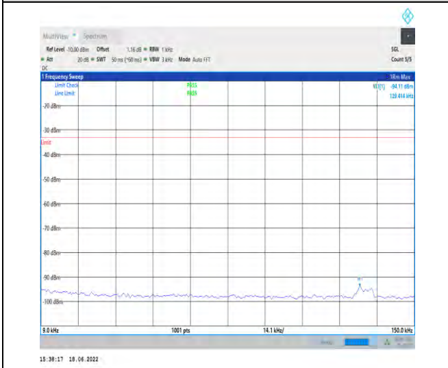
1-N5--15-20-H-1-DFT-PI2BPSK-Inner_1RB_Left-1@ 1-0.009-0.15-Ant1--94.11--33-PASS
