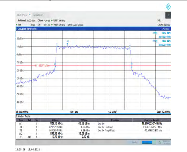
1-N5--15-20-H-7-CP-16QAM-Outer_Full-106@0-Ant1-18.861-19.720-≤20-PASS
