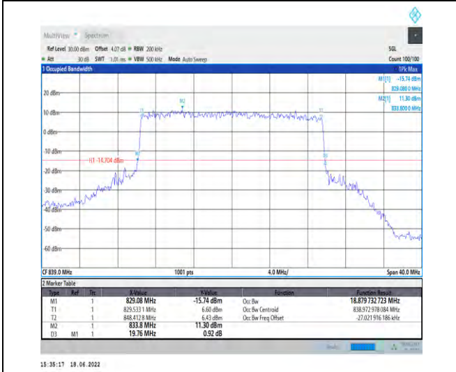
1-N5--15-20-H-8-CP-64QAM-Outer_Full-106@0-Ant1-18.88-19.760-≤20-PASS
