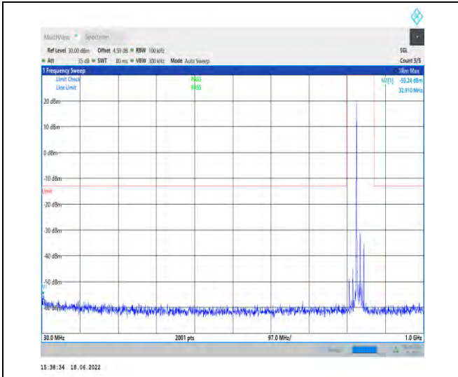
1-N5--15-20-H-1-DFT-PI2BPSK-Inner_1RB_Left-1@ 1-30-1000-Ant1--55.24--13-PASS
