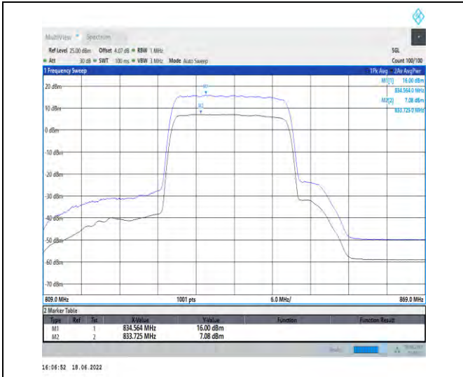
1-N5--15-20-H-1-DFT-256QAM-Outer_Full-100@0-A nt1-8.92-100%-0.00-8.92-PASS-≤13
