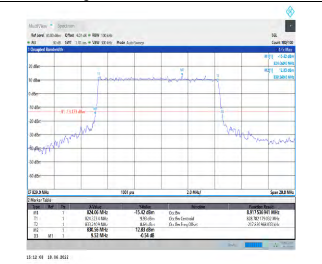
1-N5--15-10-L-3-DFT-16QAM-Outer_Full-50@0-Ant1 -8.918-9.520-≤10-PASS
