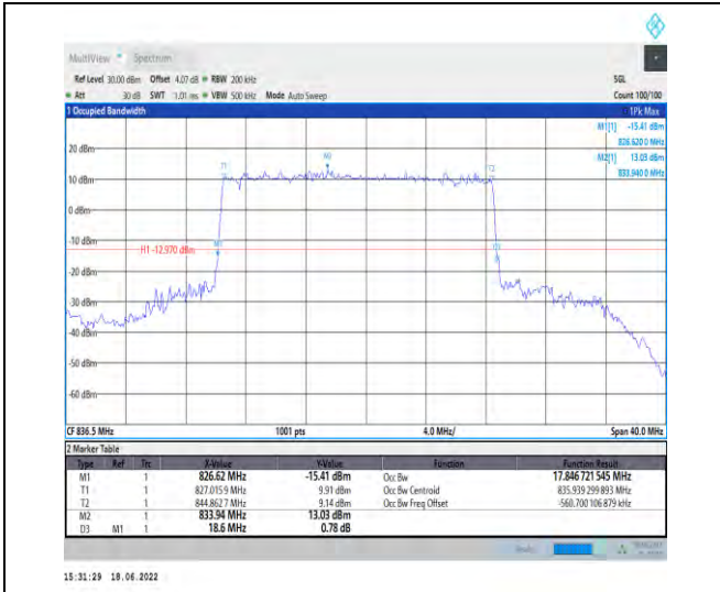
1-N5--15-20-M-3-DFT-16QAM-Outer_Full-100@0-A nt1-17.847-18.600-≤20-PASS
