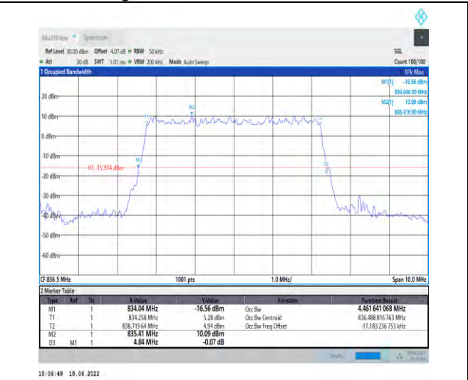
1-N5--15-5-M-5-DFT-256QAM-Outer_Full-25@0-Ant 1-4.462-4.840-≤5-PASS
