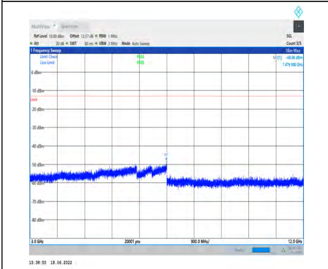
1-N5--15-20-H-1-DFT-PI2BPSK-Inner_1RB_Left-1@ 1-3000-12000-Ant1--48.06--13-PASS
