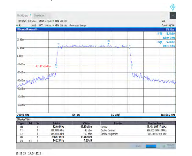
1-N5--15-15-M-3-DFT-16QAM-Outer_Full-75@0-Ant 1-13.432-14.220-≤15-PASS
