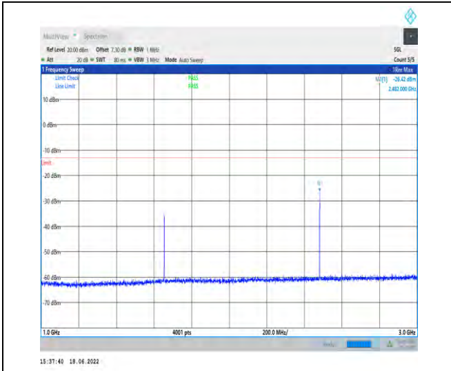
1-N5--15-20-M-1-DFT-PI2BPSK-Inner_1RB_Left-1@ 1-1000-3000-Ant1--26.42--13-PASS
