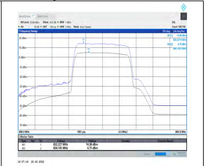
1-N5--15-20-H-2-CP-256QAM-Outer_Full-106@0-A nt1-9.63-100%-0.00-9.63-PASS-≤13
