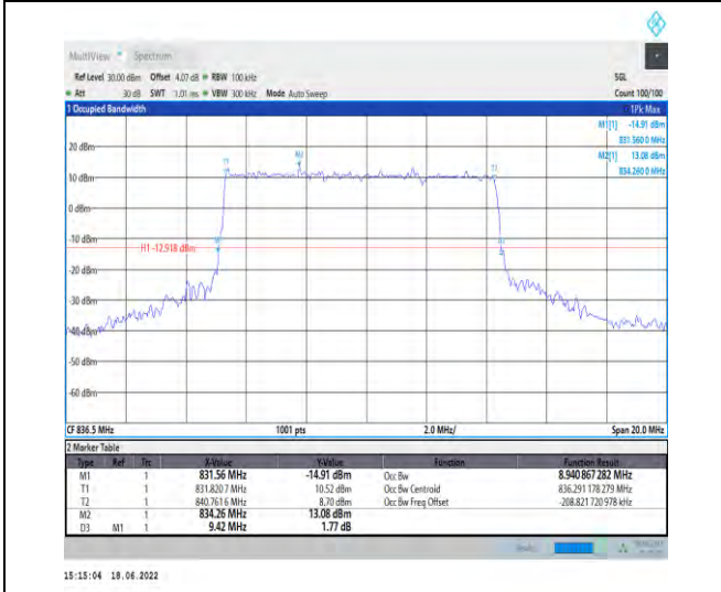
1-N5--15-10-M-3-DFT-16QAM-Outer_Full-50@0-Ant1 1-8.941-9.420-≤10-PASS
