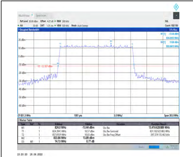
1-N5--15-15-L-3-DFT-16QAM-Outer_Full-75@0-Ant 1-13.417-14.130≤15-PASS
