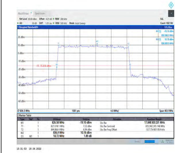
1-N5--15-20-M-5-DFT-256QAM-Outer_Full-100@0-A nt1-17.848-18.720-≤20-PASS
