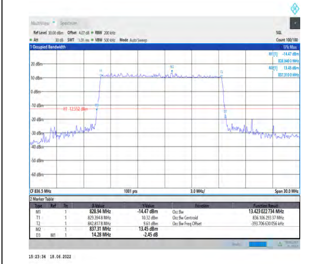
1-N5--15-15-M-4-DFT-64QAM-Outer_Full-75@0-Ant 1-13.423-14.280-≤15-PASS
