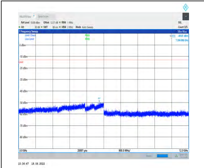
1-N5--15-20-L-1-DFT-PI2BPSK-Inner_1RB_Left-1@ 1-3000-12000-Ant1--49.81--13-PASS
