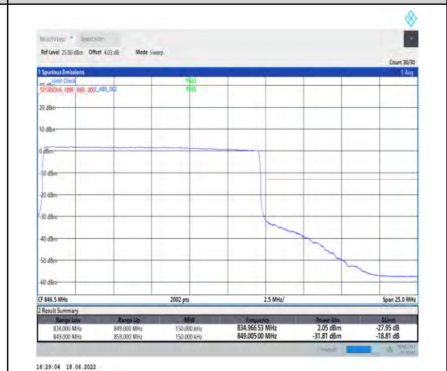
1-N5--15-15-H-6-CP-QPSK-Outer_Full-79@0-Ant1-seegraph-PASS-see graph
