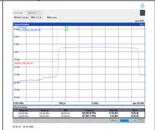
1-N5--15-20-L-3-DFT-PI2BPSK-Outer_Full-100@0-Ant1-seegraph-PASS-see graph
