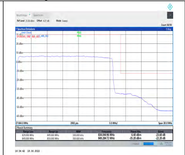
1-N5--15-20-H-3-DFT-PI2BPSK-Outer_Full-100@0-Ant1-seegraph-PASS-see graph
