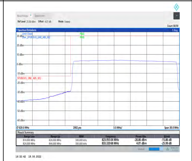
1-N5--15-20-L-6-CP-QPSK-Outer_Full-106@0-Ant1-seegraph-PASS-see graph
