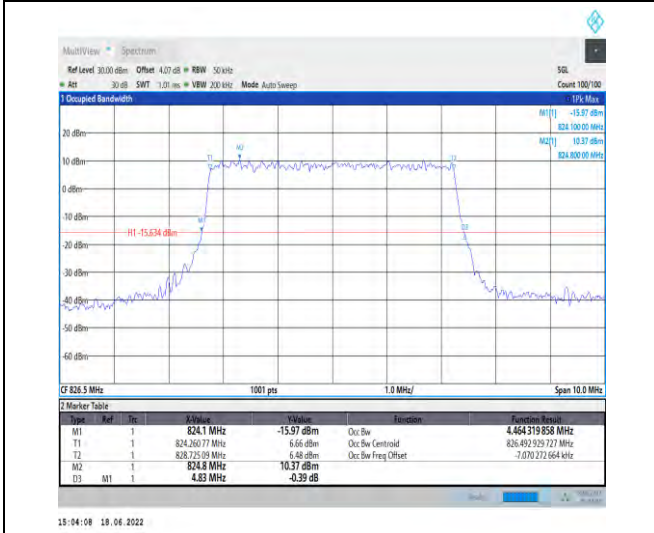
1-N5--15-5-L-7-CP-16QAM-Outer_Full-25@0-Ant1-4 .464-4.830-≤5-PASS
