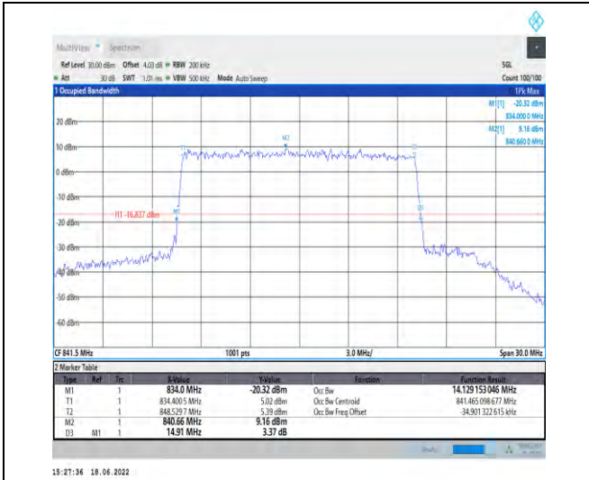
1-N5--15-15-H-9-CP-256QAM-Outer_Full-79@0-Ant 1-14.129-14.910-≤15-PASS
