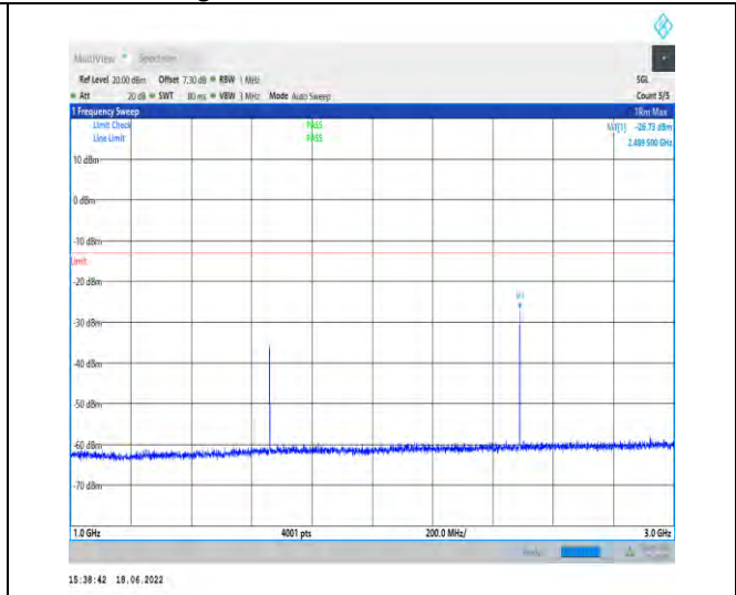
1-N5--15-20-H-1-DFT-PI2BPSK-Inner_1RB_Left-1@ 1-1000-3000-Ant1--26.73--13-PASS
