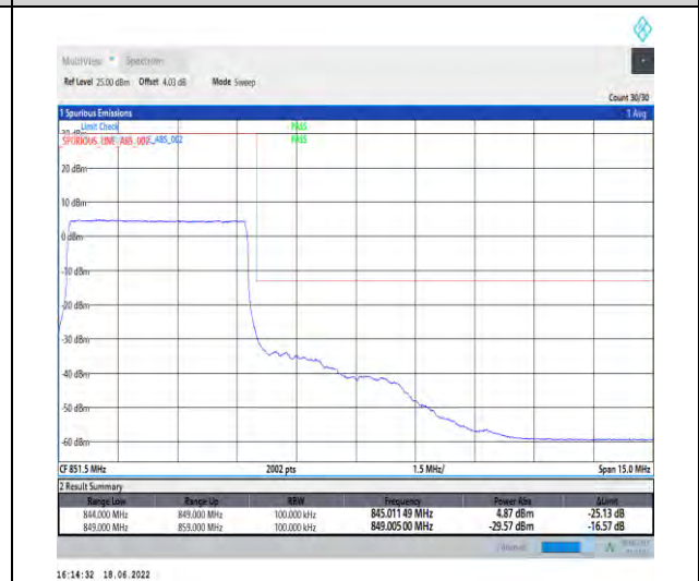
1-N5--15-5-H-6-CP-QPSK-Outer_Full-25@0-Ant1 seegraph-PASS-see graph
