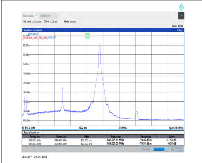
1-N5--15-10-H-5-CP-QPSK-Edge_1RB_Right-1@51-Ant1-seegraph-PASS-see graph
