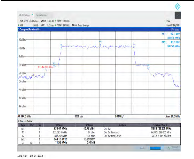
1-N5--15-10-H-2-DFT-PI2BPSK-Outer_Full-50@0-A nt1-8.939-11.560-≤10-PASS
