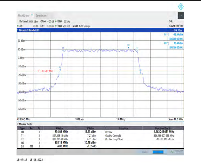
1-N5--15-5-M-7-CP-16QAM-Outer_Full-25@0-Ant1- 4.462-4.820-≤5-PASS
