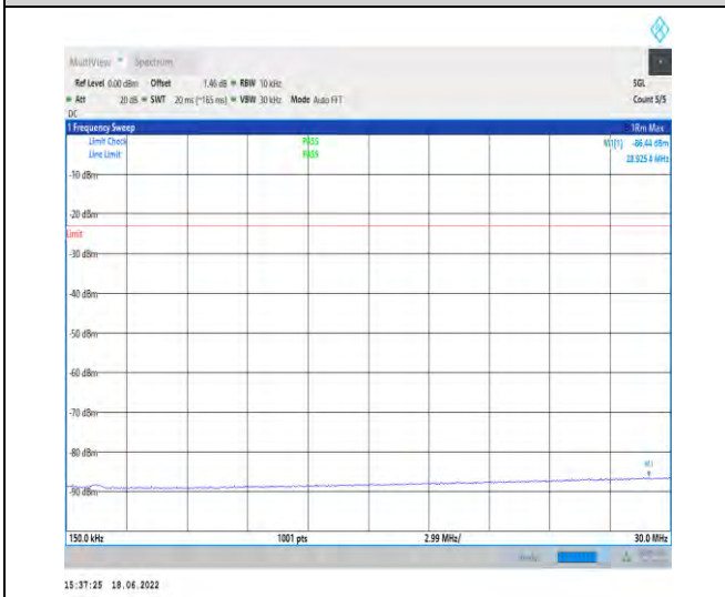
1-N5--15-20-M-1-DFT-PI2BPSK-Inner_1RB_Left-1@ 1-0.15-30-Ant1--86.44--23-PASS
