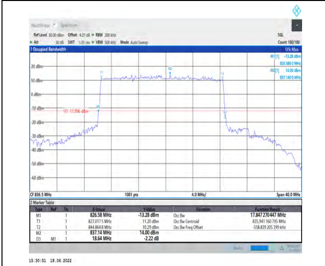
1-N5--15-20-M-1-DFT-QPSK-Outer_Full-100@0-Ant 1-17.847-18.640-≤20-PASS
