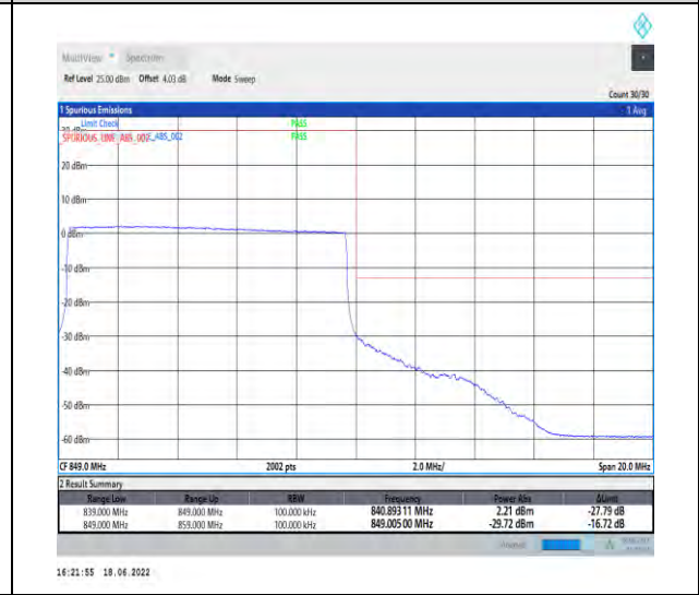
1-N5--15-10-H-6-CP-QPSK-Outer_Full-52@0-Ant1-seegraph-PASS-see graph
