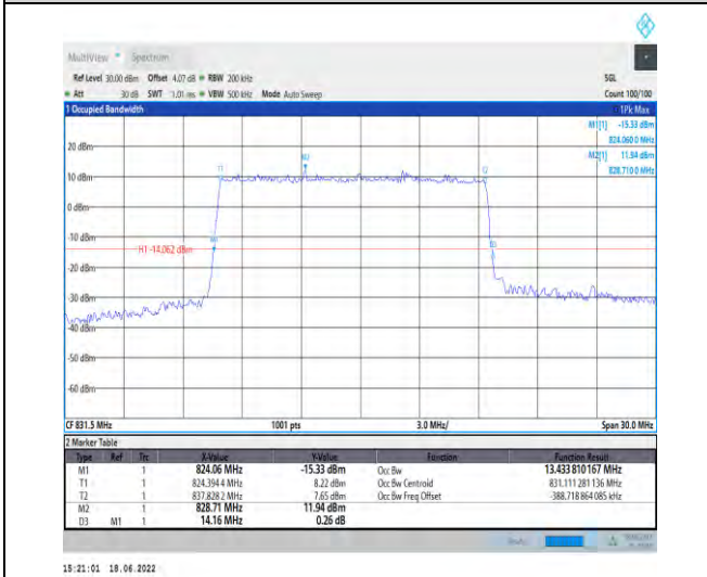
1-N5--15-15-L-5-DFT-256QAM-Outer_Full-75@0-An t1-13.434-14.160≤15-PASS
