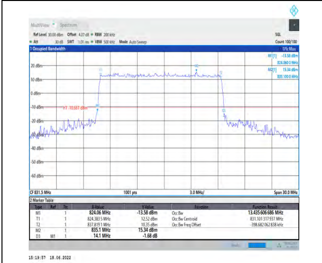
1-N5--15-15-L-1-DFT-QPSK-Outer_Full-75@0-Ant1- 13.436-14.100-≤15-PASS
