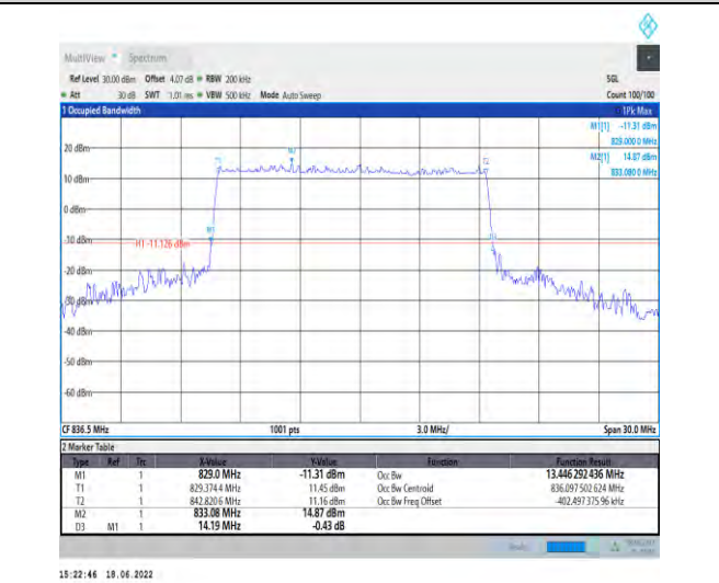
1-N5--15-15-M-1-DFT-QPSK-Outer_Full-75@0-Ant1-13.446-14.190-<=15-PASS
