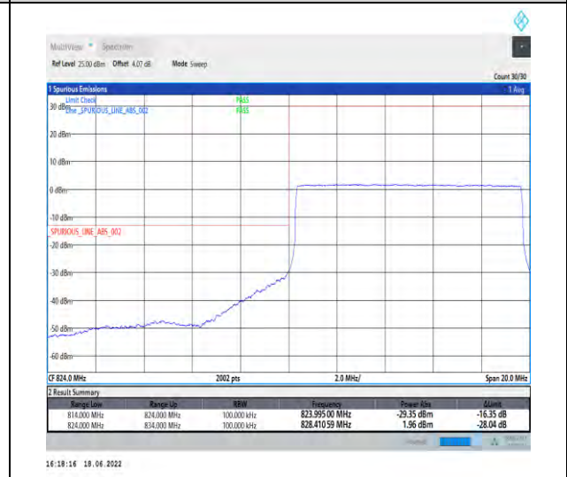
1-N5--15-10-L-6-CP-QPSK-Outer_Full-52@0-Ant1-seegraph-PASS-see graph
