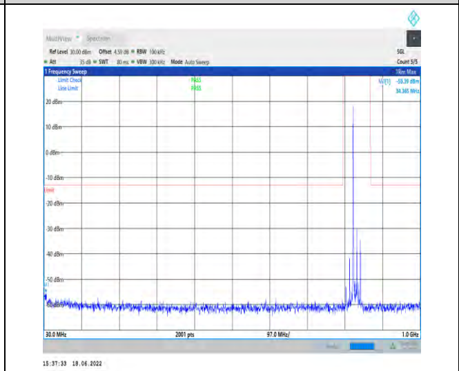
1-N5--15-20-M-1-DFT-PI2BPSK-Inner_1RB_Left-1@ 1-30-1000-Ant1--55.39--13-PASS
