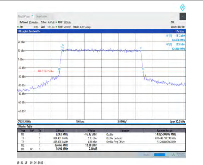
1-N5--15-15-L-6-CP-QPSK-Outer_Full-79@0-Ant1-1 4.095-14.940≤15-PASS
