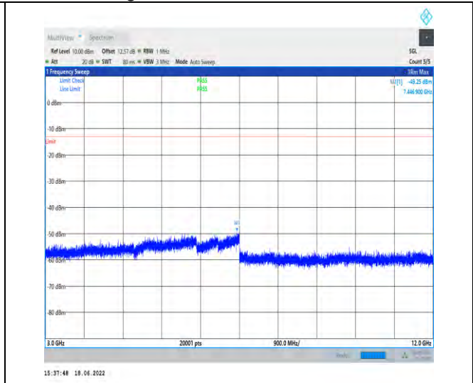
1-N5--15-20-M-1-DFT-PI2BPSK-Inner_1RB_Left-1@ 1-3000-12000-Ant1--49.25--13-PASS
