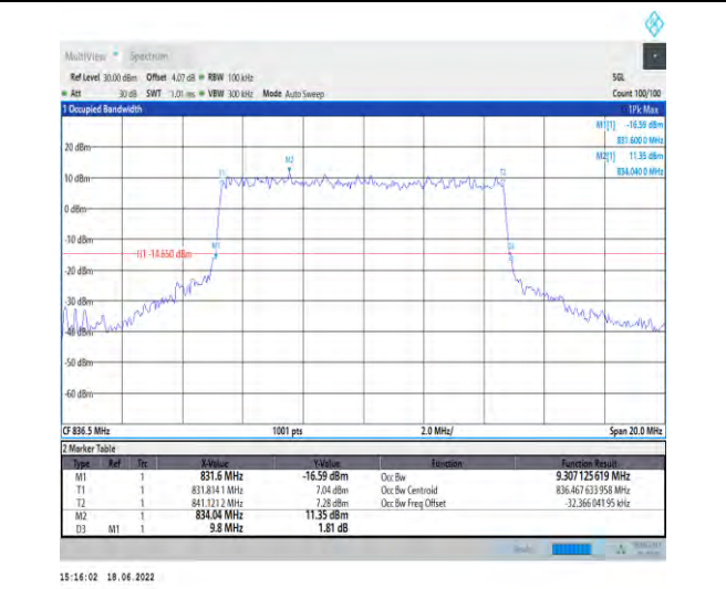
1-N5--15-10-M-8-CP-64QAM-Outer_Full-52@0-Ant1 -9.307-9.800-≤10-PASS
