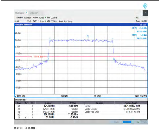
1-N5--15-20-L-6-CP-QPSK-Outer_Full-106@0-Ant1- 18.874-19.800-<=20-PASS
