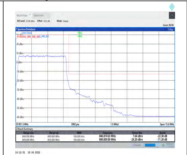
1-N5--15-5-H-3-DFT-PI2BPSK-Outer_Full-25@0-A nt1-seegraph-PASS-see graph
