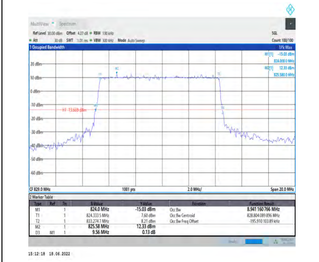
1-N5--15-10-L-4-DFT-64QAM-Outer_Full-50@0-Ant 1-8.941-9.560-≤10-PASS
