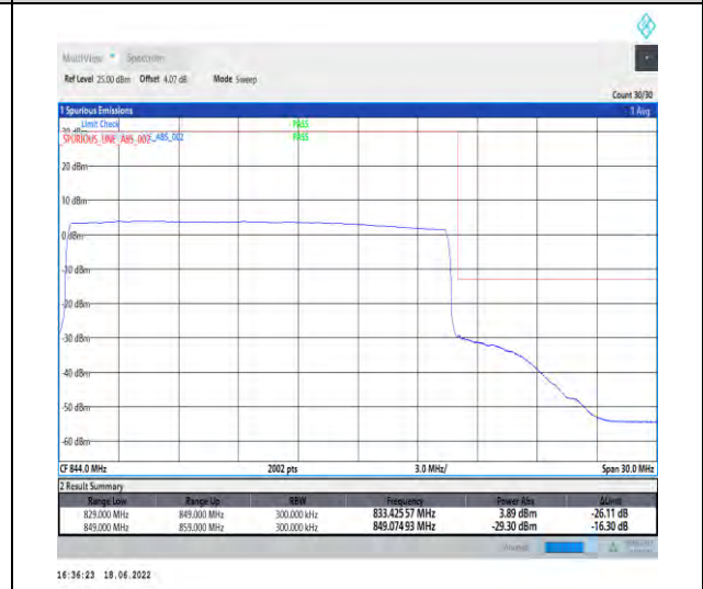
1-N5--15-20-H-6-CP-QPSK-Outer_Full-106@0-Ant1-seegraph-PASS-see graph
