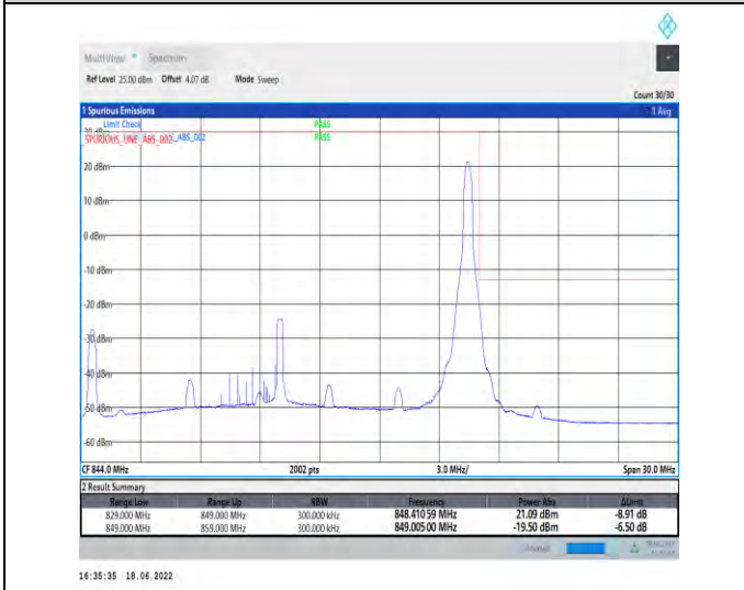
1-N5--15-20-H-5-CP-QPSK-Edge_1RB_Right-1@105-Ant1-seegraph-PASS-see graph
