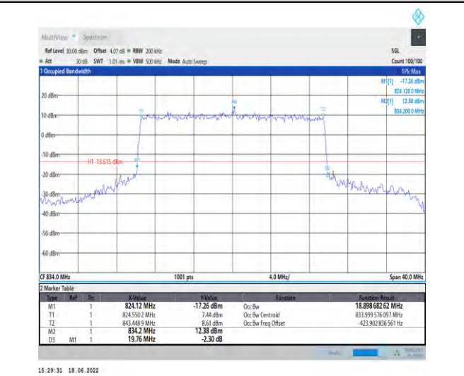
1-N5--15-20-L-7-CP-16QAM-Outer_Full-106@0-Ant1 -18.899-19.760-<=20-PASS
