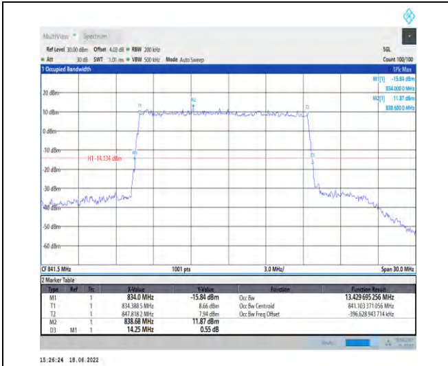
1-N5--15-15-H-5-DFT-256QAM-Outer_Full-75@0-An t1-13.43-14.250-≤15-PASS
