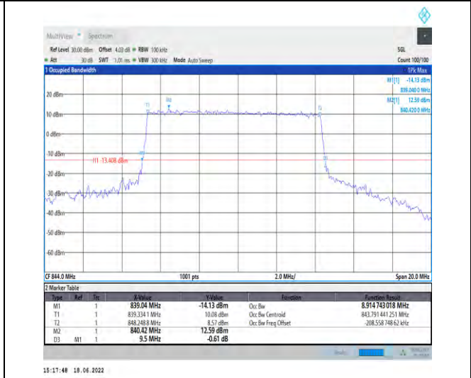
1-N5--15-10-H-3-DFT-16QAM-Outer_Full-50@0-Ant 1-8.915-9.500-≤10-PASS
