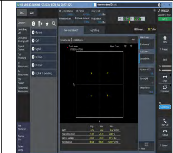
1-N2--15-20-M-2-DFT-QPSK-Outer_Full-100@0-Ant 1-see graph-PASS
