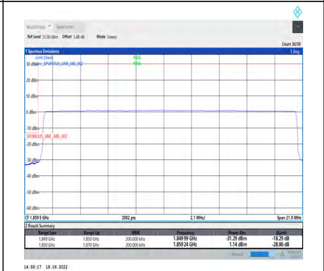
1-N2--15-20-L-6-CP-QPSK-Outer_Full-106@0-Ant1-seegraph-PASS-see graph
