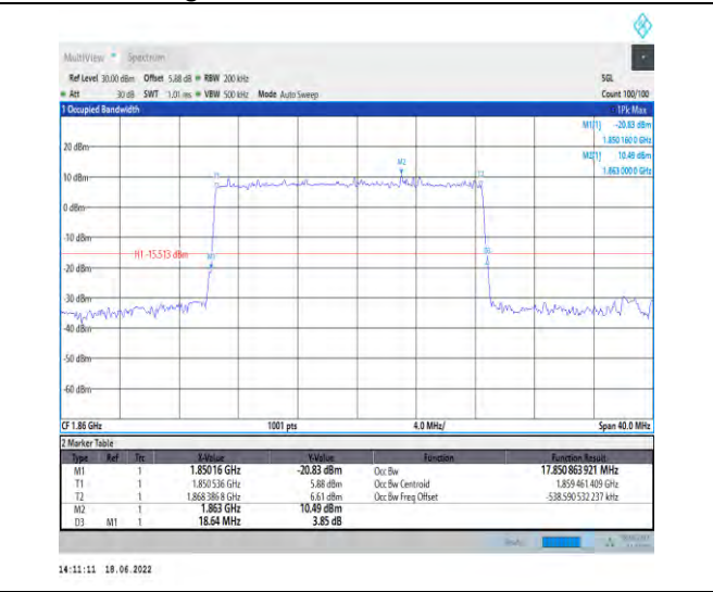
1-N2--15-20-L-5-DFT-256QAM-Outer_Full-100@0-A nt1-17.851-18.640-<20-PASS
