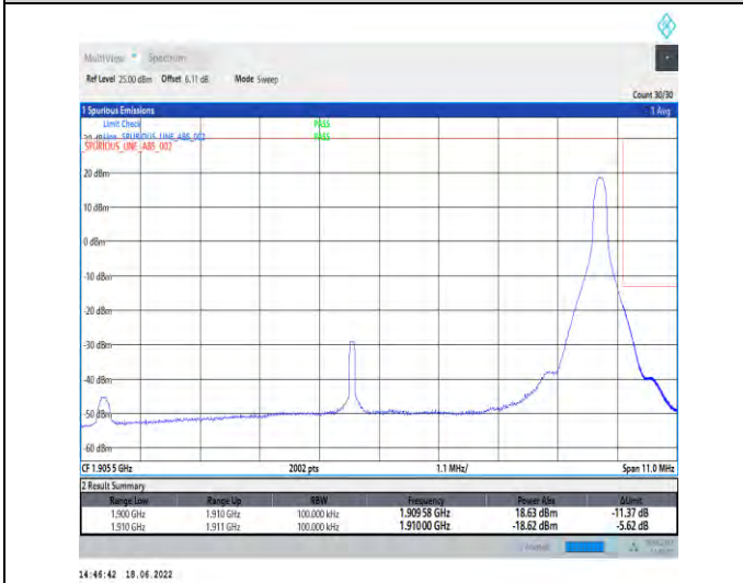
1-N2--15-10-H-5-CP-QPSK-Edge_1RB_Right-1@51-Ant1-seegraph-PASS-see graph
