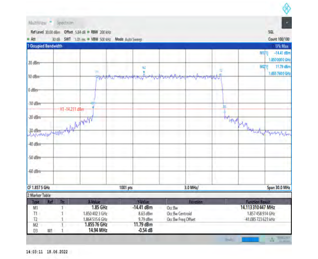
1-N2--15-15-L-6-CP-QPSK-Outer_Full-79@0-Ant1-1 4.113-14.940-≤15-PASS
