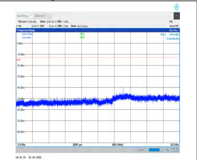
1-N2--15-20-H-1-DFT-PI2BPSK-Inner_1RB_Left-1@ 1-12000-20000-Ant1--43.54--13-PASS
