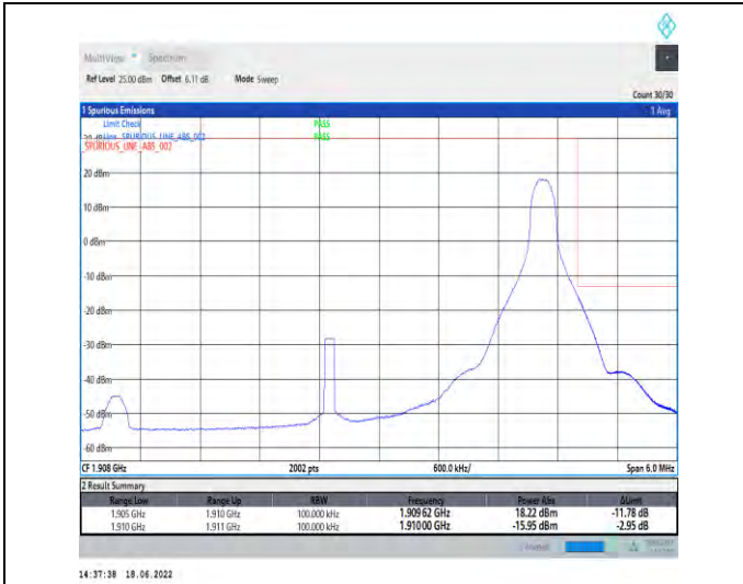
1-N2--15-5-H-2-DFT-PI2BPSK-Edge_1RB_Right-1@2 4-Ant1-seegraph-PASS-see graph
