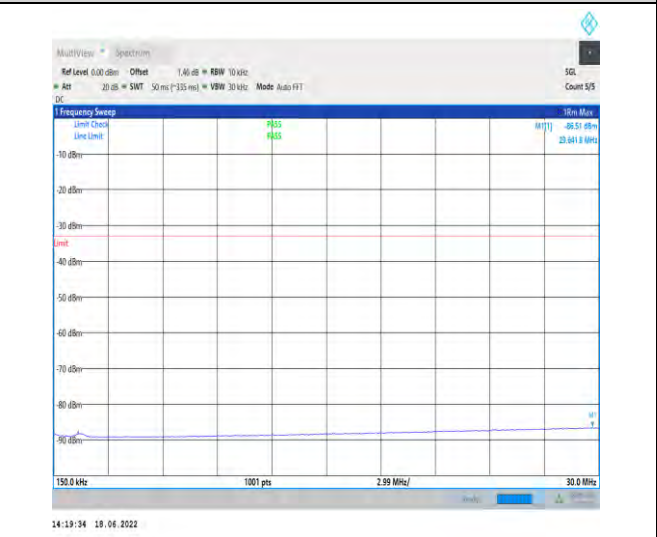
1-N2--15-20-M-1-DFT-PI2BPSK-Inner_1RB_Left-1@ 1-0.15-30-Ant1--86.51--33-PASS
