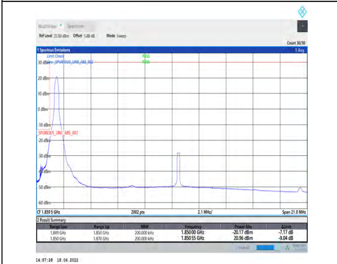
1-N2--15-20-L-4-CP-QPSK-Edge_1RB_Left-1@0-Ant1-seegraph-PASS-see graph
