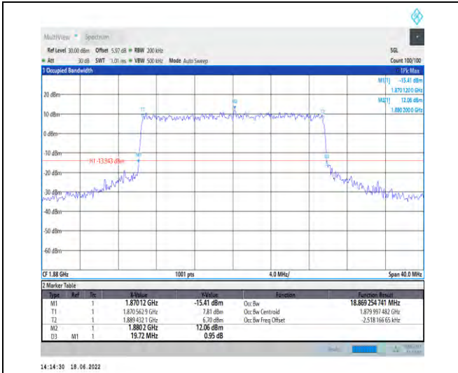
1-N2--15-20-M-7-CP-16QAM-Outer_Full-106@0-Ant 1-18.869-19.720-≤20-PASS
