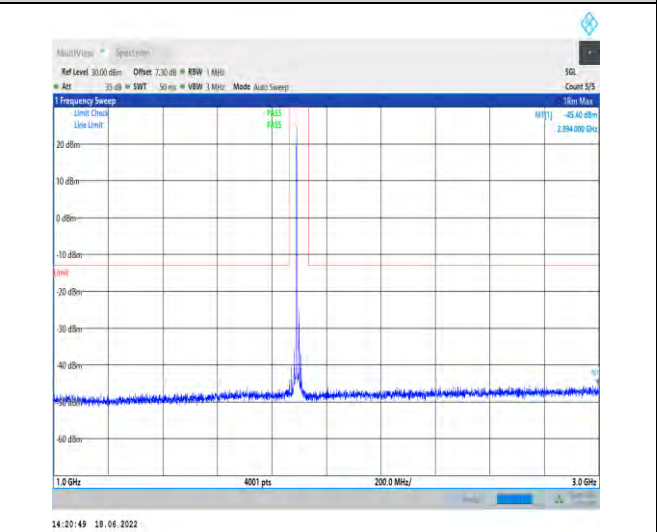
1-N2--15-20-H-1-DFT-PI2BPSK-Inner_1RB_Left-1@ 1-1000-3000-Ant1--45.40--13-PASS
