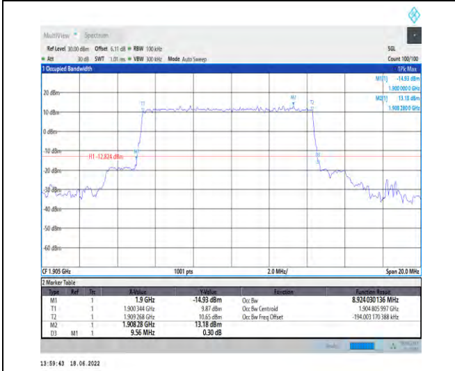
1-N2--15-10-H-2-DFT-PI2BPSK-Outer_Full-50@0-A nt1-8.924-9.560-≤10-PASS
