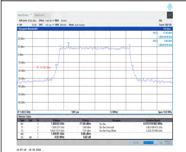
1-N2--15-5-L-7-CP-16QAM-Outer_Full-25@0-Ant1-4 .475-4.920-≤5-PASS
