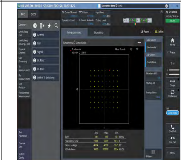
1-N2--15-20-M-4-DFT-64QAM-Outer_Full-100@0-A nt1-see graph-PASS
