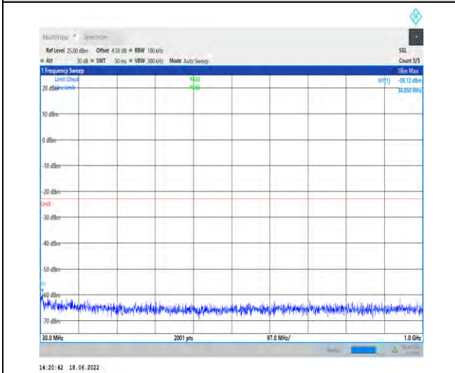
1-N2--15-20-H-1-DFT-PI2BPSK-Inner_1RB_Left-1@ 1-30-1000-Ant1--59.12--23-PASS
