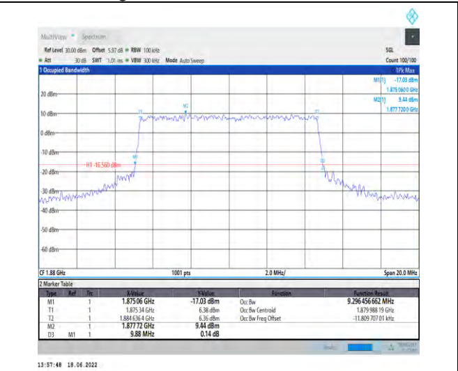
1-N2--15-10-M-6-CP-QPSK-Outer_Full-52@0-Ant1-9 .296-9.880-≤10-PASS
