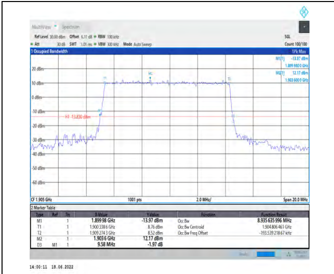
1-N2--15-10-H-4-DFT-64QAM-Outer_Full-50@0-Ant 1-8.936-9.580-≤10-PASS
