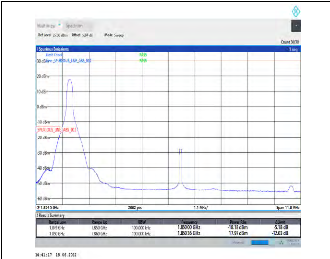
1-N2--15-10-L-1-DFT-PI2BPSK-Edge_1RB_Left-1@0-Ant1-seegraph-PASS-see graph
