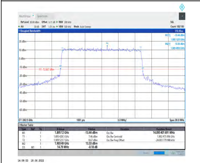
1-N2--15-15-H-7-CP-16QAM-Outer_Full-79@0-Ant1 -14.095-14.790-≤15-PASS
