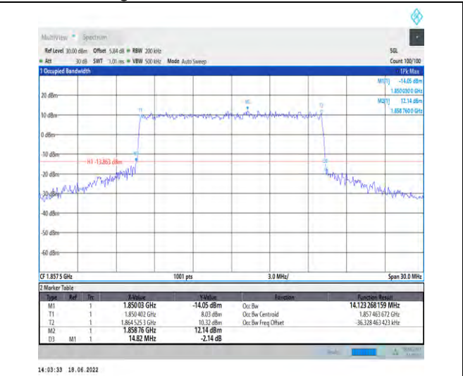
1-N2--15-15-L-8-CP-64QAM-Outer_Full-79@0-Ant1-14.123-14.820-≤15-PASS
