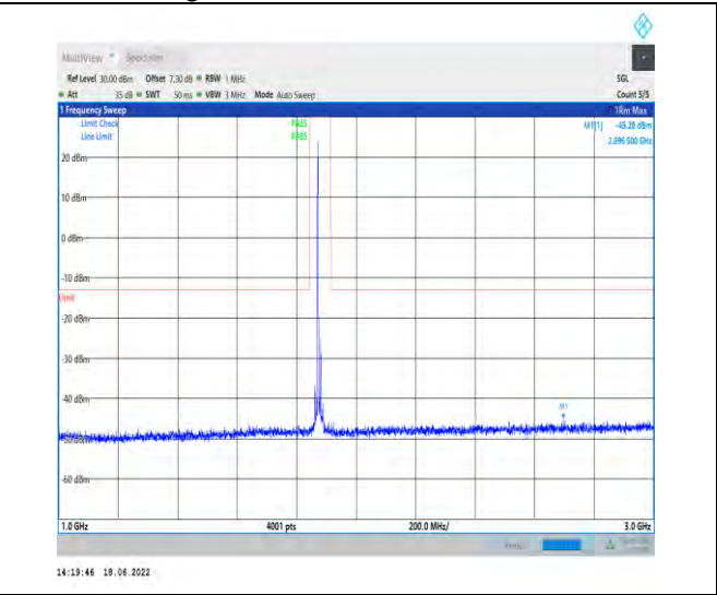
1-N2--15-20-M-1-DFT-PI2BPSK-Inner_1RB_Left-1@ 1-1000-3000-Ant1--45.28--13-PASS
