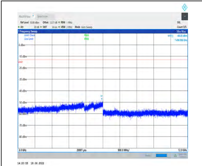
1-N2--15-20-H-1-DFT-PI2BPSK-Inner_1RB_Left-1@ 1-3000-12000-Ant1--48.03--13-PASS
