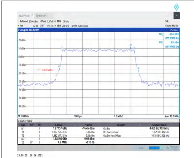
1-N2--15-5-M-8-CP-64QAM-Outer_Full-25@0-Ant1-4.467-4.900-≤5-PASS
