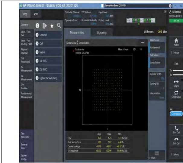
1-N2--15-20-M-5-DFT-256QAM-Outer_Full-100@0-A nt1-see graph-PASS
