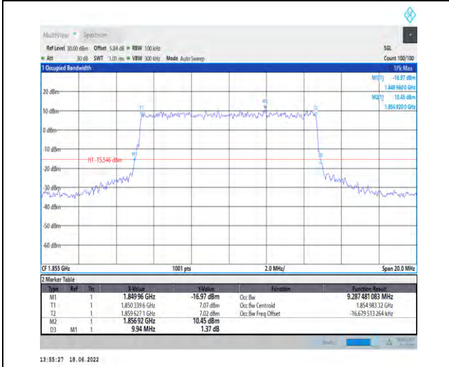
1-N2--15-10-L-8-CP-64QAM-Outer_Full-52@0-Ant1-9 .287-9.940-≤10-PASS
