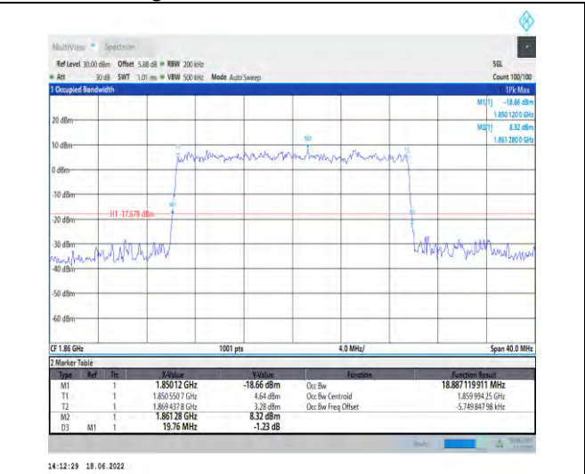
1-N2--15-20-L-9-CP-256QAM-Outer_Full-106@0-Ant 1-18.887-19.760-≤20-PASS
