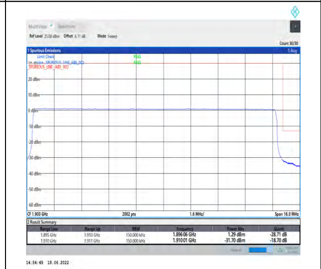
1-N2--15-15-H-6-CP-QPSK-Outer_Full-79@0-Ant1-seegraph-PASS-see graph
