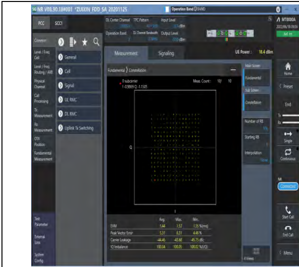
1-N2--15-20-M-9-CP-256QAM-Outer_Full-106@0-Ant 1-see graph-PASS
