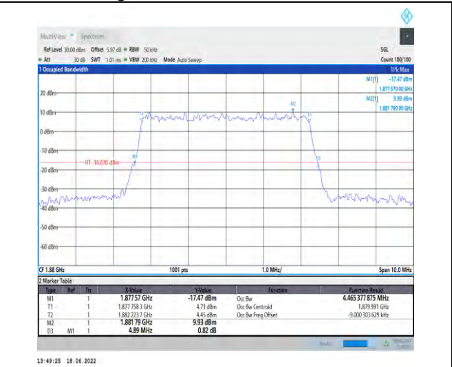
1-N2--15-5-M-5-DFT-256QAM-Outer_Full-25@0-Ant 1-4.465-4.890-≤5-PASS
