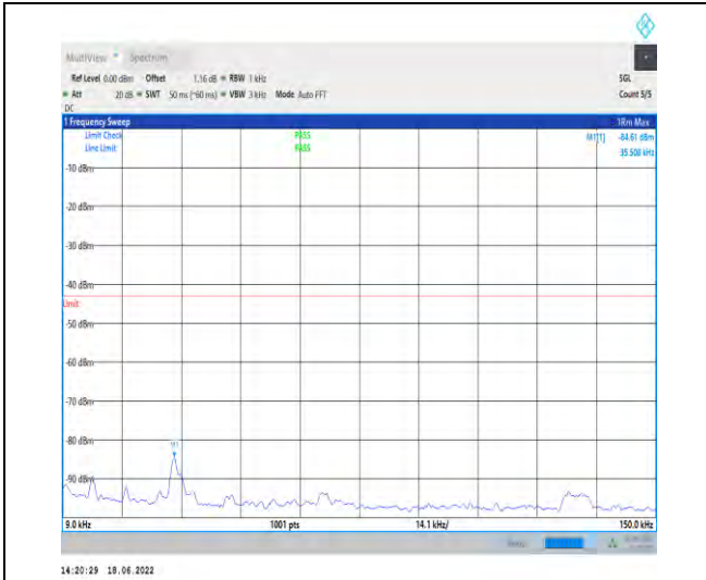
1-N2--15-20-H-1-DFT-PI2BPSK-Inner_1RB_Left-1@ 1-0.009-0.15-Ant1--84.61--43-PASS
