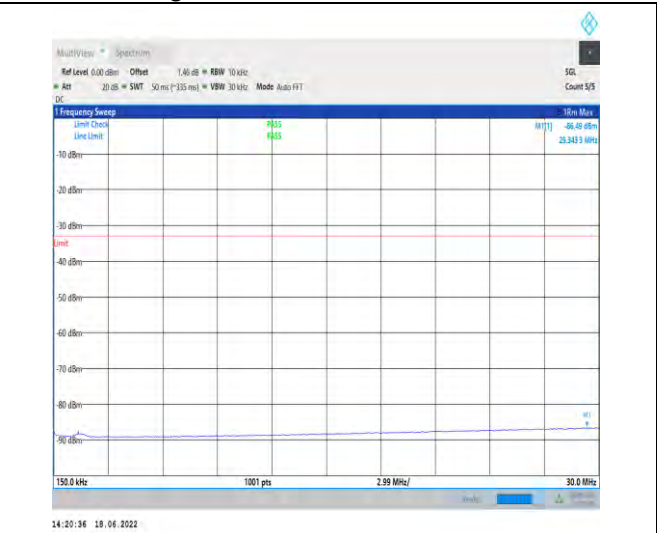
1-N2--15-20-H-1-DFT-PI2BPSK-Inner_1RB_Left-1@ 1-0.15-30-Ant1--86.49--33-PASS
