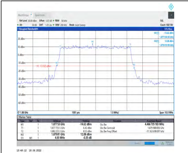
1-N2--15-5-M-4-DFT-64QAM-Outer_Full-25@0-Ant1 -4.467-4.930-≤5-PASS
