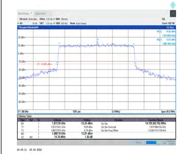
1-N2--15-15-M-8-CP-64QAM-Outer_Full-79@0-Ant1-14.105-14.760-≤15-PASS
