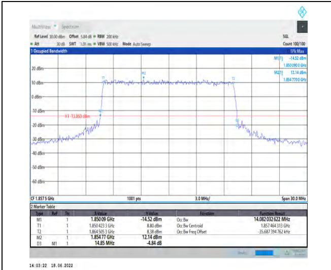
1-N2--15-15-L-7-CP-16QAM-Outer_Full-79@0-Ant1-14.082-14.850-≤15-PASS
