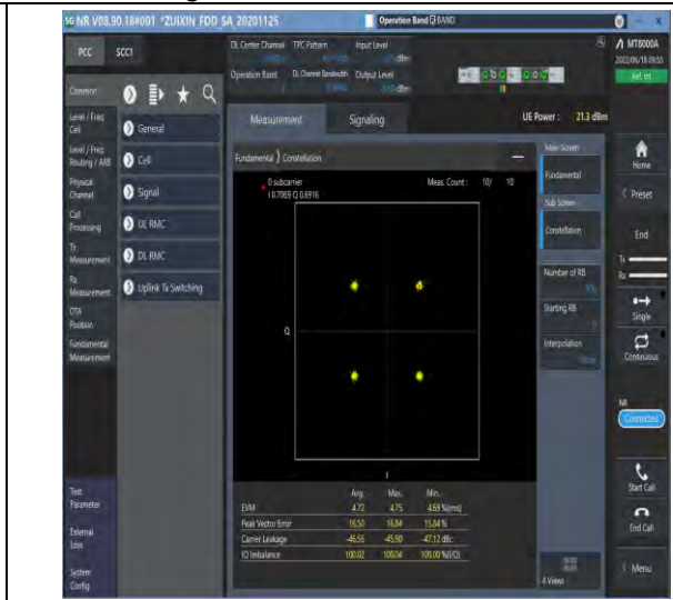
1-N2--15-20-M-6-CP-QPSK-Outer_Full-106@0-Ant 1-see graph-PASS
