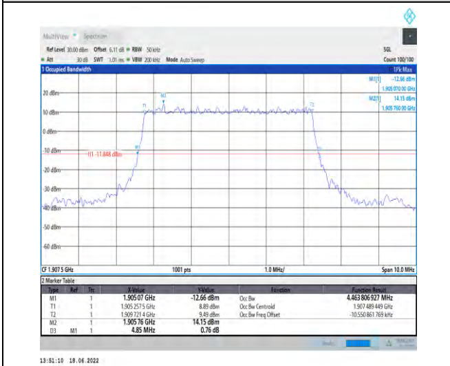
1-N2--15-5-H-1-DFT-QPSK-Outer_Full-25@0-Ant1-4.464-4.850-≤5-PASS
