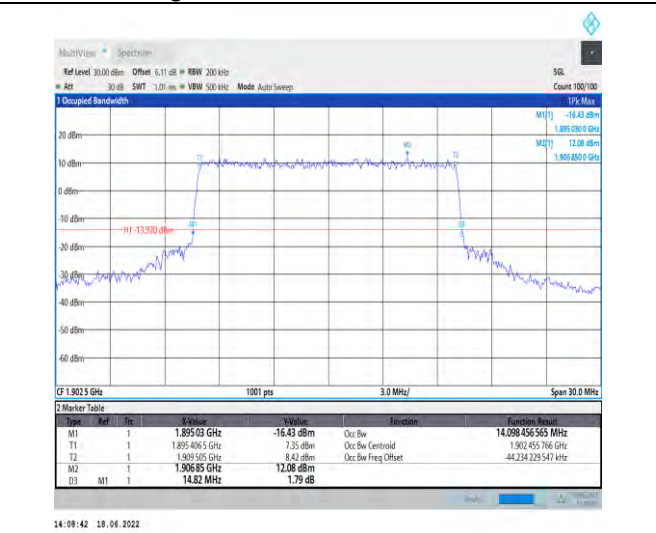
1-N2--15-15-H-6-CP-QPSK-Outer_Full-79@0-Ant1-1 4.098-14.820-≤15-PASS
