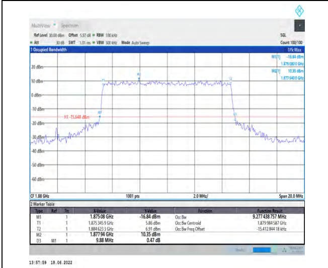
1-N2--15-10-M-7-CP-16QAM-Outer_Full-52@0-Ant1 -9.277-9.880-≤10-PASS
