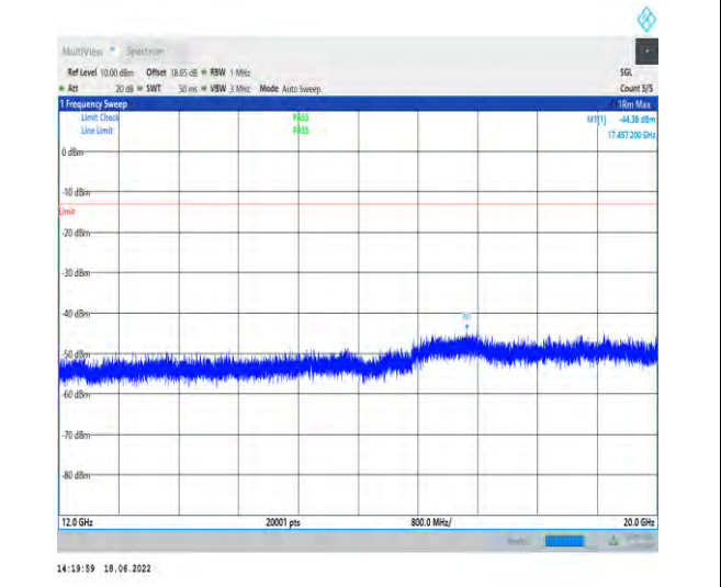
1-N2--15-20-M-1-DFT-PI2BPSK-Inner_1RB_Left-1@ 1-12000-20000-Ant1--44.38--13-PASS
