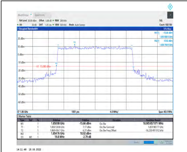
1-N2--15-20-L-8-CP-64QAM-Outer_Full-106@0-Ant 1-18.906-19.800-≤20-PASS
