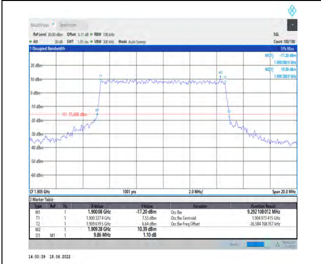
1-N2--15-10-H-6-CP-QPSK-Outer_Full-52@0-Ant1-9 .292-9.860-≤10-PASS
