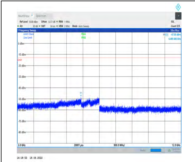
1-N2--15-20-L-1-DFT-PI2BPSK-Inner_1RB_Left-1@ 1-3000-12000-Ant1--47.93--13-PASS
