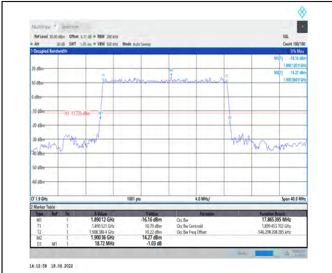
1-N2--15-20-H-2-DFT-PI2BPSK-Outer_Full-100@0-Ant1-17.865-18.720-<math>\leq 20</math>-PASS
