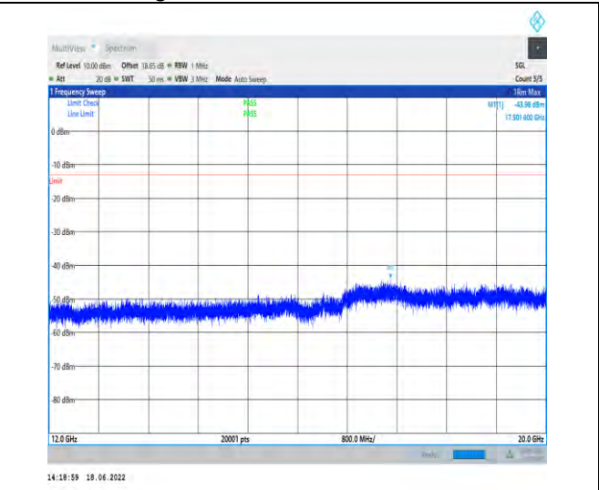
1-N2--15-20-L-1-DFT-PI2BPSK-Inner_1RB_Left-1@ 1-12000-20000-Ant1--43.98--13-PASS
