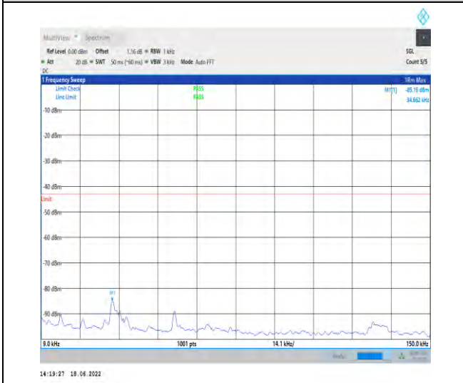
1-N2--15-20-M-1-DFT-PI2BPSK-Inner_1RB_Left-1@ 1-0.009-0.15-Ant1--85.16--43-PASS
