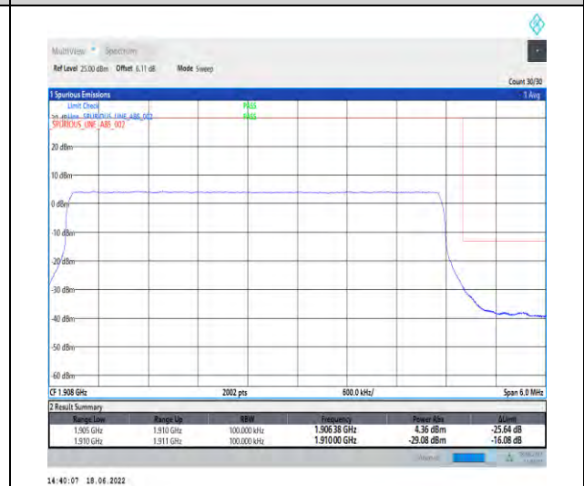
1-N2--15-5-H-6-CP-QPSK-Outer_Full-25@0-Ant1 seegraph-PASS-see graph
