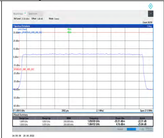
1-N2--15-20-L-3-DFT-PI2BPSK-Outer_Full-100@0-Ant1-seegraph-PASS-see graph
