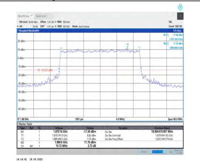
1-N2--15-20-M-8-CP-64QAM-Outer_Full-106@0-Ant 1-18.905-19.720-≤20-PASS
