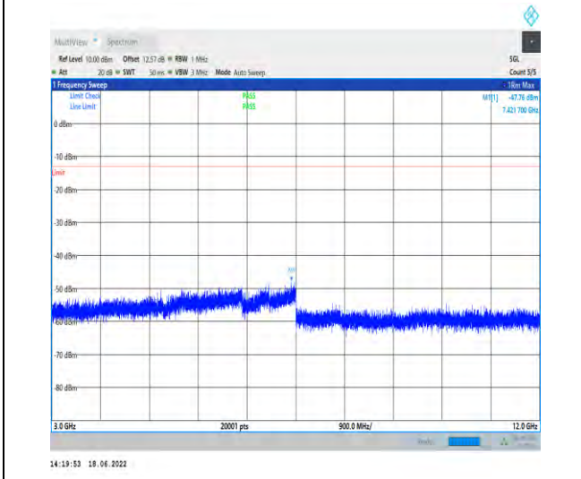
1-N2--15-20-M-1-DFT-PI2BPSK-Inner_1RB_Left-1 @1-3000-12000-Ant1--47.76--13-PASS
