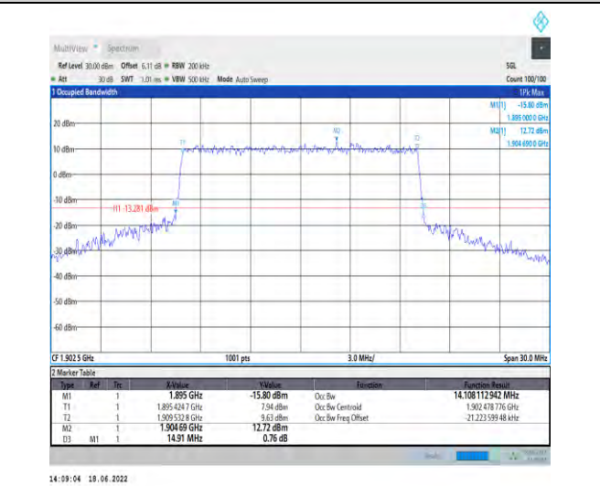
1-N2--15-15-H-8-CP-64QAM-Outer_Full-79@0-Ant1-1 14.108-14.910-≤15-PASS
