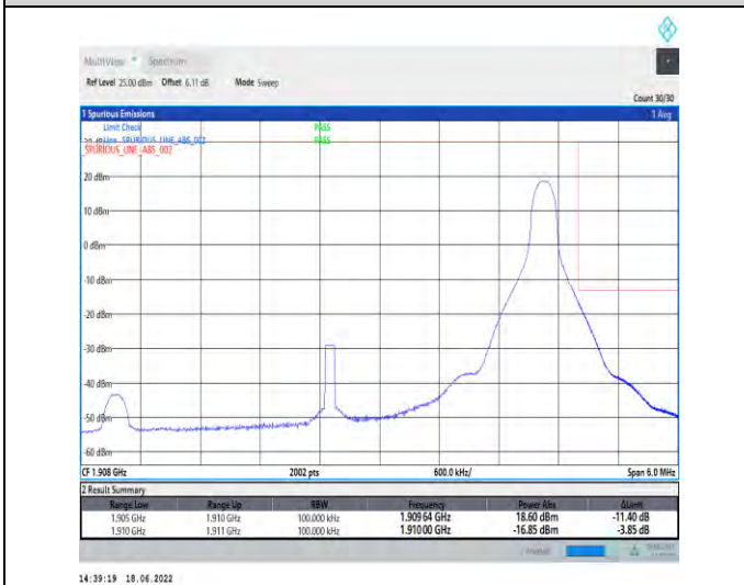
1-N2--15-5-H-5-CP-QPSK-Edge_1RB_Right-1@24-Ant 1-seegraph-PASS-see graph
