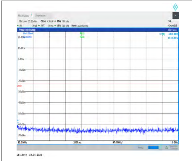
1-N2--15-20-M-1-DFT-PI2BPSK-Inner_1RB_Left-1 @1-30-1000-Ant1--59.85--23-PASS
