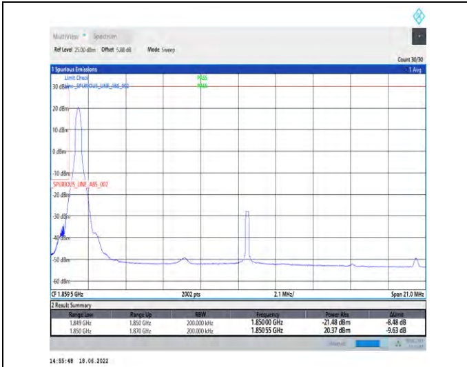
1-N2--15-20-L-1-DFT-PI2BPSK-Edge_1RB_Left-1@0-Ant1-seegraph-PASS-see graph
