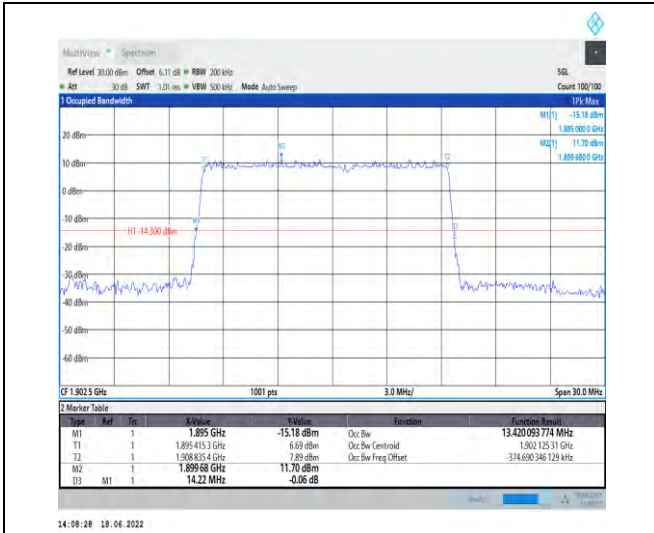
1-N2--15-15-H-5-DFT-256QAM-Outer_Full-75@0-Ant t1-13.42-14.220-≤15-PASS
