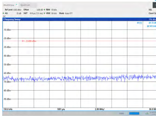
Band26-15MHz-QPSK-26865-1RB#0-Range2:0.15~30MHz
