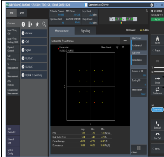
1-N48-PC3-30-40-M-3-DFT-16QAM-Outer_Full-100@0-Ant1-see graph-PASS
