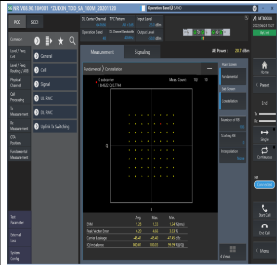
1-N48-PC3-30-40-M-8-CP-64QAM-Outer_Full-106@0-Ant1-see graph-PASS
