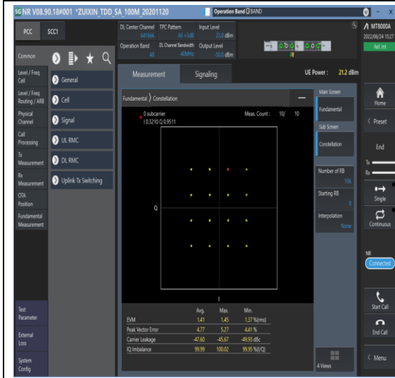
1-N48-PC3-30-40-M-7-CP-16QAM-Outer_Full-106@0-Ant1-see graph-PASS
