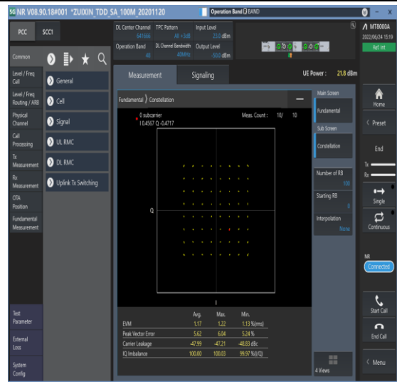
1-N48-PC3-30-40-M-4-DFT-64QAM-Outer_Full-100@0-Ant1-see graph-PASS
