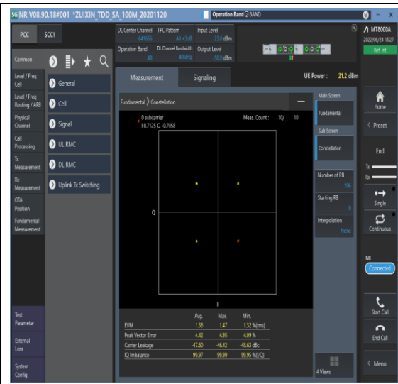
1-N48-PC3-30-40-M-6-CP-QPSK-Outer_Full-106@0-Ant1-see graph-PASS
