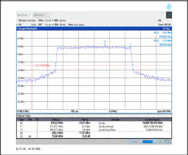
1-N71--15-20-M-6-CP-QPSK-Outer_Full-106@0-Ant 1-18.885-19.840-≤20-PASS
