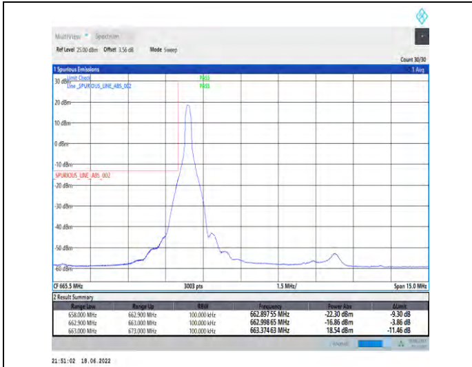
1-N71--15-10-L-1-DFT-PI2BPSK-Edge_1RB_Left-1@0-Ant1-PASS-see graph
