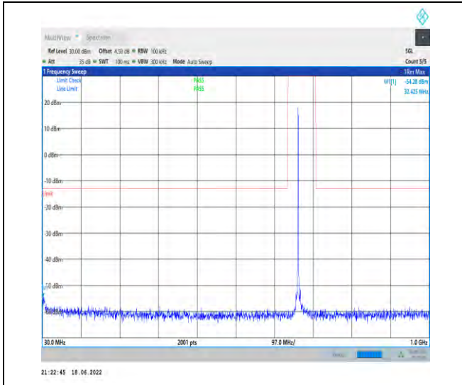
1-N71--15-20-M-1-DFT-PI2BPSK-Inner_1RB_Left-1 @1-30-1000-Ant1--54.28--13-PASS
