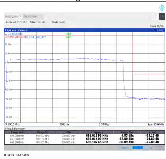
1-N71-PC3-15-20-H-3-DFT-PI2BPSK-Outer_Full-100@0-Ant1-PASS-see graph
