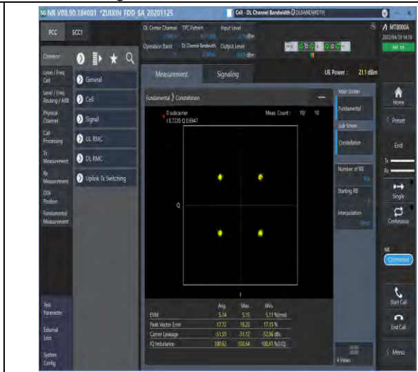
1-N71--15-20-M-6-CP-QPSK-Outer_Full-106@0-Ant1-see graph-PASS
