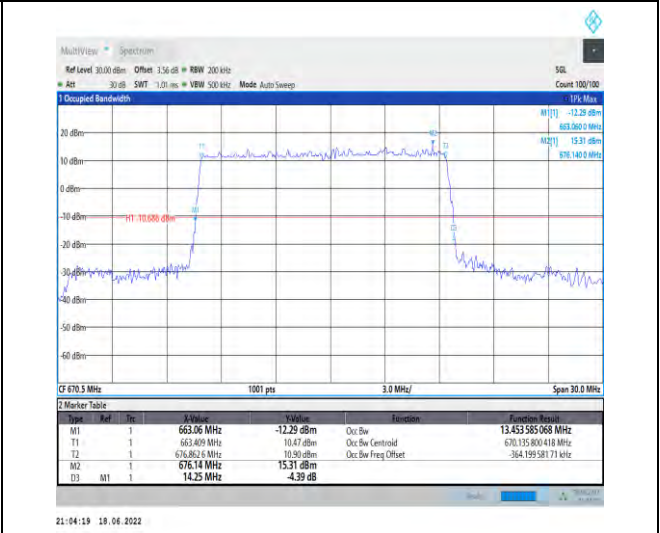
1-N71--15-15-L-2-DFT-PI2BPSK-Outer_Full-75@0-Ant1 nt1-13.454-14.250-≤15-PASS
