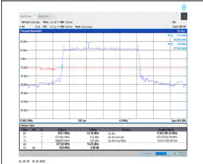
1-N71--15-20-M-1-DFT-QPSK-Outer_Full-100@0-Ant 1-17.815-18.600-<20-PASS
