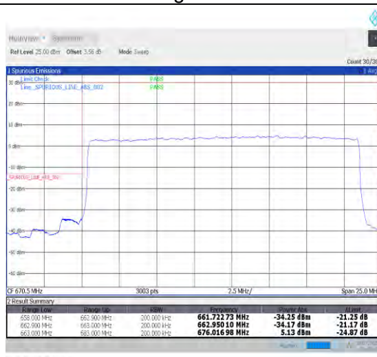
09:06:33 10.07.2022 1-N71-PC3-15-20-L-3-DFT-PI2BPSK-Outer_Full-100@0-Ant1-PASS-see graph
