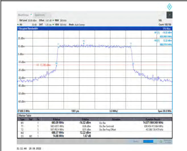
1-N71--15-15-H-7-CP-16QAM-Outer_Full-79@0-Ant 1-14.072-14.880-≤15-PASS
