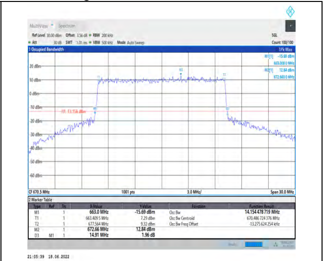
1-N71--15-15-L-8-CP-64QAM-Outer_Full-79@0-Ant 1-14.154-14.910-≤15-PASS
