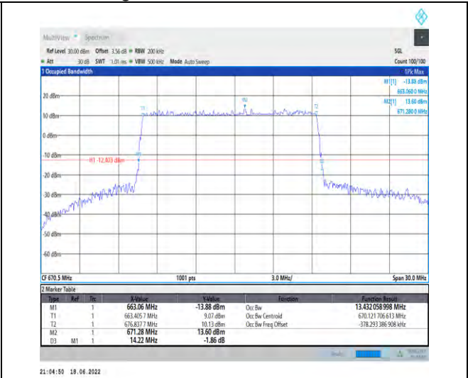
1-N71--15-15-L-4-DFT-64QAM-Outer_Full-75@0-An t1-13.432-14.220≤15-PASS
