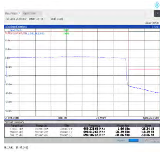
1-N71-PC3-15-20-H-6-CP-QPSK-Outer_Full-106@0-Ant1-PASS-see graph
