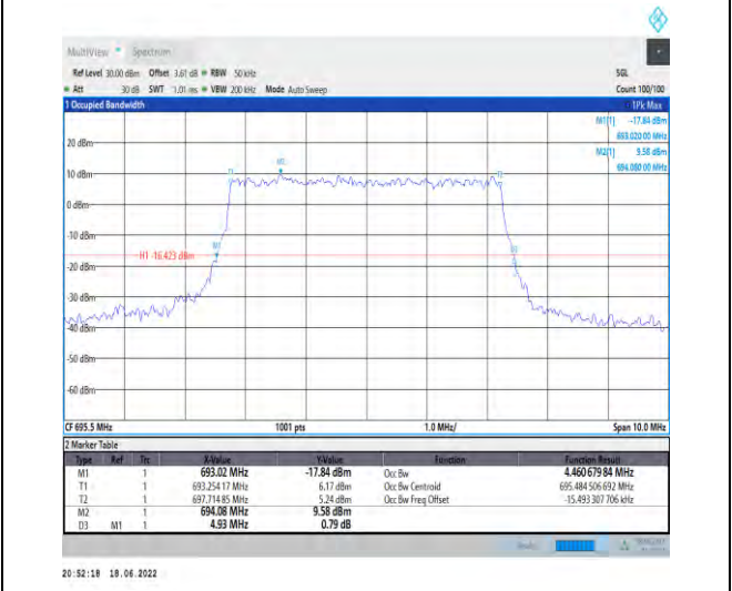
1-N71--15-5-H-6-CP-QPSK-Outer_Full-25@0-Ant1-4 .461-4.930-≤5-PASS
