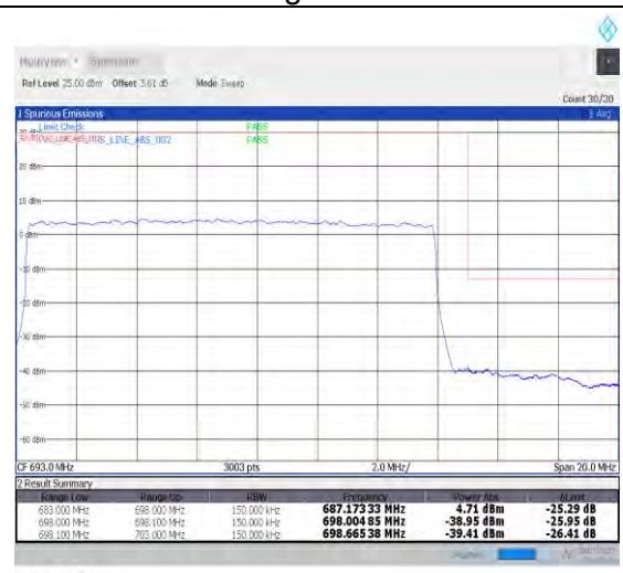
1-N71-PC3-15-15-H-3-DFT-PI2BPSK-Outer_Full-75@0-Ant1-PASS-see graph
