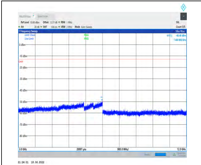
1-N71--15-20-H-1-DFT-PI2BPSK-Inner_1RB_Left-1 @1-3000-12000-Ant1--49.49--13-PASS
