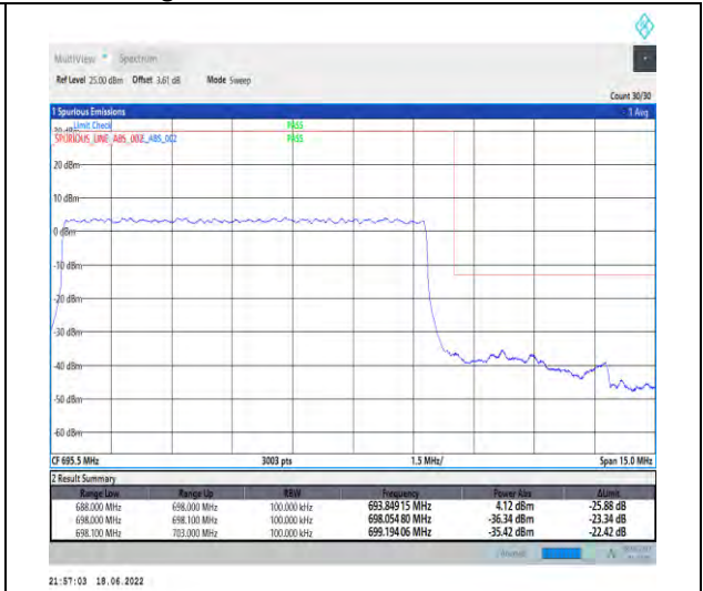
1-N71--15-10-H-3-DFT-PI2BPSK-Outer_Full-50@0-Ant1-PASS-see graph
