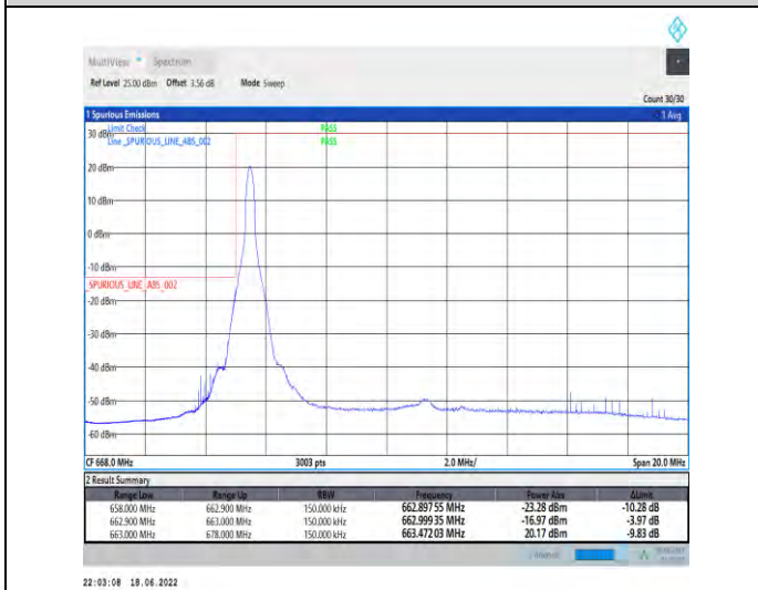
1-N71--15-15-L-4-CP-QPSK-Edge_1RB_Left-1@0-Ant1-PASS-see graph
