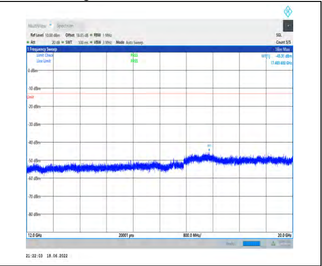
1-N71--15-20-L-1-DFT-PI2BPSK-Inner_1RB_Left-1@ 1-12000-20000-Ant1--45.31--13-PASS
