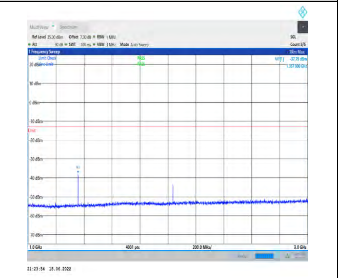
1-N71--15-20-H-1-DFT-PI2BPSK-Inner_1RB_Left-1 @1-1000-3000-Ant1--37.79--13-PASS
