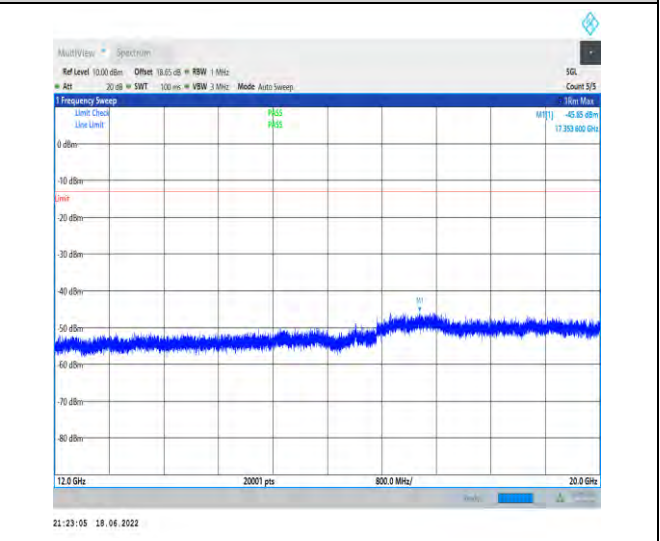
1-N71--15-20-M-1-DFT-PI2BPSK-Inner_1RB_Left-1 @1-12000-20000-Ant1--45.85--13-PASS
