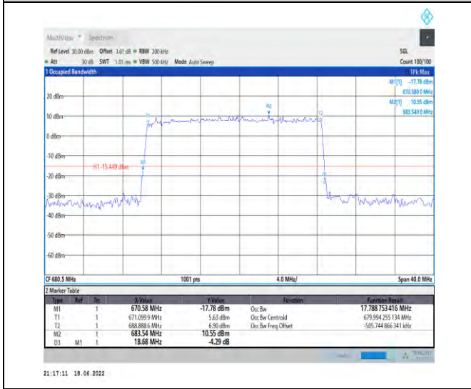
1-N71--15-20-M-5-DFT-256QAM-Outer_Full-100@0-A Ant1-17.789-18.680-≤20-PASS
