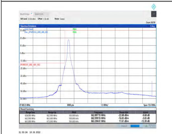
1-N71--15-10-L-4-CP-QPSK-Edge_1RB_Left-1@0-Ant1-PASS-see graph
