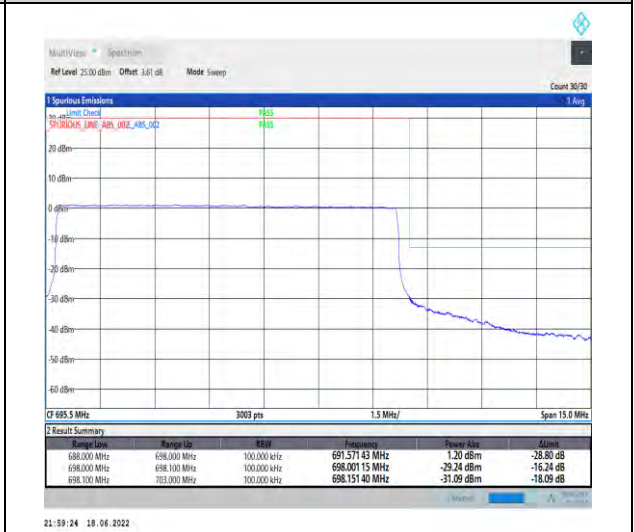
1-N71--15-10-H-6-CP-QPSK-Outer_Full-52@0-Ant1-PASS-see graph
