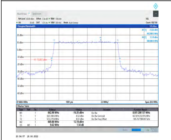
1-N71--15-10-L-4-DFT-64QAM-Outer_Full-50@0-Ant 1-8.931-9.620-≤10-PASS
