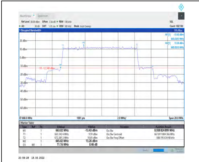
1-N71--15-10-L-2-DFT-PI2BPSK-Outer_Full-50@0-A nt1-8.939-11.160-≤10-PASS
