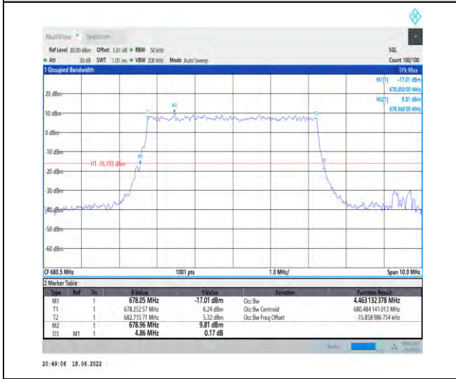
1-N71--15-5-M-6-CP-QPSK-Outer_Full-25@0-Ant1-4 .463-4.860-≤5-PASS
