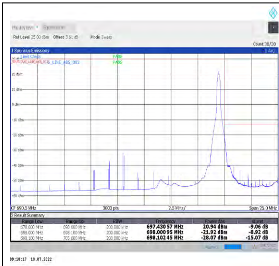
1-N71-PC3-15-20-H-2-DFT-PI2BPSK-Edge_1RB_Right-1@105-Ant1-PASS-see graph
