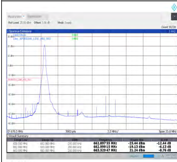
09:07:46 10.07.2022 1-N71-PC3-15-20-L-4-CP-QPSK-Edge_1RB_Left-1@0-Ant1-PASS-see graph
