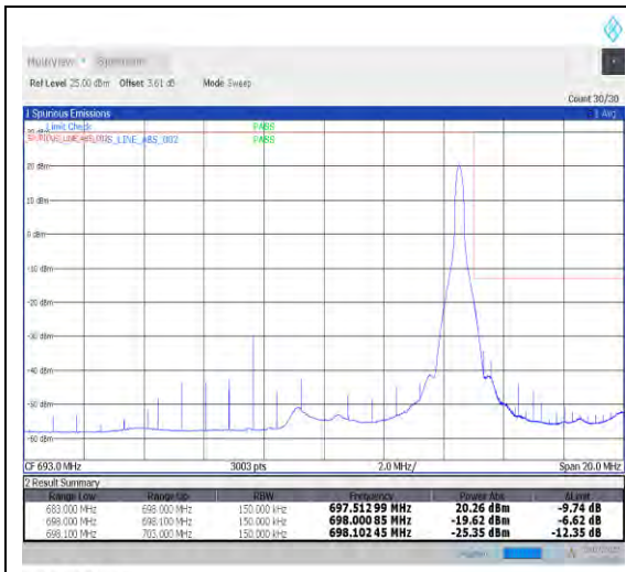
1-N71-PC3-15-15-H-2-DFT-PI2BPSK-Edge_1RB_Right-1@78-Ant1-PASS-see graph
