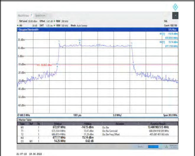
1-N71--15-15-M-1-DFT-QPSK-Outer_Full-75@0-Ant 1-13.481-14.250-≤15-PASS
