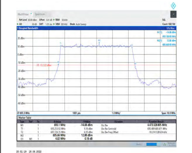
1-N71--15-5-H-2-DFT-PI2BPSK-Outer_Full-25@0-A nt1-4.473-4.820-≤5-PASS
