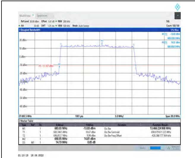
1-N71--15-15-H-1-DFT-QPSK-Outer_Full-75@0-Ant t1-13.466-14.190-≤15-PASS
