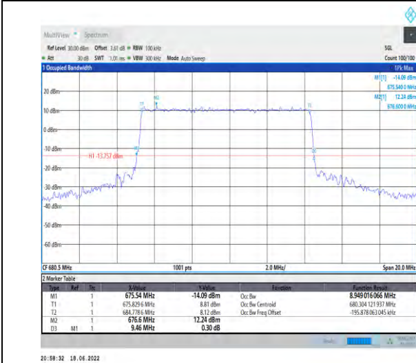
1-N71--15-10-M-3-DFT-16QAM-Outer_Full-50@0-Ant t1-8.949-9.460-≤10-PASS
