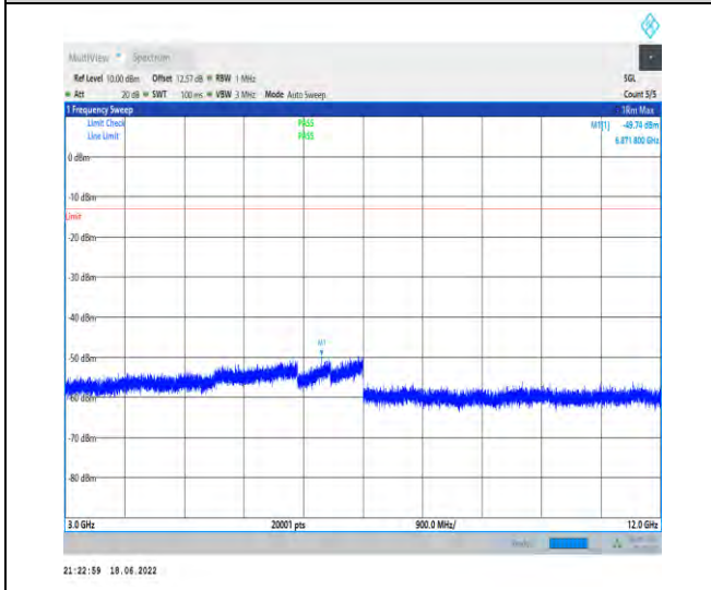
1-N71--15-20-M-1-DFT-PI2BPSK-Inner_1RB_Left-1 @1-3000-12000-Ant1--49.74--13-PASS
