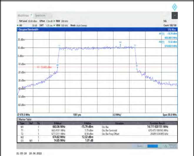
1-N71--15-15-L-6-CP-QPSK-Outer_Full-79@0-Ant1 14.112-14.850≤15-PASS
