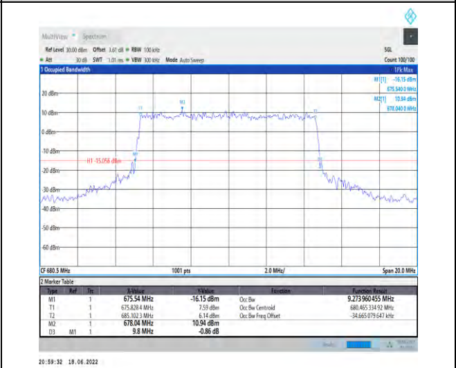
1-N71--15-10-M-8-CP-64QAM-Outer_Full-52@0-Ant 1-9.274-9.800-≤10-PASS
