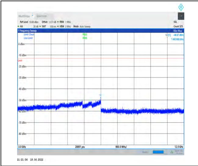
1-N71--15-20-L-1-DFT-PI2BPSK-Inner_1RB_Left-1 @1-3000-12000-Ant1--48.87--13-PASS
