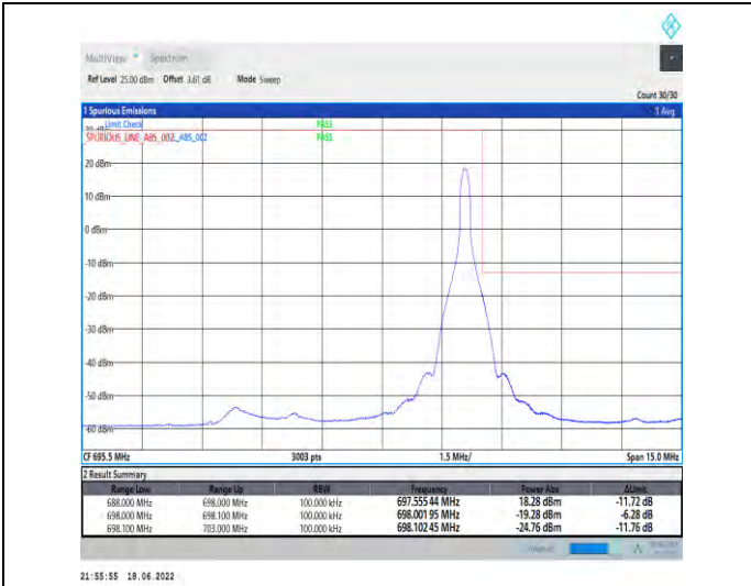
1-N71--15-10-H-2-DFT-PI2BPSK-Edge_1RB_Right-1@51-Ant1-PASS-see graph
