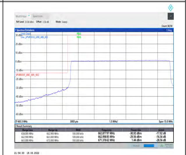
1-N71--15-10-L-6-CP-QPSK-Outer_Full-52@0-Ant1-PASS-see graph
