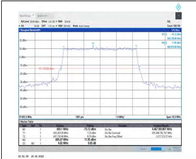
1-N71--15-5-H-3-DFT-16QAM-Outer_Full-25@0-Ant 1-4.467-4.820-≤5-PASS
