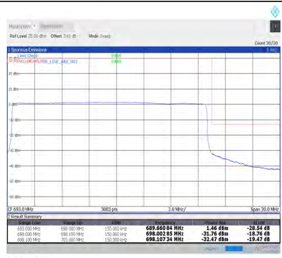
1-N71-PC3-15-15-H-6-CP-QPSK-Outer_Full-79@0-Ant1-PASS-see graph
