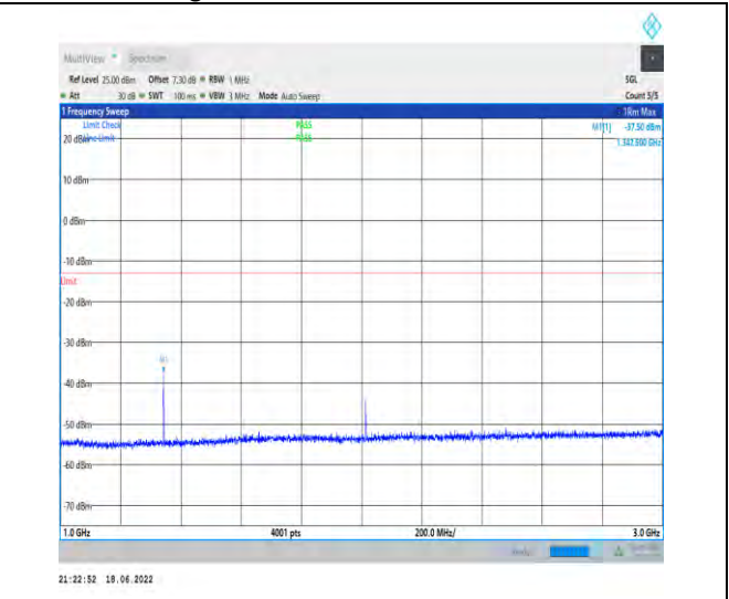
1-N71--15-20-M-1-DFT-PI2BPSK-Inner_1RB_Left-1 @1-1000-3000-Ant1--37.50--13-PASS
