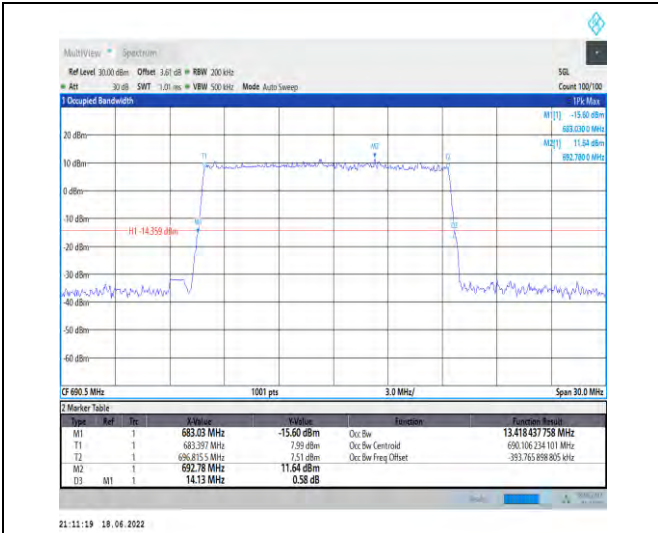
1-N71--15-15-H-5-DFT-256QAM-Outer_Full-75@0-A nt1-13.418-14.130-≤15-PASS
