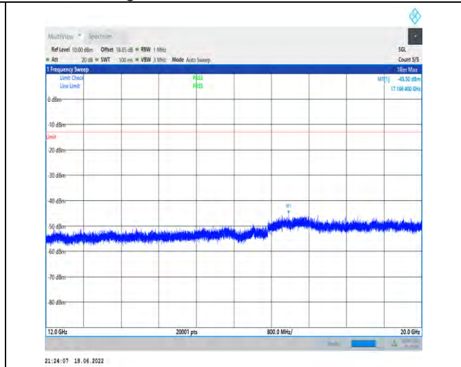
1-N71--15-20-H-1-DFT-PI2BPSK-Inner_1RB_Left-1 @1-12000-20000-Ant1--45.50--13-PASS
