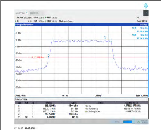
1-N71--15-5-L-7-CP-16QAM-Outer_Full-25@0-Ant1- 4.475-4.890-≤5-PASS
