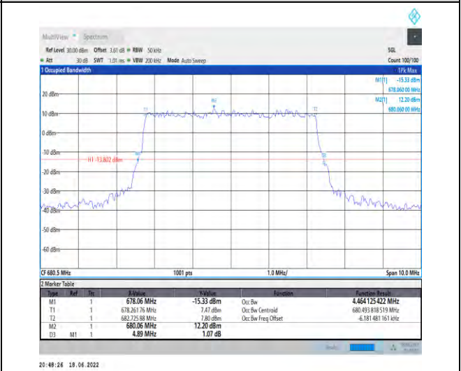
1-N71--15-5-M-3-DFT-16QAM-Outer_Full-25@0-Ant1 1-4.464-4.890-≤5-PASS
