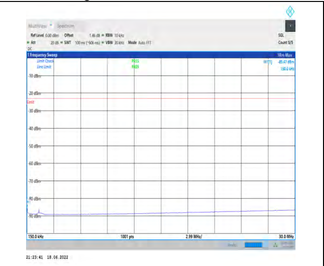
1-N71--15-20-H-1-DFT-PI2BPSK-Inner_1RB_Left-1 @1-0.15-30-Ant1--85.47--23-PASS
