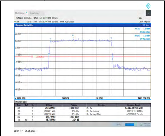
1-N71--15-20-M-4-DFT-64QAM-Outer_Full-100@0-A Ant1-17.846-18.720-≤20-PASS
