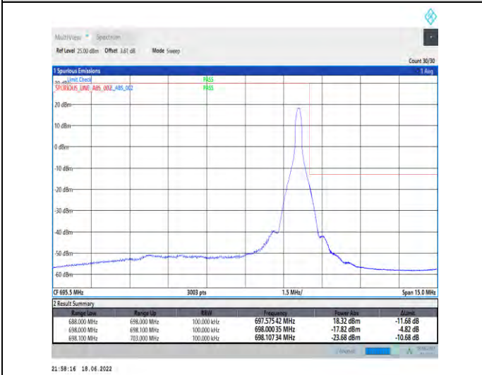
1-N71--15-10-H-5-CP-QPSK-Edge_1RB_Right-1@51-Ant1-PASS-see graph
