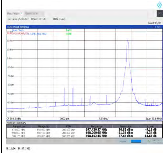
1-N71-PC3-15-20-H-5-CP-QPSK-Edge_1RB_Right-1@105-Ant1-PASS-see graph
