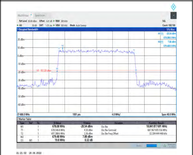
1-N71--15-20-H-9-CP-256QAM-Outer_Full-106@0-Ant t1-18.842-19.800-≤20-PASS
