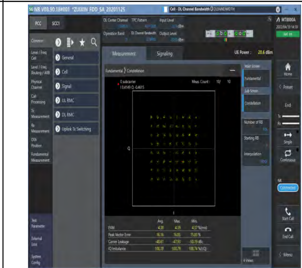
1-N71--15-20-M-8-CP-64QAM-Outer_Full-106@0-Ant1-see graph-PASS
