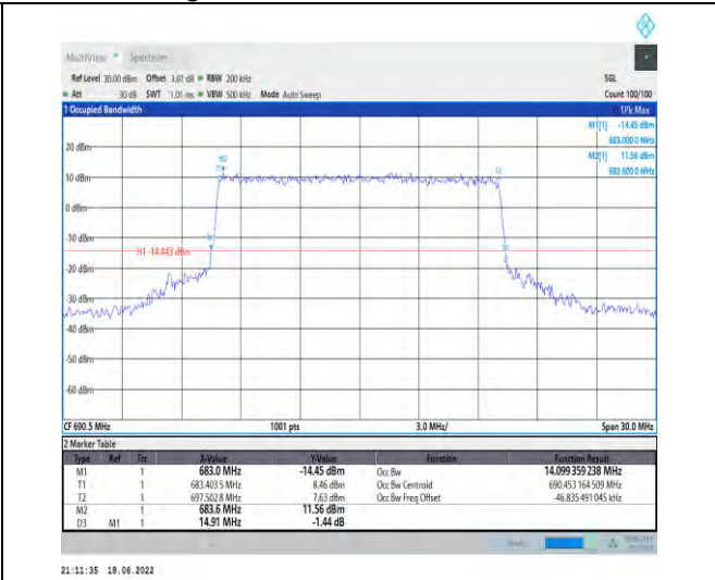
1-N71--15-15-H-6-CP-QPSK-Outer_Full-79@0-Ant1- 14.099-14.910-≤15-PASS
