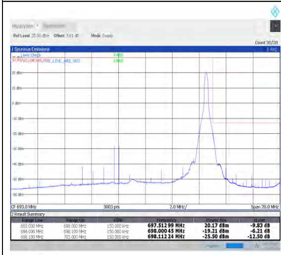
1-N71-PC3-15-15-H-5-CP-QPSK-Edge_1RB_Right-1@78-Ant1-PASS-see graph
