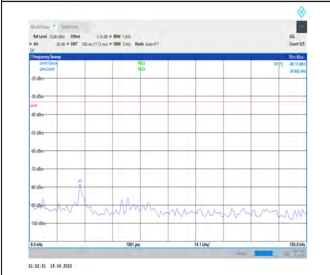
1-N71--15-20-M-1-DFT-PI2BPSK-Inner_1RB_Left-1 @1-0.009-0.15-Ant1--80.13--33-PASS
