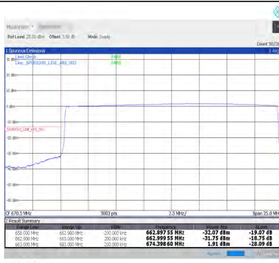
09:08:52 10.07.2022 1-N71-PC3-15-20-L-6-CP-QPSK-Outer_Full-106@0-Ant1-PASS-see graph
