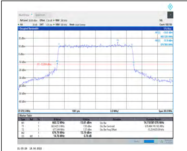
1-N71--15-15-L-7-CP-16QAM-Outer_Full-79@0-Ant1 -14.119-14.760-≤15-PASS
