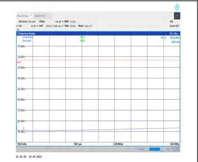
1-N71--15-20-M-1-DFT-PI2BPSK-Inner_1RB_Left-1 @1-0.15-30-Ant1--85.28--23-PASS
