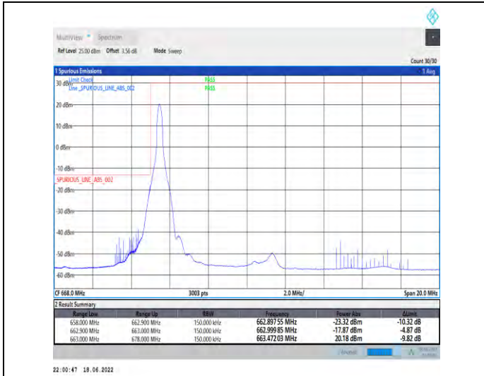
1-N71--15-15-L-1-DFT-PI2BPSK-Edge_1RB_Left-1@0-Ant1-PASS-see graph
