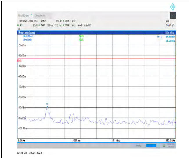
1-N71--15-20-H-1-DFT-PI2BPSK-Inner_1RB_Left-1 @1-0.009-0.15-Ant1--80.15--33-PASS
