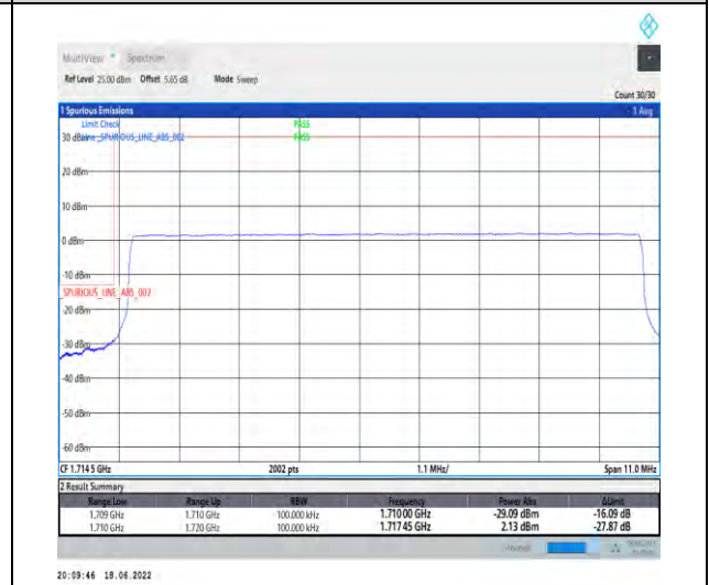
1-N66--15-10-L-6-CP-QPSK-Outer_Full-52@0-Ant1-seegraph-PASS-see graph
