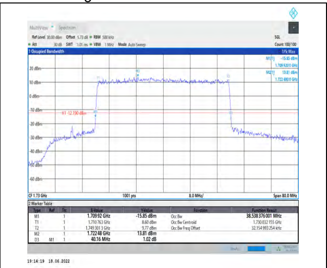
1-N66--15-40-L-7-CP-16QAM-Outer_Full-216@0-Ant1 t1-38.538-40.160-≤40-PASS
