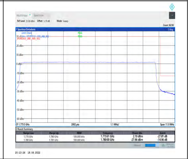
1-N66--15-10-H-6-CP-QPSK-Outer_Full-52@0-Ant1-seegraph-PASS-see graph
