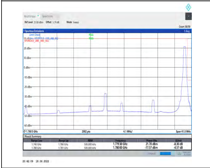
1-N66--15-40-H-5-CP-QPSK-Edge_1RB_Right-1@215 -Ant1-seegraph-PASS-see graph
