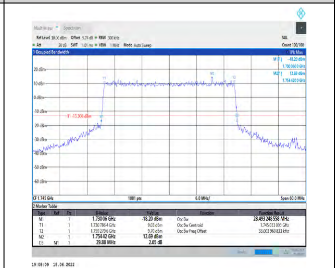
1-N66--15-30-M-7-CP-16QAM-Outer_Full-160@0-A nt1-28.493-29.880-≤30-PASS
