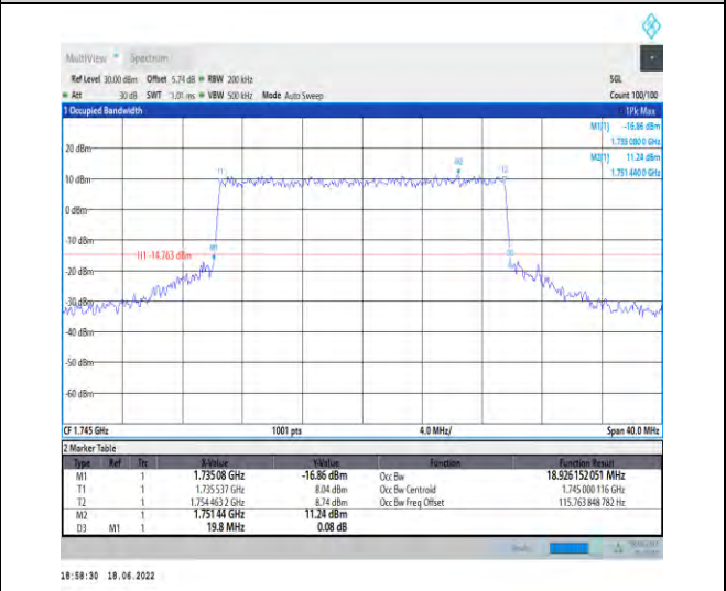
1-N66--15-20-M-6-CP-QPSK-Outer_Full-106@0-Ant 1-18.926-19.800-<20-PASS
