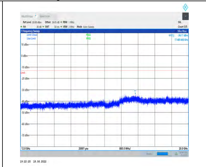
1-N66--15-40-L-1-DFT-PI2BPSK-Inner_1RB_Left-1 @1-12000-20000-Ant1--34.17--13-PASS
