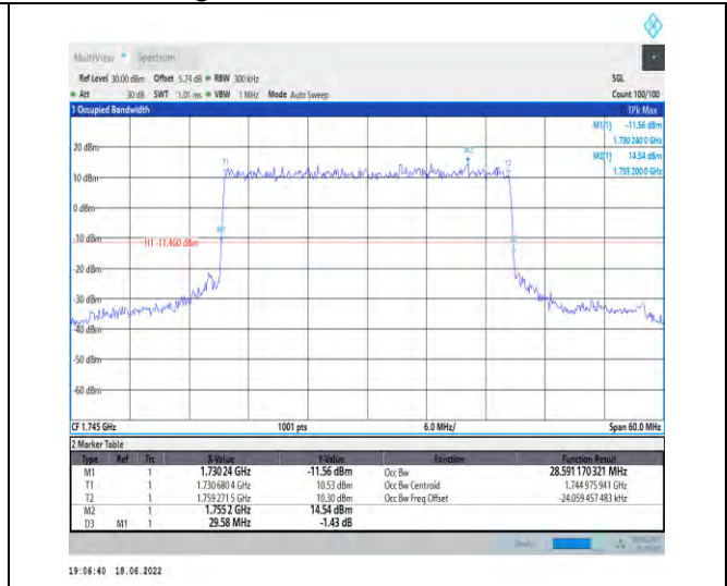
1-N66--15-30-M-1-DFT-QPSK-Outer_Full-160@0-An t1-28.591-29.580- \leq 30 -PASS
