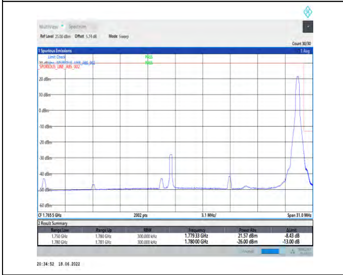
1-N66--15-30-H-5-CP-QPSK-Edge_1RB_Right-1@159 -Ant1-seegraph-PASS-see graph
