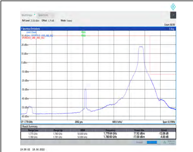
1-N66--15-5-H-2-DFT-PI2BPSK-Edge_1RB_Right-1@24-Ant1-seegraph-PASS-see graph
