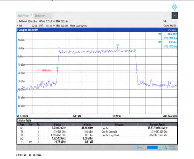
1-N66--15-20-L-9-CP-256QAM-Outer_Full-106@0-A nt1-18.837-19.720-<=20-PASS
