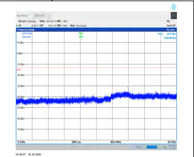
1-N66--15-40-H-1-DFT-PI2BPSK-Inner_1RB_Left-1 @1-12000-20000-Ant1--34.27--13-PASS
