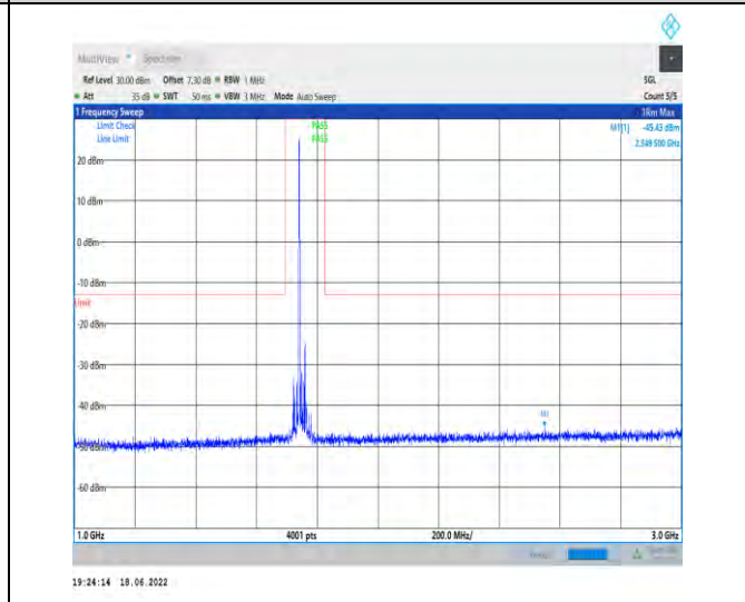
1-N66--15-40-H-1-DFT-PI2BPSK-Inner_1RB_Left-1 @1-1000-3000-Ant1--45.43--13-PASS
