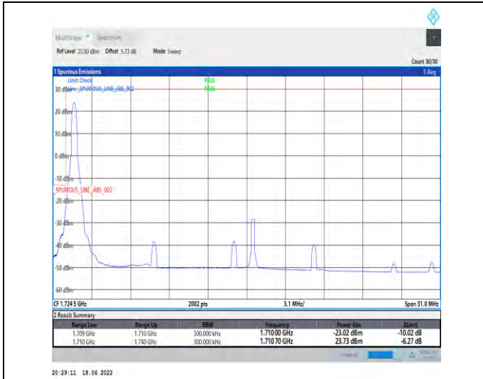
1-N66--15-30-L-1-DFT-PI2BPSK-Edge_1RB_Left-1@0-Ant1-seegraph-PASS-see graph
