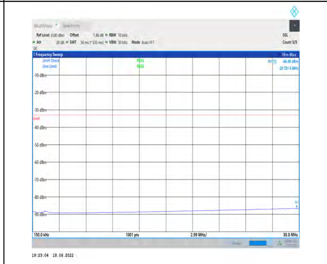
1-N66--15-40-M-1-DFT-PI2BPSK-Inner_1RB_Left-1 @1-0.15-30-Ant1--86.49--33-PASS
