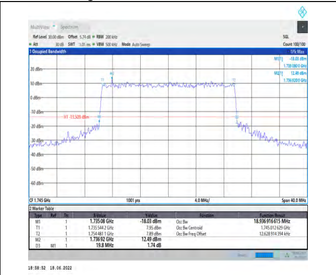
1-N66--15-20-M-8-CP-64QAM-Outer_Full-106@0-A nt1-18.937-19.800-≤20-PASS
