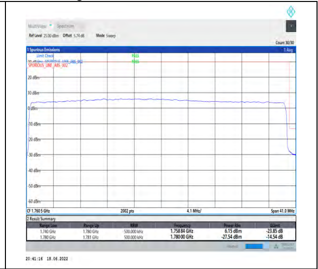
1-N66--15-40-H-3-DFT-PI2BPSK-Outer_Full-216 @0-Ant1-seegraph-PASS-see graph
