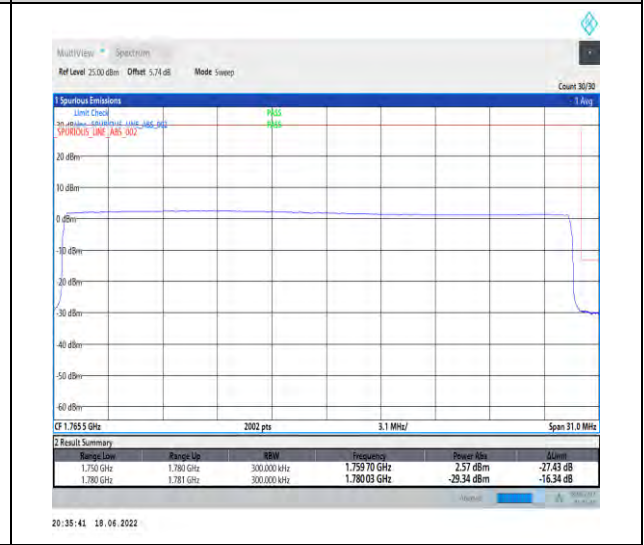
1-N66--15-30-H-6-CP-QPSK-Outer_Full-160@0-A -nt1-seegraph-PASS-see graph
