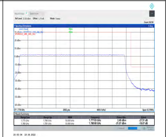
1-N66--15-5-H-6-CP-QPSK-Outer_Full-25@0-Ant1-seegraph-PASS-see graph
