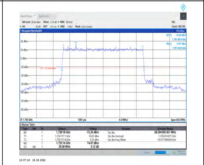
1-N66--15-30-M-3-DFT-16QAM-Outer_Full-160@0-A nt1-28.595-29.580- \leq 30 -PASS
