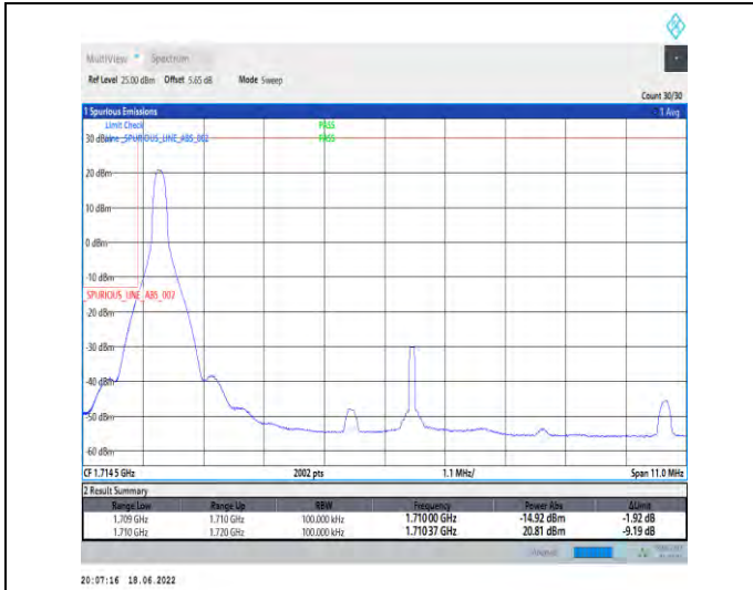
1-N66--15-10-L-1-DFT-PI2BPSK-Edge_1RB_Left-1@0-Ant1-seegraph-PASS-see graph
