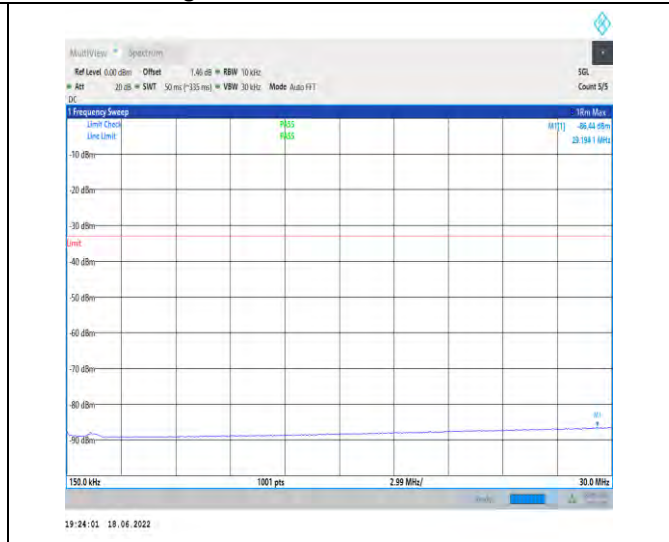
1-N66--15-40-H-1-DFT-PI2BPSK-Inner_1RB_Left-1 @1-0.15-30-Ant1--86.44--33-PASS
