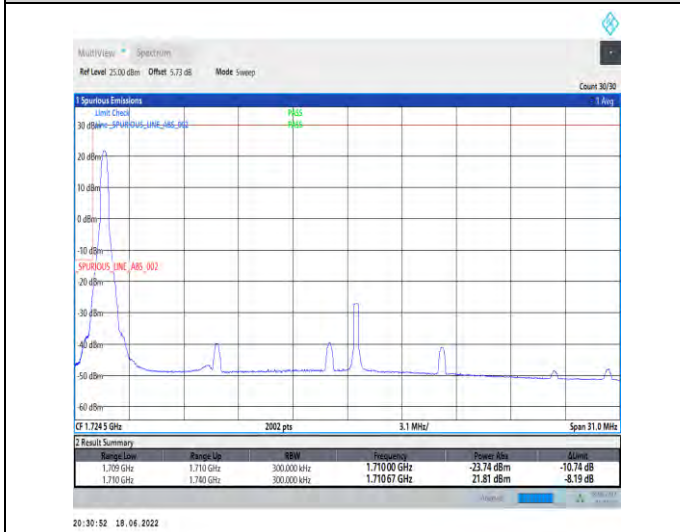
1-N66--15-30-L-4-CP-QPSK-Edge_1RB_Left-1@0-Ant1-seegraph-PASS-see graph
