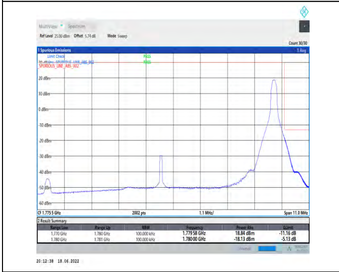
1-N66--15-10-H-5-CP-QPSK-Edge_1RB_Right-1@51-Ant1-seegraph-PASS-see graph
