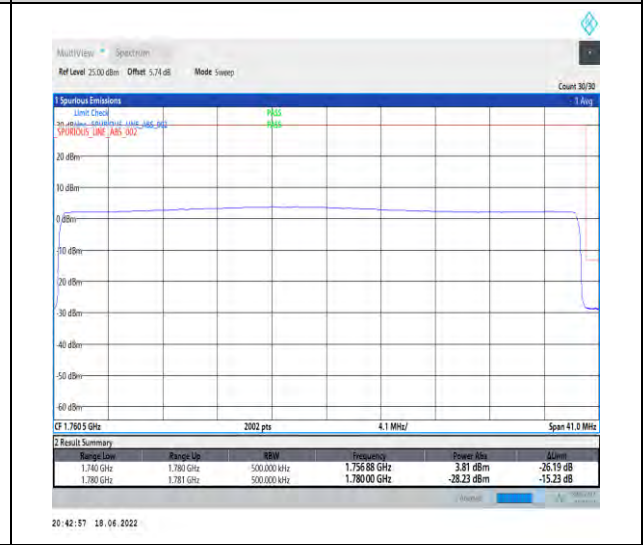
1-N66--15-40-H-6-CP-QPSK-Outer_Full-216@0-A -nt1-seegraph-PASS-see graph
