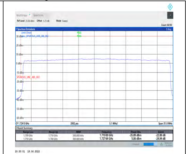
1-N66--15-30-L-3-DFT-PI2BPSK-Outer_Full-160@0-Ant1-seegraph-PASS-see graph
