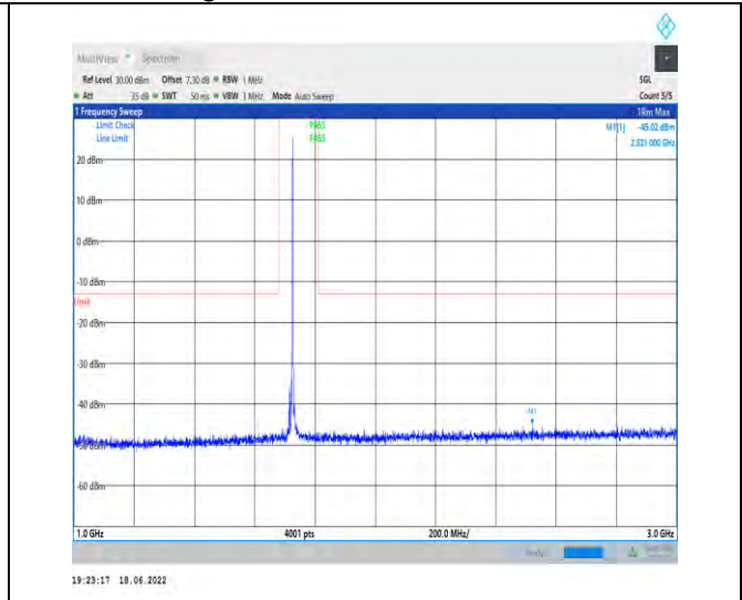
1-N66--15-40-M-1-DFT-PI2BPSK-Inner_1RB_Left-1 @1-1000-3000-Ant1--45.02--13-PASS
