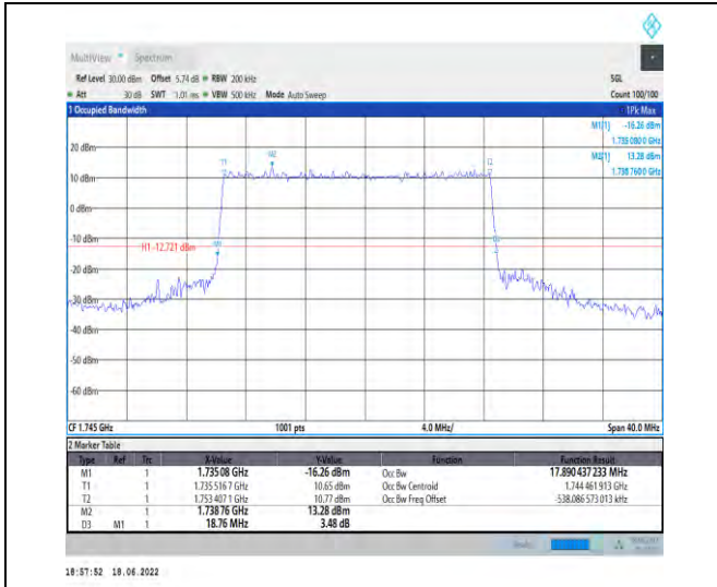
1-N66--15-20-M-3-DFT-16QAM-Outer_Full-100@0-A nt1-17.89-18.760-<20-PASS
