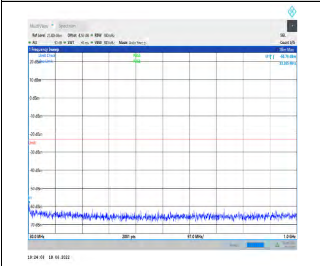
1-N66--15-40-H-1-DFT-PI2BPSK-Inner_1RB_Left-1 @1-30-1000-Ant1--58.74--23-PASS
