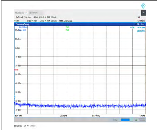
1-N66--15-40-M-1-DFT-PI2BPSK-Inner_1RB_Left-1 @1-30-1000-Ant1--58.71--23-PASS
