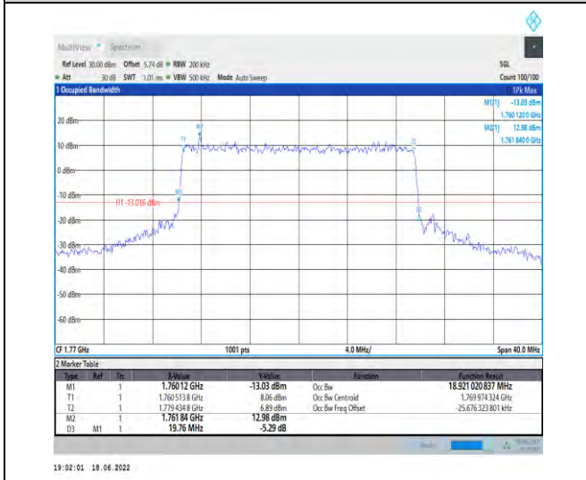
1-N66--15-20-H-8-CP-64QAM-Outer_Full-106@0-An t1-18.921-19.760-≤20-PASS
