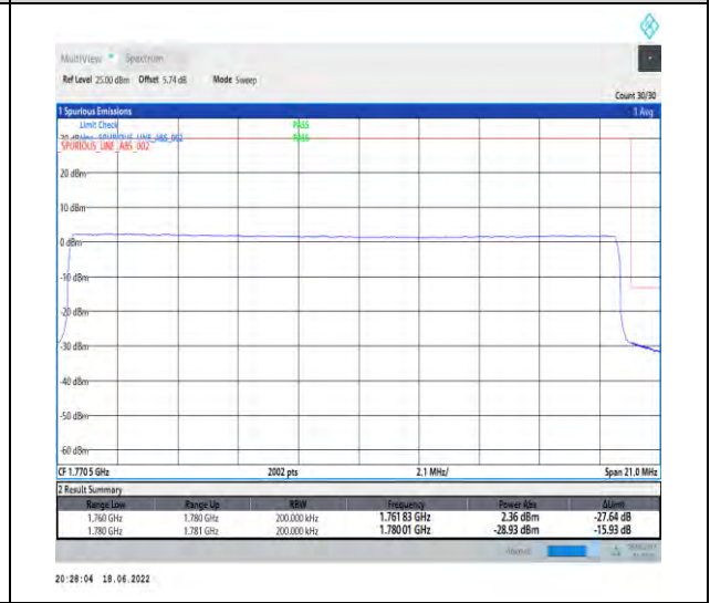
1-N66--15-20-H-6-CP-QPSK-Outer_Full-106@0-A nt1-seegraph-PASS-see graph
