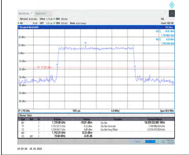
1-N66--15-20-M-9-CP-256QAM-Outer_Full-106@0-A Ant1-18.929-19.840-≤20-PASS
