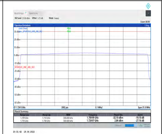
1-N66--15-30-L-6-CP-QPSK-Outer_Full-160@0-Ant1-seegraph-PASS-see graph
