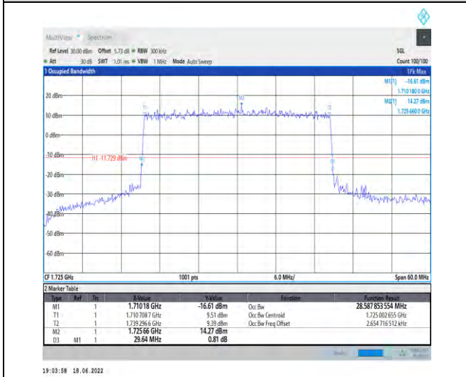
1-N66--15-30-L-3-DFT-16QAM-Outer_Full-160@0-Ant 1-28.588-29.640-≤30-PASS
