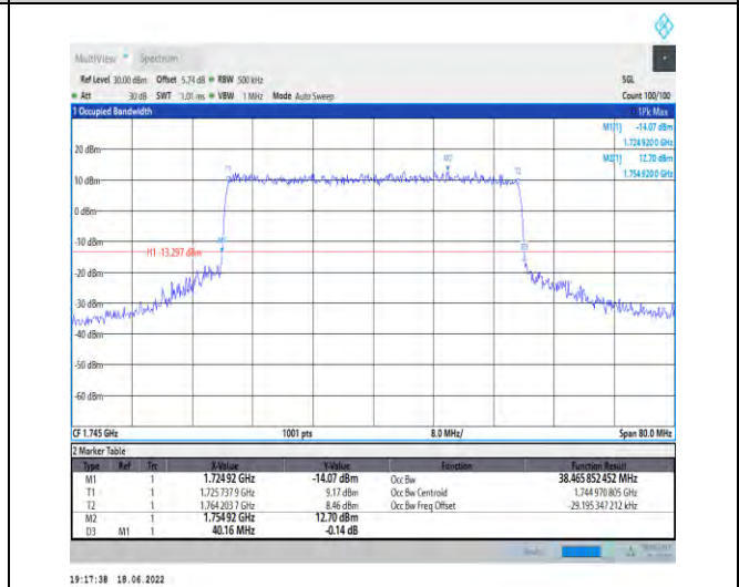
1-N66--15-40-M-8-CP-64QAM-Outer_Full-216@0-Ant1-38.466-40.160-<math>\leq 40</math>-PASS
