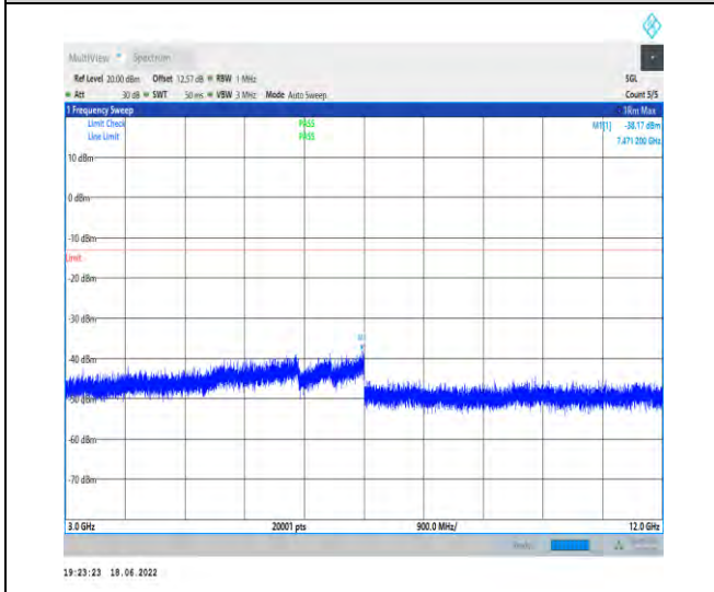
1-N66--15-40-M-1-DFT-PI2BPSK-Inner_1RB_Left-1 @1-3000-12000-Ant1--38.17--13-PASS
