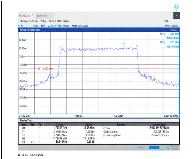
1-N66--15-20-L-8-CP-64QAM-Outer_Full-106@0-An t1-18.913-19.840-<=20-PASS
