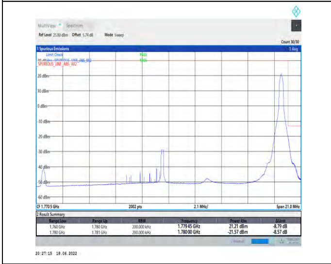
1-N66--15-20-H-5-CP-QPSK-Edge_1RB_Right-1@105 -Ant1-seegraph-PASS-see graph
