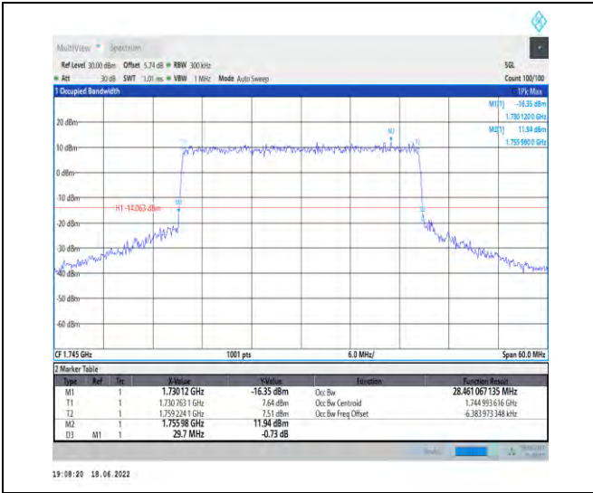
1-N66--15-30-M-8-CP-64QAM-Outer_Full-160@0-A nt1-28.461-29.700-≤30-PASS
