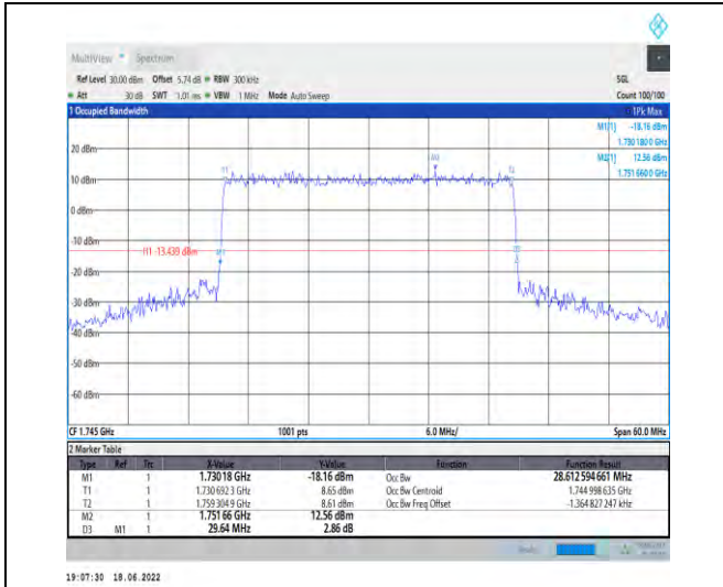
1-N66--15-30-M-4-DFT-64QAM-Outer_Full-160@0-A nt1-28.613-29.640-≤30-PASS
