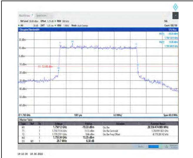
1-N66--15-30-H-3-DFT-16QAM-Outer_Full-160@0-A nt1-28.556-29.700-≤30-PASS
