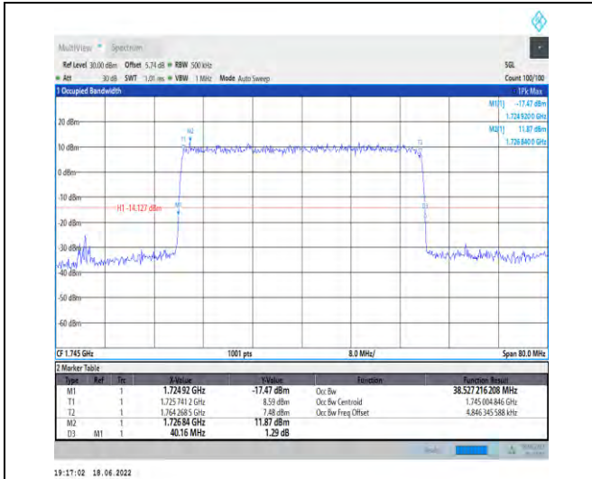
1-N66--15-40-M-5-DFT-256QAM-Outer_Full-216@0-Ant1-38.527-40.160-<math>\leq 40</math>-PASS
