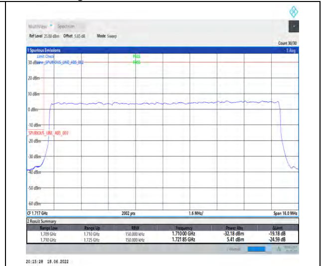
1-N66--15-15-L-3-DFT-PI2BPSK-Outer_Full-75@0-Ant1-seegraph-PASS-see graph
