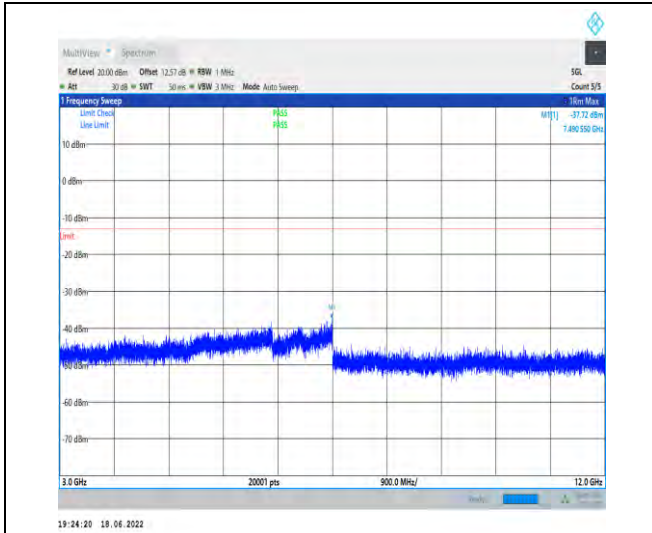
1-N66--15-40-H-1-DFT-PI2BPSK-Inner_1RB_Left-1 @1-3000-12000-Ant1--37.72--13-PASS
