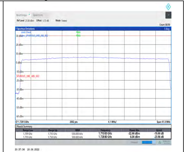
1-N66--15-40-L-3-DFT-PI2BPSK-Outer_Full-216@0-Ant1-seegraph-PASS-see graph
