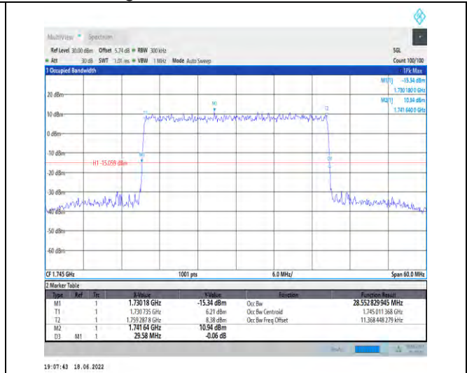
1-N66--15-30-M-5-DFT-256QAM-Outer_Full-160@0-A Ant1-28.553-29.580-≤30-PASS
