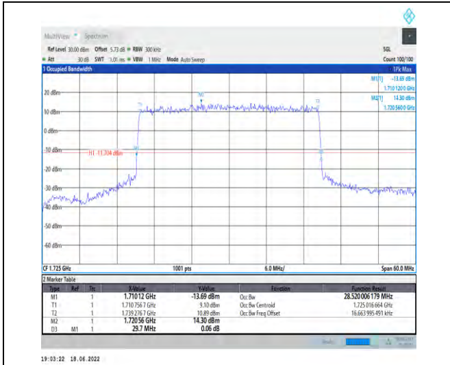
1-N66--15-30-L-1-DFT-QPSK-Outer_Full-160@0-Ant 1-28.52-29.700-≤30-PASS
