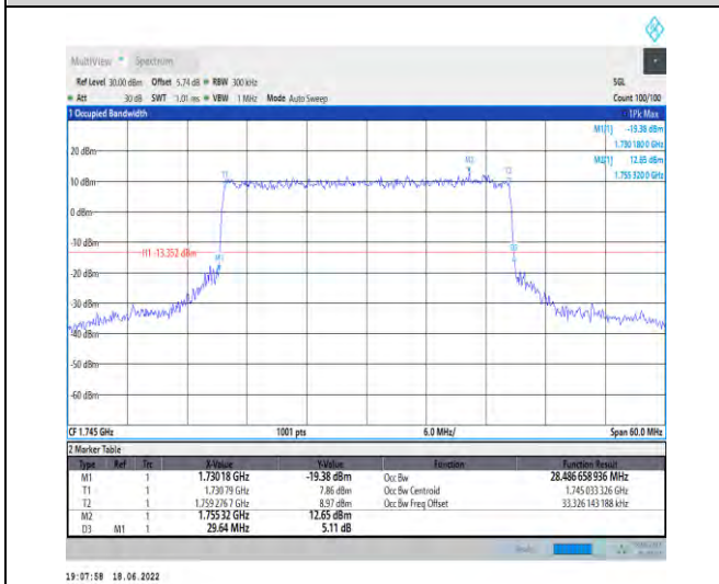
1-N66--15-30-M-6-CP-QPSK-Outer_Full-160@0-Ant 1-28.487-29.640-≤30-PASS
