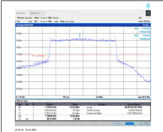
1-N66--15-40-H-8-CP-64QAM-Outer_Full-216@0-An t1-38.393-40.160-<40-PASS
