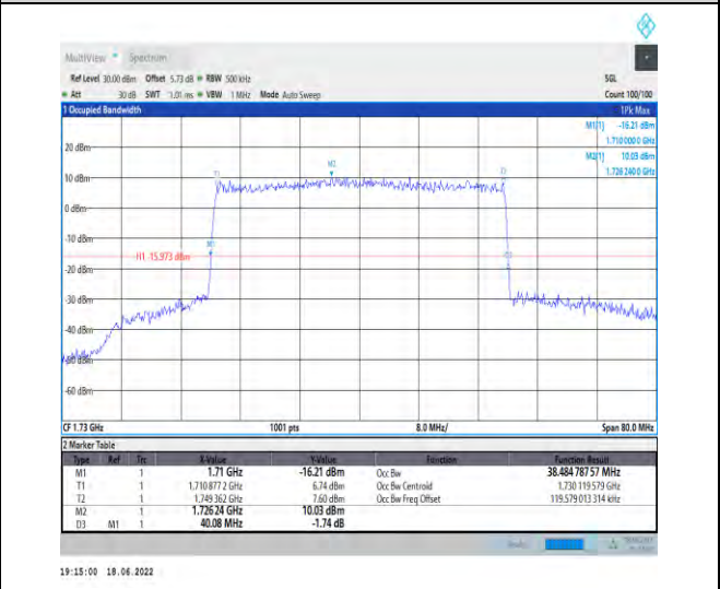
1-N66--15-40-L-9-CP-256QAM-Outer_Full-216@0-Ant1 t1-38.485-40.080-≤40-PASS
