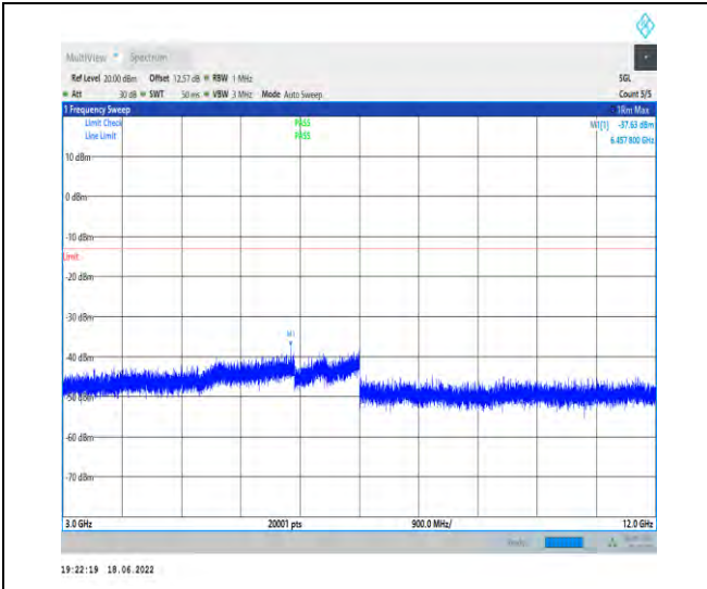
1-N66--15-40-L-1-DFT-PI2BPSK-Inner_1RB_Left-1 @1-3000-12000-Ant1--37.63--13-PASS
