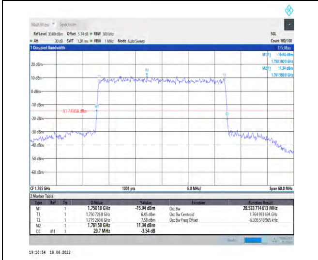
1-N66--15-30-H-5-DFT-256QAM-Outer_Full-160@0-Ant1 Ant1-28.534-29.700-≤30-PASS
