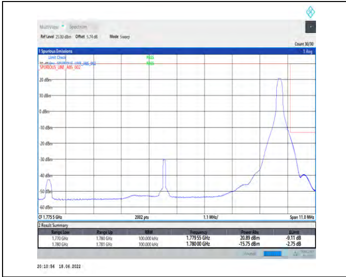
1-N66--15-10-H-2-DFT-PI2BPSK-Edge_1RB_Right-1@51-Ant1-seegraph-PASS-see graph
