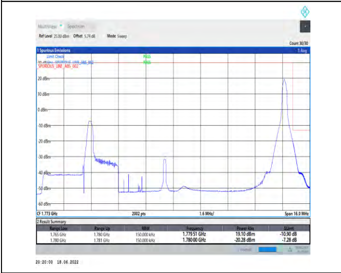
1-N66--15-15-H-5-CP-QPSK-Edge_1RB_Right-1@78-Ant1-seegraph-PASS-see graph
