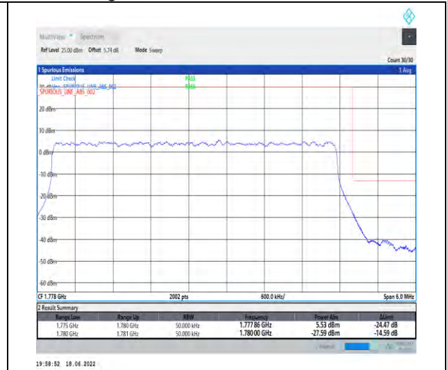
1-N66--15-5-H-3-DFT-PI2BPSK-Outer_Full-25@0-Ant1-seegraph-PASS-see graph
