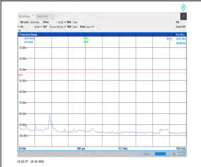
1-N66--15-40-M-1-DFT-PI2BPSK-Inner_1RB_Left-1 @1-0.009-0.15-Ant1--83.97--43-PASS
