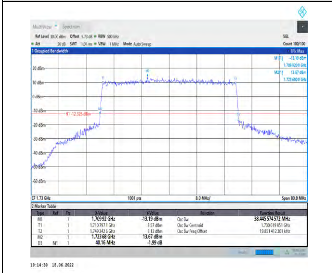
1-N66--15-40-L-8-CP-64QAM-Outer_Full-216@0-Ant1 t1-38.446-40.160-≤40-PASS
