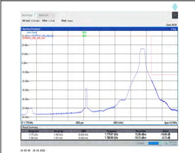
1-N66--15-5-H-5-CP-QPSK-Edge_1RB_Right-1@24-Ant1-seegraph-PASS-see graph
