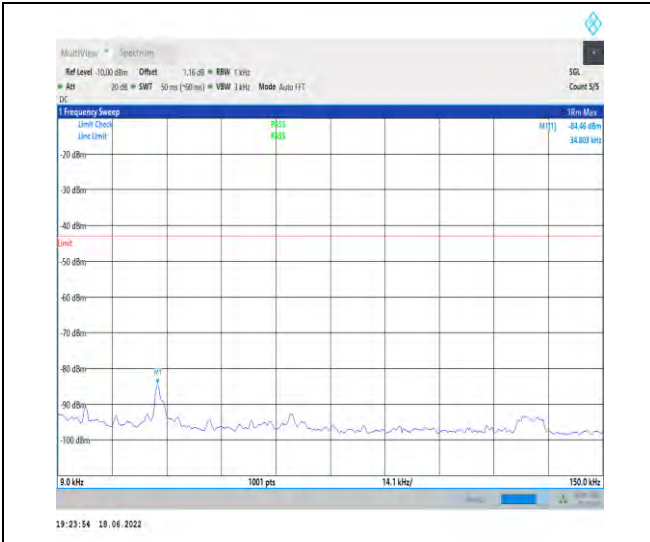
1-N66--15-40-H-1-DFT-PI2BPSK-Inner_1RB_Left-1 @1-0.009-0.15-Ant1--84.46--43-PASS
