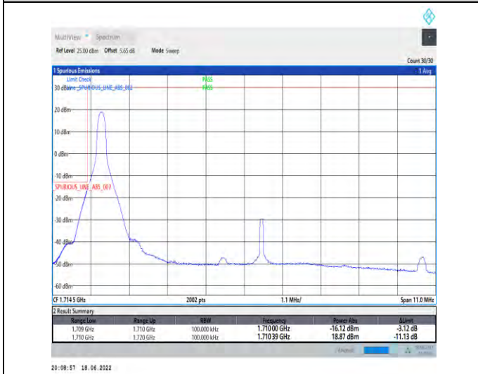
1-N66--15-10-L-4-CP-QPSK-Edge_1RB_Left-1@0-Ant1-seegraph-PASS-see graph
