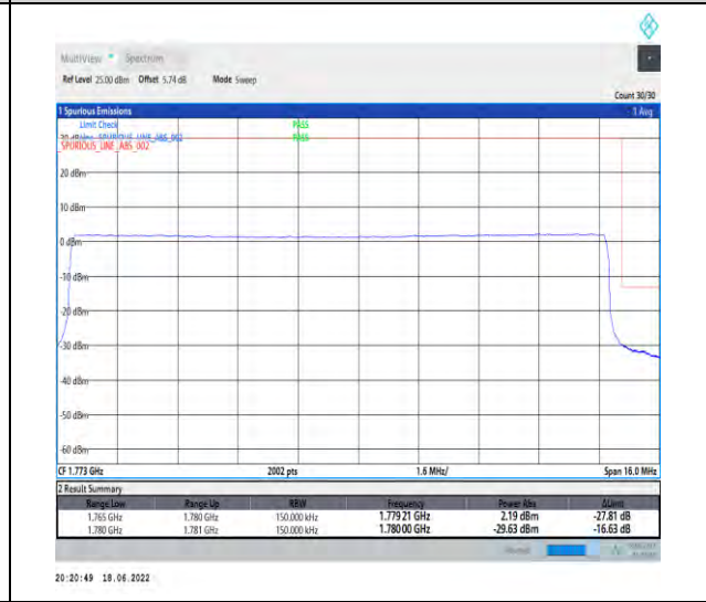
1-N66--15-15-H-6-CP-QPSK-Outer_Full-79@0-Ant1-seegraph-PASS-see graph
