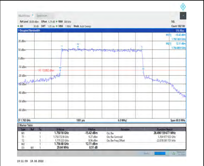
1-N66--15-30-H-6-CP-QPSK-Outer_Full-160@0-Ant 1-28.49-29.640-≤30-PASS
