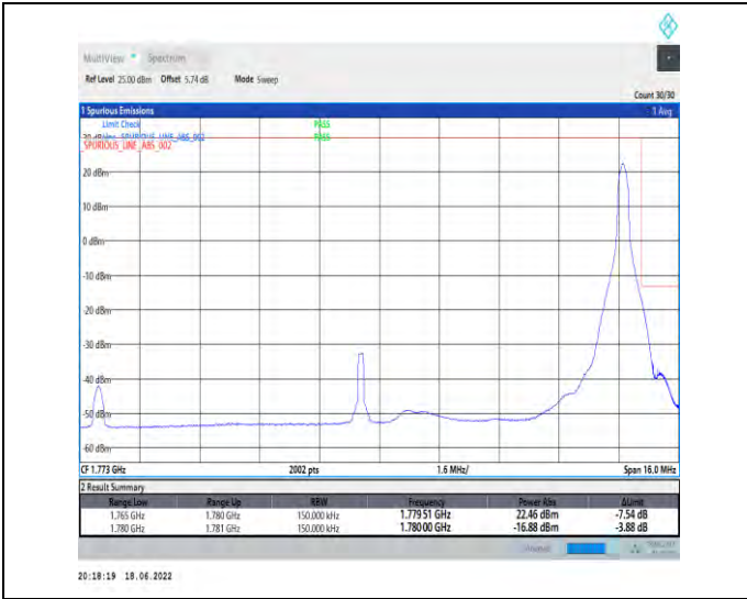
1-N66--15-15-H-2-DFT-PI2BPSK-Edge_1RB_Right-1@78-Ant1-seegraph-PASS-see graph
