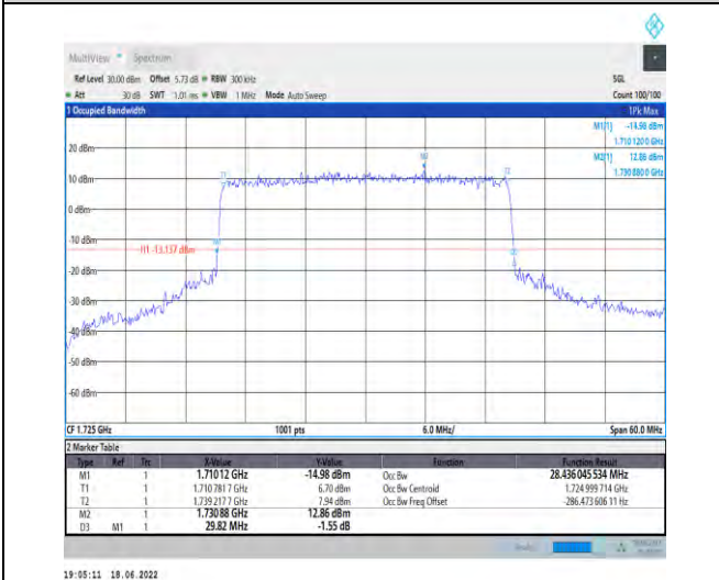
1-N66--15-30-L-7-CP-16QAM-Outer_Full-160@0-Ant1-28.436-29.820-<=30-PASS
