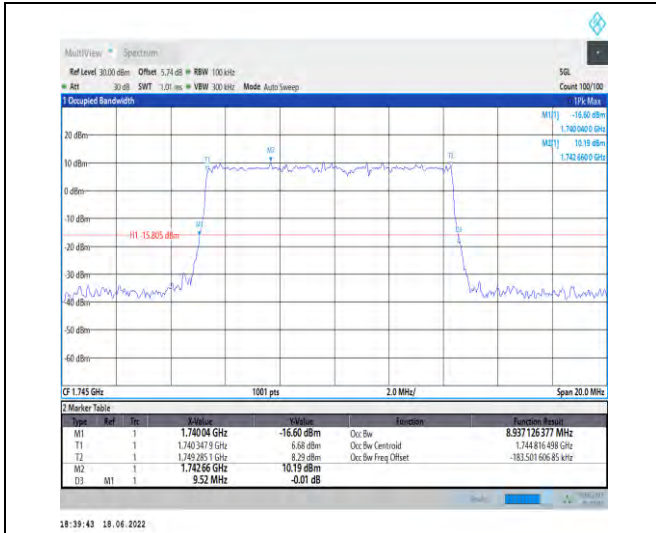
1-N66--15-10-M-5-DFT-256QAM-Outer_Full-50@0-A nt1-8.937-9.520-≤10-PASS
