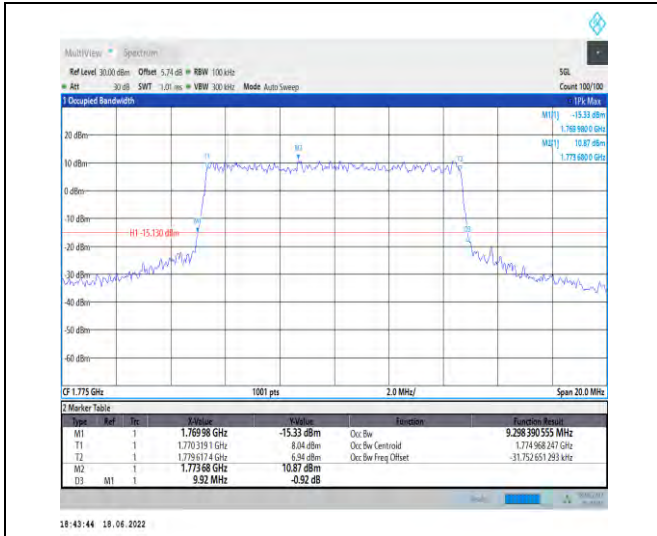
1-N66--15-10-H-8-CP-64QAM-Outer_Full-52@0-Ant 1-9.298-9.920≤10-PASS
