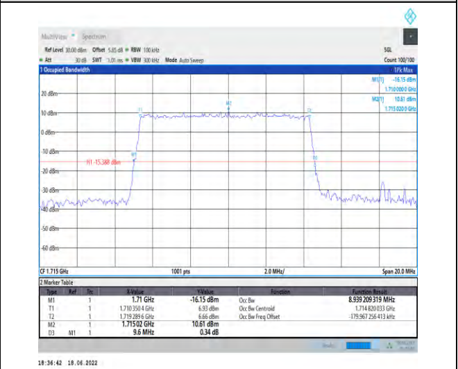
1-N66--15-10-L-5-DFT-256QAM-Outer_Full-50@0-A nt1-8.939-9.600-≤10-PASS
