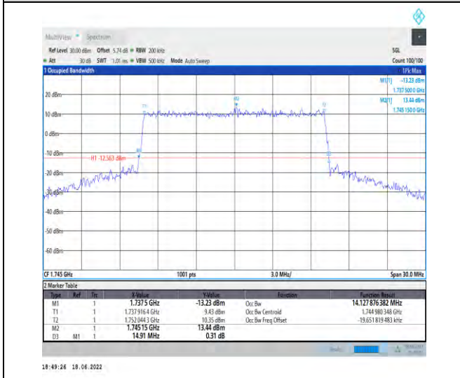
1-N66--15-15-M-8-CP-64QAM-Outer_Full-79@0-Ant 1-14.128-14.910-≤15-PASS
