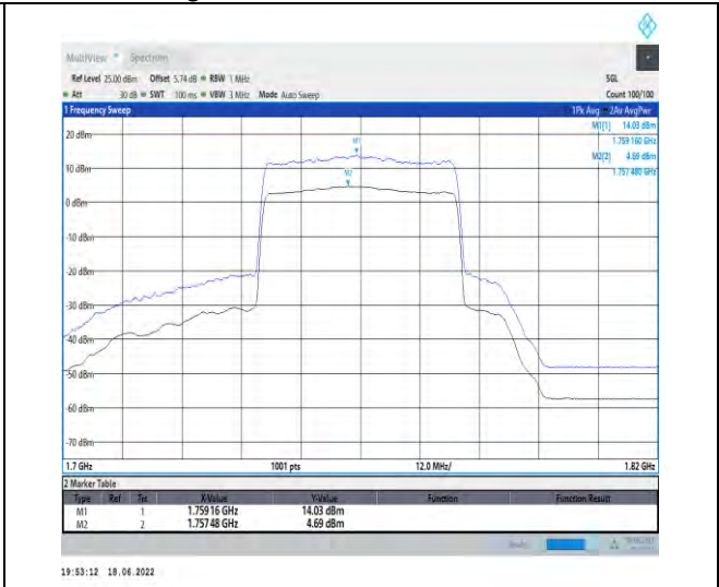
1-N66--15-40-H-2-CP-256QAM-Outer_Full-216@0-Ant1-9.34-100%-0.00-9.34-PASS- \leq 13
