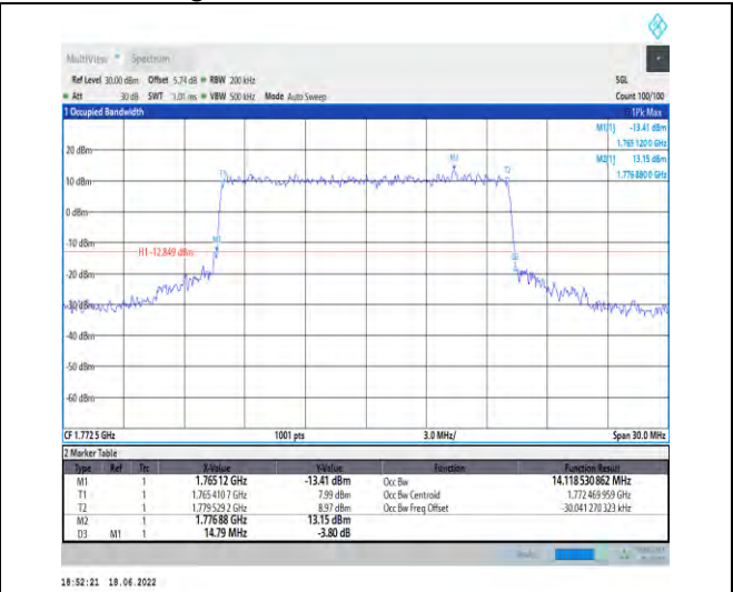
1-N66--15-15-H-6-CP-QPSK-Outer_Full-79@0-Ant1- 14.119-14.790-≤15-PASS
