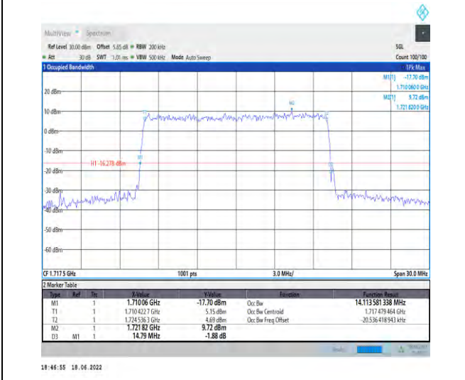
1-N66--15-15-L-9-CP-256QAM-Outer_Full-79@0-An t1-14.114-14.790-≤15-PASS
