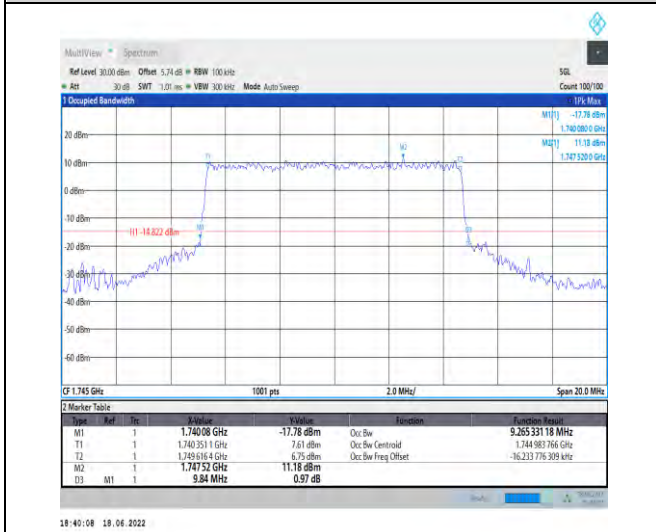
1-N66--15-10-M-7-CP-16QAM-Outer_Full-52@0-Ant 1-9.265-9.840-≤10-PASS
