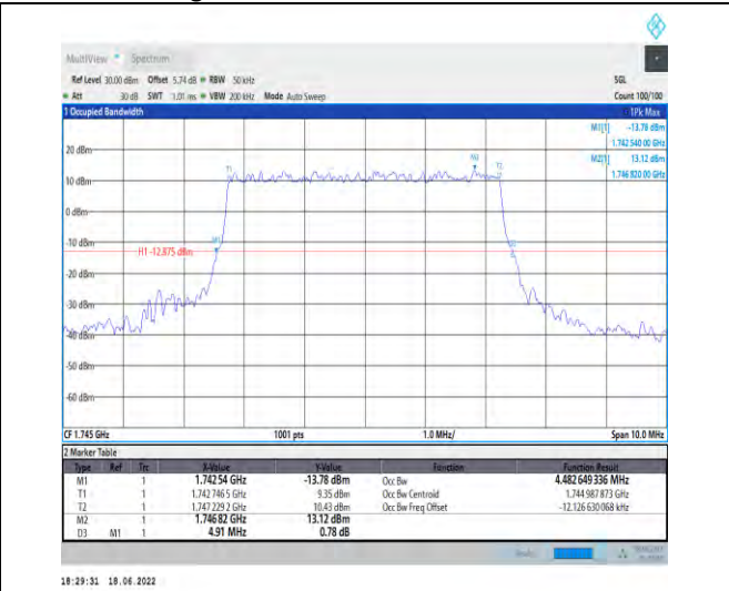
1-N66--15-5-M-1-DFT-QPSK-Outer_Full-25@0-Ant1- 4.483-4.910-≤5-PASS
