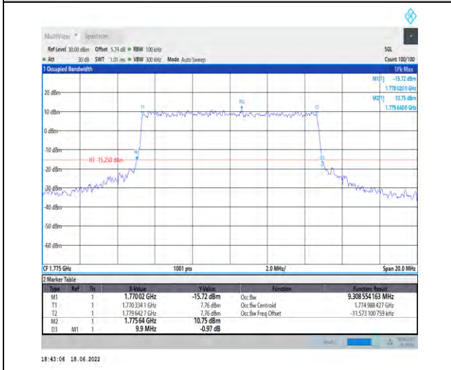
1-N66--15-10-H-6-CP-QPSK-Outer_Full-52@0-Ant-1 9.309-9.900-≤10-PASS
