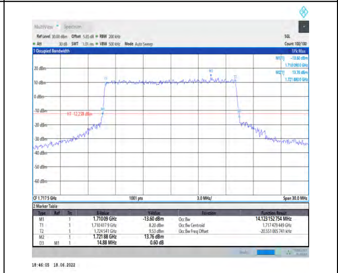
1-N66--15-15-L-6-CP-QPSK-Outer_Full-79@0-Ant1 14.123-14.880-≤15-PASS
