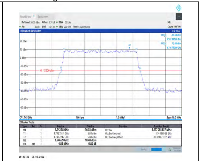
1-N66--15-5-M-5-DFT-256QAM-Outer_Full-25@0-An t1-4.477-4.860-≤5-PASS
