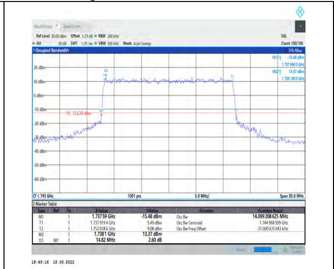
1-N66--15-15-M-7-CP-16QAM-Outer_Full-79@0-Ant 1-14.099-14.820-≤15-PASS
