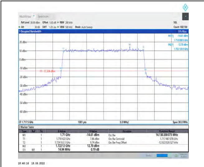
1-N66--15-15-L-7-CP-16QAM-Outer_Full-79@0-Ant 1-14.13-14.940-≤15-PASS
