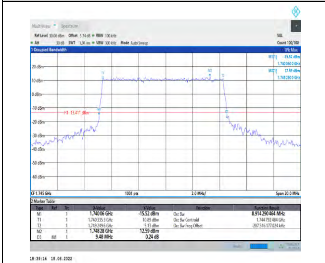
1-N66--15-10-M-3-DFT-16QAM-Outer_Full-50@0-Ant t1-8.914-9.480-≤10-PASS
