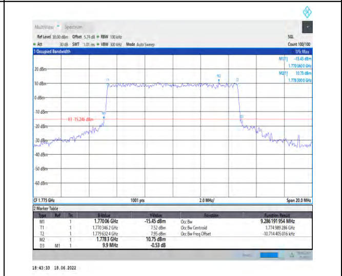
1-N66--15-10-H-7-CP-16QAM-Outer_Full-52@0-Ant 1-9.286-9.900-≤10-PASS
