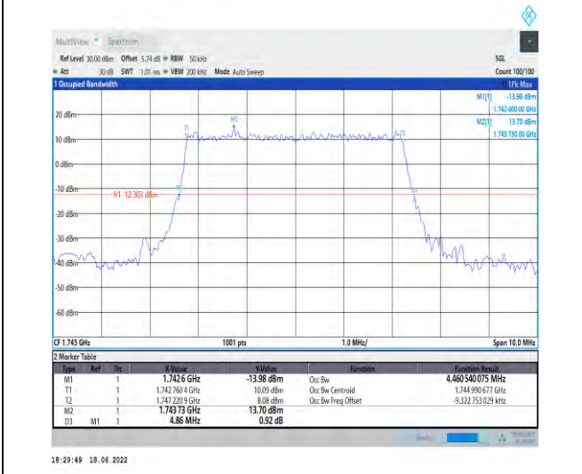
1-N66--15-5-M-2-DFT-PI2BPSK-Outer_Full-25@0-A nt1-4.461-4.860-≤5-PASS
