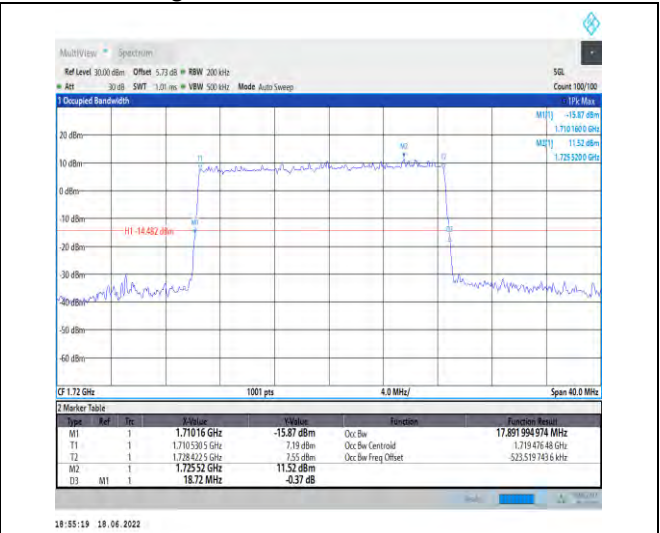
1-N66--15-20-L-5-DFT-256QAM-Outer_Full-100@0-A Ant1-17.892-18.720-≤20-PASS
