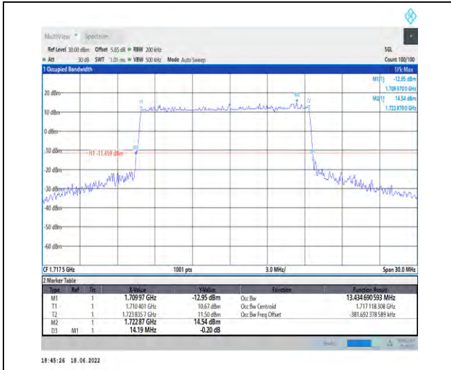
1-N66--15-15-L-3-DFT-16QAM-Outer_Full-75@0-Ant 1-13.435-14.190-≤15-PASS
