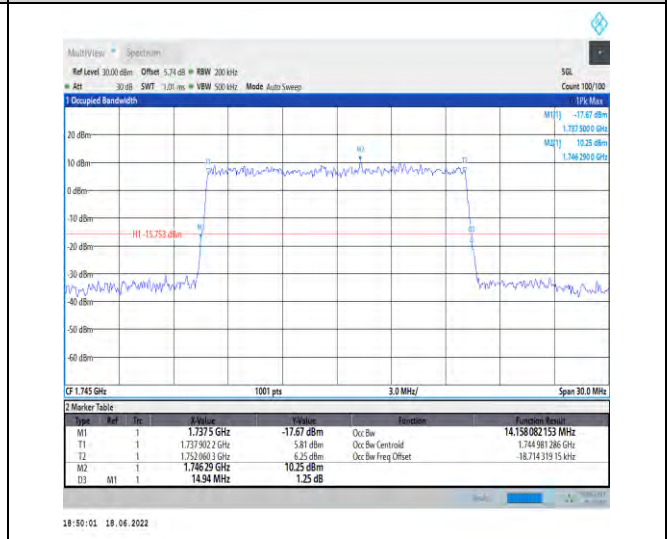
1-N66--15-15-M-9-CP-256QAM-Outer_Full-79@0-A nt1-14.158-14.940-≤15-PASS
