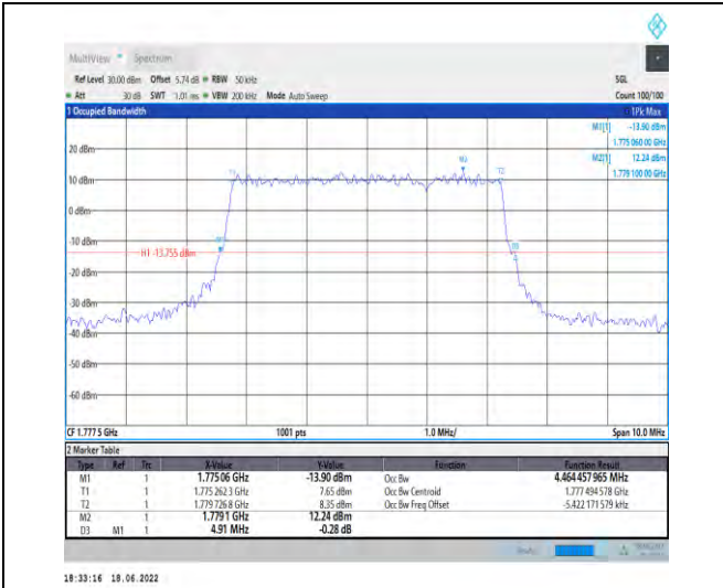
1-N66--15-5-H-3-DFT-16QAM-Outer_Full-25@0-Ant 1-4.464-4.910-≤5-PASS
