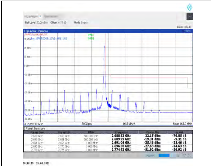
1-N41-PC2-30-80-H-2-DFT-PI2BPSK-Edge_1RB_Right t-1@216-Ant1-PASS-see graph
