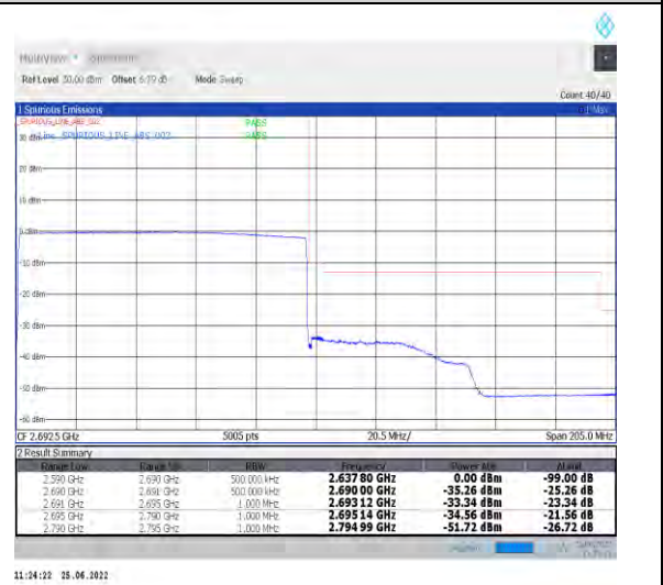
1-N41-PC2-30-100-H-6-CP-QPSK-Outer_Full-273 @0-Ant1-PASS-see graph
