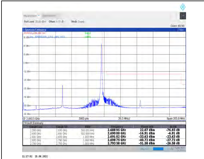
1-N41-PC2-30-100-H-2-DFT-PI2BPSK-Edge_1RB_Rig ht-1@272-Ant1-PASS-see graph
