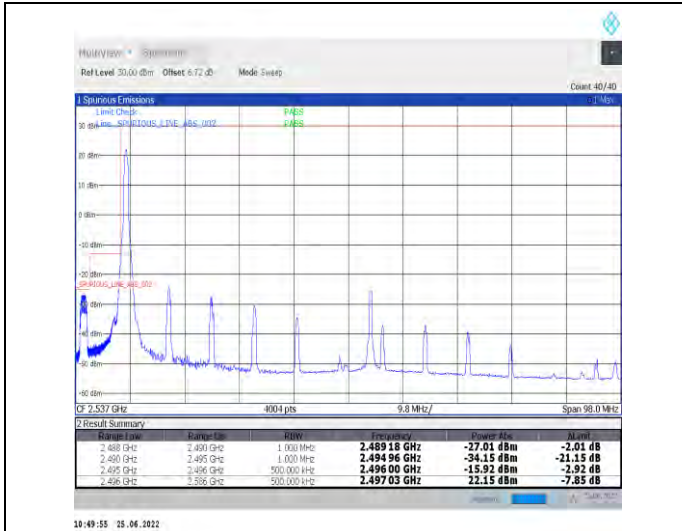
1-N41-PC2-30-90-L-1-DFT-PI2BPSK-Edge_1RB_Left-1@0-Ant1-PASS-see graph
