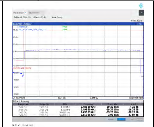
1-N41-PC2-30-90-L-3-DFT-PI2BPSK-Outer_Full-240@0-Ant1-PASS-see graph
