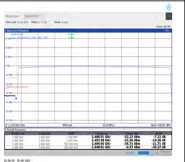
1-N41-PC2-30-100-L-6-CP-QPSK-Outer_Full-273@0-Ant1-PASS-see graph
