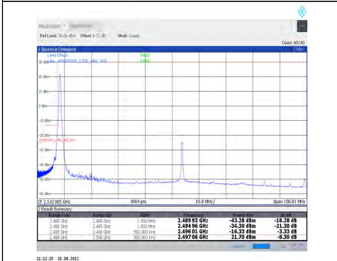
1-N41-PC2-30-100-L-4-CP-QPSK-Edge_1RB_Left-1@0-Ant1-PASS-see graph
