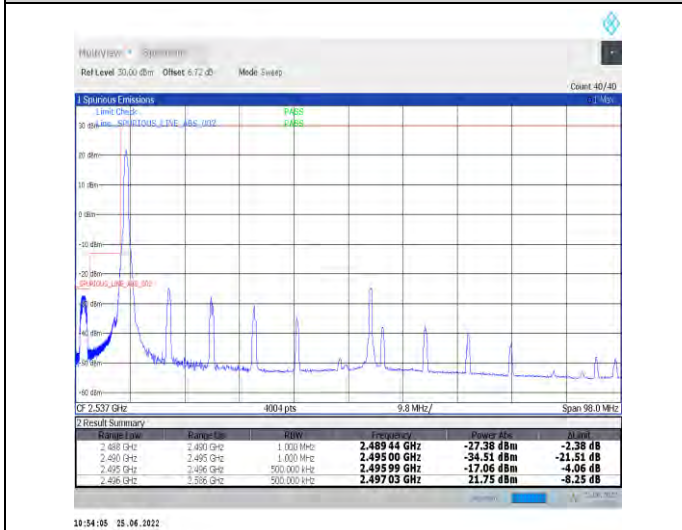
1-N41-PC2-30-90-L-4-CP-QPSK-Edge_1RB_Left-1@0-Ant1-PASS-see graph
