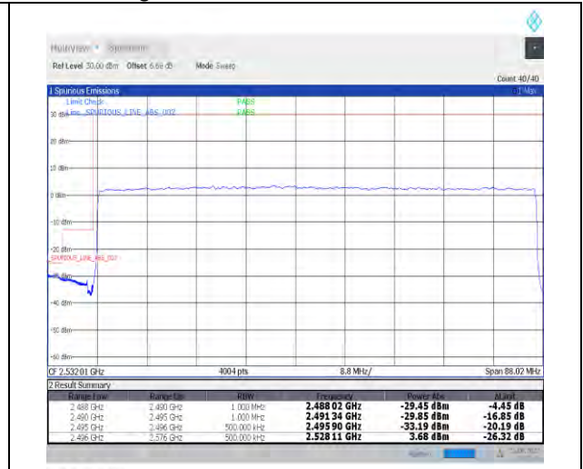
1-N41-PC2-30-80-L-3-DFT-PI2BPSK-Outer_Full-216@0-Ant1-PASS-see graph
