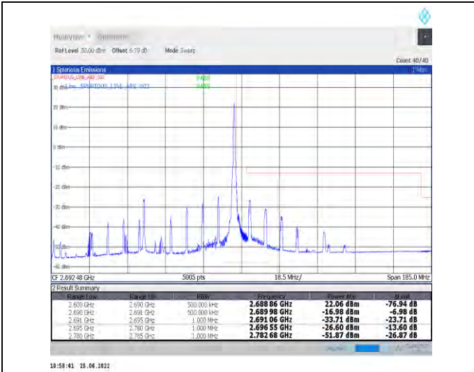
1-N41-PC2-30-90-H-2-DFT-PI2BPSK-Edge_1RB_Right-t1@244-Ant1-PASS-see graph
