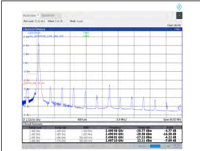
1-N41-PC2-30-80-L-1-DFT-PI2BPSK-Edge_1RB_Left-1@0-Ant1-PASS-see graph
