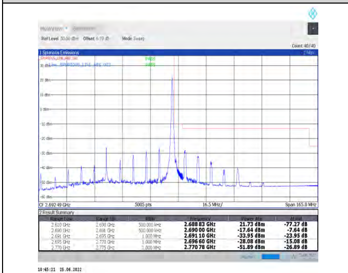
1-N41-PC2-30-80-H-5-CP-QPSK-Edge_1RB_Right-1 @216-Ant1-PASS-see graph
