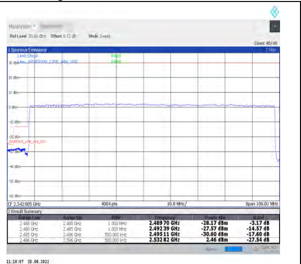
1-N41-PC2-30-100-L-3-DFT-PI2BPSK-Outer_Full-270@0-Ant1-PASS-see graph
