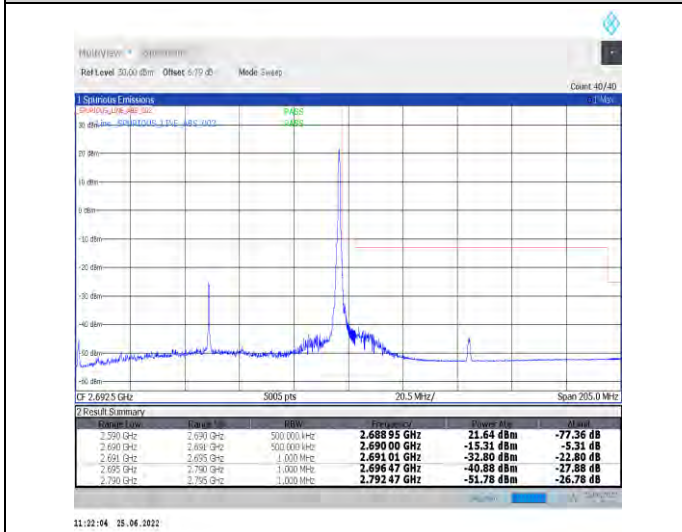
1-N41-PC2-30-100-H-5-CP-QPSK-Edge_1RB_Right-1 @272-Ant1-PASS-see graph
