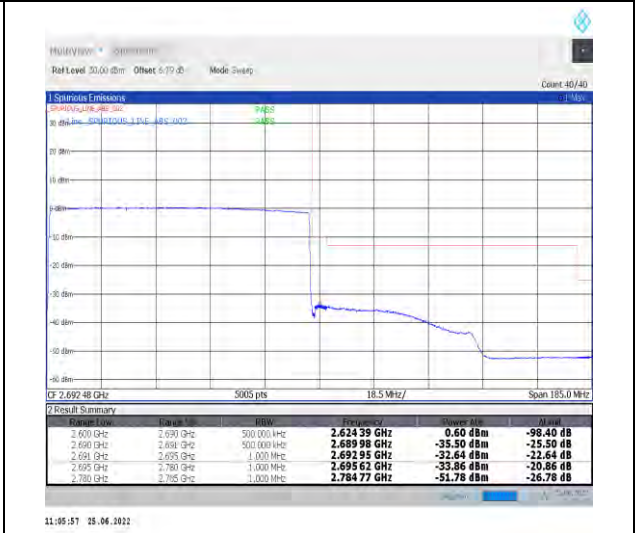
1-N41-PC2-30-90-H-6-CP-QPSK-Outer_Full-245@0-Ant1-PASS-see graph
