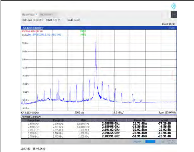
1-N41-PC2-30-90-H-5-CP-QPSK-Edge_1RB_Right-1@244-Ant1-PASS-see graph
