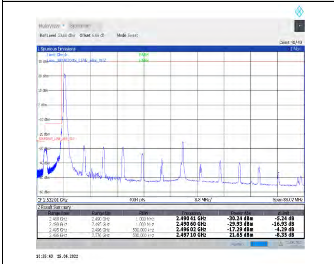
1-N41-PC2-30-80-L-4-CP-QPSK-Edge_1RB_Left-1@0-Ant1-PASS-see graph
