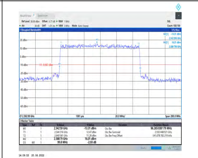
1-N41-PC2-30-100-M-2-DFT-PI2BPSK-Outer_Full-270 @0-Ant1-96.265-99.800-≤100-PASS
