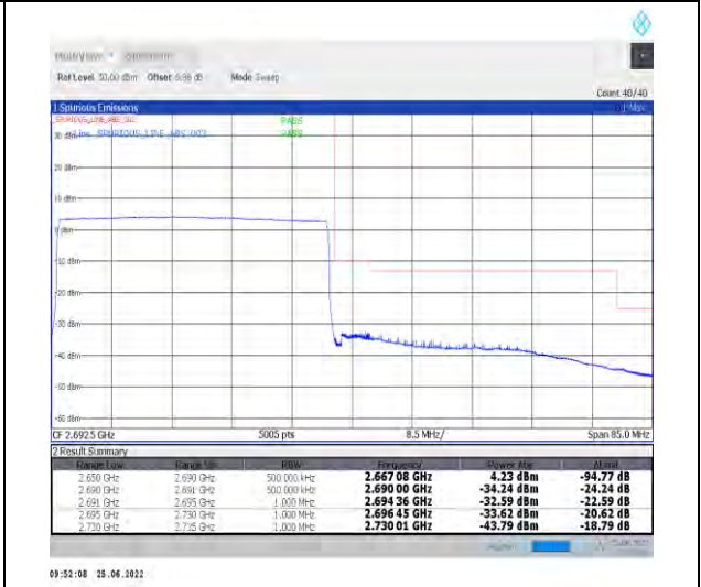
1-N41-PC2-30-40-H-6-CP-QPSK-Outer_Full-106 @0-Ant1-PASS-see graph
