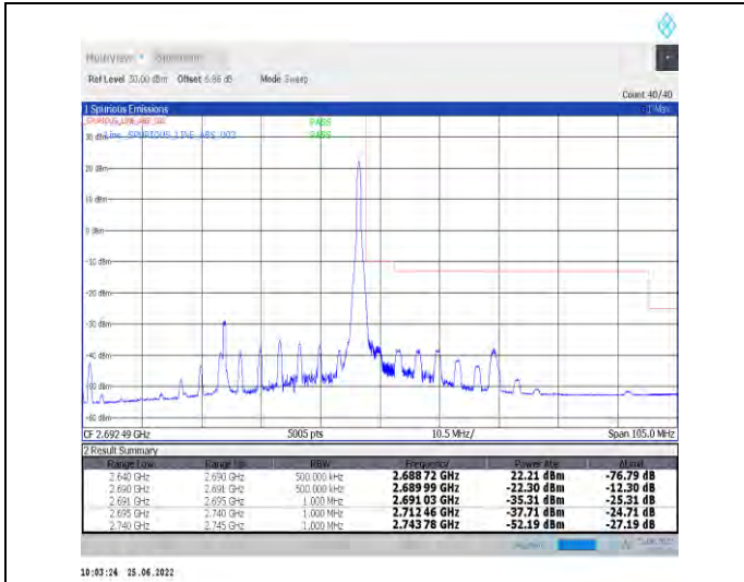
1-N41-PC2-30-50-H-2-DFT-PI2BPSK-Edge_1RB_Right-t1@132-Ant1-PASS-see graph
