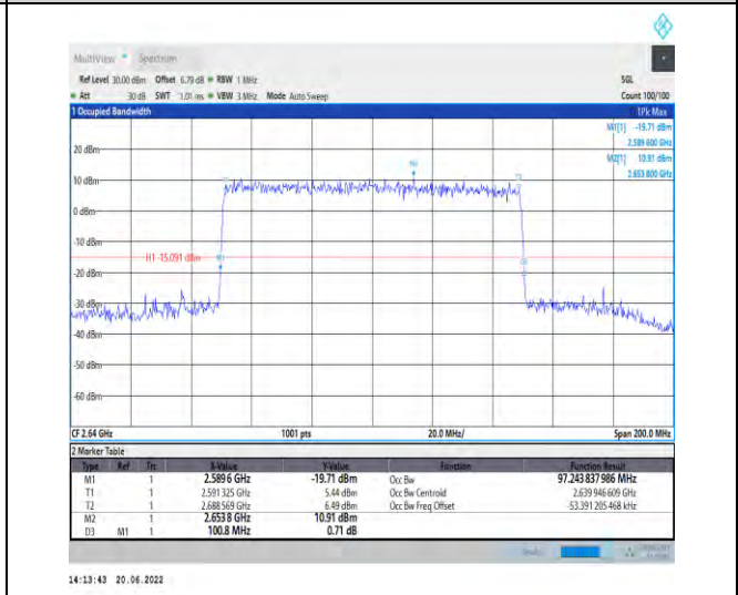
1-N41-PC2-30-100-H-9-CP-256QAM-Outer_Full-273 @0-Ant1-97.244-100.800-≤100-PASS
