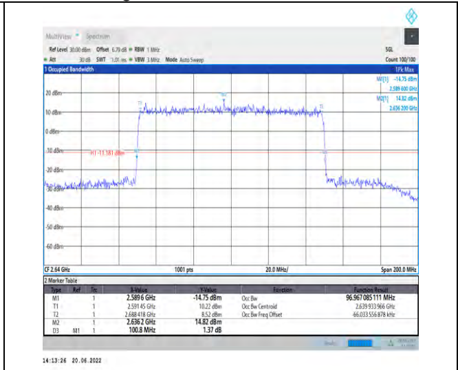
1-N41-PC2-30-100-H-7-CP-16QAM-Outer_Full-273 @0-Ant1-96.967-100.800-≤100-PASS
