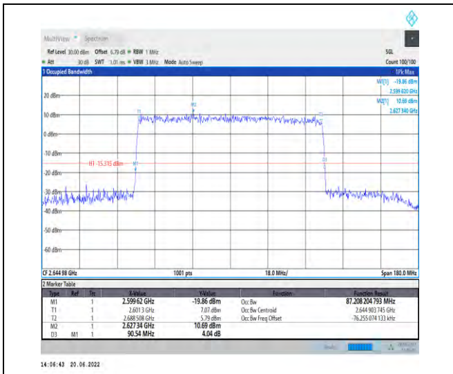
1-N41-PC2-30-90-H-9-CP-256QAM-Outer_Full-245 @0-Ant1-87.208-90.540-≤90-PASS
