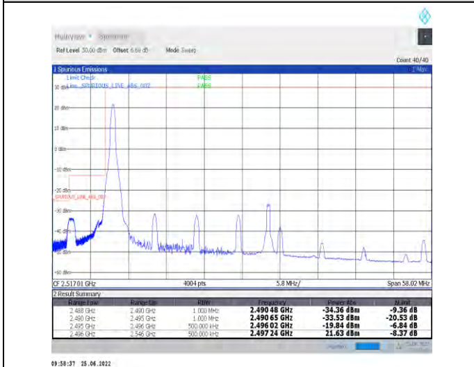
1-N41-PC2-30-50-L-4-CP-QPSK-Edge_1RB_Left-1@0-Ant1-PASS-see graph
