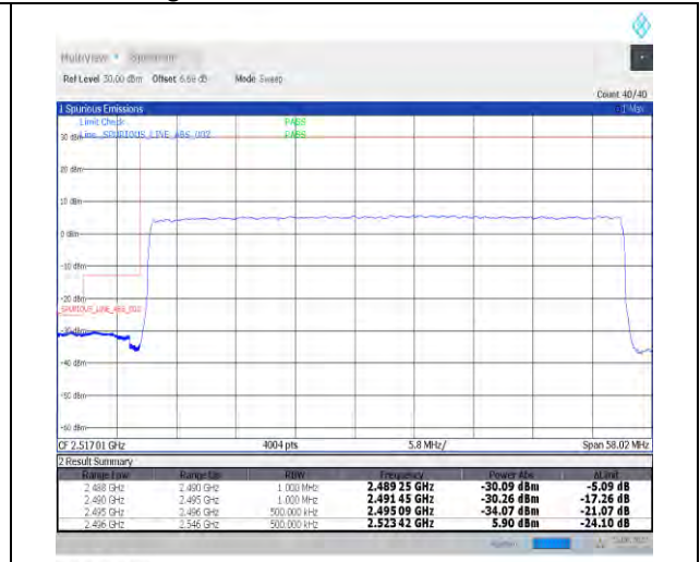
1-N41-PC2-30-50-L-3-DFT-PI2BPSK-Outer_Full-128@0-Ant1-PASS-see graph
