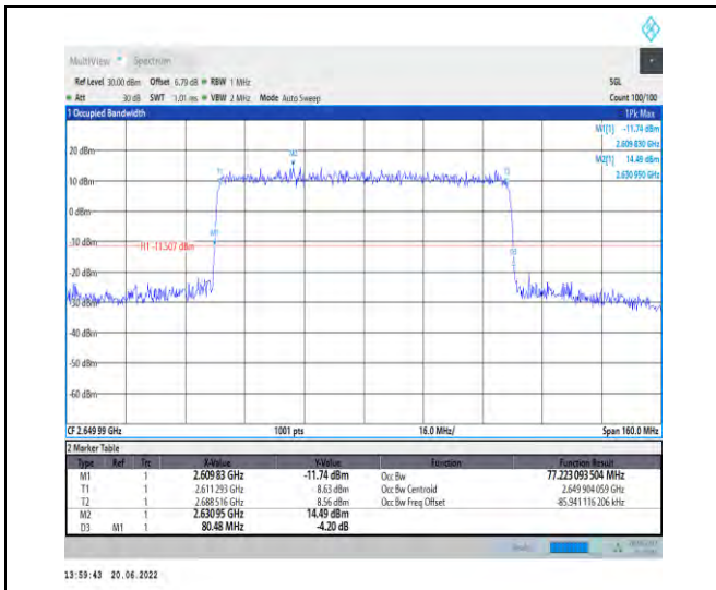
1-N41-PC2-30-80-H-8-CP-64QAM-Outer_Full-217@ 0-Ant1-77.223-80.480-≤80-PASS
