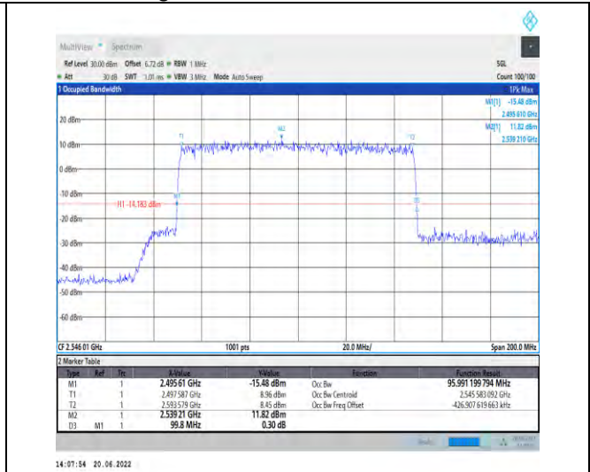
1-N41-PC2-30-100-L-5-DFT-256QAM-Outer_Full-270 @0-Ant1-95.991-99.800-≤100-PASS
