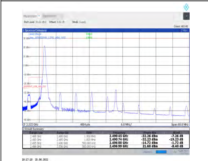
1-N41-PC2-30-60-L-4-CP-QPSK-Edge_1RB_Left-1@0-Ant1-PASS-see graph
