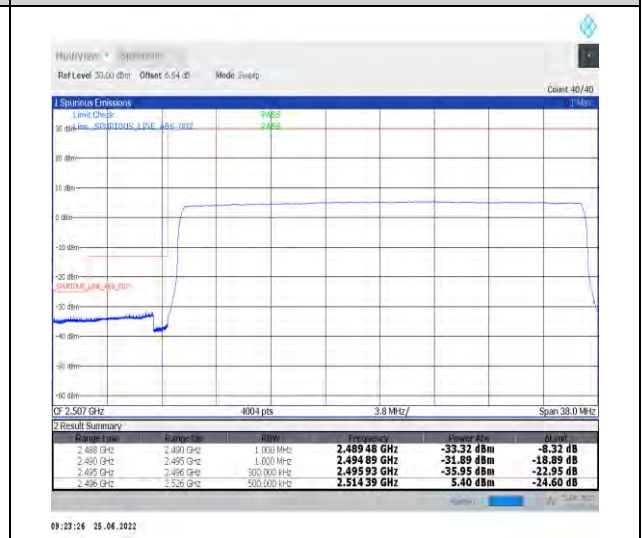
1-N41-PC2-30-30-L-6-CP-QPSK-Outer_Full-78@0-Ant1-PASS-see graph
