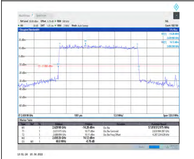
1-N41-PC2-30-60-H-1-DFT-QPSK-Outer_Full-162@ 0-Ant1-57.819-60.000-≤60-PASS
