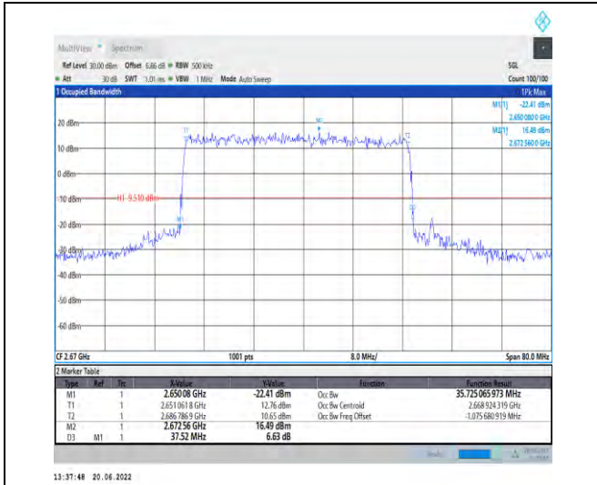
1-N41-PC2-30-40-H-1-DFT-QPSK-Outer_Full-100@ 0-Ant1-35.725-37.520-≤40-PASS
