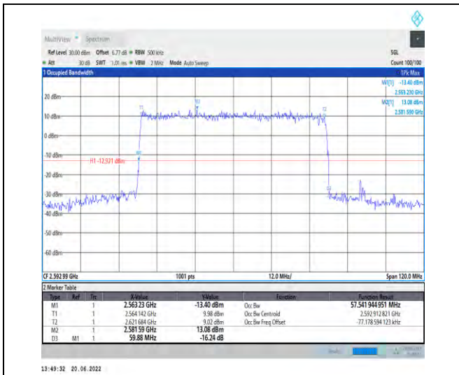
1-N41-PC2-30-60-M-4-DFT-64QAM-Outer_Full-162 @0-Ant1-57.542-59.880-≤60-PASS
