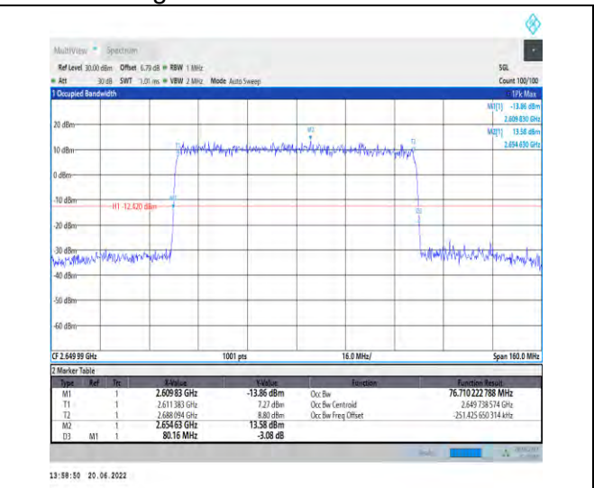
1-N41-PC2-30-80-H-5-DFT-256QAM-Outer_Full-216 @0-Ant1-76.71-80.160-≤80-PASS
