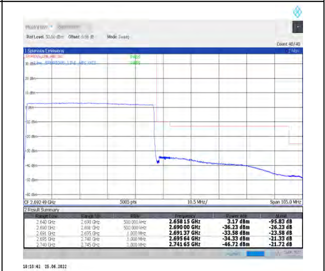
1-N41-PC2-30-50-H-6-CP-QPSK-Outer_Full-133@0-Ant1-PASS-see graph
