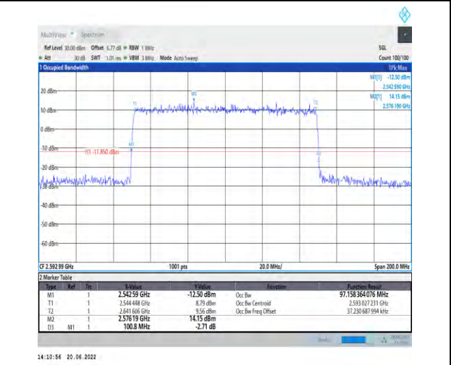
1-N41-PC2-30-100-M-6-CP-QPSK-Outer_Full-273 @0-Ant1-97.158-100.800-≤100-PASS
