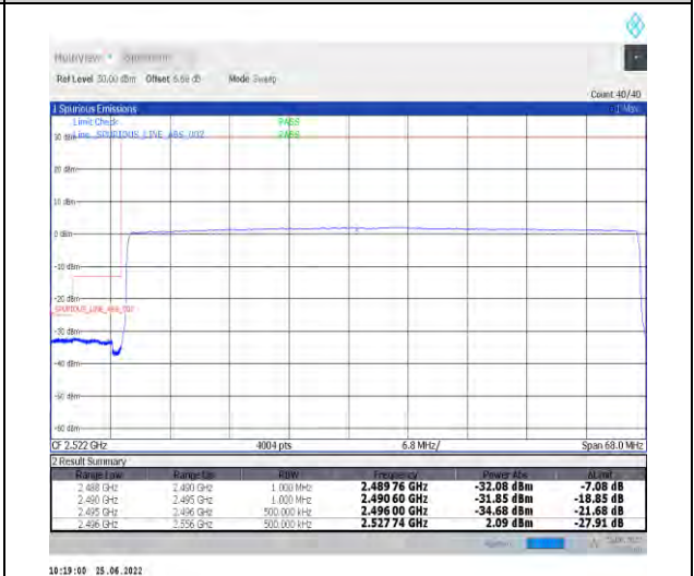
1-N41-PC2-30-60-L-6-CP-QPSK-Outer_Full-162@0-Ant1-PASS-see graph
