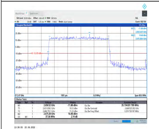
1-N41-PC2-30-40-H-3-DFT-16QAM-Outer_Full-100 @0-Ant1-35.734-37.360-≤40-PASS
