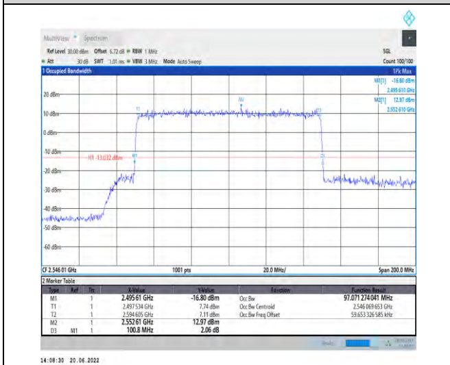
1-N41-PC2-30-100-L-6-CP-QPSK-Outer_Full-273 @0-Ant1-97.071-100.800-≤100-PASS
