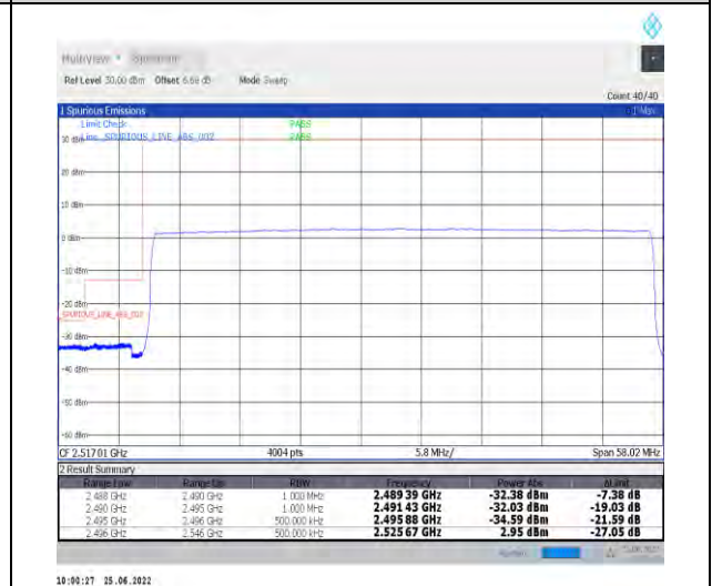
1-N41-PC2-30-50-L-6-CP-QPSK-Outer_Full-133@0-Ant1-PASS-see graph
