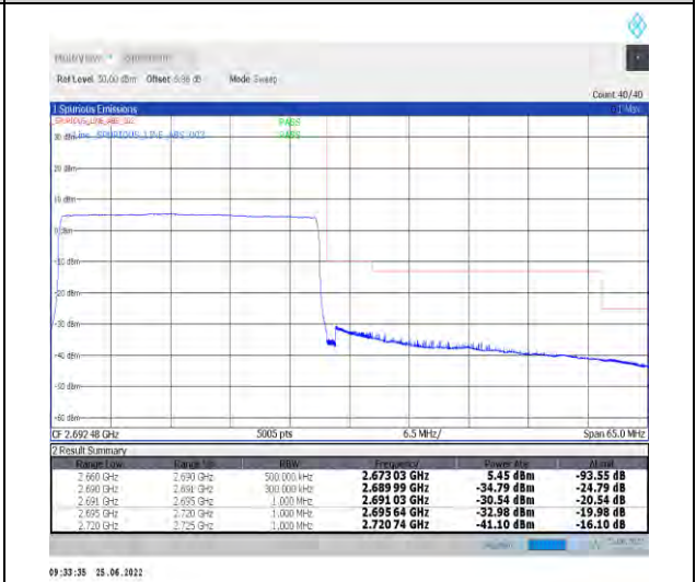
1-N41-PC2-30-30-H-6-CP-QPSK-Outer_Full-78@0-Ant1-PASS-see graph
