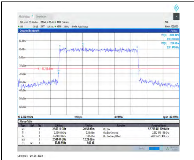
1-N41-PC2-30-60-M-8-CP-64QAM-Outer_Full-162@ 0-Ant1-57.738-59.880-≤60-PASS
