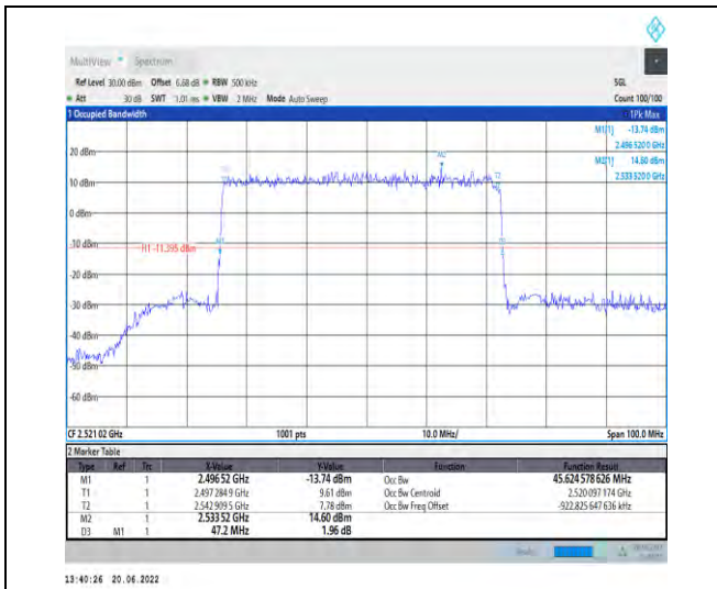
1-N41-PC2-30-50-L-4-DFT-64QAM-Outer_Full-128 @0-Ant1-45.625-47.200-≤50-PASS
