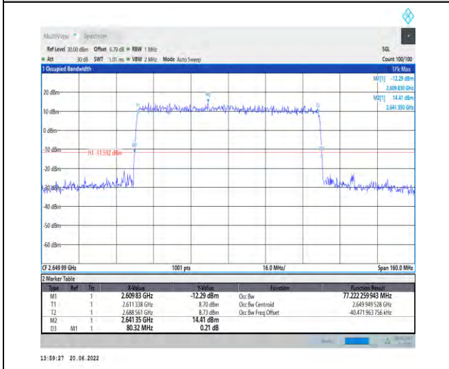
1-N41-PC2-30-80-H-6-CP-QPSK-Outer_Full-217@0 -Ant1-77.222-80.320-≤80-PASS
