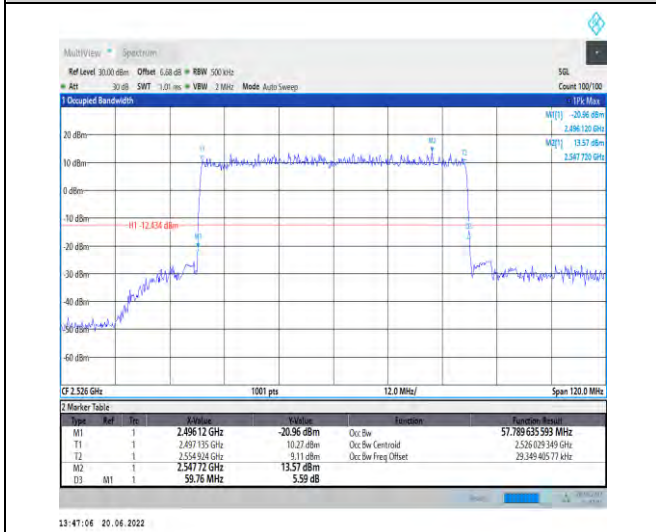
1-N41-PC2-30-60-L-3-DFT-16QAM-Outer_Full-162 @0-Ant1-57.79-59.760-≤60-PASS
