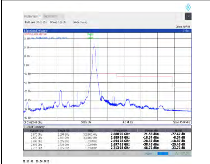
1-N41-PC2-30-20-H-5-CP-QPSK-Edge_1RB_Right-1@50-Ant1-PASS-see graph
