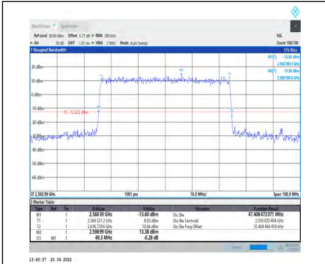
1-N41-PC2-30-50-M-7-CP-16QAM-Outer_Full-133@ 0-Ant1-47.408-49.300-≤50-PASS
