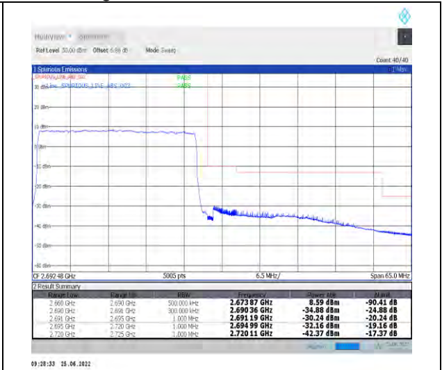
1-N41-PC2-30-30-H-3-DFT-PI2BPSK-Outer_Full-75@0-Ant1-PASS-see graph
