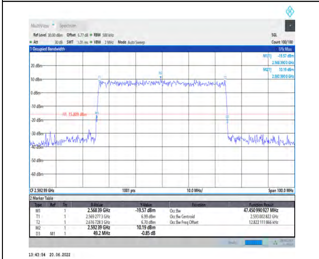
1-N41-PC2-30-50-M-9-CP-256QAM-Outer_Full-133 @0-Ant1-47.451-49.200-≤50-PASS
