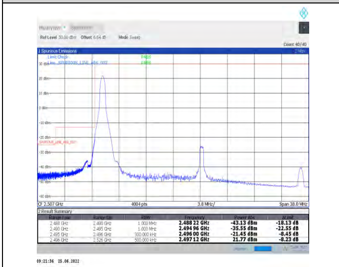
1-N41-PC2-30-30-L-4-CP-QPSK-Edge_1RB_Left-1@0-Ant1-PASS-see graph
