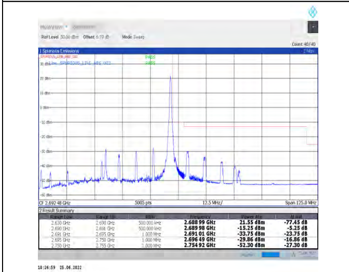
1-N41-PC2-30-60-H-5-CP-QPSK-Edge_1RB_Right-1@161-Ant1-PASS-see graph
