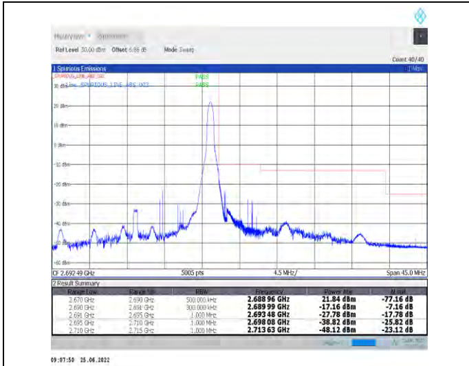
1-N41-PC2-30-20-H-2-DFT-PI2BPSK-Edge_1RB_Right-t-1@50-Ant1-PASS-see graph
