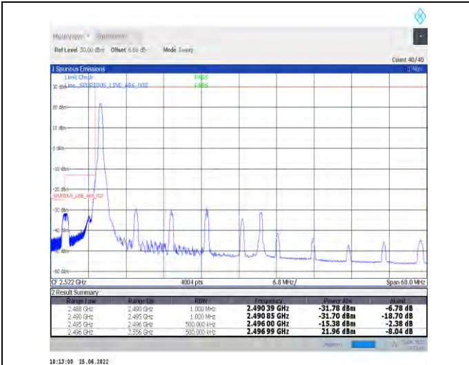
1-N41-PC2-30-60-L-1-DFT-PI2BPSK-Edge_1RB_Left-1@0-Ant1-PASS-see graph
