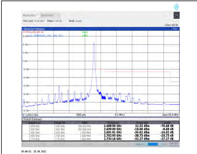
1-N41-PC2-30-40-H-2-DFT-PI2BPSK-Edge_1RB_Righ t-1@105-Ant1-PASS-see graph
