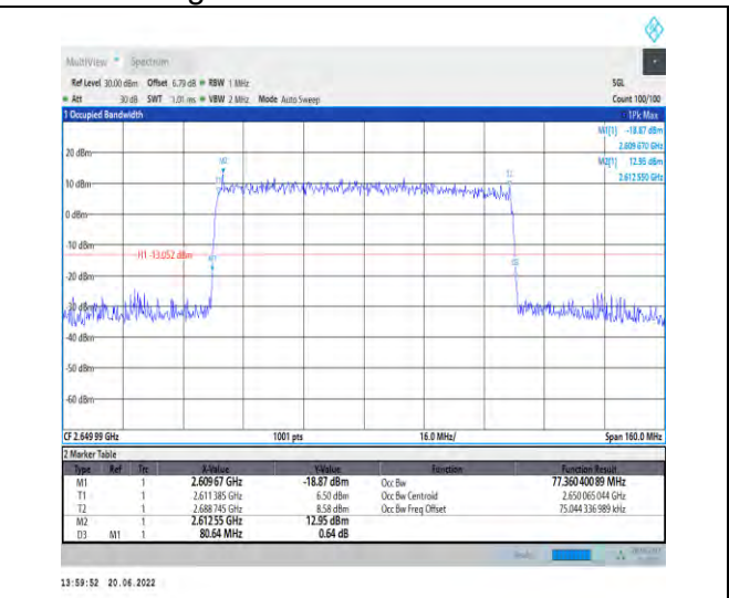
1-N41-PC2-30-80-H-9-CP-256QAM-Outer_Full-217 @0-Ant1-77.36-80.640-≤80-PASS
