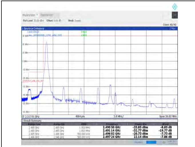
1-N41-PC2-30-50-L-1-DFT-PI2BPSK-Edge_1RB_Left-1@0-Ant1-PASS-see graph
