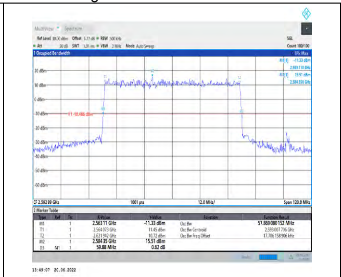
1-N41-PC2-30-60-M-1-DFT-QPSK-Outer_Full-162 @0-Ant1-57.869-59.880-≤60-PASS
