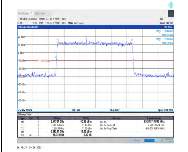
1-N41-PC2-30-90-M-4-DFT-64QAM-Outer_Full-240 @0-Ant1-85.582-88.740-≤90-PASS
