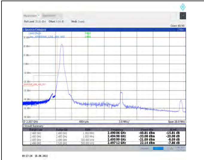
1-N41-PC2-30-30-L-1-DFT-PI2BPSK-Edge_1RB_Left-1@0-Ant1-PASS-see graph
