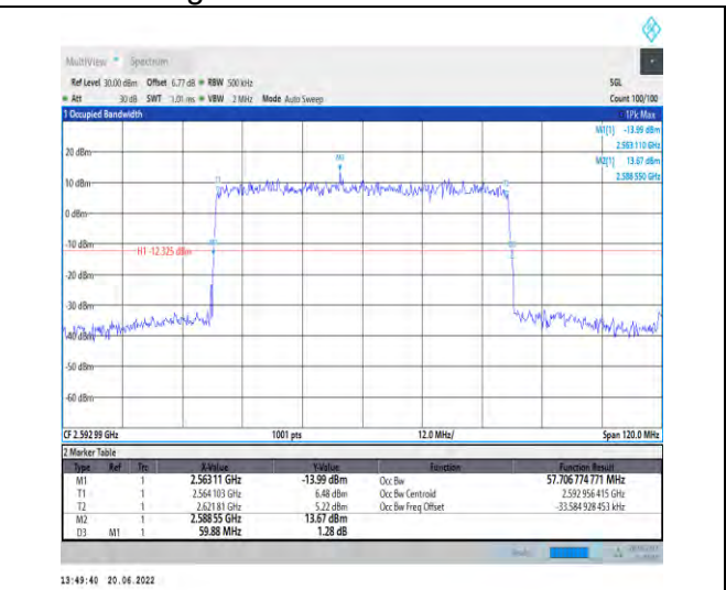
1-N41-PC2-30-60-M-5-DFT-256QAM-Outer_Full-162 @0-Ant1-57.707-59.880-≤60-PASS
