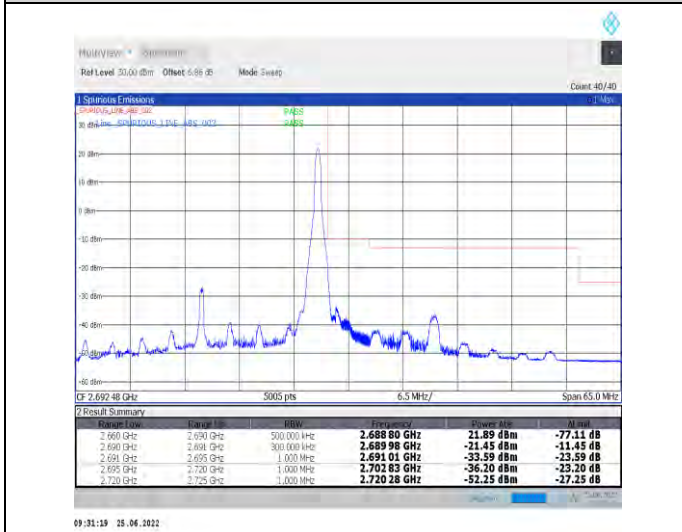
1-N41-PC2-30-30-H-5-CP-QPSK-Edge_1RB_Right-1@77-Ant1-PASS-see graph
