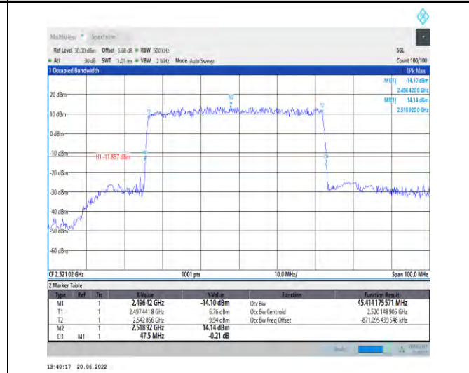
1-N41-PC2-30-50-L-3-DFT-16QAM-Outer_Full-128 @0-Ant1-45.414-47.500-≤50-PASS
