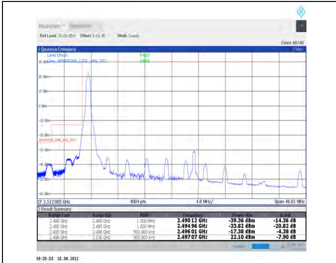
1-N41-PC2-30-40-L-1-DFT-PI2BPSK-Edge_1RB_Left-1@0-Ant1-PASS-see graph
