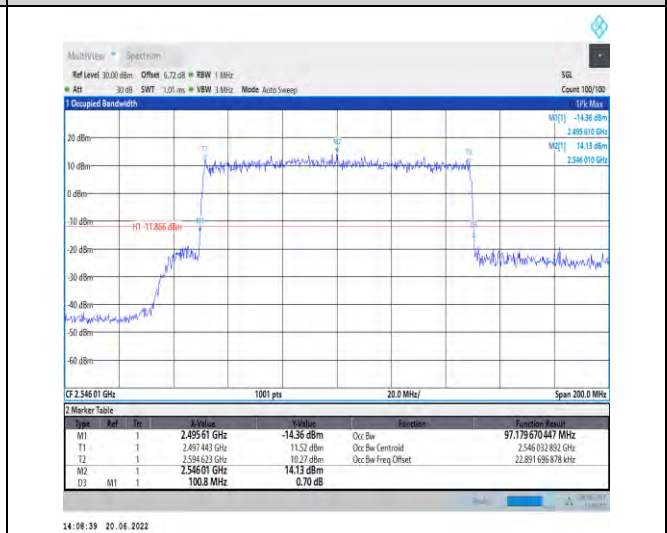
1-N41-PC2-30-100-L-7-CP-16QAM-Outer_Full-273 @0-Ant1-97.18-100.800-≤100-PASS
