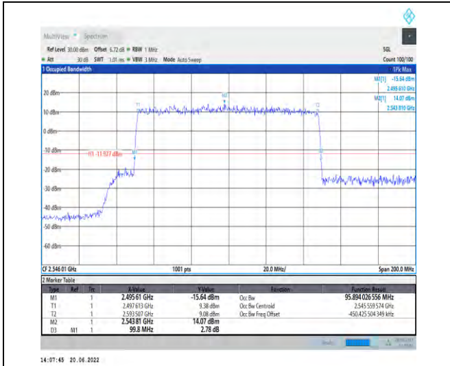
1-N41-PC2-30-100-L-4-DFT-64QAM-Outer_Full-270 @0-Ant1-95.894-99.800-≤100-PASS
