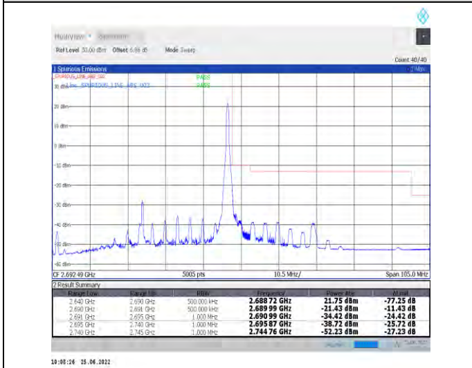
1-N41-PC2-30-50-H-5-CP-QPSK-Edge_1RB_Right-1@132-Ant1-PASS-see graph
