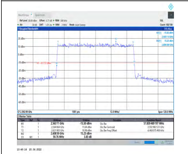
1-N41-PC2-30-60-M-2-DFT-PI2BPSK-Outer_Full-162 @0-Ant1-57.839-59.760-≤60-PASS
