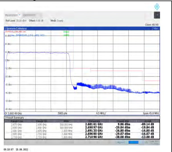
1-N41-PC2-30-20-H-3-DFT-PI2BPSK-Outer_Full-50@0-Ant1-PASS-see graph
