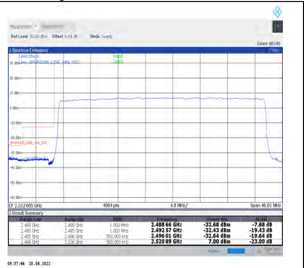
1-N41-PC2-30-40-L-3-DFT-PI2BPSK-Outer_Full-100@0-Ant1-PASS-see graph
