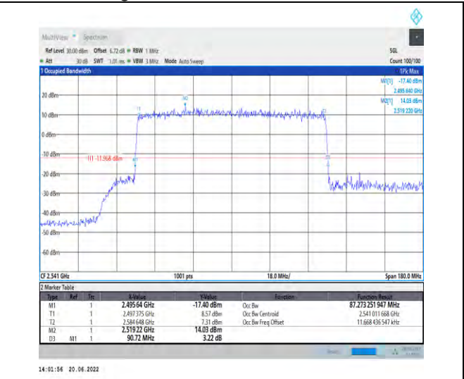
1-N41-PC2-30-90-L-8-CP-64QAM-Outer_Full-245@ 0-Ant1-87.273-90.720-≤90-PASS
