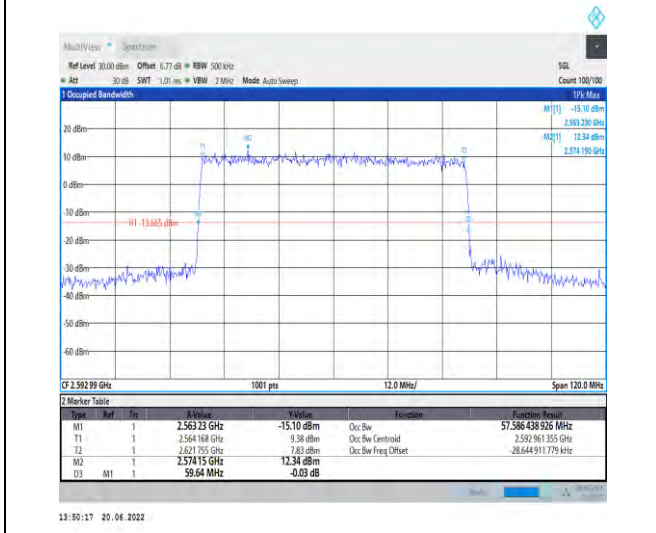
1-N41-PC2-30-60-M-6-CP-QPSK-Outer_Full-162@0 -Ant1-57.586-59.640-≤60-PASS
