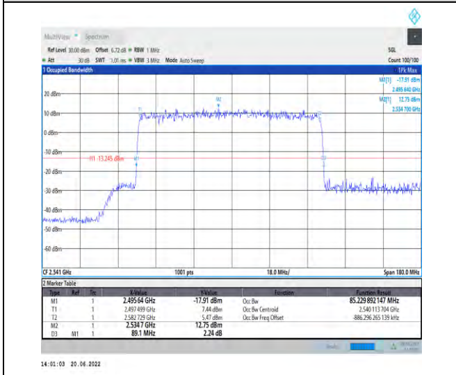
1-N41-PC2-30-90-L-5-DFT-256QAM-Outer_Full-240 @0-Ant1-85.23-89.100-≤90-PASS
