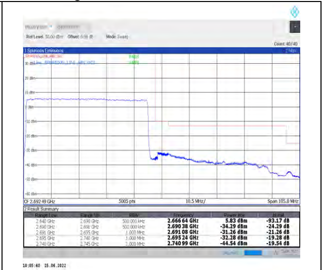
1-N41-PC2-30-50-H-3-DFT-PI2BPSK-Outer_Full-128@0-Ant1-PASS-see graph
