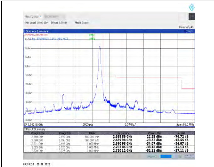
1-N41-PC2-30-30-H-2-DFT-PI2BPSK-Edge_1RB_Right-t1@77-Ant1-PASS-see graph
