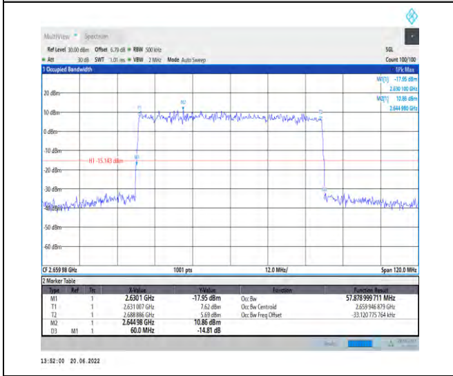
1-N41-PC2-30-60-H-5-DFT-256QAM-Outer_Full-162 @0-Ant1-57.879-60.000-≤60-PASS
