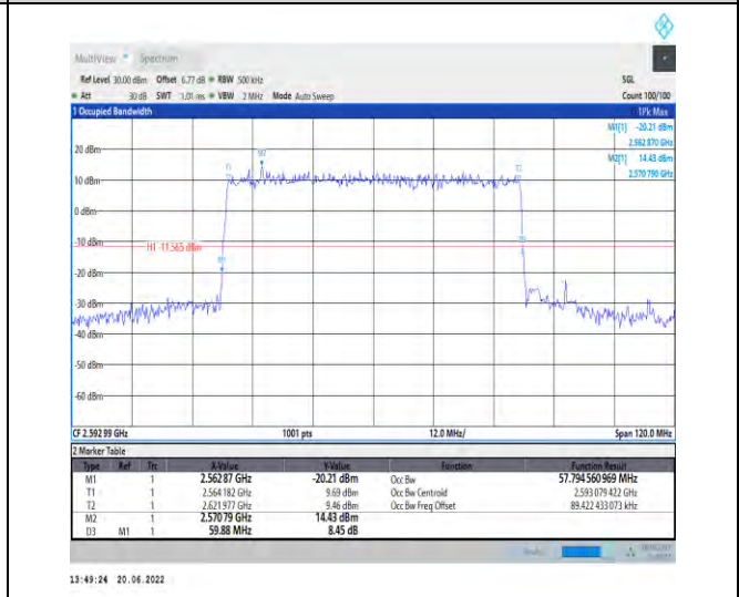
1-N41-PC2-30-60-M-3-DFT-16QAM-Outer_Full-162 @0-Ant1-57.795-59.880-≤60-PASS
