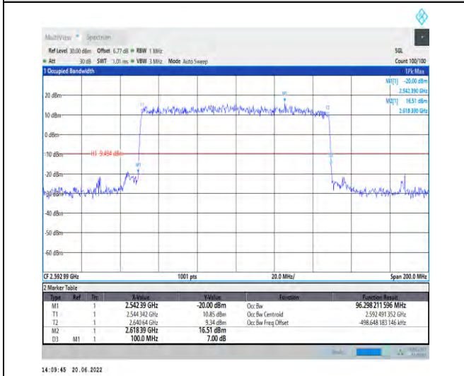
1-N41-PC2-30-100-M-1-DFT-QPSK-Outer_Full-270 @0-Ant1-96.298-100.000-≤100-PASS
