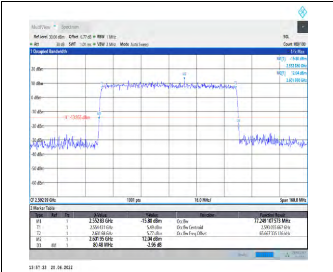
1-N41-PC2-30-80-M-9-CP-256QAM-Outer_Full-217 @0-Ant1-77.249-80.480-<=80-PASS
