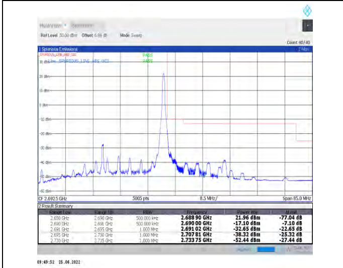
1-N41-PC2-30-40-H-5-CP-QPSK-Edge_1RB_Righ t-1@105-Ant1-PASS-see graph
