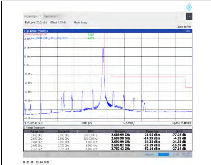
1-N41-PC2-30-60-H-2-DFT-PI2BPSK-Edge_1RB_Right-t1@161-Ant1-PASS-see graph
