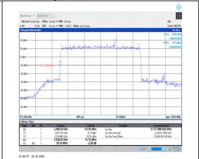
1-N41-PC2-30-60-L-2-DFT-PI2BPSK-Outer_Full-162 @0-Ant1-57.578-59.760-≤60-PASS
