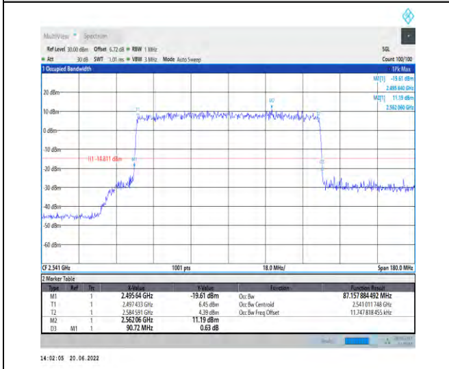
1-N41-PC2-30-90-L-9-CP-256QAM-Outer_Full-245 @0-Ant1-87.158-90.720-≤90-PASS
