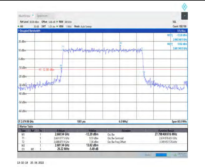
1-N41-PC2-30-30-H-7-CP-16QAM-Outer_Full-78@0 -Ant1-27.798-29.220-≤30-PASS
