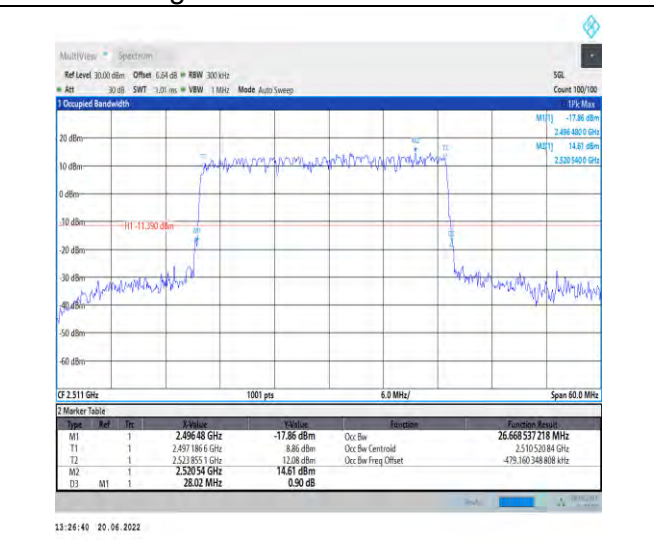
1-N41-PC2-30-30-L-3-DFT-16QAM-Outer_Full-75 @0-Ant1-26.669-28.020-≤30-PASS
