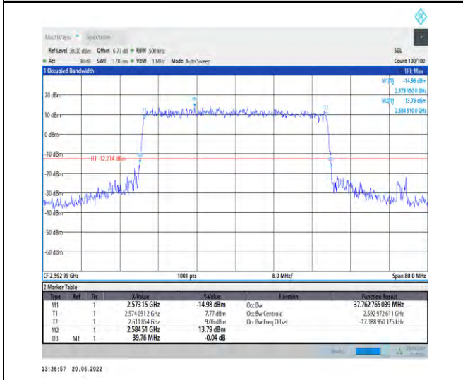
1-N41-PC2-30-40-M-8-CP-64QAM-Outer_Full-106@0 -Ant1-37.763-39.760-≤40-PASS
