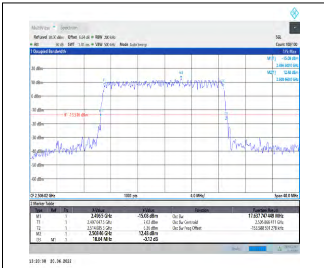
1-N41-PC2-30-20-L-5-DFT-256QAM-Outer_Full-50 @0-Ant1-17.638-18.640-≤20-PASS
