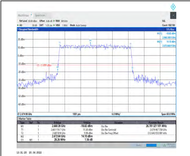
1-N41-PC2-30-30-H-4-DFT-64QAM-Outer_Full-75@ 0-Ant1-26.701-28.260-≤30-PASS
