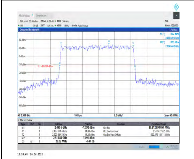
1-N41-PC2-30-30-L-4-DFT-64QAM-Outer_Full-75 @0-Ant1-26.813-28.020-≤30-PASS
