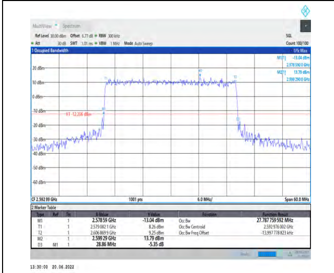
1-N41-PC2-30-30-M-7-CP-16QAM-Outer_Full-78@0-Ant1-27.788-28.860-≤30-PASS
