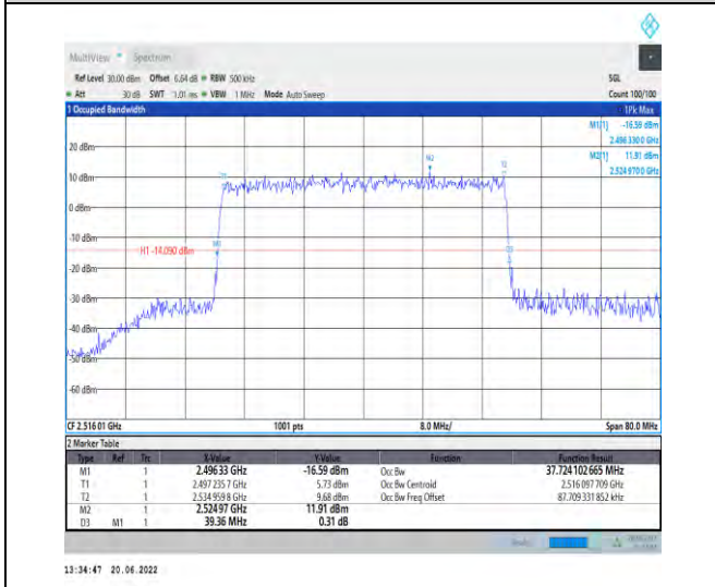
1-N41-PC2-30-40-L-9-CP-256QAM-Outer_Full-106 @0-Ant1-37.724-39.360-≤40-PASS
