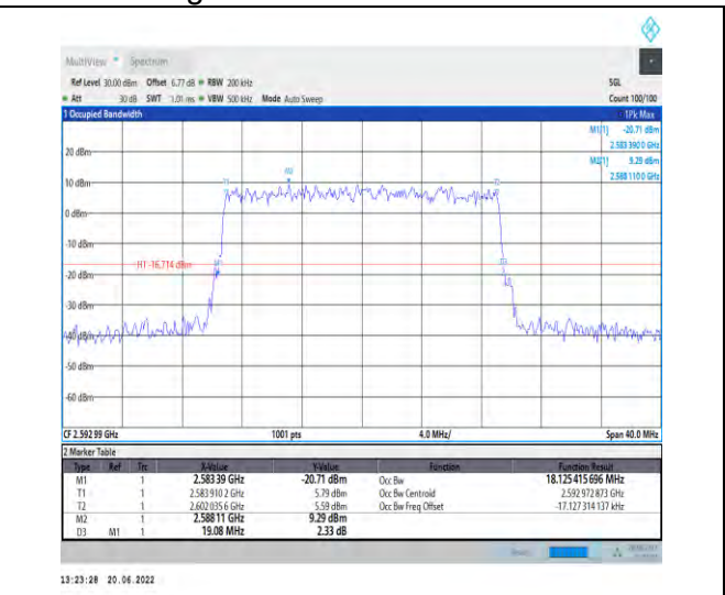
1-N41-PC2-30-20-M-9-CP-256QAM-Outer_Full-51@0 -Ant1-18.125-19.080-≤20-PASS
