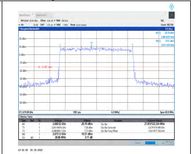
1-N41-PC2-30-30-H-9-CP-256QAM-Outer_Full-78@0 -Ant1-27.82-28.860-≤30-PASS
