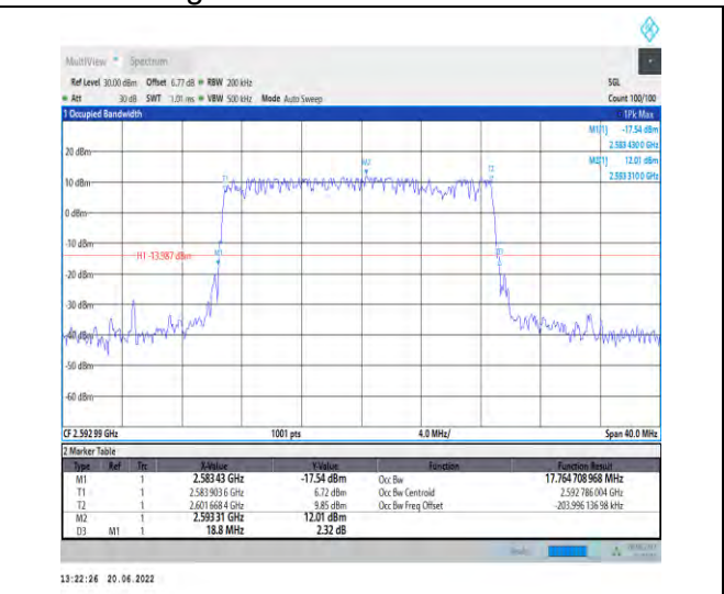
1-N41-PC2-30-20-M-5-DFT-256QAM-Outer_Full-50 @0-Ant1-17.765-18.800-≤20-PASS
