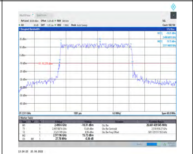
1-N41-PC2-30-30-L-1-DFT-QPSK-Outer_Full-75@0 -Ant1-26.661-27.780-≤30-PASS
