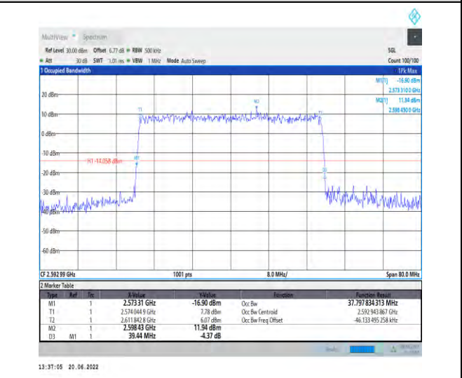
1-N41-PC2-30-40-M-9-CP-256QAM-Outer_Full-106@0 -Ant1-37.798-39.440-≤40-PASS
