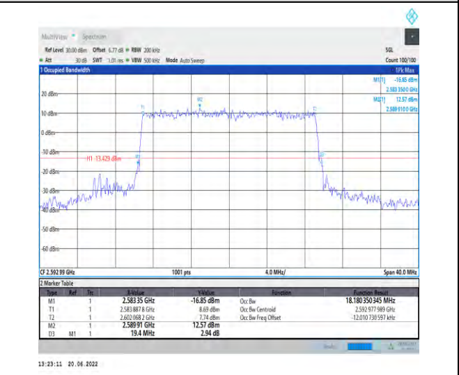
1-N41-PC2-30-20-M-7-CP-16QAM-Outer_Full-51@0- Ant1-18.18-19.400-≤20-PASS
