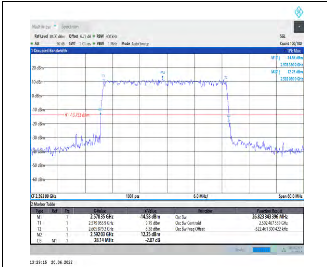
1-N41-PC2-30-30-M-5-DFT-256QAM-Outer_Full-75 @0-Ant1-26.823-28.140-≤30-PASS
