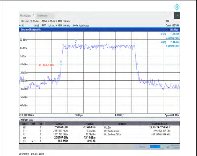
1-N41-PC2-30-20-M-3-DFT-16QAM-Outer_Full-50@ 0-Ant1-17.792-18.800-≤20-PASS
