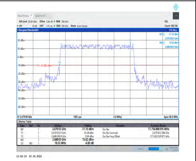
1-N41-PC2-30-20-H-2-DFT-PI2BPSK-Outer_Full-50@0 -Ant1-17.757-18.520-≤20-PASS
