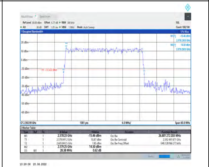
1-N41-PC2-30-30-M-4-DFT-64QAM-Outer_Full-75@0 0-Ant1-26.801-28.380-<=30-PASS
