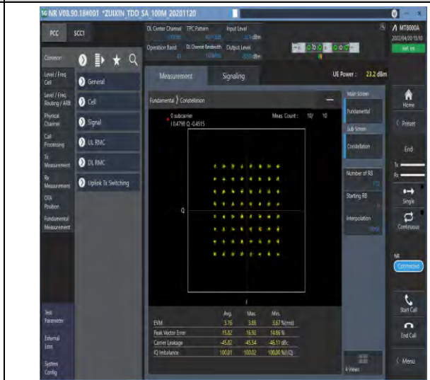
1-N41--30-100-M-8-CP-64QAM-Outer_Full-273@0-Ant1-see graph-PASS
