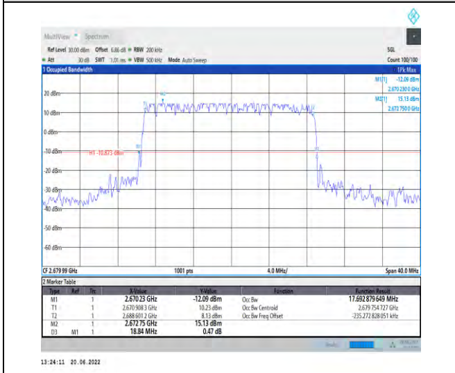
1-N41-PC2-30-20-H-1-DFT-QPSK-Outer_Full-50@0 -Ant1-17.693-18.840-≤20-PASS
