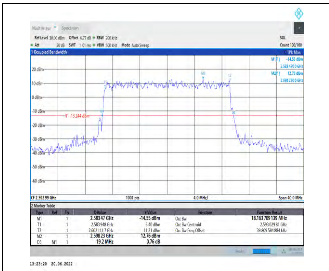
1-N41-PC2-30-20-M-8-CP-64QAM-Outer_Full-51@0 -Ant1-18.164-19.200-≤20-PASS
