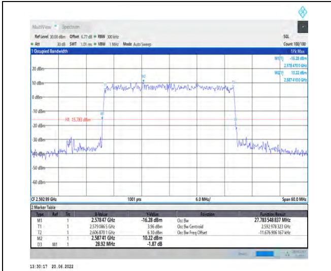
1-N41-PC2-30-30-M-9-CP-256QAM-Outer_Full-78@ 0-Ant1-27.784-28.920-≤30-PASS
