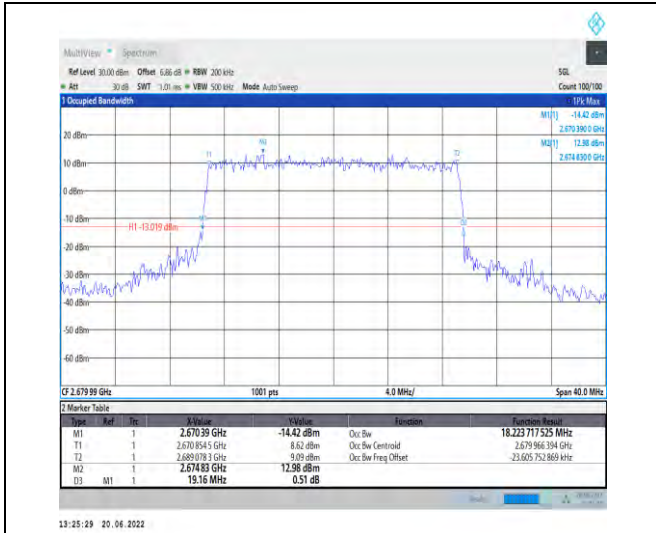
1-N41-PC2-30-20-H-7-CP-16QAM-Outer_Full-51@0 -Ant1-18.224-19.160-≤20-PASS
