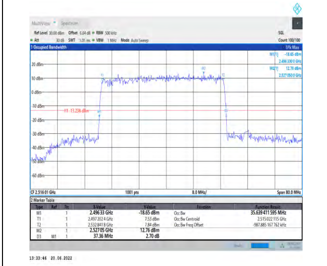
1-N41-PC2-30-40-L-5-DFT-256QAM-Outer_Full-100 @0-Ant1-35.639-37.360-≤40-PASS
