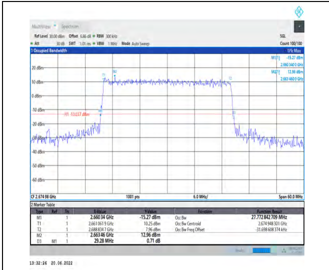
1-N41-PC2-30-30-H-8-CP-64QAM-Outer_Full-78@0 -Ant1-27.773-29.280-≤30-PASS
