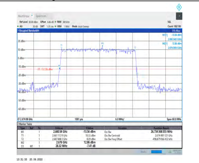
1-N41-PC2-30-30-H-5-DFT-256QAM-Outer_Full-75 @0-Ant1-26.734-28.320-≤30-PASS
