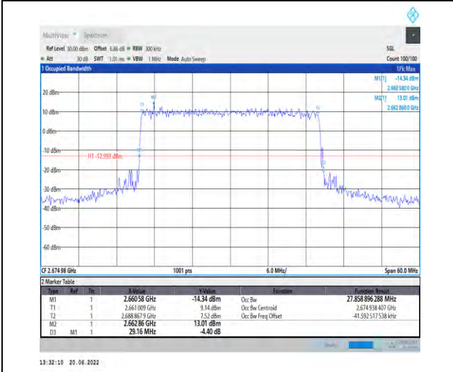
1-N41-PC2-30-30-H-6-CP-QPSK-Outer_Full-78@0- Ant1-27.859-29.160-≤30-PASS
