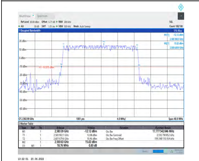
1-N41-PC2-30-20-M-2-DFT-PI2BPSK-Outer_Full-50@ 0-Ant1-17.778-18.760-≤20-PASS
