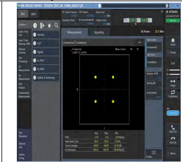
1-N41--30-100-M-6-CP-QPSK-Outer_Full-273@0-Ant1-see graph-PASS
