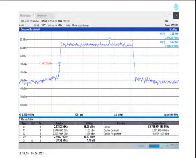
1-N41-PC2-30-40-M-1-DFT-QPSK-Outer_Full-100@ 0-Ant1-35.754-37.520-≤40-PASS
