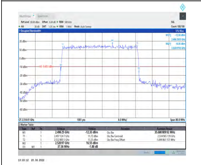
1-N41-PC2-30-40-L-1-DFT-QPSK-Outer_Full-100@0 -Ant1-35.681-37.360-≤40-PASS
