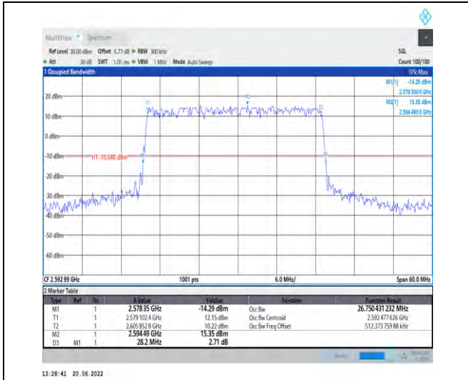
1-N41-PC2-30-30-M-1-DFT-QPSK-Outer_Full-75@0 -Ant1-26.75-28.200-<=30-PASS
