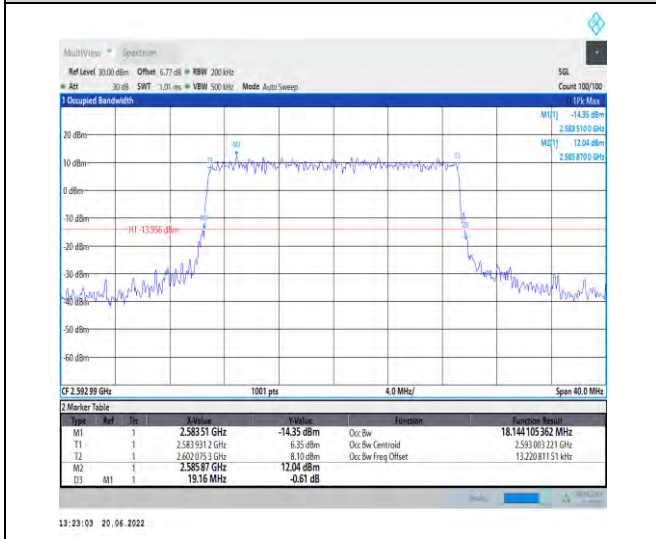
1-N41-PC2-30-20-M-6-CP-QPSK-Outer_Full-51@0- Ant1-18.144-19.160-≤20-PASS
