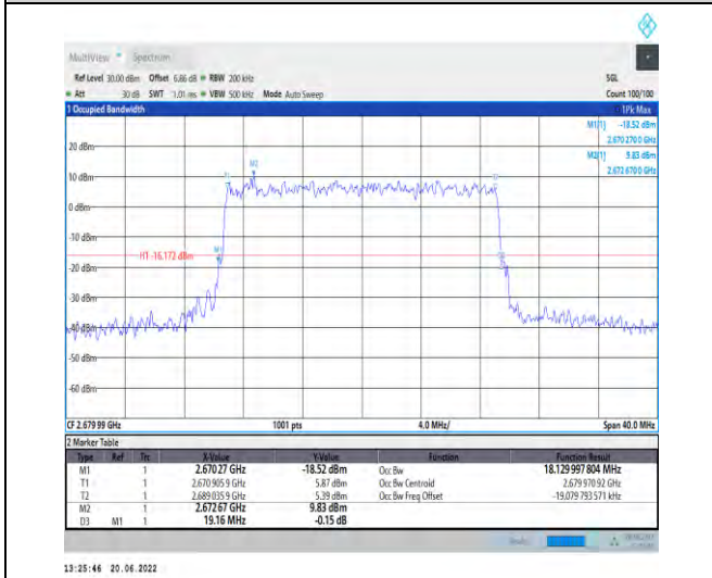
1-N41-PC2-30-20-H-9-CP-256QAM-Outer_Full-51@0 -Ant1-18.13-19.160-≤20-PASS
