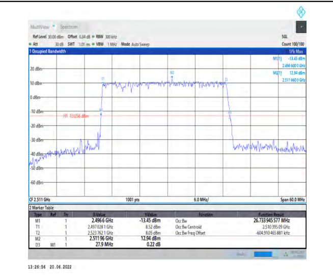
1-N41-PC2-30-30-L-5-DFT-256QAM-Outer_Full-75 @0-Ant1-26.734-27.900-≤30-PASS
