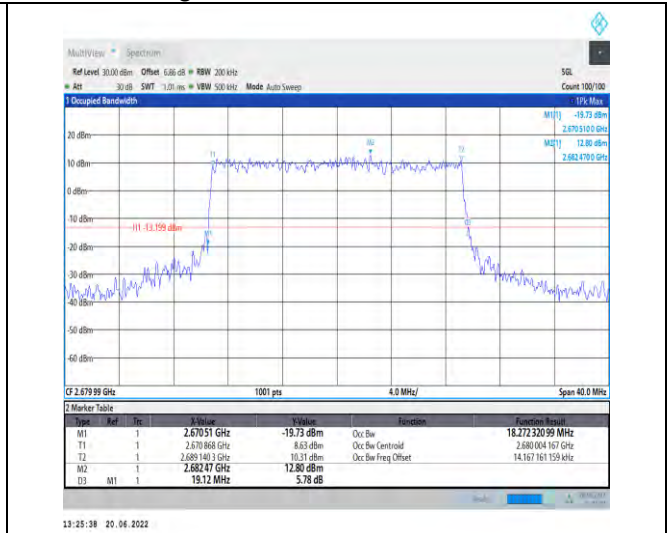
1-N41-PC2-30-20-H-8-CP-64QAM-Outer_Full-51@0 -Ant1-18.272-19.120-≤20-PASS
