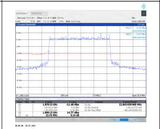
1-N25-PC3-15-25-M-3-DFT-16QAM-Outer_Full-128 @0-Ant1-22.844-23.750-≤25-PASS
