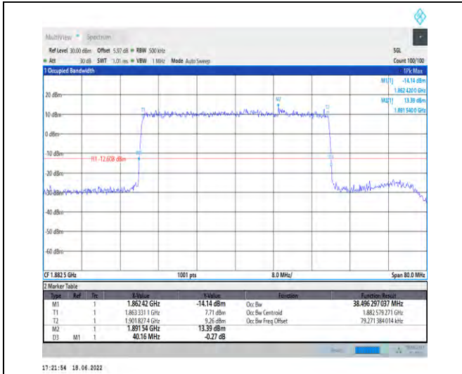
1-N25-PC3-15-40-M-6-CP-QPSK-Outer_Full-216@0 -Ant1-38.496-40.160-≤40-PASS
