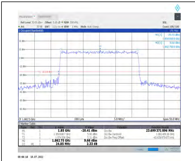
1-N25-PC3-15-25-L-9-CP-256QAM-Outer_Full-133 @0-Ant1-23.699-24.850-≤25-PASS
