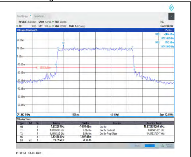
1-N25-PC3-15-20-M-8-CP-64QAM-Outer_Full-106@ 0-Ant1-18.873-19.720-≤20-PASS
