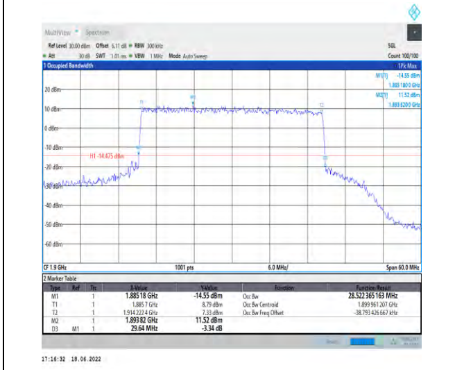
1-N25-PC3-15-30-H-6-CP-QPSK-Outer_Full-160@0 -Ant1-28.522-29.640-≤30-PASS
