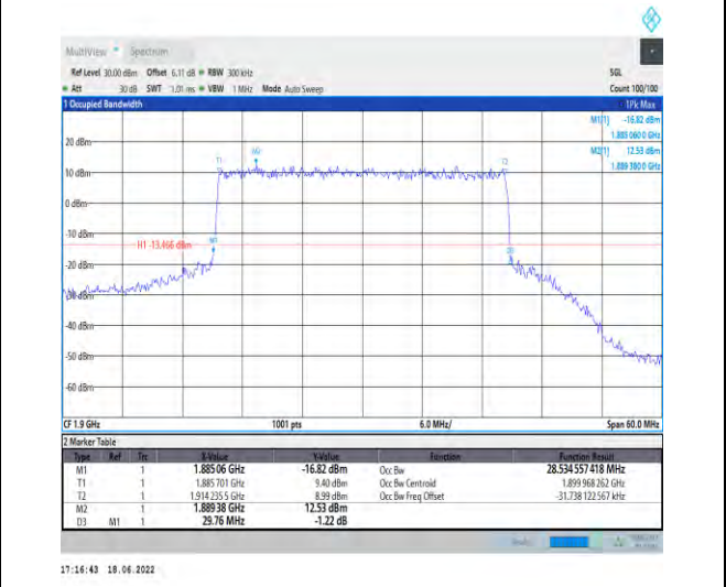
1-N25-PC3-15-30-H-7-CP-16QAM-Outer_Full-160@0 -Ant1-28.535-29.760-≤30-PASS
