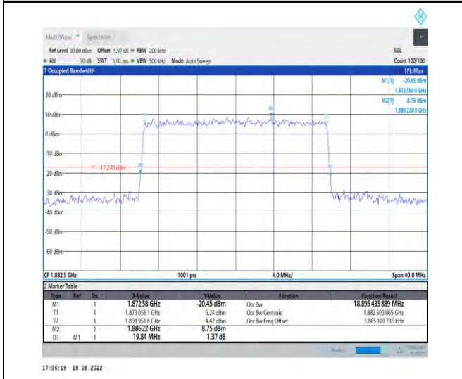
1-N25-PC3-15-20-M-9-CP-256QAM-Outer_Full-106 @0-Ant1-18.895-19.840-≤20-PASS
