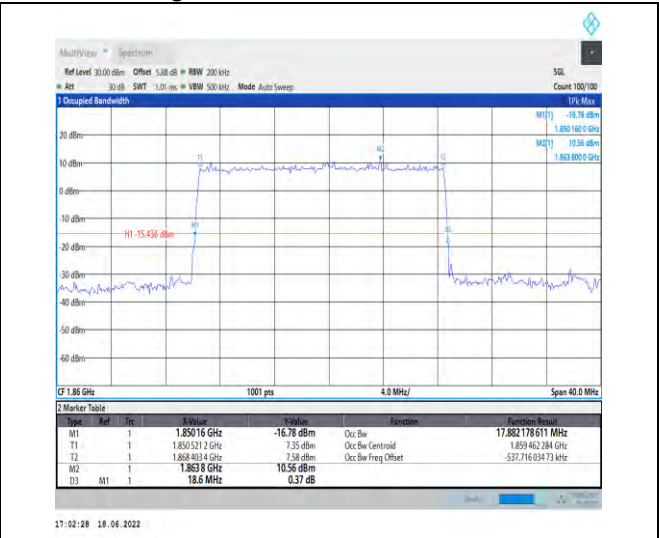
1-N25-PC3-15-20-L-5-DFT-256QAM-Outer_Full-100 @0-Ant1-17.882-18.600-≤20-PASS
