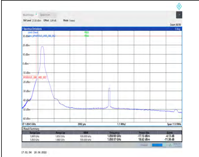
1-N25--15-10-L-4-CP-QPSK-Edge_1RB_Left-1@0-Ant1-seegraph-PASS-see graph
