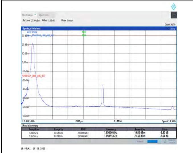
1-N25--15-20-L-4-CP-QPSK-Edge_1RB_Left-1@0-Ant1-seegraph-PASS-see graph
