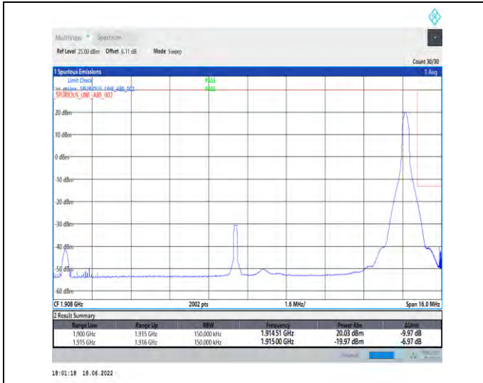
1-N25--15-15-H-2-DFT-PI2BPSK-Edge_1RB_Right-1@78-Ant1-seegraph-PASS-see graph
