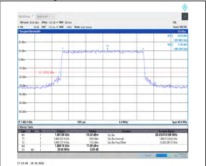
1-N25-PC3-15-30-M-6-CP-QPSK-Outer_Full-160@0 -Ant1-28.418-29.640-≤30-PASS
