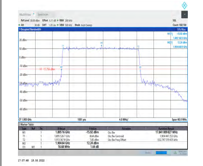
1-N25-PC3-15-20-H-4-DFT-64QAM-Outer_Full-100@0-Ant1-17.841-18.680-≤20-PASS
