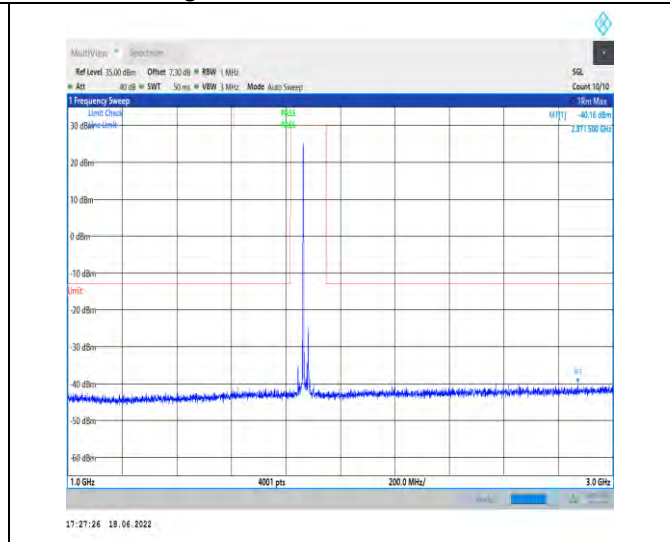
1-N25--15-40-M-1-DFT-PI2BPSK-Inner_1RB_Left-1 @1-1000-3000-Ant1--40.16--13-PASS
