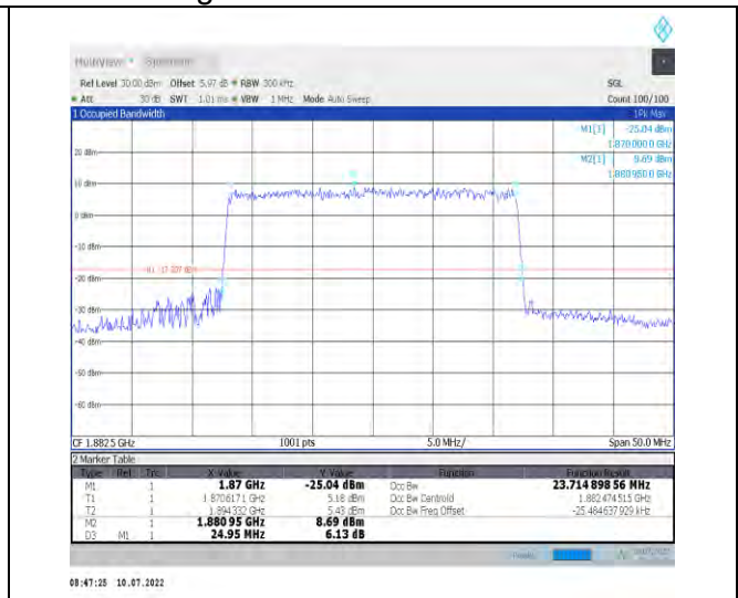
1-N25-PC3-15-25-M-9-CP-256QAM-Outer_Full-133 @0-Ant1-23.715-24.950-≤25-PASS
