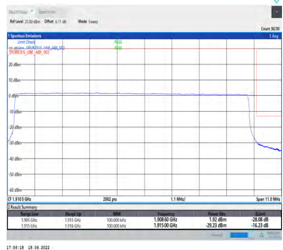
1-N25--15-10-H-6-CP-QPSK-Outer_Full-52@0-Ant 1-seegraph-PASS-see graph
