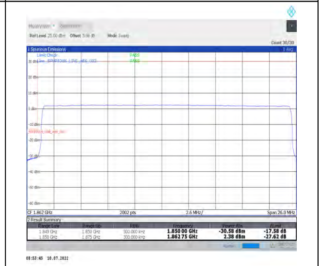
1-N25-PC3-15-25-L-6-CP-QPSK-Outer_Full-133@0-Ant1-seegraph-PASS-see graph
