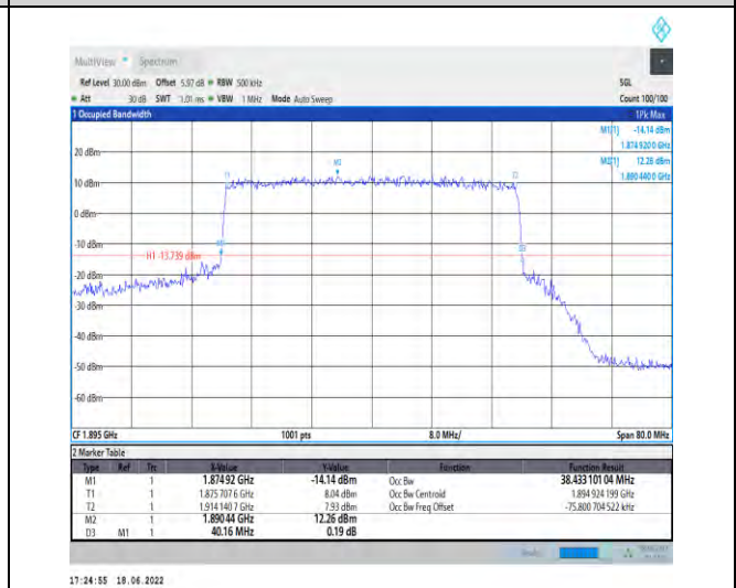
1-N25-PC3-15-40-H-8-CP-64QAM-Outer_Full-216 @0-Ant1-38.433-40.160-≤40-PASS
