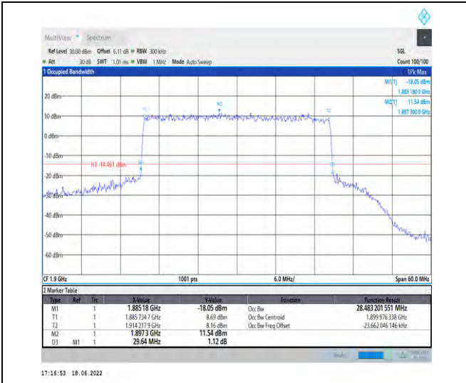
1-N25-PC3-15-30-H-8-CP-64QAM-Outer_Full-160@ 0-Ant1-28.483-29.640-≤30-PASS
