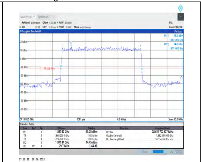
1-N25-PC3-15-30-M-2-DFT-PI2BPSK-Outer_Full-160@0-Ant1-28.612-29.700-≤30-PASS
