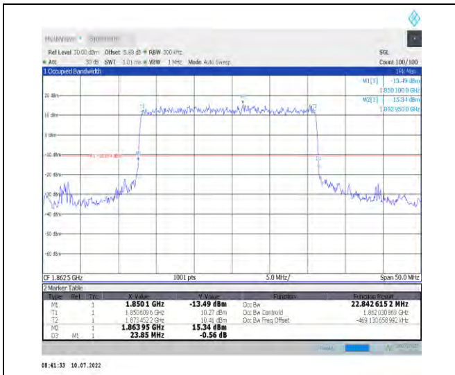
1-N25-PC3-15-25-L-1-DFT-QPSK-Outer_Full-128@ @0-Ant1-22.843-23.850-≤25-PASS
