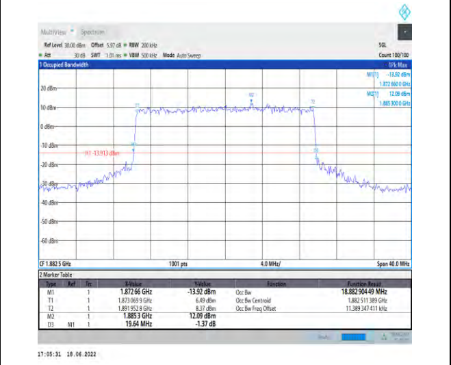
1-N25-PC3-15-20-M-6-CP-QPSK-Outer_Full-106@0-Ant1-18.883-19.640-≤20-PASS
