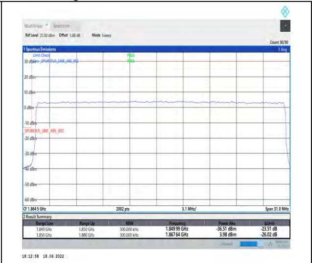
1-N25--15-30-L-3-DFT-PI2BPSK-Outer_Full-160@0-Ant1-seegraph-PASS-see graph
