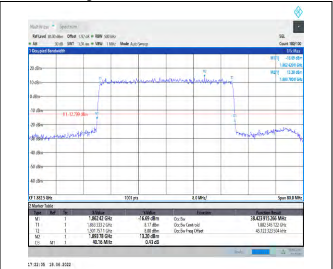
1-N25-PC3-15-40-M-7-CP-16QAM-Outer_Full-216@0 -Ant1-38.424-40.160-≤40-PASS
