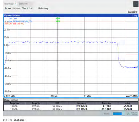
1-N25--15-10-H-3-DFT-PI2BPSK-Outer_Full-50@ 0-Ant1-seegraph-PASS-see graph
