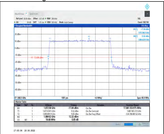
1-N25-PC3-15-20-M-4-DFT-64QAM-Outer_Full-100 @0-Ant1-17.861-18.680-≤20-PASS
