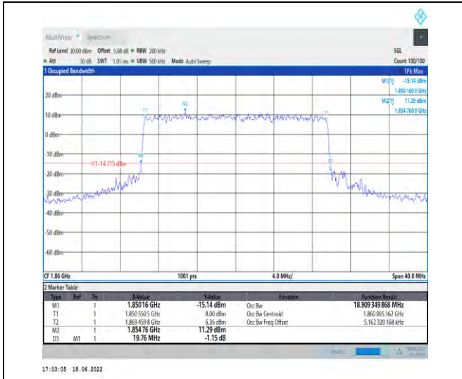
1-N25-PC3-15-20-L-8-CP-64QAM-Outer_Full-106@0-Ant1-18.909-19.760-≤20-PASS
