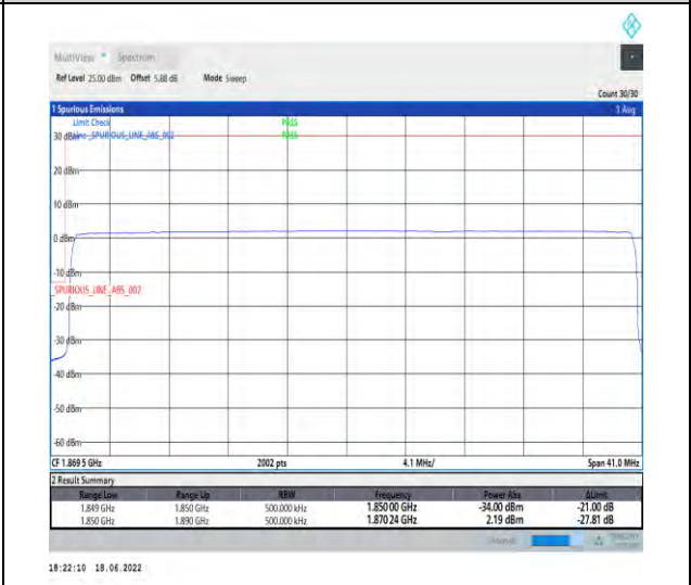
1-N25--15-40-L-6-CP-QPSK-Outer_Full-216@0-Ant1-seegraph-PASS-see graph
