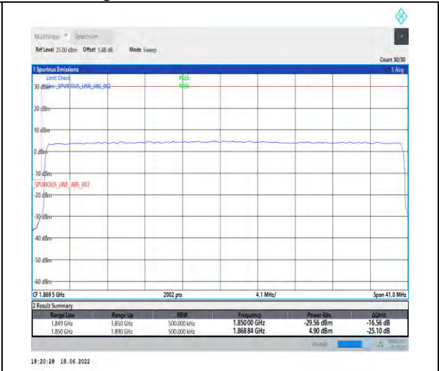
1-N25--15-40-L-3-DFT-PI2BPSK-Outer_Full-216@0-Ant1-seegraph-PASS-see graph
