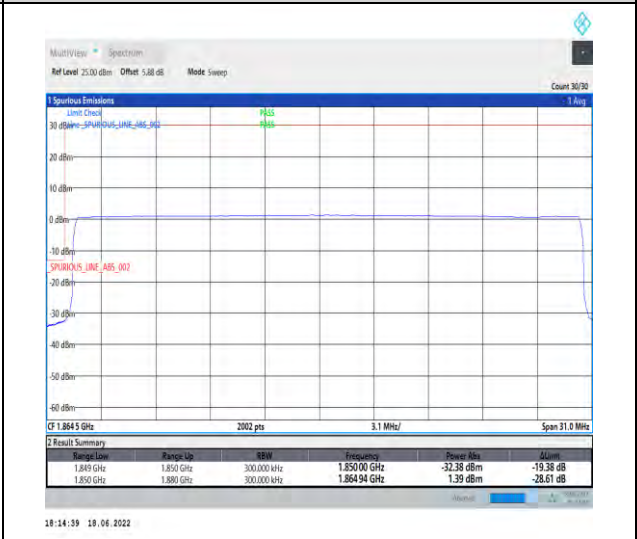
1-N25--15-30-L-6-CP-QPSK-Outer_Full-160@0-Ant1-seegraph-PASS-see graph
