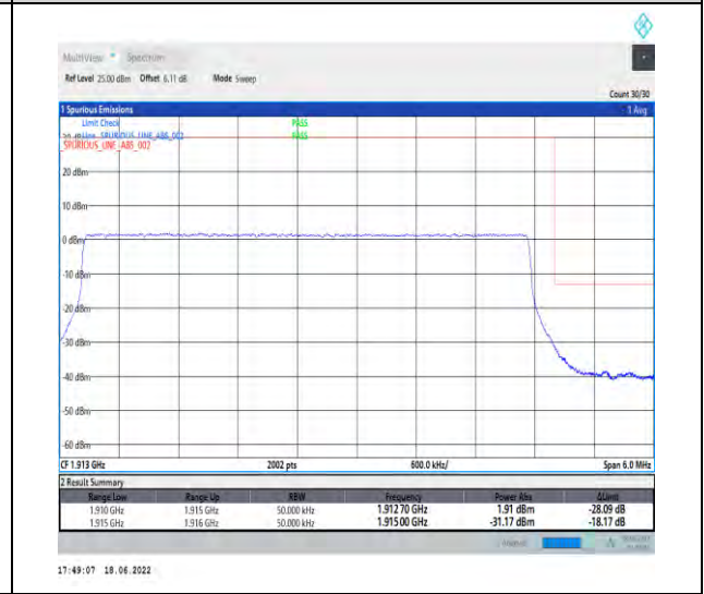
1-N25--15-5-H-6-CP-QPSK-Outer_Full-25@0-Ant1-seegraph-PASS-see graph
