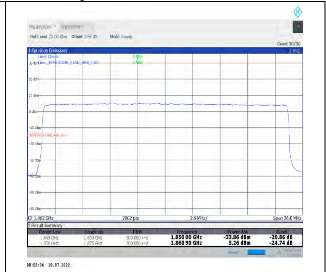
1-N25-PC3-15-25-L-3-DFT-PI2BPSK-Outer_Full-1 28@0-Ant1-seegraph-PASS-see graph
