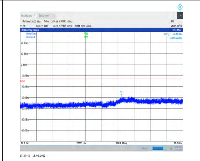
1-N25--15-40-M-1-DFT-PI2BPSK-Inner_1RB_Left-1 @1-12000-20000-Ant1--28.11--13-PASS
