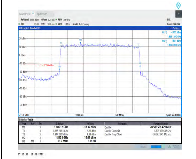
1-N25-PC3-15-30-H-2-DFT-PI2BPSK-Outer_Full-160 @0-Ant1-28.509-29.700-≤30-PASS
