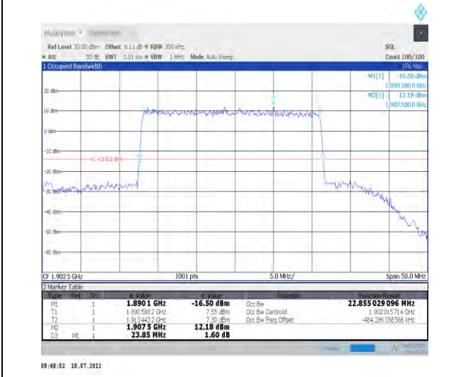
1-N25-PC3-15-25-H-5-DFT-256QAM-Outer_Full-128 @0-Ant1-22.855-23.850-≤25-PASS
