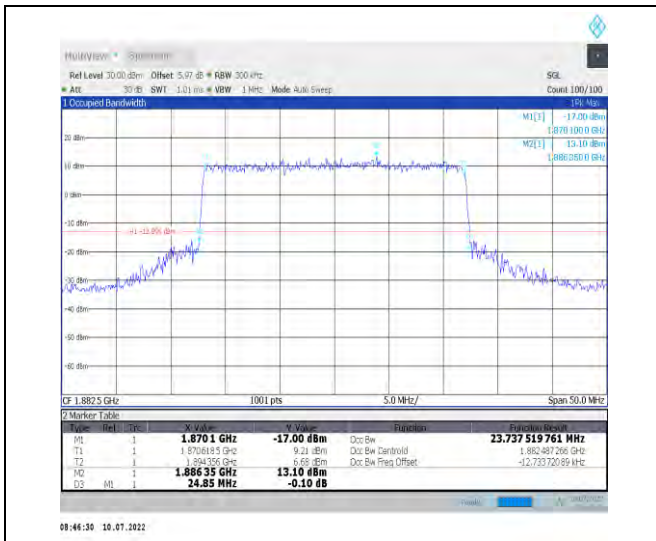
1-N25-PC3-15-25-M-8-CP-64QAM-Outer_Full-133@ 0-Ant1-23.738-24.850-≤25-PASS
