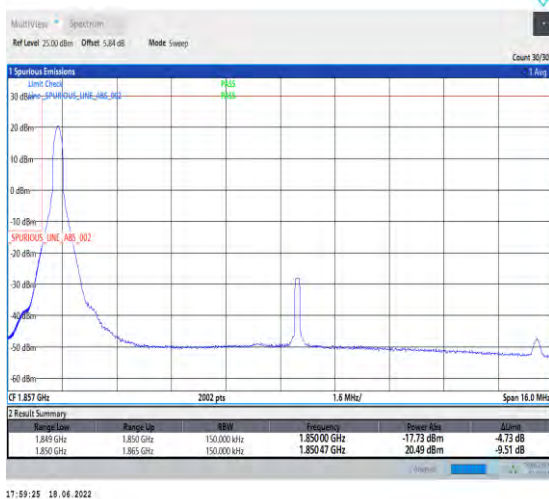
1-N25--15-15-L-4-CP-QPSK-Edge_1RB_Left-1@0-Ant 1-seegraph-PASS-see graph
