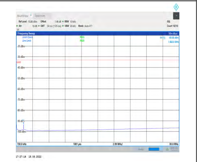
1-N25--15-40-M-1-DFT-PI2BPSK-Inner_1RB_Left-1 @1-0.15-30-Ant1--93.06--33-PASS
