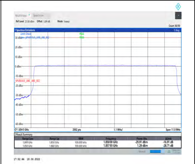
1-N25--15-10-L-6-CP-QPSK-Outer_Full-52@0-Ant1-seegraph-PASS-see graph
