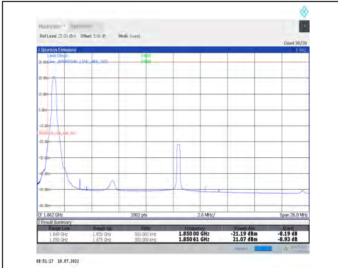
1-N25-PC3-15-25-L-1-DFT-PI2BPSK-Edge_1RB_Left-1@0-Ant1-seegraph-PASS-see graph
