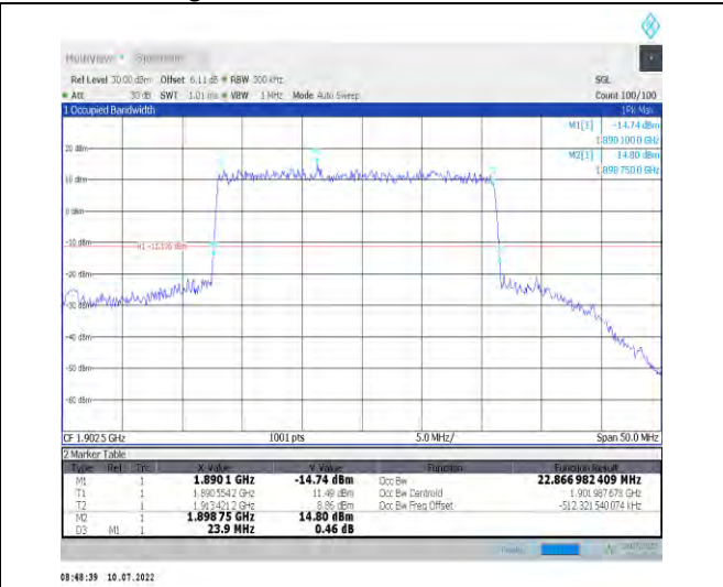
1-N25-PC3-15-25-H-4-DFT-64QAM-Outer_Full-128 @0-Ant1-22.867-23.900-≤25-PASS
