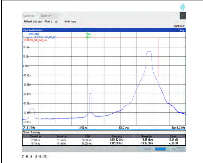
1-N25--15-5-H-5-CP-QPSK-Edge_1RB_Right-1@24-Ant1-seegraph-PASS-see graph
