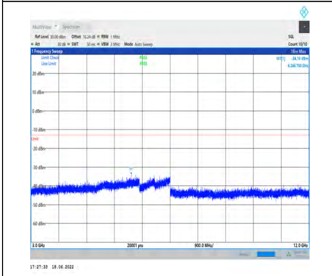
1-N25--15-40-M-1-DFT-PI2BPSK-Inner_1RB_Left-1 @1-3000-12000-Ant1--34.19--13-PASS
