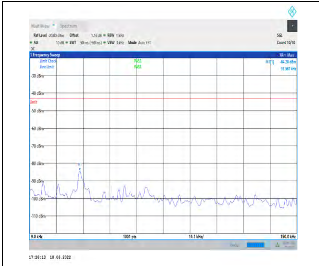
1-N25--15-40-H-1-DFT-PI2BPSK-Inner_1RB_Left-1 @1-0.009-0.15-Ant1--84.28--43-PASS
