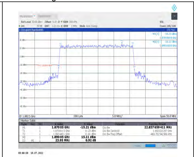
1-N25-PC3-15-25-M-1-DFT-QPSK-Outer_Full-128 @0-Ant1-22.838-23.950-≤25-PASS
