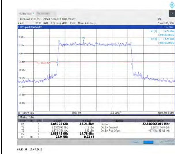
1-N25-PC3-15-25-L-3-DFT-16QAM-Outer_Full-128 @0-Ant1-22.847-23.900-≤25-PASS
