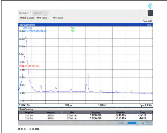
1-N25--15-30-L-4-CP-QPSK-Edge_1RB_Left-1@0-Ant1-seegraph-PASS-see graph
