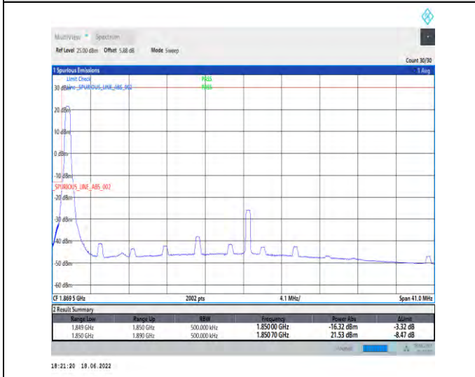
1-N25--15-40-L-4-CP-QPSK-Edge_1RB_Left-1@0-Ant1-seegraph-PASS-see graph
