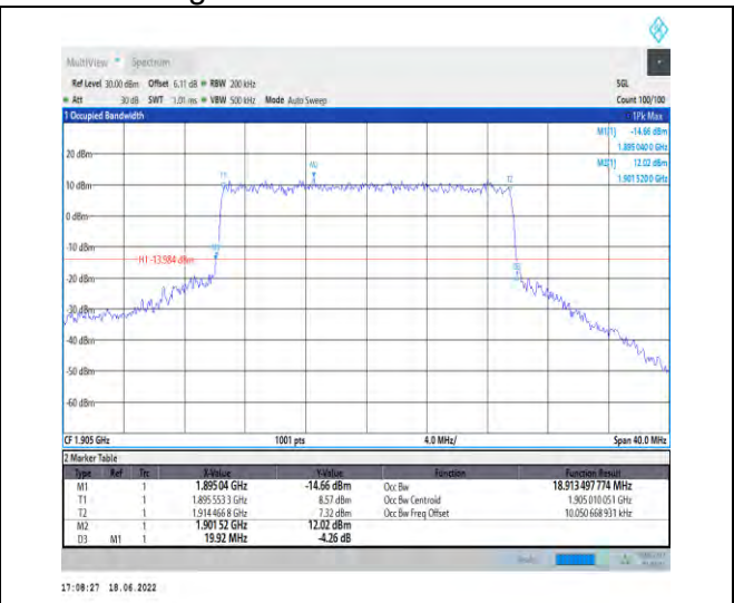
1-N25-PC3-15-20-H-7-CP-16QAM-Outer_Full-106@0 -Ant1-18.913-19.920-≤20-PASS
