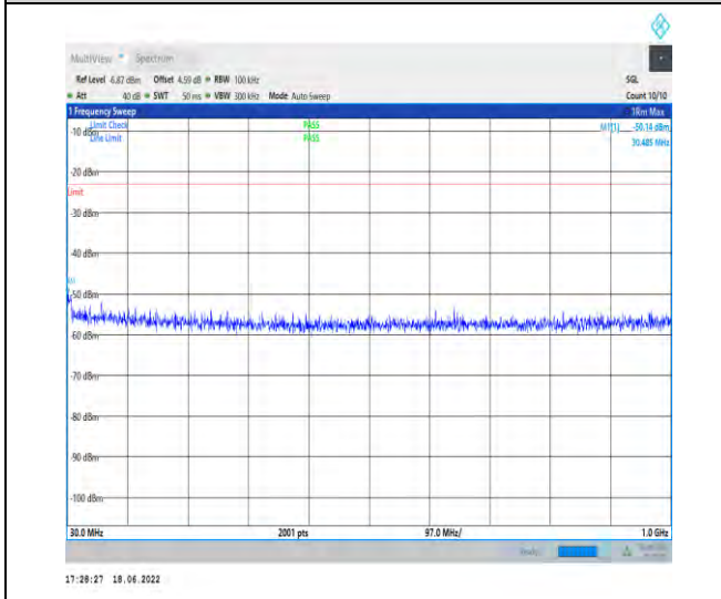
1-N25--15-40-H-1-DFT-PI2BPSK-Inner_1RB_Left-1 @1-30-1000-Ant1--50.14--23-PASS
