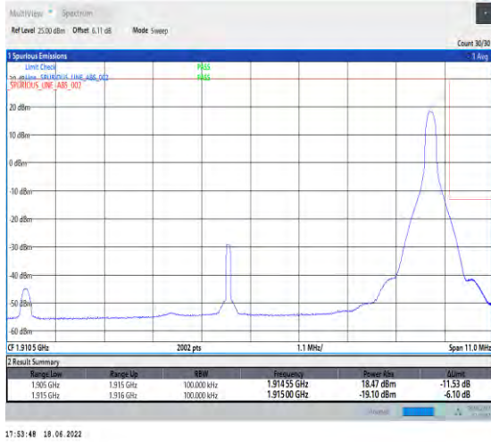
1-N25--15-10-H-2-DFT-PI2BPSK-Edge_1RB_Right-1 @51-Ant1-seegraph-PASS-see graph
