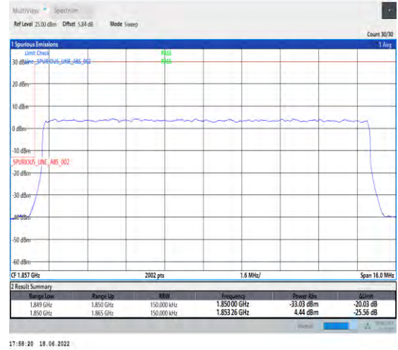
1-N25--15-15-L-3-DFT-PI2BPSK-Outer_Full-75@0 -Ant1-seegraph-PASS-see graph
