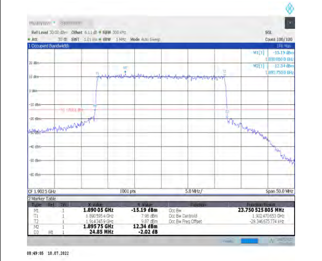
1-N25-PC3-15-25-H-6-CP-QPSK-Outer_Full-133@0-Ant1-23.751-24.850-≤25-PASS
