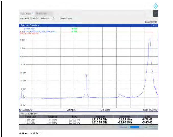
1-N25-PC3-15-25-H-2-DFT-PI2BPSK-Edge_1RB_Right-t-1@132-Ant1-seegraph-PASS-see graph
