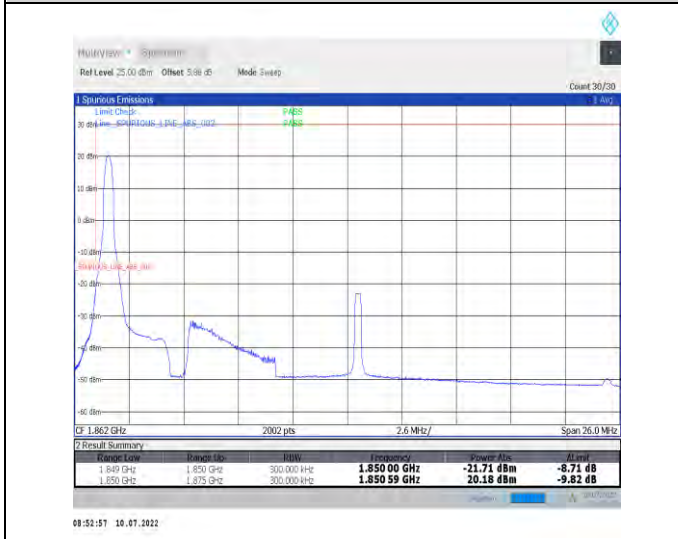
1-N25-PC3-15-25-L-4-CP-QPSK-Edge_1RB_Left-1@0-Ant1-seegraph-PASS-see graph
