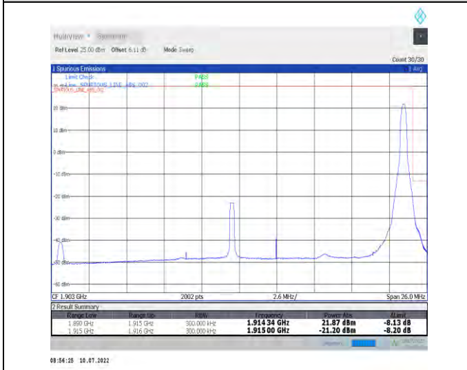
1-N25-PC3-15-25-H-5-CP-QPSK-Edge_1RB_Right-1@132-Ant1-seegraph-PASS-see graph
