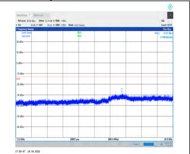
1-N25--15-40-H-1-DFT-PI2BPSK-Inner_1RB_Left-1 @1-12000-20000-Ant1--27.87--13-PASS
