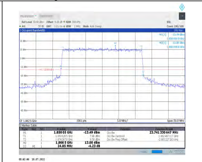
1-N25-PC3-15-25-L-6-CP-QPSK-Outer_Full-133@0-Ant1-23.741-24.850-≤25-PASS
