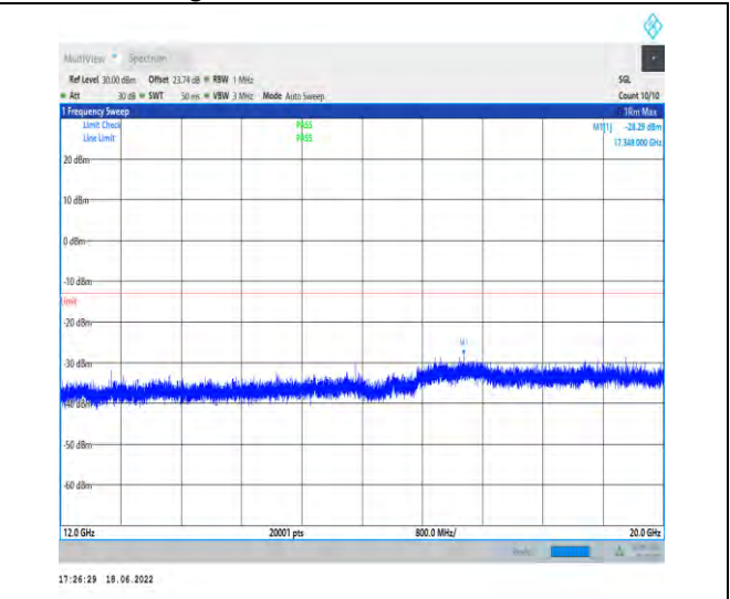
1-N25--15-40-L-1-DFT-PI2BPSK-Inner_1RB_Left-1@ 1-12000-20000-Ant1--28.29--13-PASS
