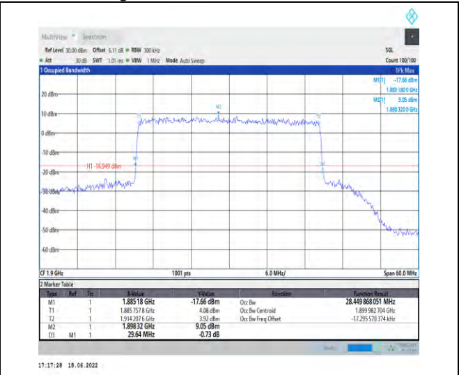
1-N25-PC3-15-30-H-9-CP-256QAM-Outer_Full-160 @0-Ant1-28.45-29.640-≤30-PASS
