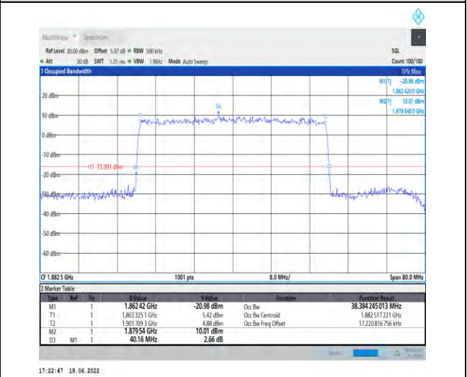
1-N25-PC3-15-40-M-9-CP-256QAM-Outer_Full-216@0 -Ant1-38.384-40.160-≤40-PASS
