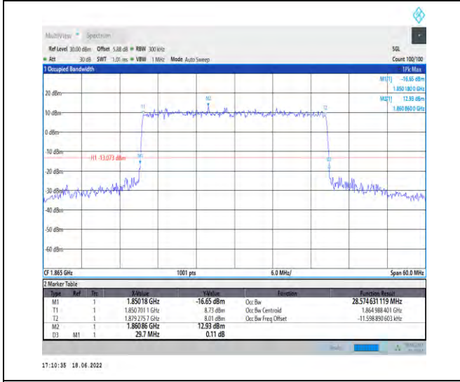
1-N25-PC3-15-30-L-4-DFT-64QAM-Outer_Full-160 @0-Ant1-28.575-29.700-≤30-PASS
