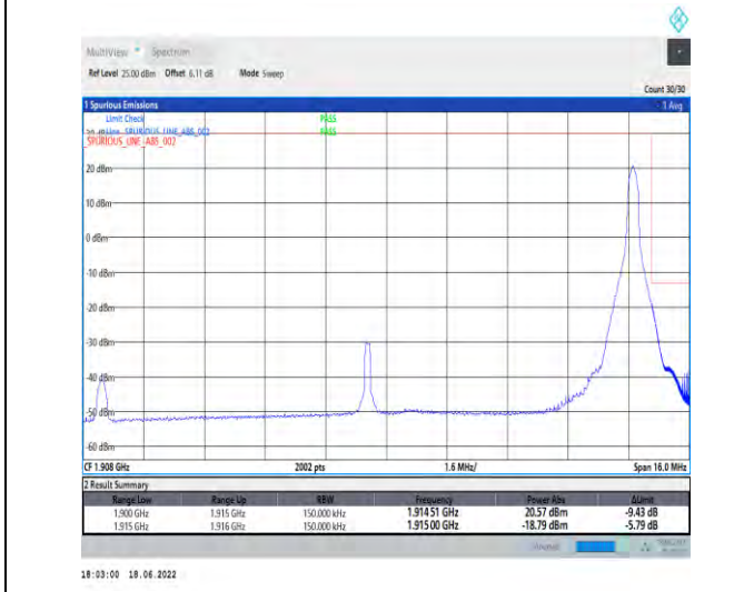
1-N25--15-15-H-5-CP-QPSK-Edge_1RB_Right-1@78-Ant1-seegraph-PASS-see graph
