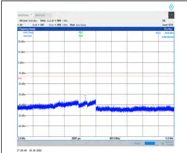
1-N25--15-40-H-1-DFT-PI2BPSK-Inner_1RB_Left-1 @1-3000-12000-Ant1--34.40--13-PASS
