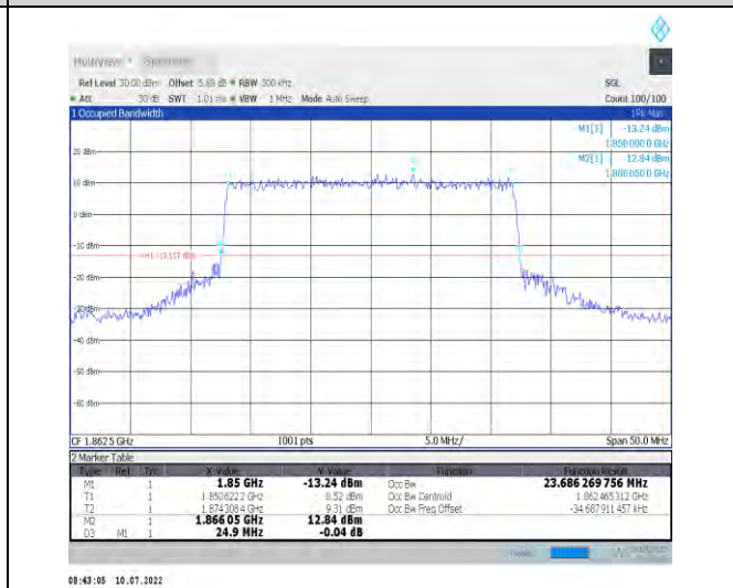
1-N25-PC3-15-25-L-8-CP-64QAM-Outer_Full-133@0-Ant1-23.686-24.900-≤25-PASS
