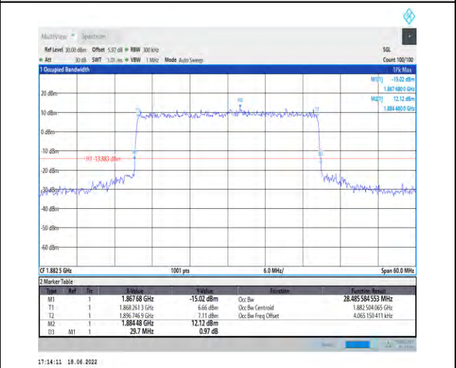
1-N25-PC3-15-30-M-8-CP-64QAM-Outer_Full-160@0-Ant1-28.486-29.700-≤30-PASS
