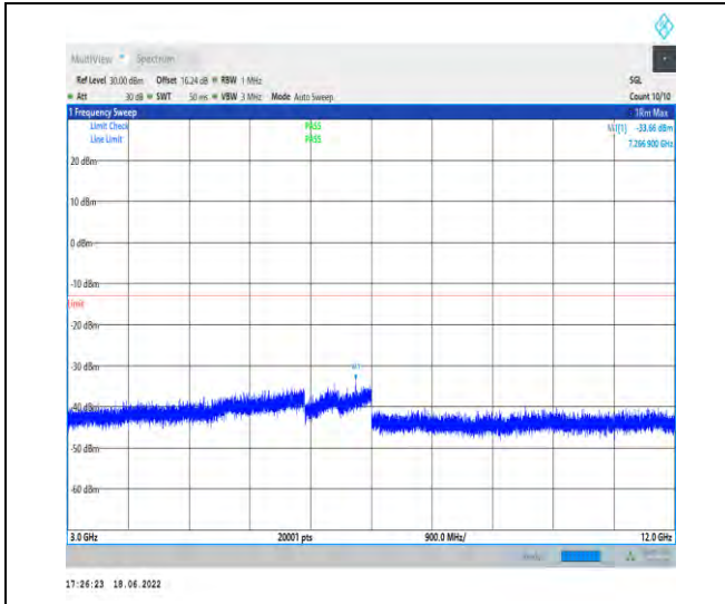
1-N25--15-40-L-1-DFT-PI2BPSK-Inner_1RB_Left-1 @1-3000-12000-Ant1--33.66--13-PASS
