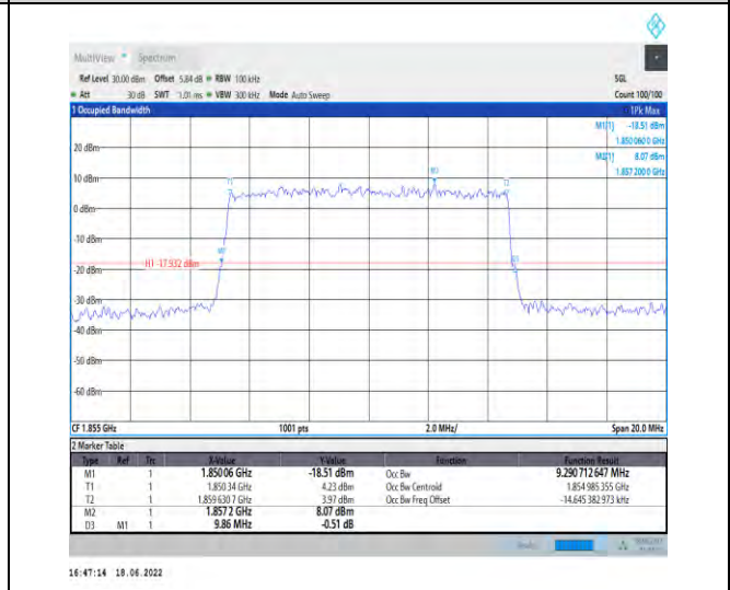
1-N25-PC3-15-10-L-9-CP-256QAM-Outer_Full-52@0- Ant1-9.291-9.860-≤10-PASS
