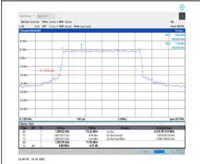
1-N25-PC3-15-10-L-8-CP-64QAM-Outer_Full-52@0- Ant1-9.277-9.880-≤10-PASS
