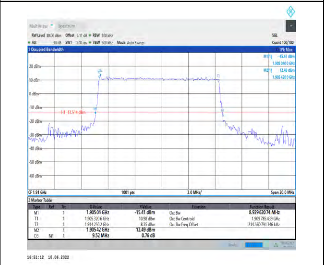
1-N25-PC3-15-10-H-3-DFT-16QAM-Outer_Full-50@ 0-Ant1-8.93-9.520-≤10-PASS
