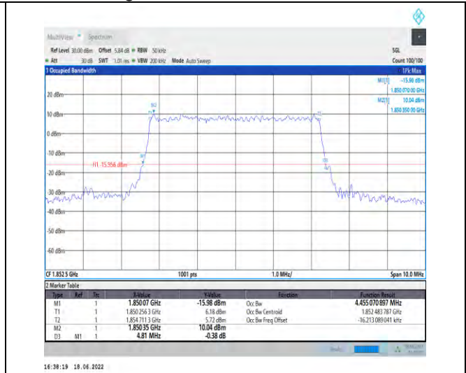
1-N25-PC3-15-5-L-6-CP-QPSK-Outer_Full-25@0-An t1-4.455-4.810-≤5-PASS
