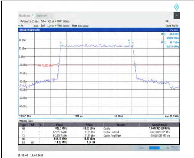
1-N5--15-15-M-2-DFT-PI2BPSK-Outer_Full-75@0-A nt1-13.408-14.250-≤15-PASS
