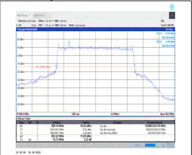
1-N5--15-20-H-7-CP-16QAM-Outer_Full-106@0-Ant 1-18.861-19.720-≤20-PASS
