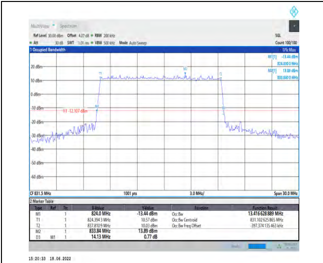
1-N5--15-15-L-3-DFT-16QAM-Outer_Full-75@0-Ant 1-13.417-14.130≤15-PASS
