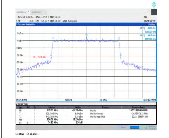
1-N5--15-15-M-8-CP-64QAM-Outer_Full-79@0-Ant1-14.113-14.850-≤15-PASS
