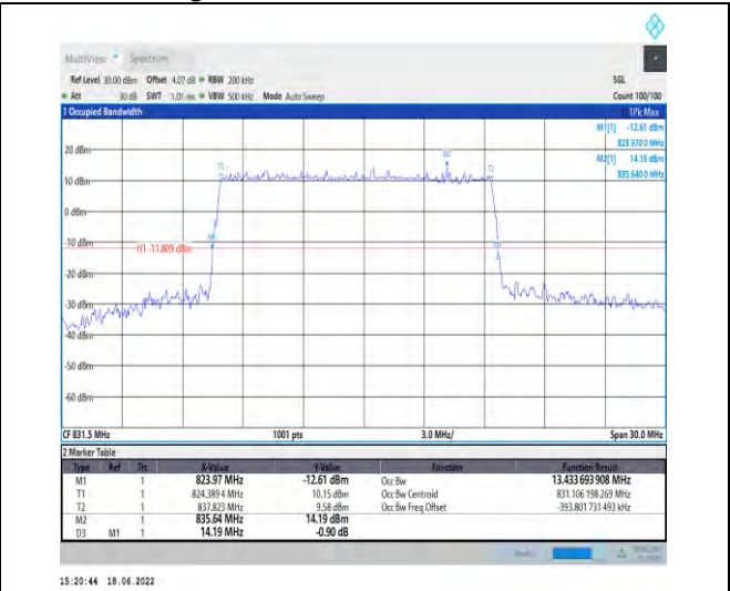
1-N5--15-15-L-4-DFT-64QAM-Outer_Full-75@0-Ant1 -13.434-14.190≤15-PASS
