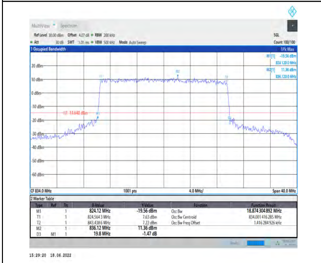
1-N5--15-20-L-6-CP-QPSK-Outer_Full-106@0-Ant1- 18.874-19.800-<=20-PASS
