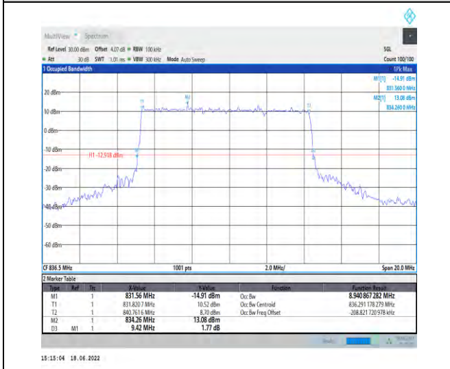
1-N5--15-10-M-3-DFT-16QAM-Outer_Full-50@0-Ant1 1-8.941-9.420-≤10-PASS
