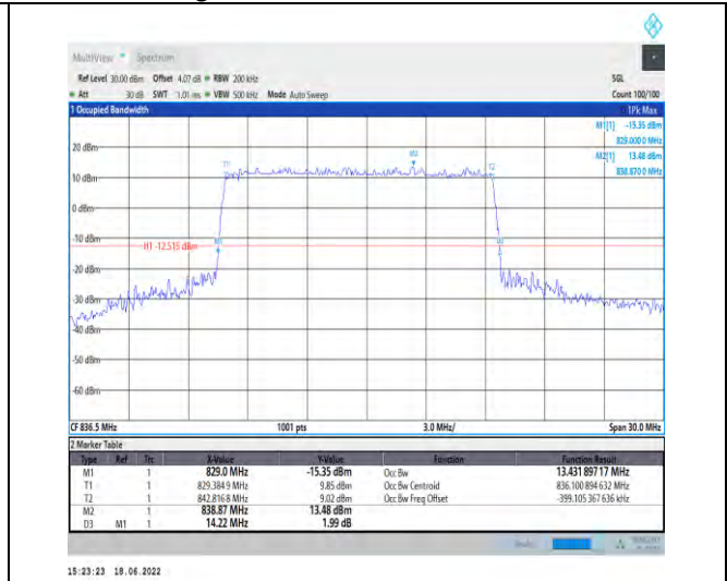
1-N5--15-15-M-3-DFT-16QAM-Outer_Full-75@0-Ant 1-13.432-14.220-≤15-PASS
