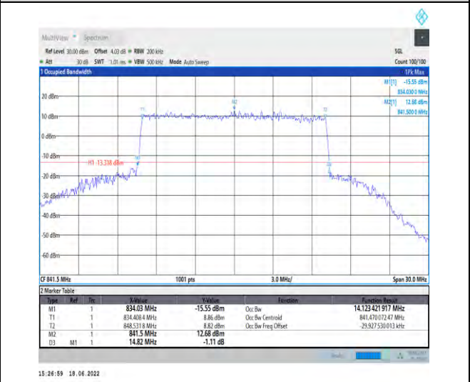
1-N5--15-15-H-8-CP-64QAM-Outer_Full-79@0-Ant1-1 14.123-14.820- \leq 15 -PASS
