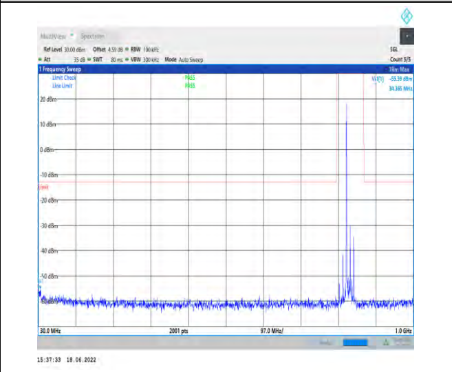
1-N5--15-20-M-1-DFT-PI2BPSK-Inner_1RB_Left-1@ 1-30-1000-Ant1--55.39--13-PASS
