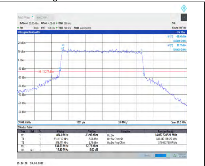
1-N5--15-15-H-6-CP-QPSK-Outer_Full-79@0-Ant1-1 4.058-14.850- \leq 15 -PASS
