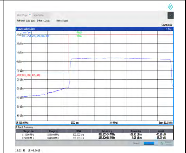
1-N5--15-20-L-6-CP-QPSK-Outer_Full-106@0-Ant1-seegraph-PASS-see graph
