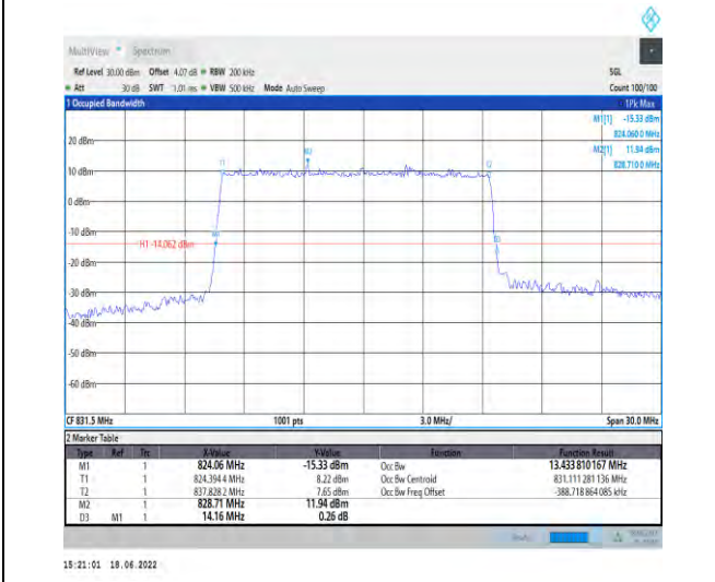
1-N5--15-15-L-5-DFT-256QAM-Outer_Full-75@0-An t1-13.434-14.160≤15-PASS
