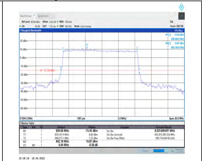
1-N5--15-10-H-5-DFT-256QAM-Outer_Full-50@0-Ant t1-8.926-9.440-≤10-PASS
