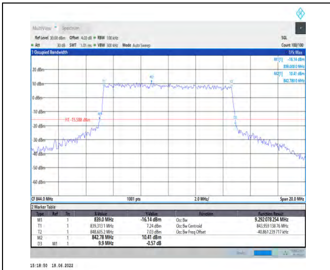
1-N5--15-10-H-8-CP-64QAM-Outer_Full-52@0-Ant1 -9.292-9.900-≤10-PASS
