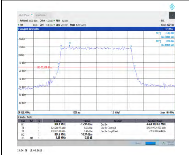
1-N5--15-5-L-7-CP-16QAM-Outer_Full-25@0-Ant1-4 .464-4.830-≤5-PASS
