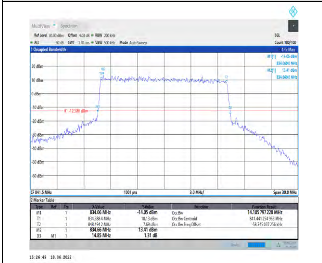
1-N5--15-15-H-7-CP-16QAM-Outer_Full-79@0-Ant1 -14.106-14.850- \leq 15 -PASS
