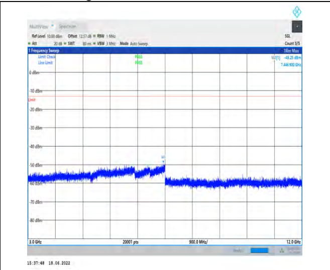
1-N5--15-20-M-1-DFT-PI2BPSK-Inner_1RB_Left-1@ 1-3000-12000-Ant1--49.25--13-PASS
