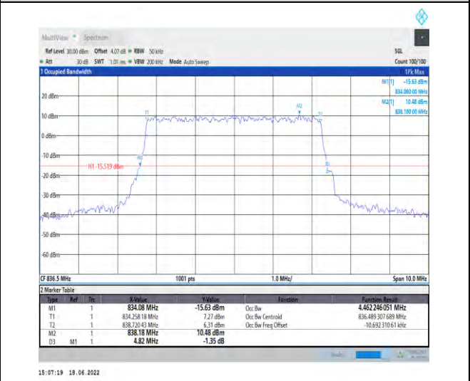
1-N5--15-5-M-7-CP-16QAM-Outer_Full-25@0-Ant1- 4.462-4.820-≤5-PASS
