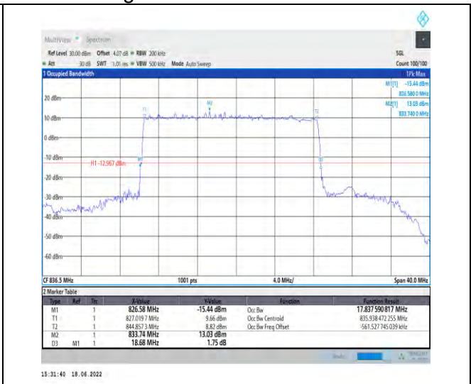
1-N5--15-20-M-4-DFT-64QAM-Outer_Full-100@0-A nt1-17.838-18.680-≤20-PASS
