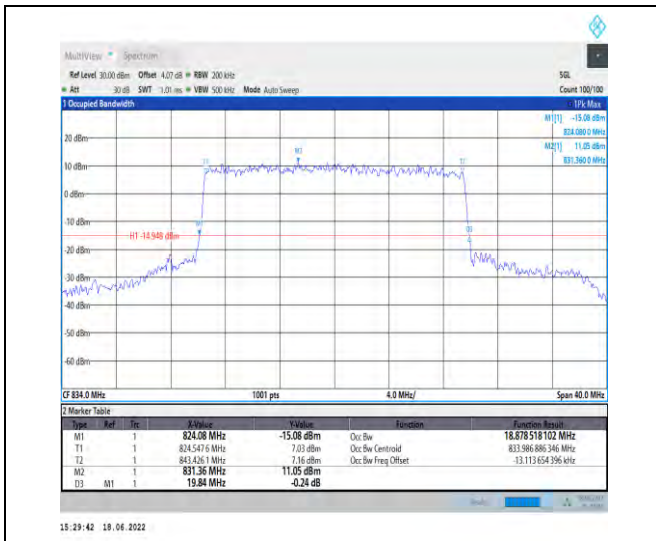
1-N5--15-20-L-8-CP-64QAM-Outer_Full-106@0-Ant 1-18.879-19.840-≤20-PASS
