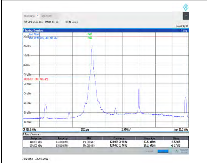
1-N5--15-15-L-4-CP-QPSK-Edge_1RB_Left-1@0-Ant1-seegraph-PASS-see graph
