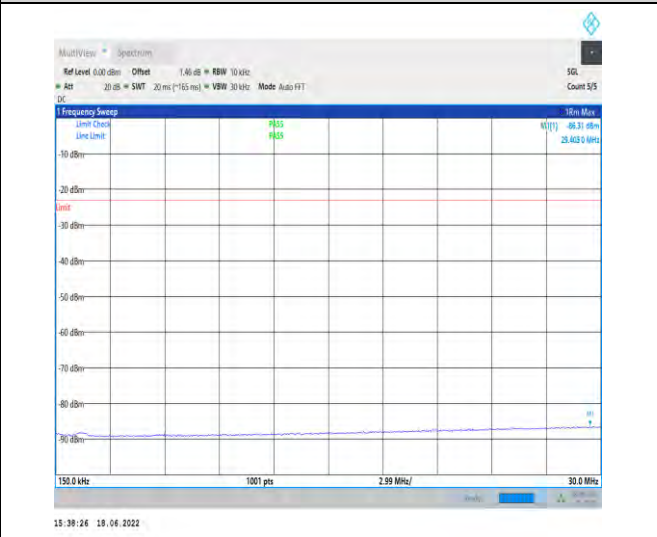
1-N5--15-20-H-1-DFT-PI2BPSK-Inner_1RB_Left-1@ 1-0.15-30-Ant1--86.31--23-PASS
