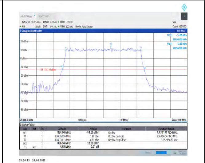
1-N5--15-5-M-3-DFT-16QAM-Outer_Full-25@0-Ant1-4.47-4.920-≤5-PASS
