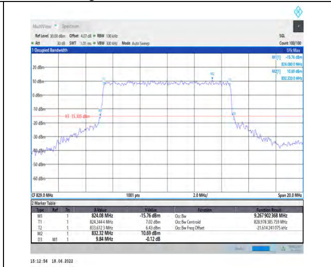
1-N5--15-10-L-7-CP-16QAM-Outer_Full-52@0-Ant1-9 -15.305 ≤ -10-PASS
