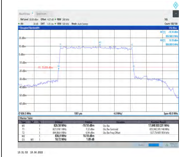
1-N5--15-20-M-5-DFT-256QAM-Outer_Full-100@0-A Ant1-17.848-18.720-≤20-PASS
