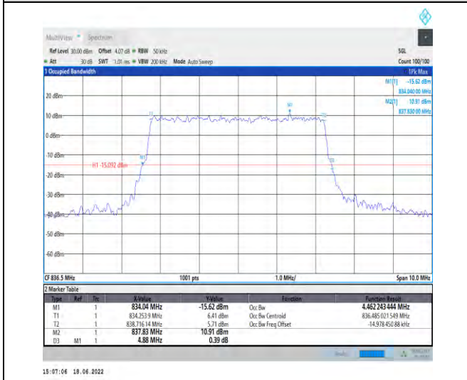
1-N5--15-5-M-6-CP-QPSK-Outer_Full-25@0-Ant1-4. 462-4.880-≤5-PASS
