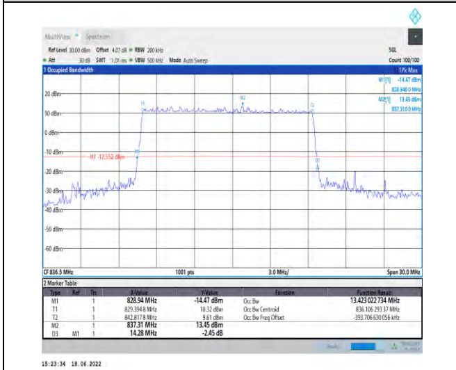
1-N5--15-15-M-4-DFT-64QAM-Outer_Full-75@0-Ant 1-13.423-14.280-≤15-PASS
