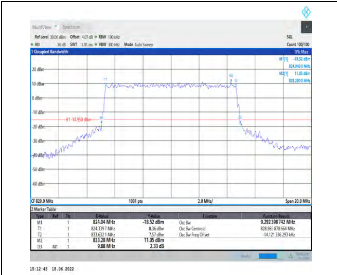
1-N5--15-10-L-6-CP-QPSK-Outer_Full-52@0-Ant1-9 -18.550 ≤ -10-PASS
