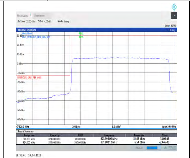
1-N5--15-20-L-3-DFT-PI2BPSK-Outer_Full-100@0-Ant1-seegraph-PASS-see graph
