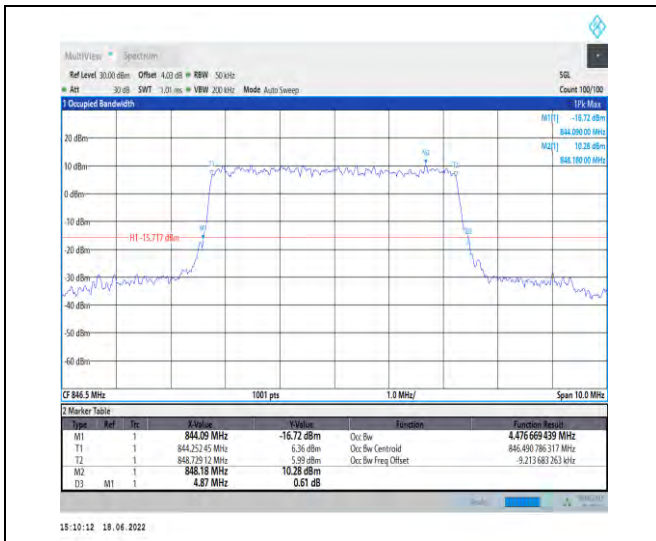
1-N5--15-5-H-7-CP-16QAM-Outer_Full-25@0-Ant1-4.477-4.870-≤5-PASS
