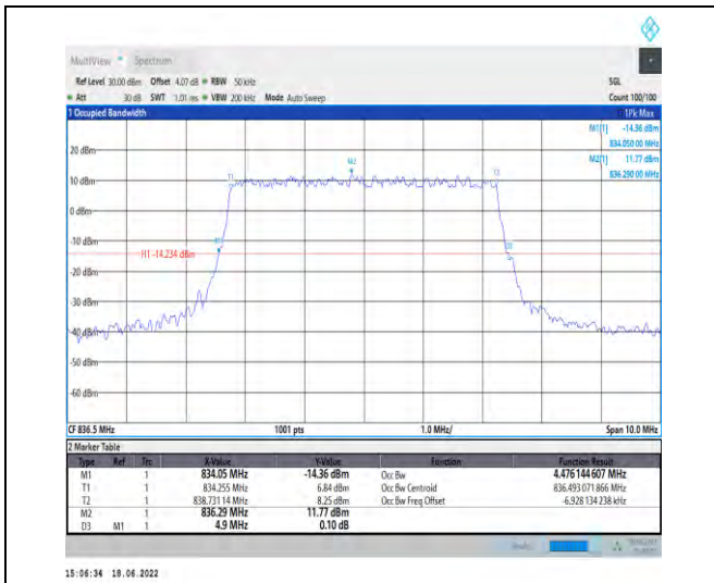
1-N5--15-5-M-4-DFT-64QAM-Outer_Full-25@0-Ant1 -4.476-4.900-≤5-PASS
