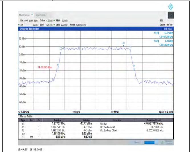
1-N2--15-5-M-5-DFT-256QAM-Outer_Full-25@0-Ant 1-4.465-4.890-≤5-PASS
