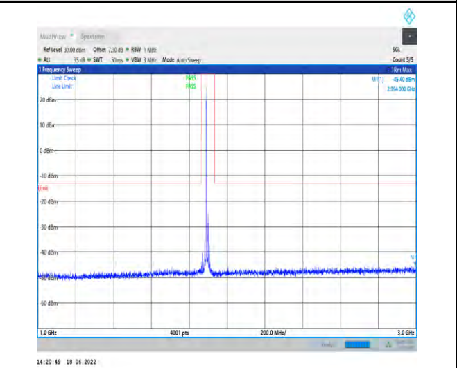
1-N2--15-20-H-1-DFT-PI2BPSK-Inner_1RB_Left-1@ 1-1000-3000-Ant1--45.40--13-PASS
