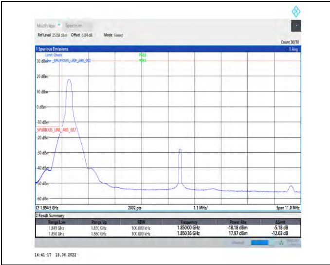
1-N2--15-10-L-1-DFT-PI2BPSK-Edge_1RB_Left-1@0-Ant1-seegraph-PASS-see graph
