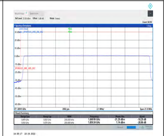
1-N2--15-20-L-6-CP-QPSK-Outer_Full-106@0-Ant1-seegraph-PASS-see graph
