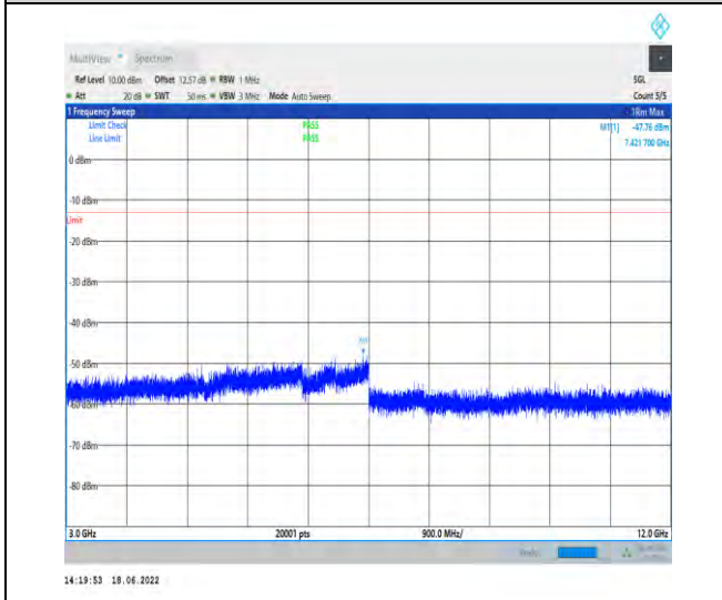
1-N2--15-20-M-1-DFT-PI2BPSK-Inner_1RB_Left-1 @1-3000-12000-Ant1--47.76--13-PASS
