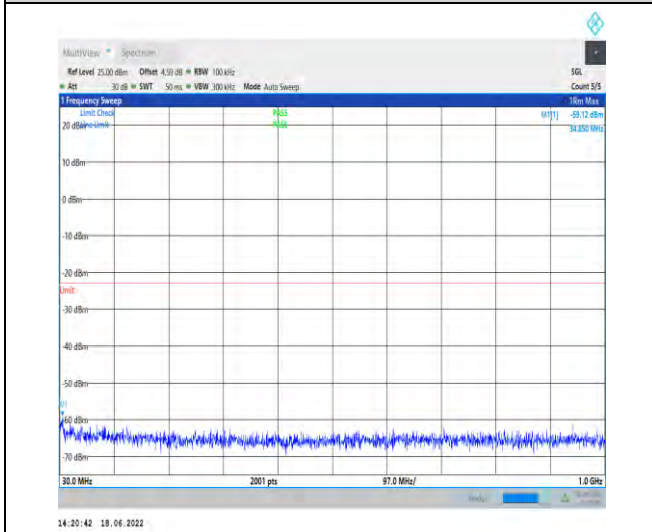
1-N2--15-20-H-1-DFT-PI2BPSK-Inner_1RB_Left-1@ 1-30-1000-Ant1--59.12--23-PASS
