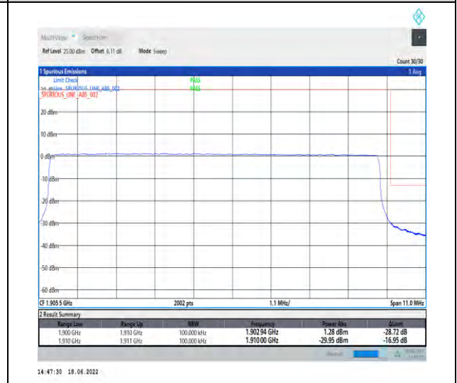
1-N2--15-10-H-6-CP-QPSK-Outer_Full-52@0-Ant1-seegraph-PASS-see graph
