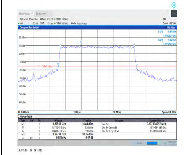
1-N2--15-10-M-7-CP-16QAM-Outer_Full-52@0-Ant1 -9.277-9.880-≤10-PASS
