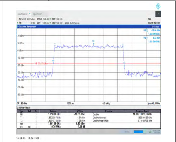
1-N2--15-20-L-9-CP-256QAM-Outer_Full-106@0-Ant 1-18.887-19.760-≤20-PASS
