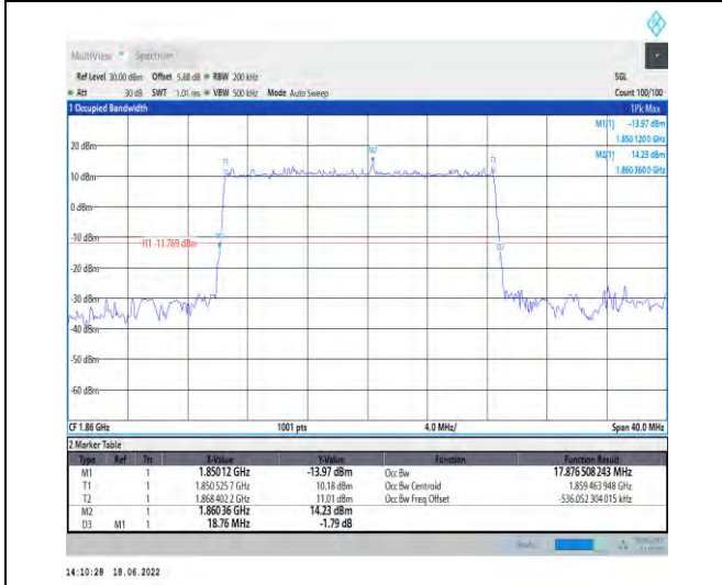
1-N2--15-20-L-2-DFT-PI2BPSK-Outer_Full-100@0-A nt1-17.877-18.760-≤20-PASS
