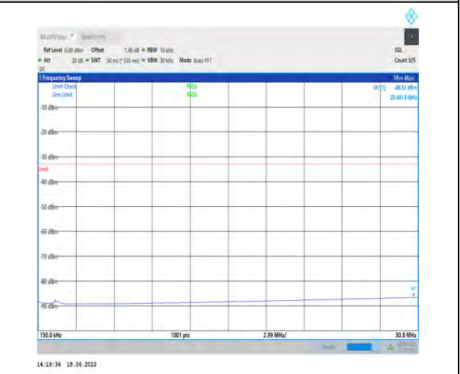
1-N2--15-20-M-1-DFT-PI2BPSK-Inner_1RB_Left-1@ 1-0.15-30-Ant1--86.51--33-PASS
