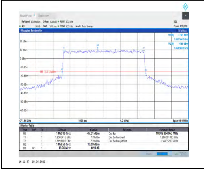
1-N2--15-20-L-6-CP-QPSK-Outer_Full-106@0-Ant1- 18.919-19.760-<=20-PASS
