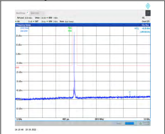
1-N2--15-20-M-1-DFT-PI2BPSK-Inner_1RB_Left-1@ 1-1000-3000-Ant1--45.28--13-PASS
