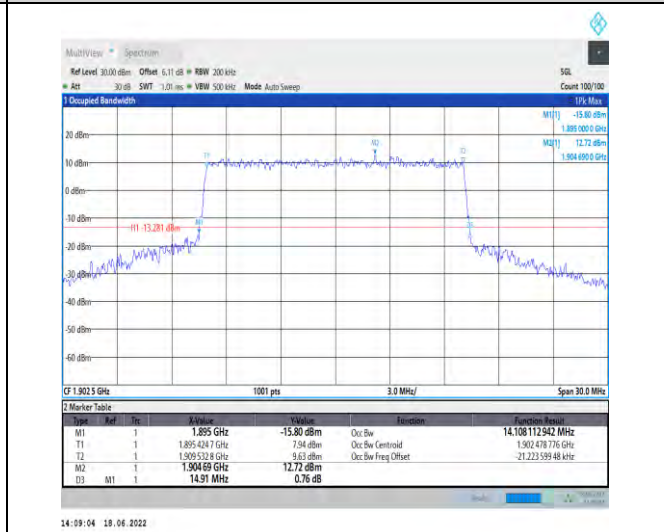
1-N2--15-15-H-8-CP-64QAM-Outer_Full-79@0-Ant1-1 14.108-14.910-≤15-PASS
