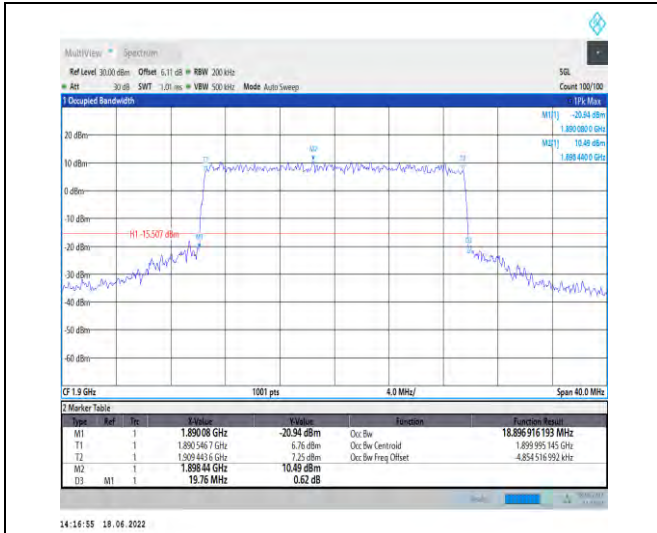
1-N2--15-20-H-6-CP-QPSK-Outer_Full-106@0-Ant1 18.897-19.760-≤20-PASS
