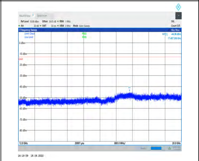
1-N2--15-20-M-1-DFT-PI2BPSK-Inner_1RB_Left-1@ 1-12000-20000-Ant1--44.38--13-PASS
