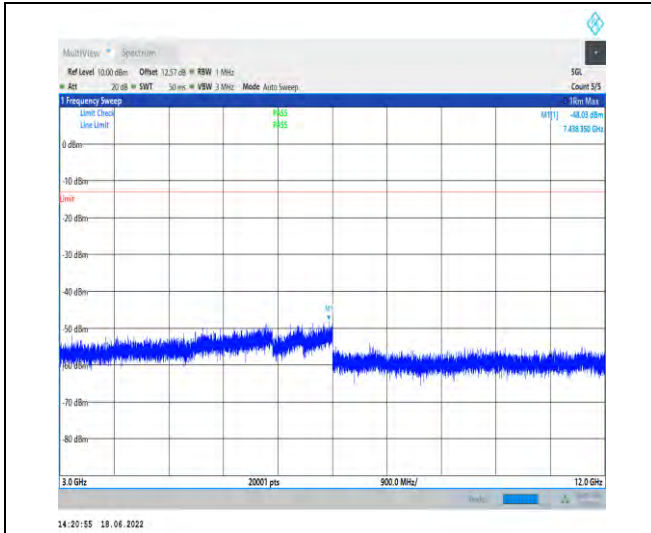
1-N2--15-20-H-1-DFT-PI2BPSK-Inner_1RB_Left-1@ 1-3000-12000-Ant1--48.03--13-PASS
