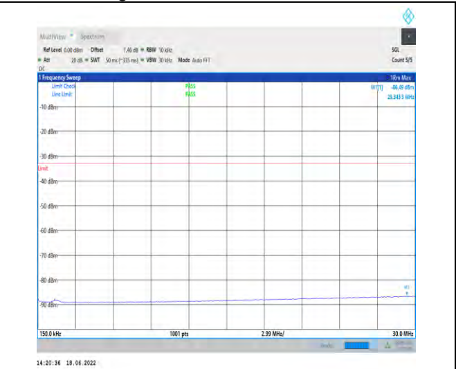
1-N2--15-20-H-1-DFT-PI2BPSK-Inner_1RB_Left-1@ 1-0.15-30-Ant1--86.49--33-PASS
