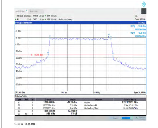
1-N2--15-10-H-6-CP-QPSK-Outer_Full-52@0-Ant1-9 .292-9.860-≤10-PASS
