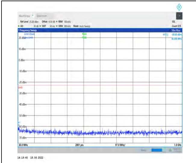
1-N2--15-20-M-1-DFT-PI2BPSK-Inner_1RB_Left-1 @1-30-1000-Ant1--59.85--23-PASS
