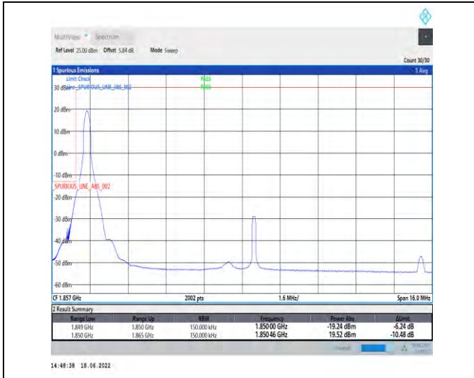
1-N2--15-15-L-1-DFT-PI2BPSK-Edge_1RB_Left-1@0-Ant1-seegraph-PASS-see graph
