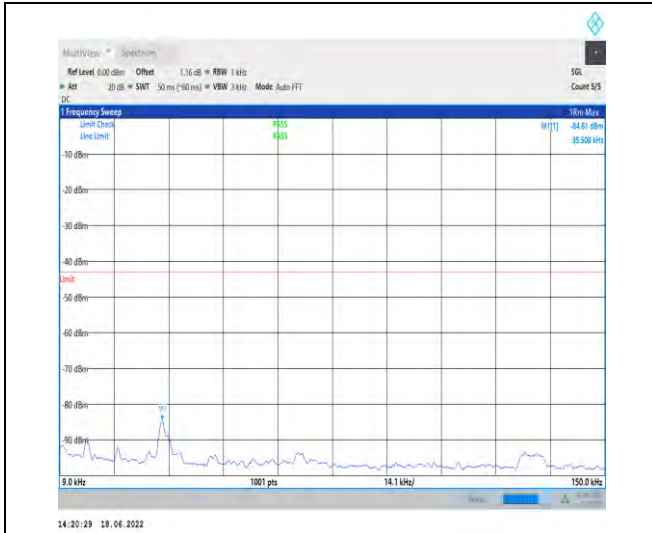
1-N2--15-20-H-1-DFT-PI2BPSK-Inner_1RB_Left-1@ 1-0.009-0.15-Ant1--84.61--43-PASS
