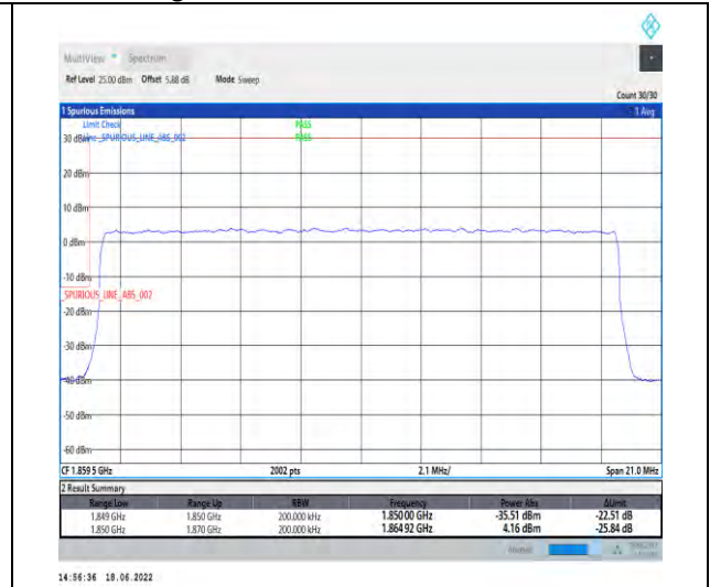
1-N2--15-20-L-3-DFT-PI2BPSK-Outer_Full-100@0-Ant1-seegraph-PASS-see graph
