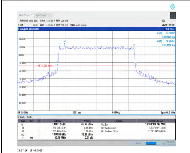
1-N2--15-20-H-8-CP-64QAM-Outer_Full-106@0-Ant 1-18.915-19.760-≤20-PASS
