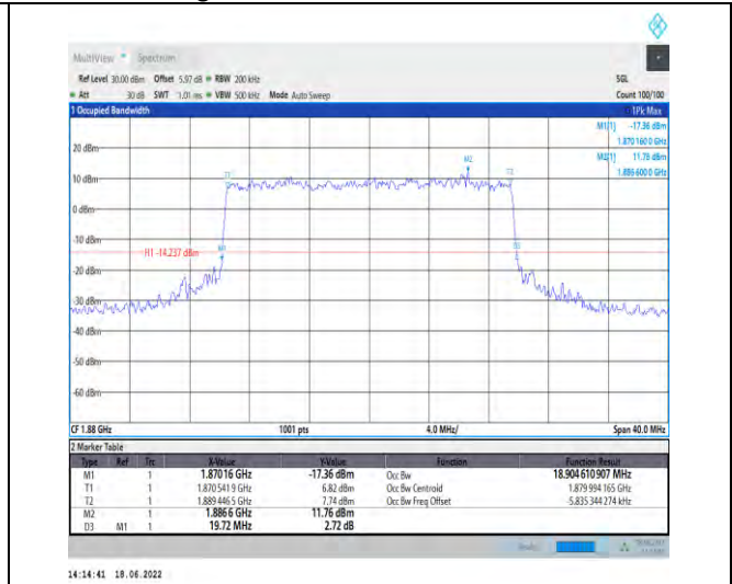
1-N2--15-20-M-8-CP-64QAM-Outer_Full-106@0-Ant 1-18.905-19.720-≤20-PASS
