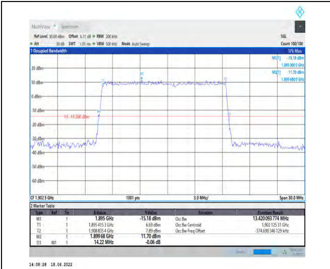
1-N2--15-15-H-5-DFT-256QAM-Outer_Full-75@0-An t1-13.42-14.220-≤15-PASS
