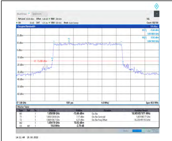
1-N2--15-20-L-8-CP-64QAM-Outer_Full-106@0-Ant 1-18.906-19.800-≤20-PASS
