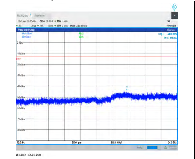
1-N2--15-20-L-1-DFT-PI2BPSK-Inner_1RB_Left-1@1 -12000-20000-Ant1--43.98--13-PASS
