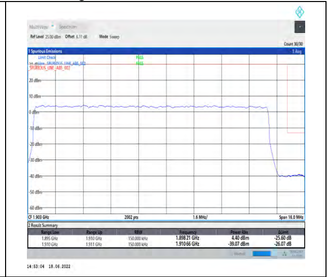
1-N2--15-15-H-3-DFT-PI2BPSK-Outer_Full-75@0-Ant1-seegraph-PASS-see graph
