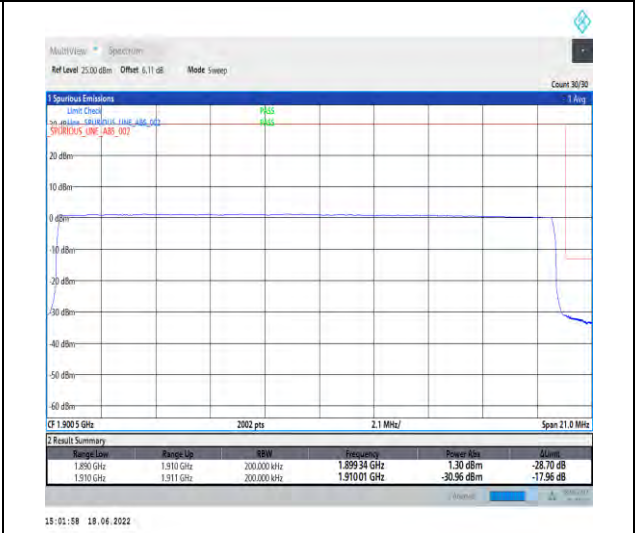
1-N2--15-20-H-6-CP-QPSK-Outer_Full-106@0-Ant1-seegraph-PASS-see graph
