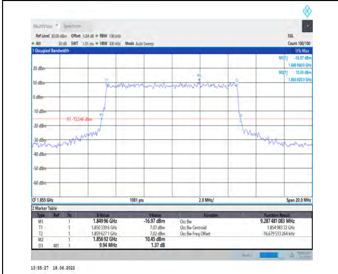
1-N2--15-10-L-8-CP-64QAM-Outer_Full-52@0-Ant1-9 9.287-9.940-≤10-PASS
