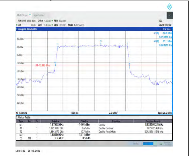
1-N2--15-10-M-2-DFT-PI2BPSK-Outer_Full-50@0-Ant1 -8.924-9.500-≤10-PASS
