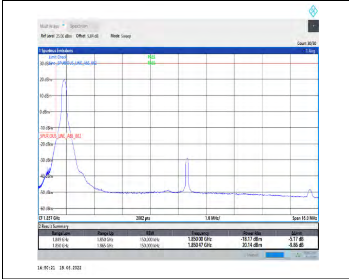
1-N2--15-15-L-4-CP-QPSK-Edge_1RB_Left-1@0-Ant1-seegraph-PASS-see graph
