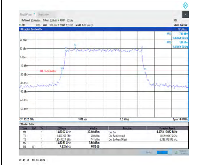
1-N2--15-5-L-7-CP-16QAM-Outer_Full-25@0-Ant1-4 .475-4.920-≤5-PASS
