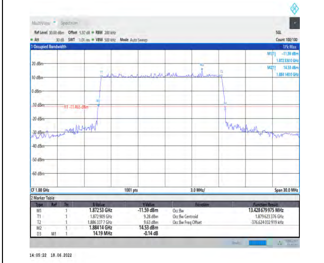
1-N2--15-15-M-4-DFT-64QAM-Outer_Full-75@0-Ant 1-13.429-14.190-≤15-PASS
