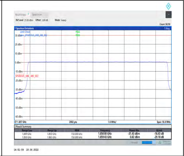
1-N2--15-15-L-6-CP-QPSK-Outer_Full-79@0-Ant1-seegraph-PASS-see graph
