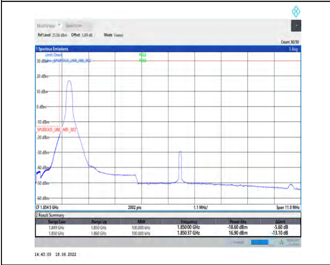
1-N2--15-10-L-4-CP-QPSK-Edge_1RB_Left-1@0-Ant1-seegraph-PASS-see graph
