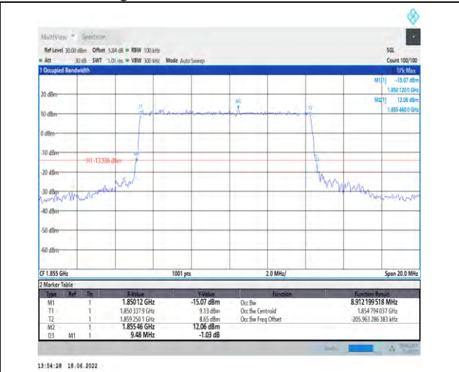
1-N2--15-10-L-3-DFT-16QAM-Outer_Full-50@0-Ant1 -8.912-9.480-≤10-PASS
