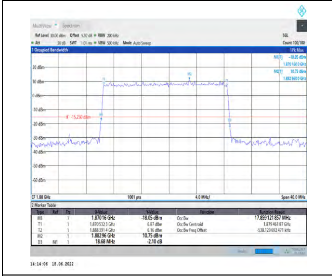
1-N2--15-20-M-5-DFT-256QAM-Outer_Full-100@0-Ant1 Ant1-17.859-18.680-≤20-PASS
