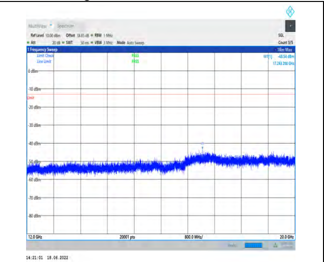
1-N2--15-20-H-1-DFT-PI2BPSK-Inner_1RB_Left-1@ 1-12000-20000-Ant1--43.54--13-PASS
