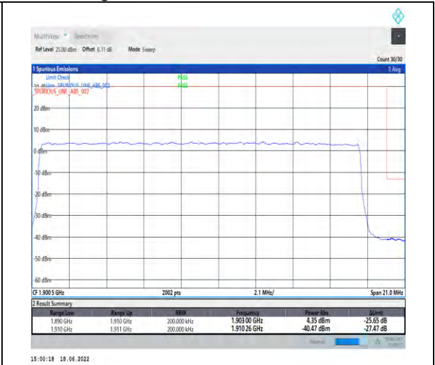
1-N2--15-20-H-3-DFT-PI2BPSK-Outer_Full-100@0-Ant1-seegraph-PASS-see graph
