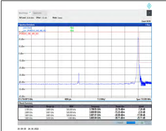
1-N78-3700-3800-PC2-30-100-H-2-DFT-PI2BPSK-Edge_1_RB_Right-1@272-Ant1-PASS-see graph
