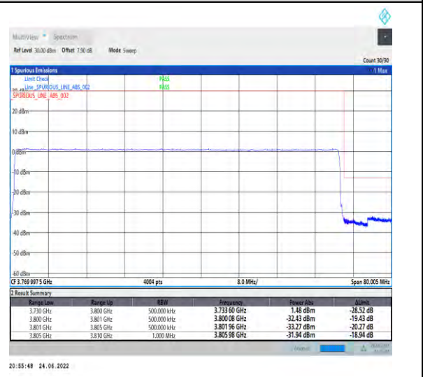
1-N78-3700-3800-PC2-30-70-H-6-CP-QPSK-Outer_Full-189@0-Ant1-PASS-see graph
