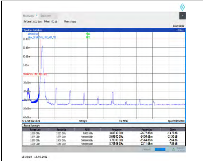
1-N78-3700-3800-PC2-30-80-L-1-DFT-PI2BPSK-Edge_1RB_Left-1@0-Ant1-PASS-see graph
