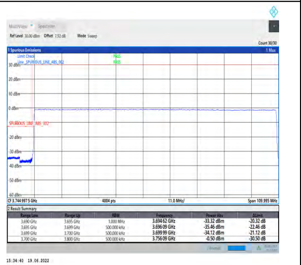
1-N78-3700-3800-PC2-30-100-L-6-CP-QPSK-Outer_Full-273@0-Ant1-PASS-see graph
