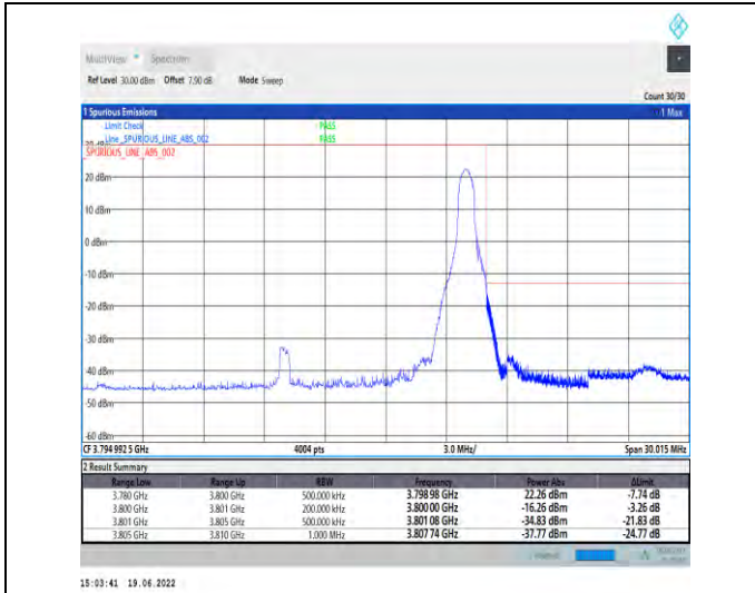
1-N78-3700-3800-PC2-30-20-H-2-DFT-PI2BPSK-Edge_1RB_Right-1@50-Ant1-PASS-see graph
