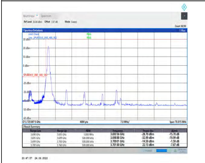
1-N78-3700-3800-PC2-30-60-L-4-CP-QPSK-Edge_1RB_Left-1@0-Ant1-PASS-see graph
