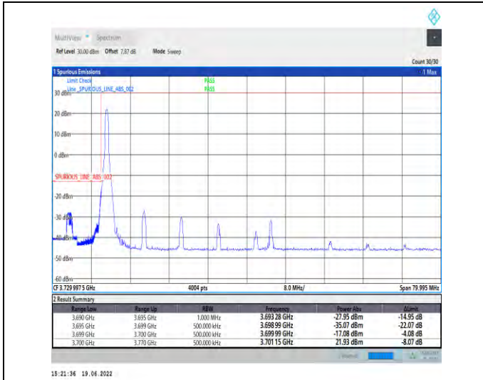
1-N78-3700-3800-PC2-30-70-L-1-DFT-PI2BPSK-Edge_1RB_Left-1@0-Ant1-PASS-see graph
