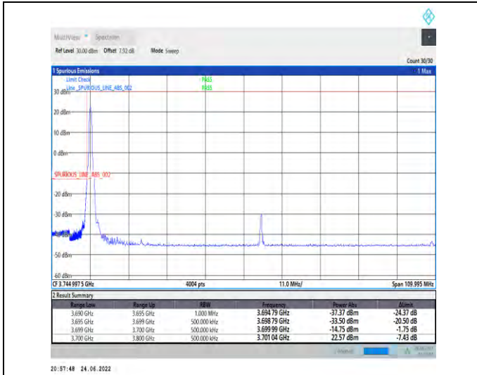
1-N78-3700-3800-PC2-30-100-L-1-DFT-PI2BPSK-Edge_1RB_Left-1@0-Ant1-PASS-see graph
