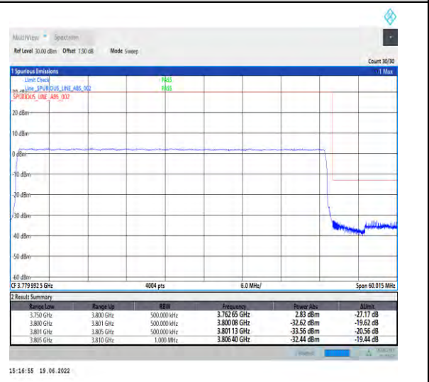
1-N78-3700-3800-PC2-30-50-H-6-CP-QPSK-Outer_Full-133@0-Ant1-PASS-see graph
