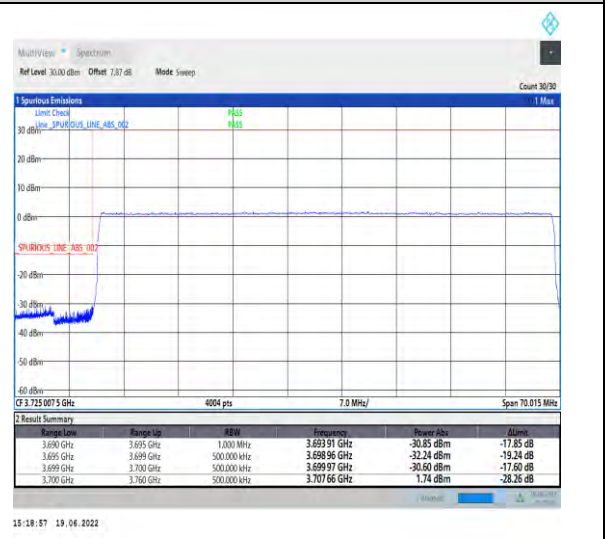
1-N78-3700-3800-PC2-30-60-L-6-CP-QPSK-Outer_Full-162@0-Ant1-PASS-see graph
