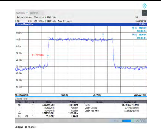
1-N78-3700-3800-PC2-30-100-H-4-DFT-64QAM-Out er_Full-270@0-Ant1-96.102-99.800-≤100-PASS
