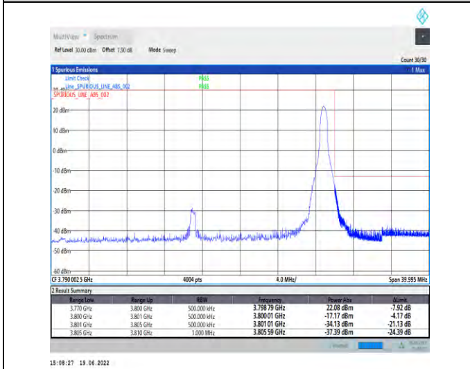
1-N78-3700-3800-PC2-30-30-H-5-CP-QPSK-Edge_1RB_Right-1@77-Ant1-PASS-see graph
