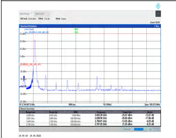
1-N78-3700-3800-PC2-30-90-L-4-CP-QPSK-Edge_1RB_Left-1@0-Ant1-PASS-see graph
