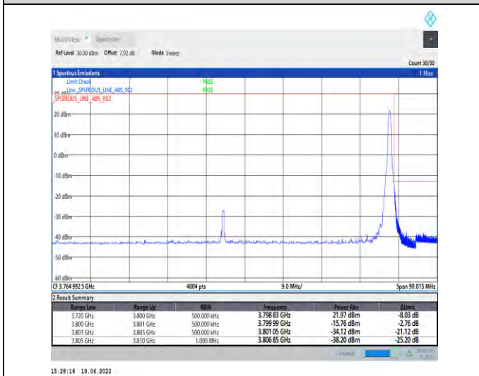
1-N78-3700-3800-PC2-30-80-H-5-CP-QPSK-Edge_1RB_Right-1@216-Ant1-PASS-see graph
