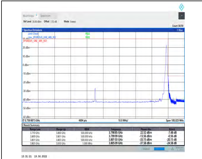
1-N78-3700-3800-PC2-30-90-H-2-DFT-PI2BPSK-Edge_1RB_Right-1@244-Ant1-PASS-see graph
