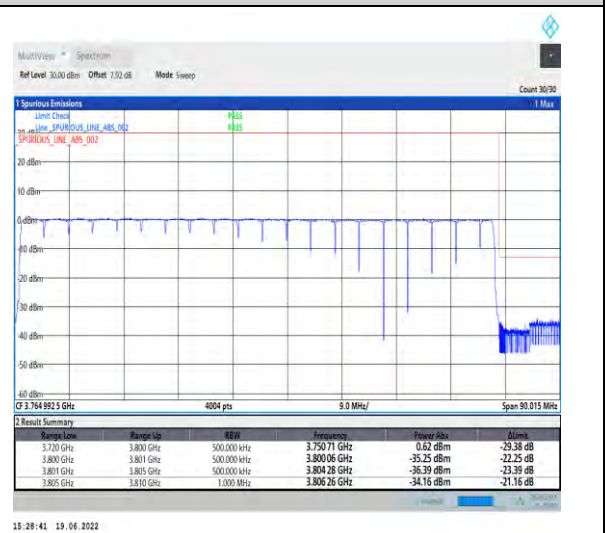
1-N78-3700-3800-PC2-30-80-H-6-CP-QPSK-Outer_Full-217@0-Ant1-PASS-see graph
