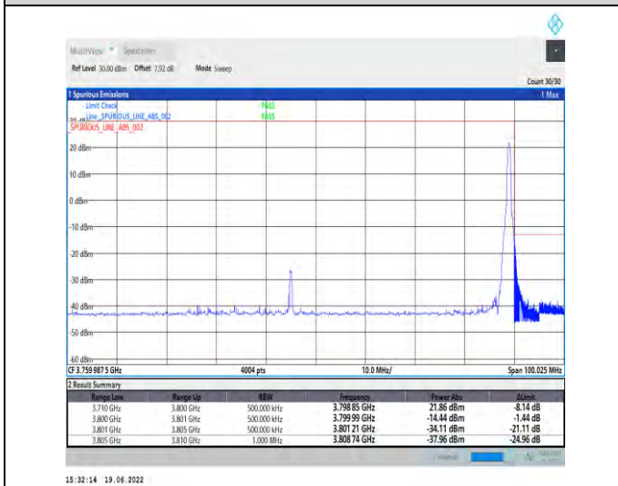
1-N78-3700-3800-PC2-30-90-H-5-CP-QPSK-Edge_1RB_Right-1@244-Ant1-PASS-see graph
