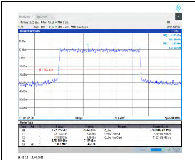
1-N78-3700-3800-PC2-30-100-M-8-CP-64QAM-Out er_Full-273@0-Ant1-97.611-101.000-≤100-PASS
