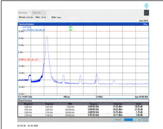
1-N78-3700-3800-PC2-30-40-L-1-DFT-PI2BPSK-Edge_1RB_Left-1@0-Ant1-PASS-see graph
