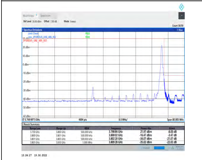
1-N78-3700-3800-PC2-30-70-H-5-CP-QPSK-Edge_1RB_Right-1@188-Ant1-PASS-see graph
