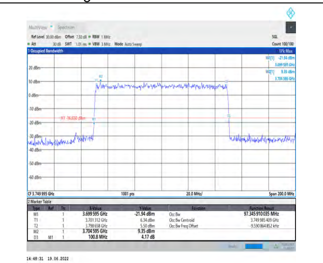
1-N78-3700-3800-PC2-30-100-M-9-CP-256QAM-Out er_Full-273@0-Ant1-97.346-100.800-≤100-PASS
