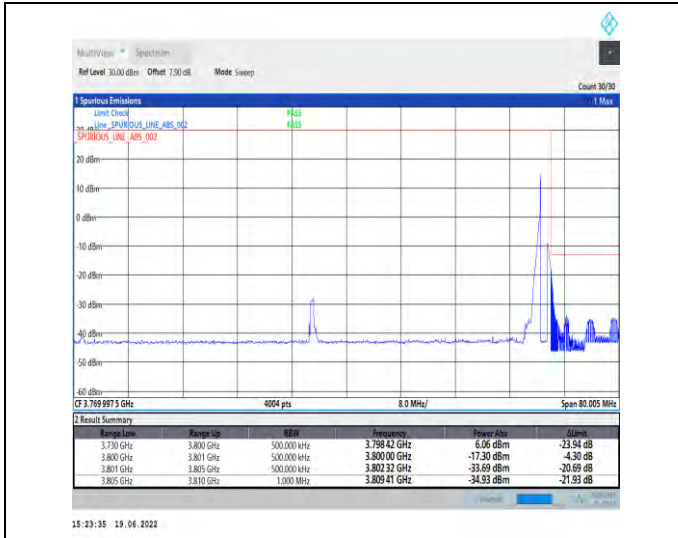
1-N78-3700-3800-PC2-30-70-H-2-DFT-PI2BPSK-Edge_1RB_Right-1@188-Ant1-PASS-see graph
