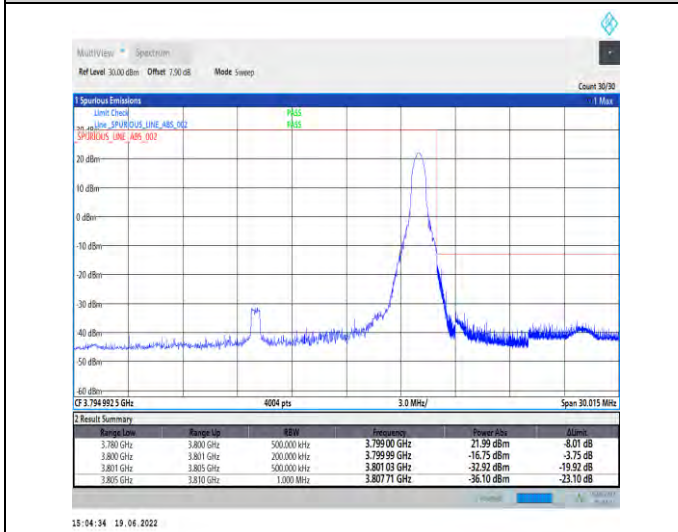
1-N78-3700-3800-PC2-30-20-H-5-CP-QPSK-Edge_1RB_Right-1@50-Ant1-PASS-see graph
