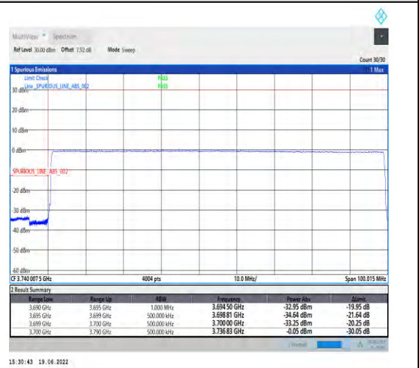
1-N78-3700-3800-PC2-30-90-L-6-CP-QPSK-Outer_Full-245@0-Ant1-PASS-see graph
