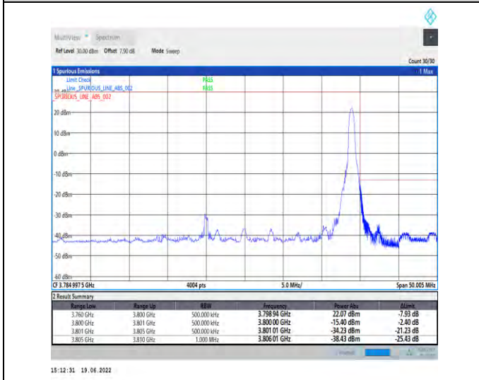
1-N78-3700-3800-PC2-30-40-H-5-CP-QPSK-Edge_1RB_Right-1@105-Ant1-PASS-see graph
