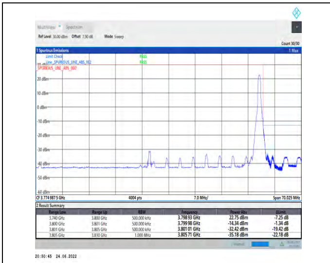
1-N78-3700-3800-PC2-30-60-H-2-DFT-PI2BPSK-Edge_1RB_Right-1@161-Ant1-PASS-see graph
