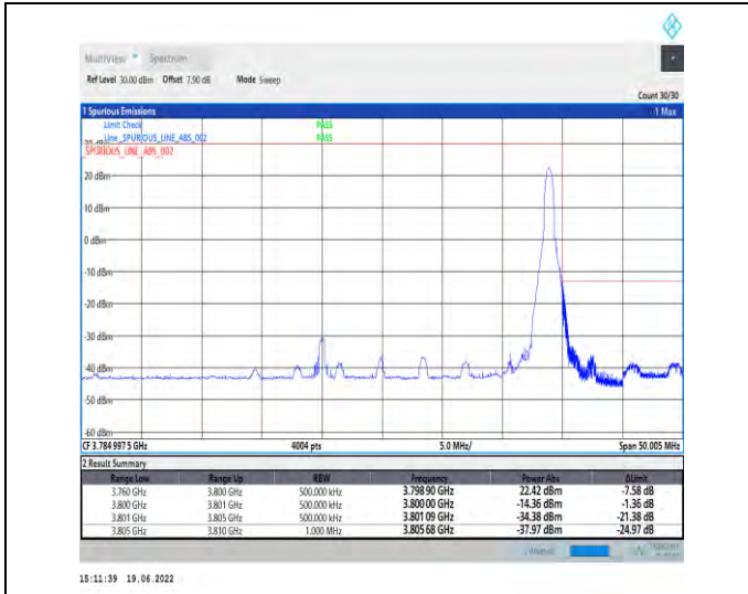
1-N78-3700-3800-PC2-30-40-H-2-DFT-PI2BPSK-Edge_1RB_Right-1@105-Ant1-PASS-see graph
