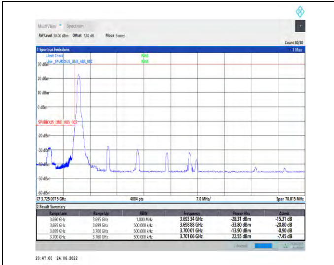
1-N78-3700-3800-PC2-30-60-L-1-DFT-PI2BPSK-Edge_1RB_Left-1@0-Ant1-PASS-see graph
