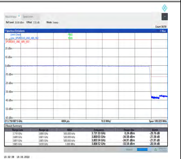
1-N78-3700-3800-PC2-30-90-H-6-CP-QPSK-Outer_Full-245@0-Ant1-PASS-see graph
