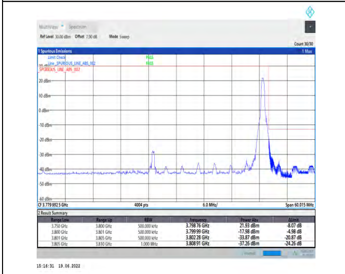
1-N78-3700-3800-PC2-30-50-H-5-CP-QPSK-Edge_1RB_Right-1@132-Ant1-PASS-see graph
