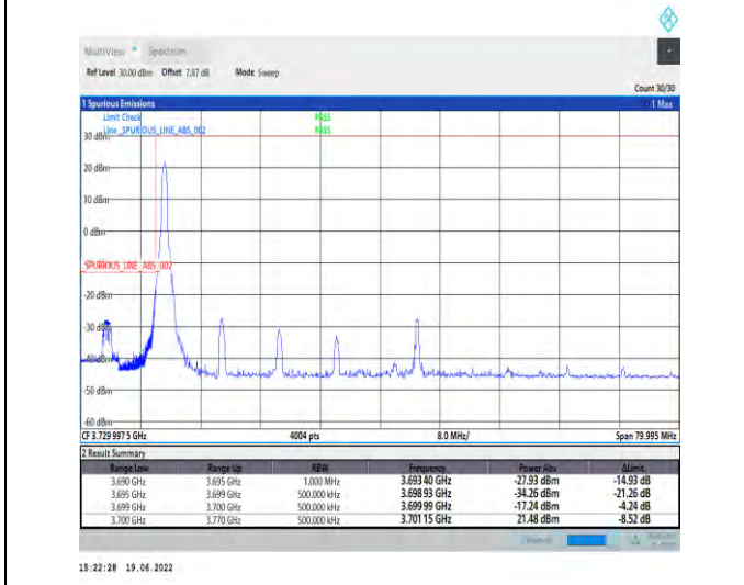
1-N78-3700-3800-PC2-30-70-L-4-CP-QPSK-Edge_1RB_Left-1@0-Ant1-PASS-see graph
