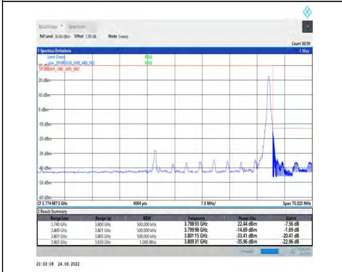
1-N78-3700-3800-PC2-30-60-H-5-CP-QPSK-Edge_1RB_Right-1@161-Ant1-PASS-see graph
