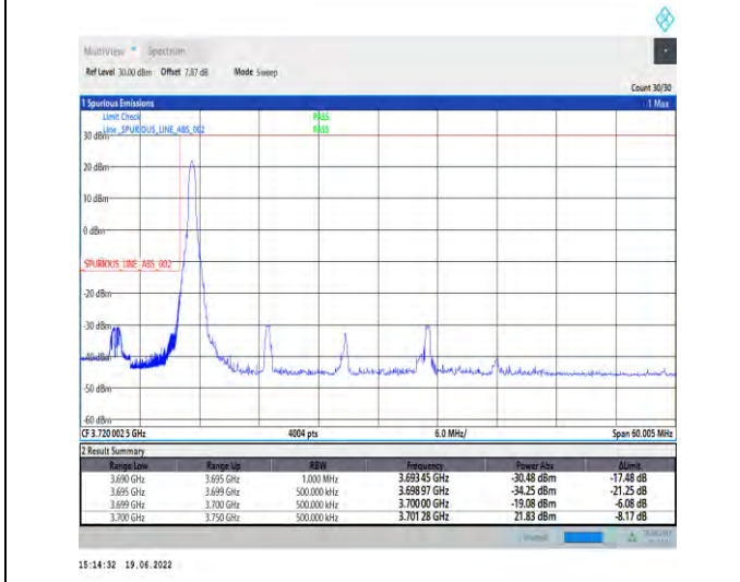
1-N78-3700-3800-PC2-30-50-L-4-CP-QPSK-Edge_1RB_Left-1@0-Ant1-PASS-see graph
