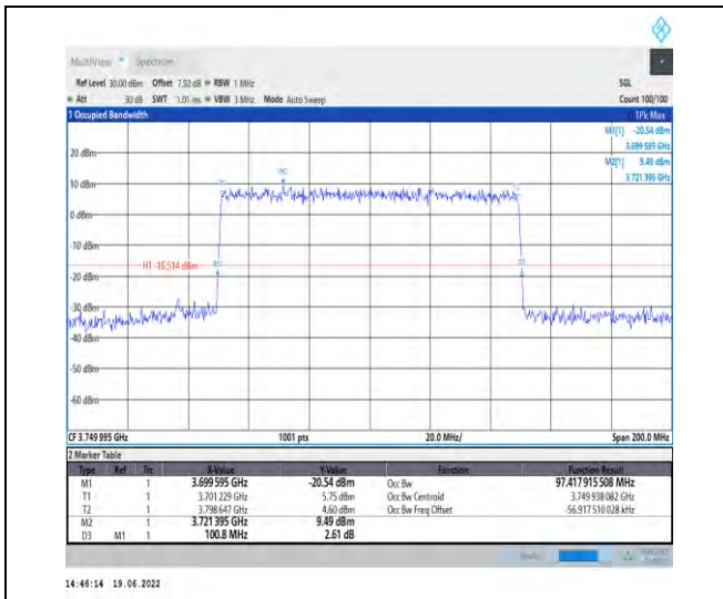
1-N78-3700-3800-PC2-30-100-L-9-CP-256QAM-Out er_Full-273@0-Ant1-97.418-100.800-≤100-PASS
