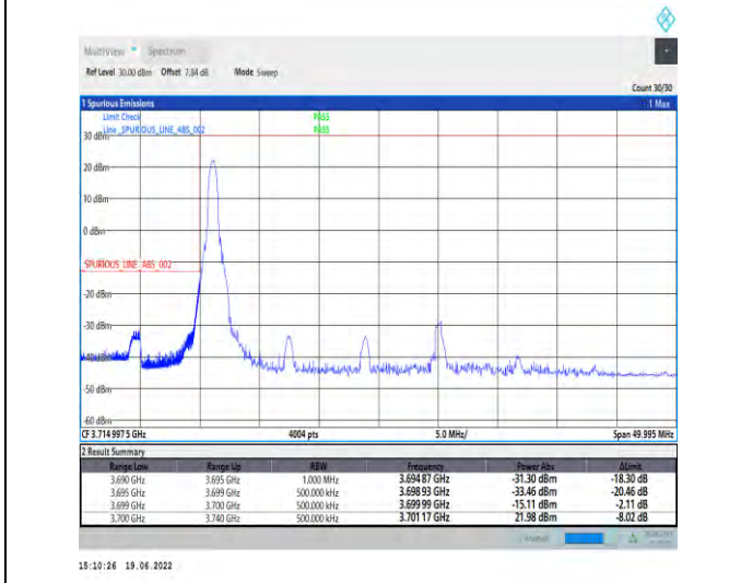
1-N78-3700-3800-PC2-30-40-L-4-CP-QPSK-Edge_1RB_Left-1@0-Ant1-PASS-see graph
