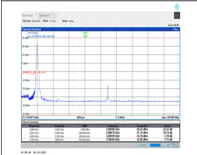
1-N78-3700-3800-PC2-30-100-L-4-CP-QPSK-Edge_1RB_Left-1@0-Ant1-PASS-see graph
