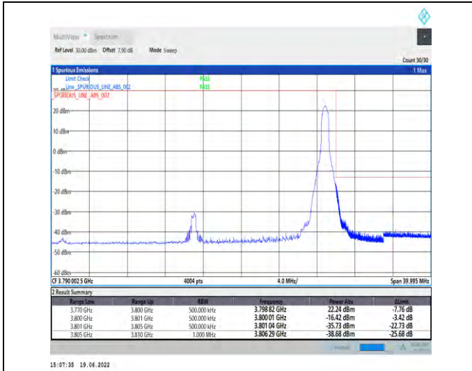
1-N78-3700-3800-PC2-30-30-H-2-DFT-PI2BPSK-Edge_1RB_Right-1@77-Ant1-PASS-see graph
