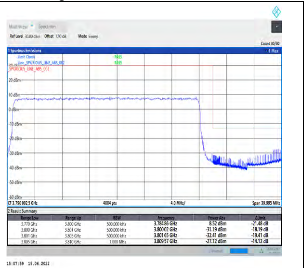
1-N78-3700-3800-PC2-30-30-H-3-DFT-PI2BPSK-Outer_Full-75@0-Ant1-PASS-see graph
