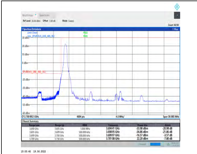
1-N78-3700-3800-PC2-30-30-L-1-DFT-PI2BPSK-Edge_1RB_Left-1@0-Ant1-PASS-see graph
