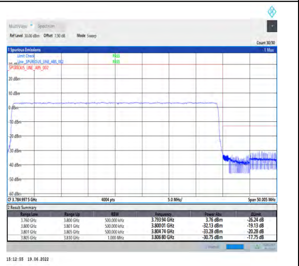
1-N78-3700-3800-PC2-30-40-H-6-CP-QPSK-Outer_Full-106@0-Ant1-PASS-see graph
