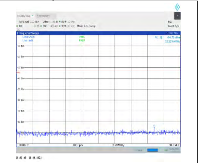
1-N78-3700-3800-PC2-30-100-H-1-DFT-PI2BPSK-In ner_1RB_Left-1@1-0.15-30-Ant1--86.76--33-PASS
