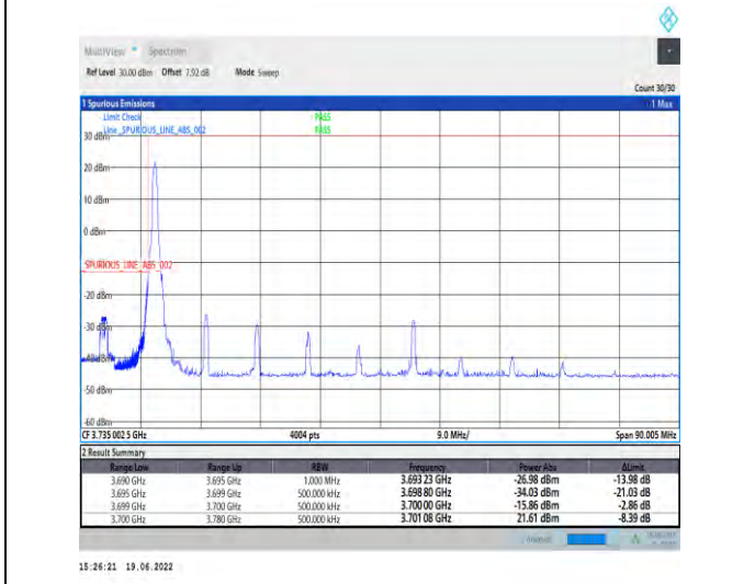
1-N78-3700-3800-PC2-30-80-L-4-CP-QPSK-Edge_1RB_Left-1@0-Ant1-PASS-see graph
