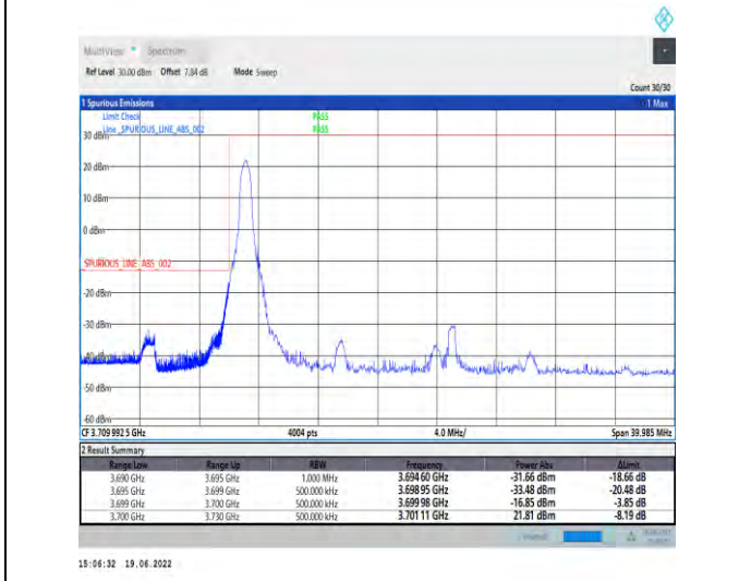
1-N78-3700-3800-PC2-30-30-L-4-CP-QPSK-Edge_1RB_Left-1@0-Ant1-PASS-see graph
