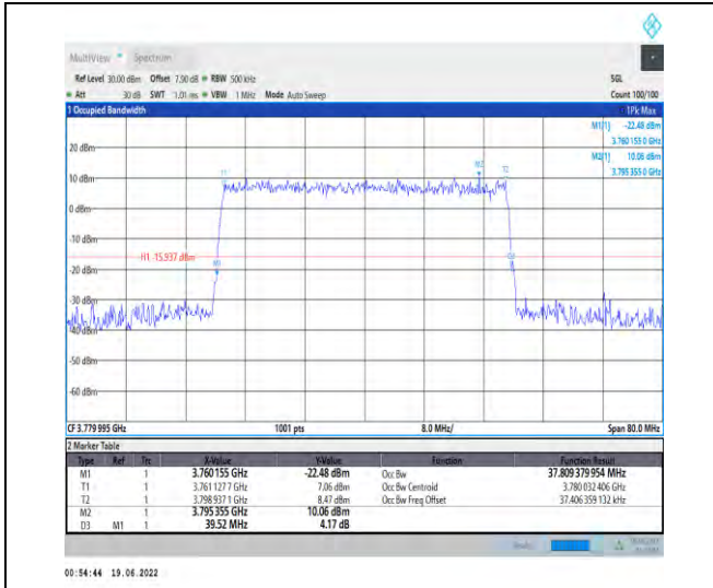
1-N78-3700-3800-PC2-30-40-H-9-CP-256QAM-Outer_Full-106@0-Ant1-37.809-39.520-≤40-PASS
