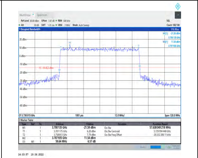
1-N78-3700-3800-PC2-30-60-L-8-CP-64QAM-Outer_Full-162@0-Ant1-57.638-59.640-≤60-PASS
