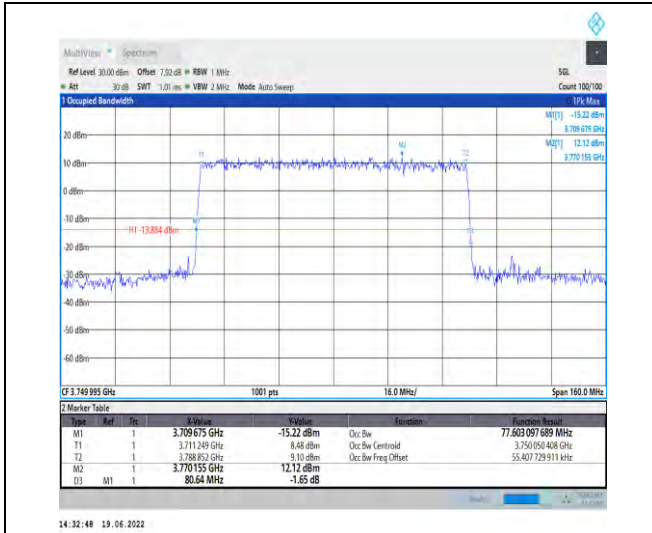
1-N78-3700-3800-PC2-30-80-M-6-CP-QPSK-Outer_Full-217@0-Ant1-77.603-80.640-≤80-PASS
