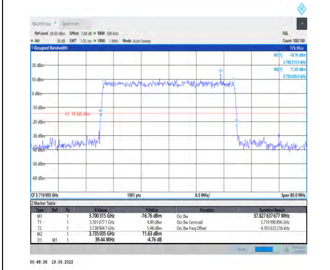
1-N78-3700-3800-PC2-30-40-L-9-CP-256QAM-Outer_Full-106@0-Ant1-37.828-39.440-≤40-PASS
