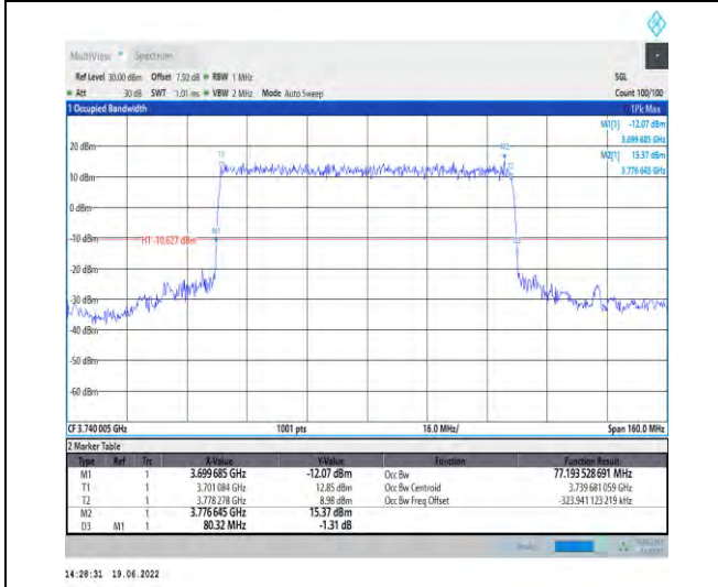
1-N78-3700-3800-PC2-30-80-L-1-DFT-QPSK-Outer_Full-216@0-Ant1-77.194-80.320-≤80-PASS
