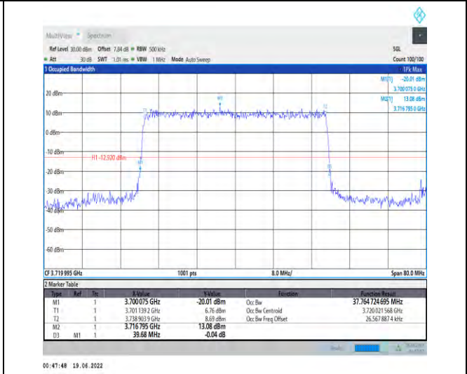
1-N78-3700-3800-PC2-30-40-L-6-CP-QPSK-Outer_Full-106@0-Ant1-37.765-39.680-≤40-PASS
