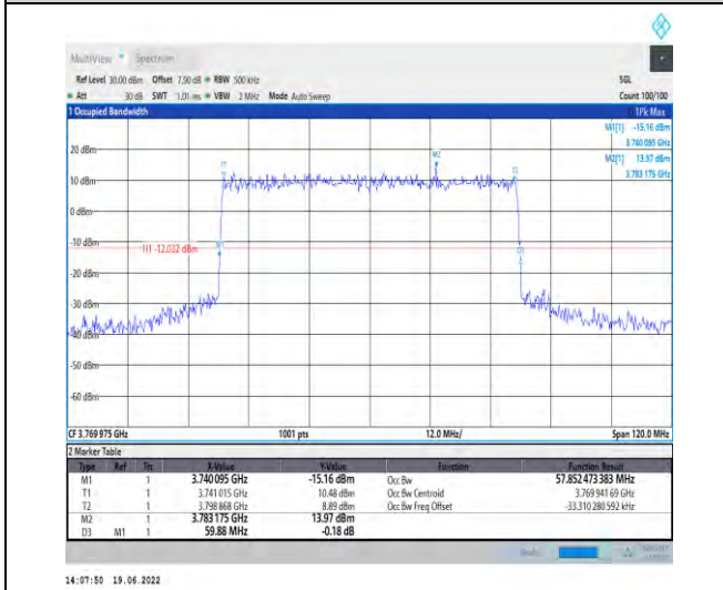
1-N78-3700-3800-PC2-30-60-H-1-DFT-QPSK-Outer_Full-162@0-Ant1-57.852-59.880-≤60-PASS
