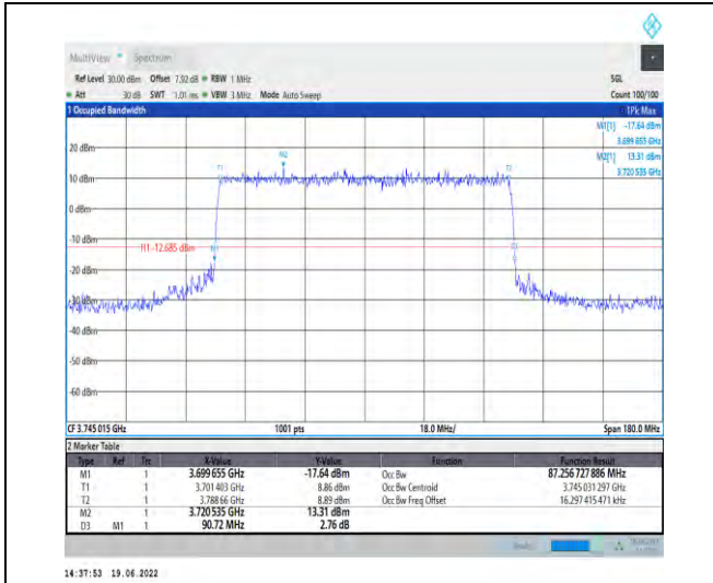
1-N78-3700-3800-PC2-30-90-L-8-CP-64QAM-Outer _Full-245@0-Ant1-87.257-90.720-≤90-PASS
