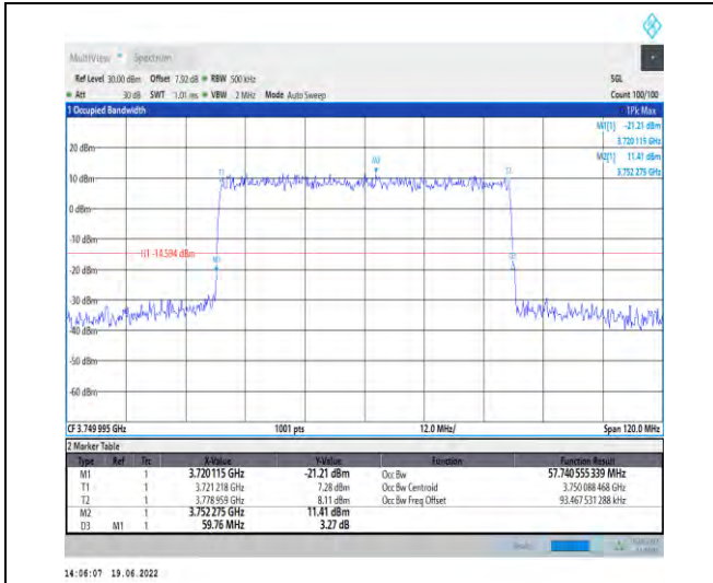
1-N78-3700-3800-PC2-30-60-M-4-DFT-64QAM-Out er_Full-162@0-Ant1-57.741-59.760-≤60-PASS
