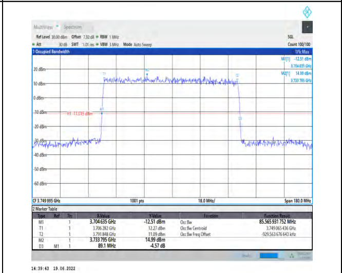
1-N78-3700-3800-PC2-30-90-M-2-DFT-PI2BPSK-Outer _Full-240@0-Ant1-85.566-89.100-≤90-PASS
