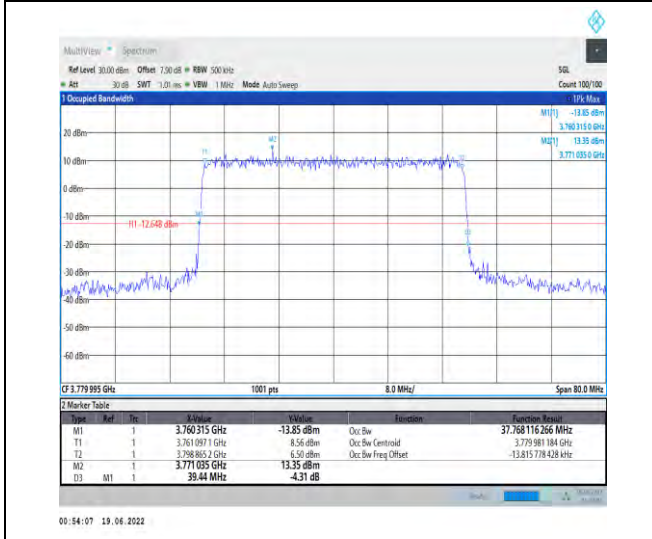
1-N78-3700-3800-PC2-30-40-H-7-CP-16QAM-Outer_Full-106@0-Ant1-37.768-39.440-≤40-PASS
