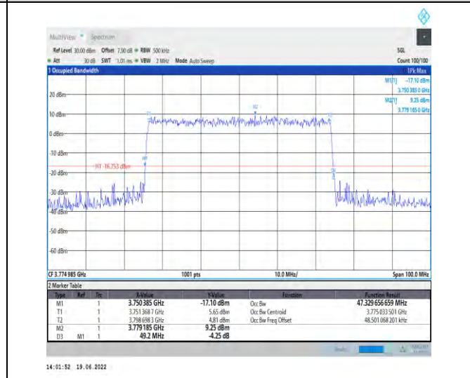
1-N78-3700-3800-PC2-30-50-H-9-CP-256QAM-Outer_Full-133@0-Ant1-47.33-49.200-≤50-PASS
