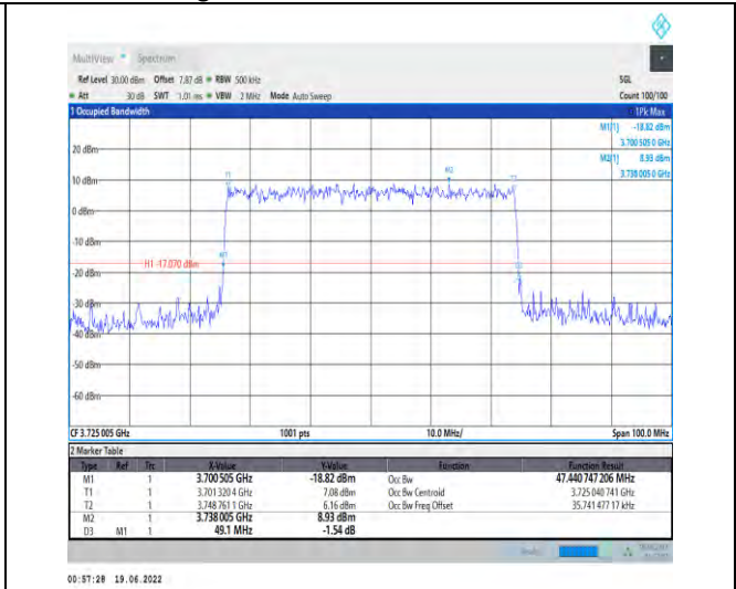
1-N78-3700-3800-PC2-30-50-L-9-CP-256QAM-Outer _Full-133@0-Ant1-47.441-49.100-≤50-PASS
