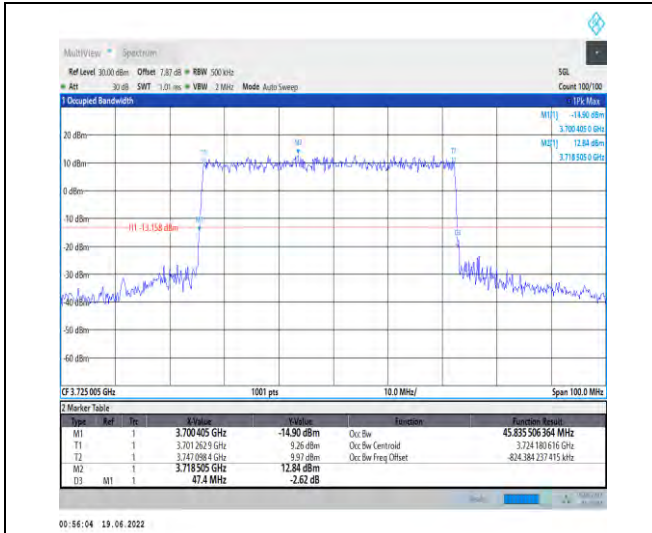
1-N78-3700-3800-PC2-30-50-L-4-DFT-64QAM-Outer_Full-128@0-Ant1-45.836-47.400-≤50-PASS
