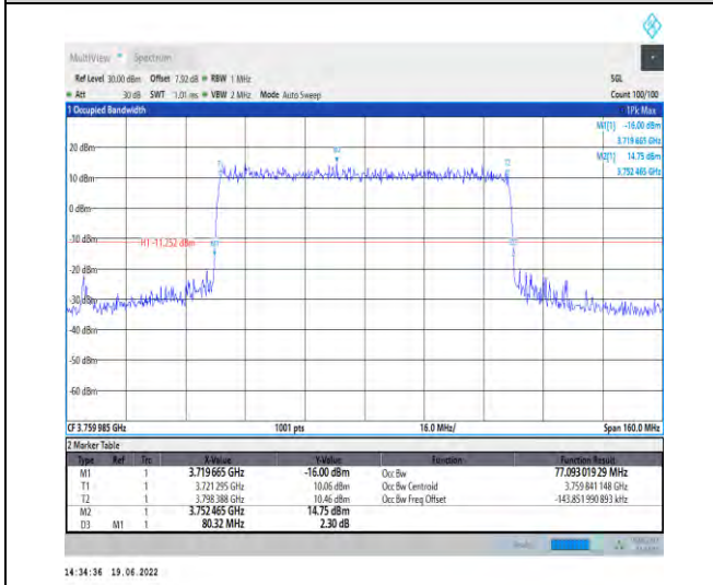
1-N78-3700-3800-PC2-30-80-H-3-DFT-16QAM-Outer_Full-216@0-Ant1-77.093-80.320-≤80-PASS
