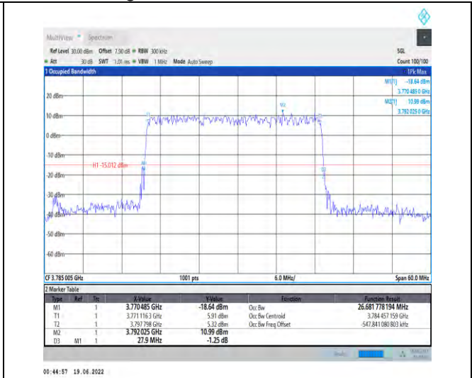
1-N78-3700-3800-PC2-30-30-H-5-DFT-256QAM-Outer_Full-75@0-Ant1-26.682-27.900-≤30-PASS
