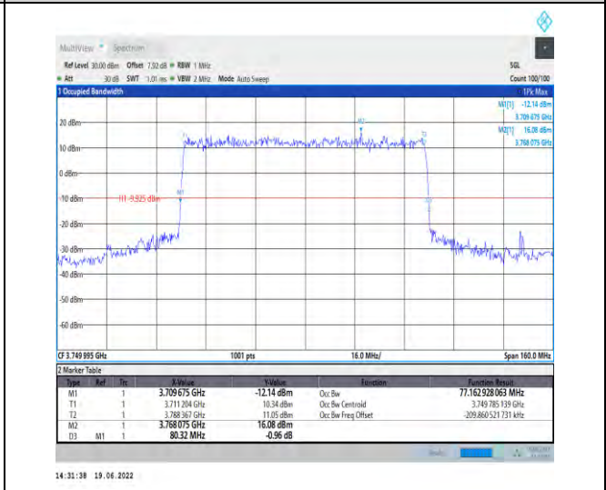
1-N78-3700-3800-PC2-30-80-M-1-DFT-QPSK-Outer_Full-216@0-Ant1-77.163-80.320-≤80-PASS
