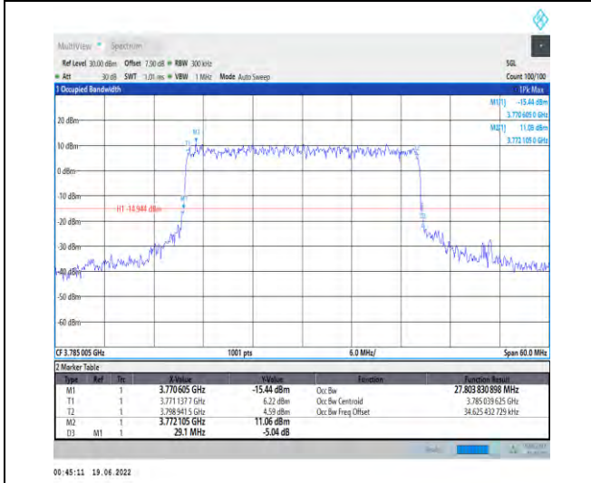
1-N78-3700-3800-PC2-30-30-H-6-CP-QPSK-Outer_Full-78@0-Ant1-27.804-29.100-≤30-PASS
