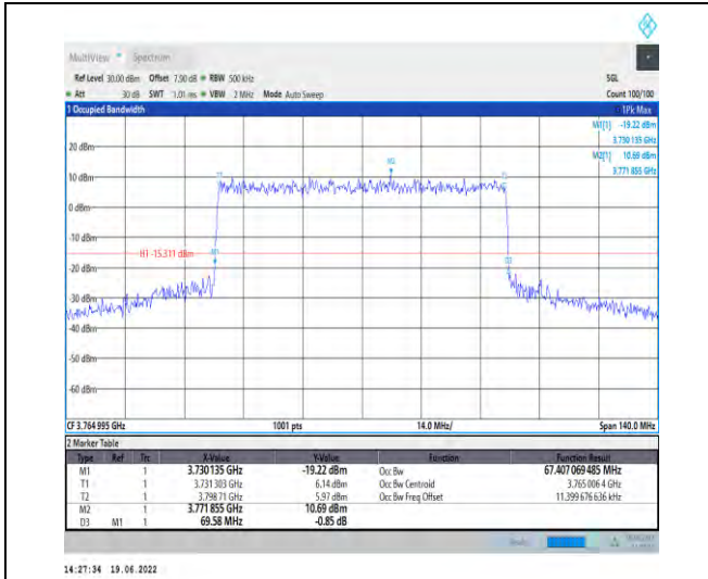
1-N78-3700-3800-PC2-30-70-H-8-CP-64QAM-Outer_Full-189@0-Ant1-67.407-69.580-≤70-PASS
