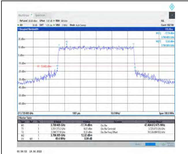
1-N78-3700-3800-PC2-30-50-L-8-CP-64QAM-Outer _Full-133@0-Ant1-47.405-49.400-≤50-PASS
