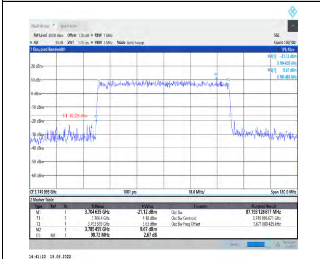
1-N78-3700-3800-PC2-30-90-M-9-CP-256QAM-Outer_Full-245@0-Ant1-87.193-90.720-≤90-PASS
