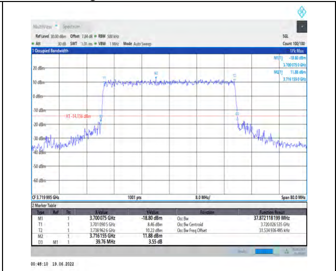
1-N78-3700-3800-PC2-30-40-L-8-CP-64QAM-Outer_Full-106@0-Ant1-37.872-39.760-≤40-PASS
