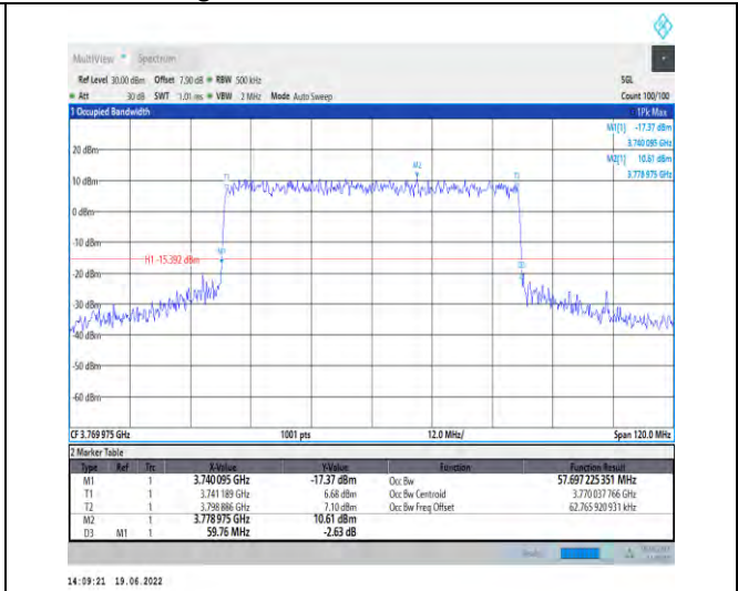
1-N78-3700-3800-PC2-30-60-H-8-CP-64QAM-Outer_Full-162@0-Ant1-57.697-59.760-≤60-PASS
