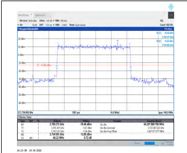
1-N78-3700-3800-PC2-30-70-L-2-DFT-PI2BPSK-Out er_Full-180@0-Ant1-64.292-66.220-≤70-PASS
