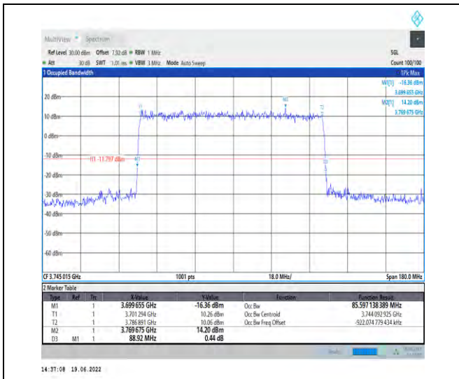
1-N78-3700-3800-PC2-30-90-L-4-DFT-64QAM-Outer_Full-240@0-Ant1-85.597-88.920-≤90-PASS
