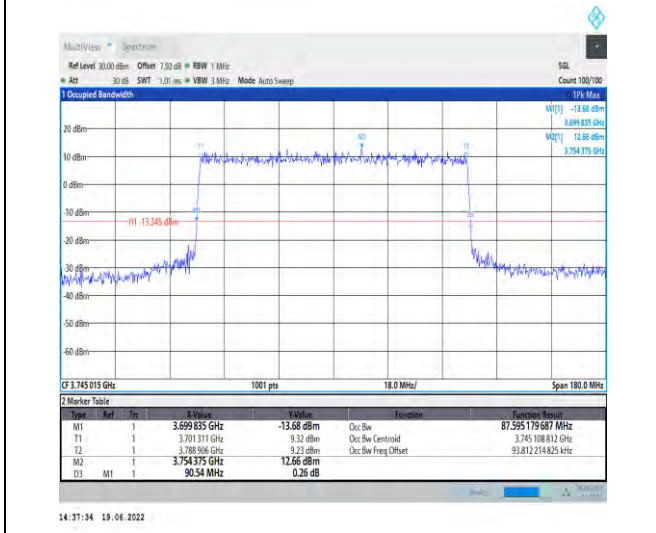
1-N78-3700-3800-PC2-30-90-L-6-CP-QPSK-Outer_Full-245@0-Ant1-87.595-90.540-≤90-PASS
