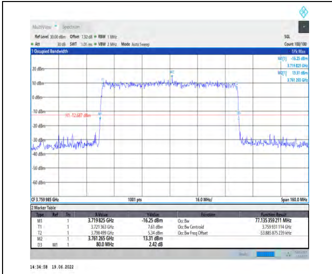
1-N78-3700-3800-PC2-30-80-H-5-DFT-256QAM-Out_er_Full-216@0-Ant1-77.135-80.000-≤80-PASS
