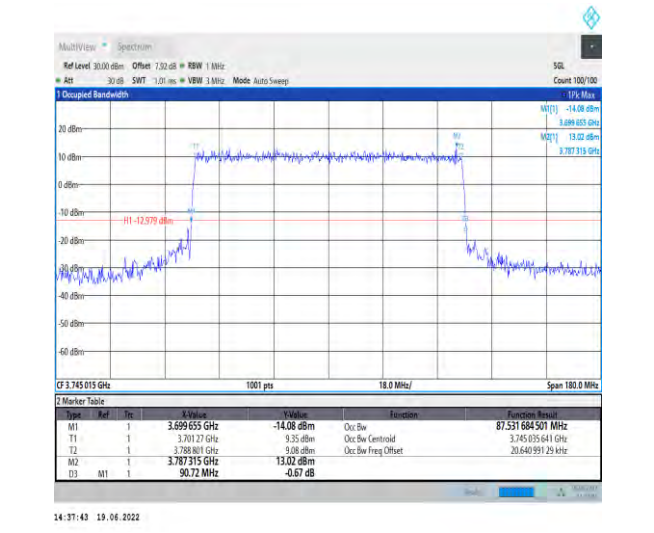
1-N78-3700-3800-PC2-30-90-L-7-CP-16QAM-Outer_Full-245@0-Ant1-87.532-90.720-≤90-PASS
