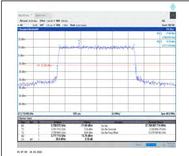
1-N78-3700-3800-PC2-30-40-L-7-CP-16QAM-Outer_Full-106@0-Ant1-37.784-39.600-≤40-PASS
