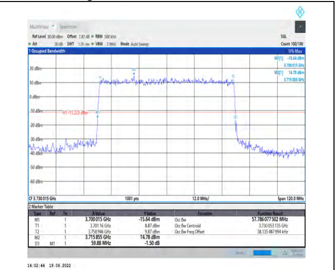
1-N78-3700-3800-PC2-30-60-L-2-DFT-PI2BPSK-Out_er_Full-162@0-Ant1-57.786-59.880-≤60-PASS
