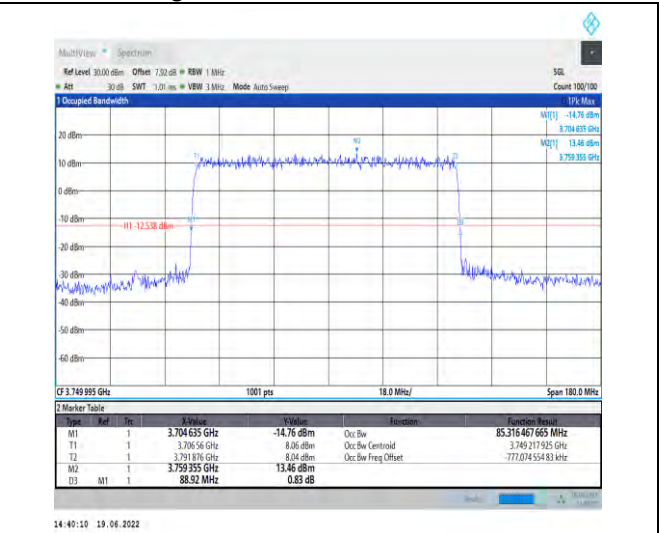
1-N78-3700-3800-PC2-30-90-M-4-DFT-64QAM-Out er_Full-240@0-Ant1-85.316-88.920-≤90-PASS
