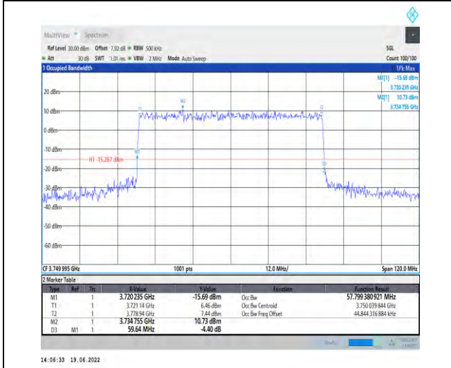
1-N78-3700-3800-PC2-30-60-M-6-CP-QPSK-Outer_Full-162@0-Ant1-57.799-59.640-≤60-PASS
