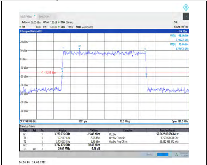
1-N78-3700-3800-PC2-30-60-M-5-DFT-256QAM-Out er_Full-162@0-Ant1-57.963-59.640-≤60-PASS
