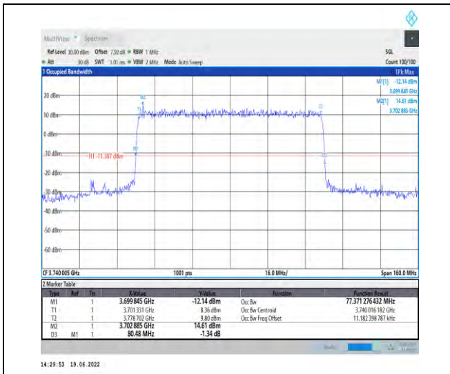
1-N78-3700-3800-PC2-30-80-L-7-CP-16QAM-Outer_Full-217@0-Ant1-77.371-80.480-≤80-PASS
