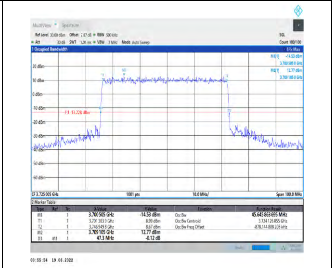
1-N78-3700-3800-PC2-30-50-L-3-DFT-16QAM-Outer_Full-128@0-Ant1-45.646-47.300-≤50-PASS
