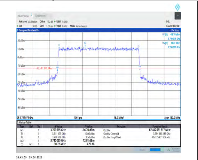
1-N78-3700-3800-PC2-30-90-H-7-CP-16QAM-Outer_Full-245@0-Ant1-87.433-90.720-≤90-PASS
