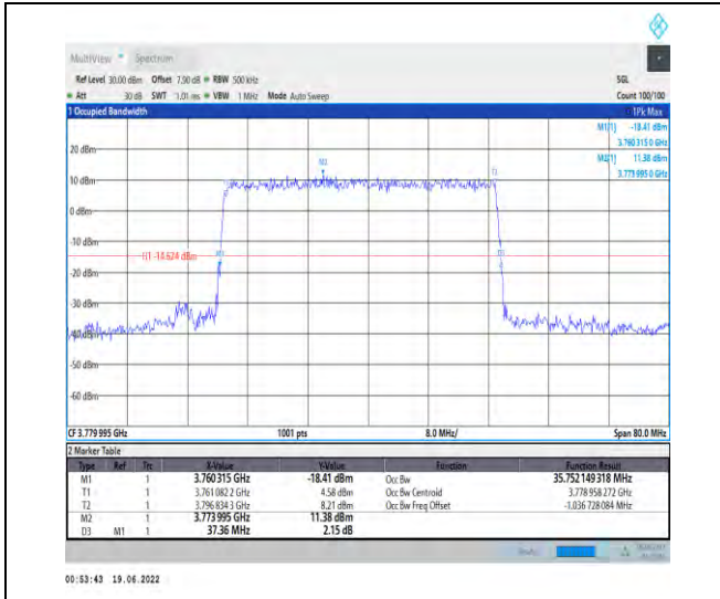
1-N78-3700-3800-PC2-30-40-H-5-DFT-256QAM-Out_er_Full-100@0-Ant1-35.752-37.360-≤40-PASS
