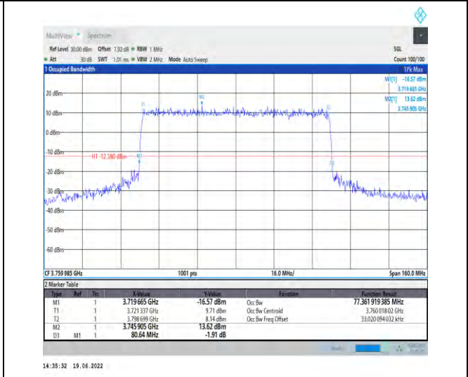
1-N78-3700-3800-PC2-30-80-H-8-CP-64QAM-Outer_Full-217@0-Ant1-77.362-80.640-≤80-PASS
