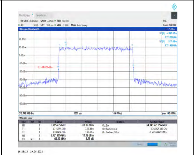
1-N78-3700-3800-PC2-30-70-M-4-DFT-64QAM-Outer_Full-180@0-Ant1-64.141-66.220-≤70-PASS
