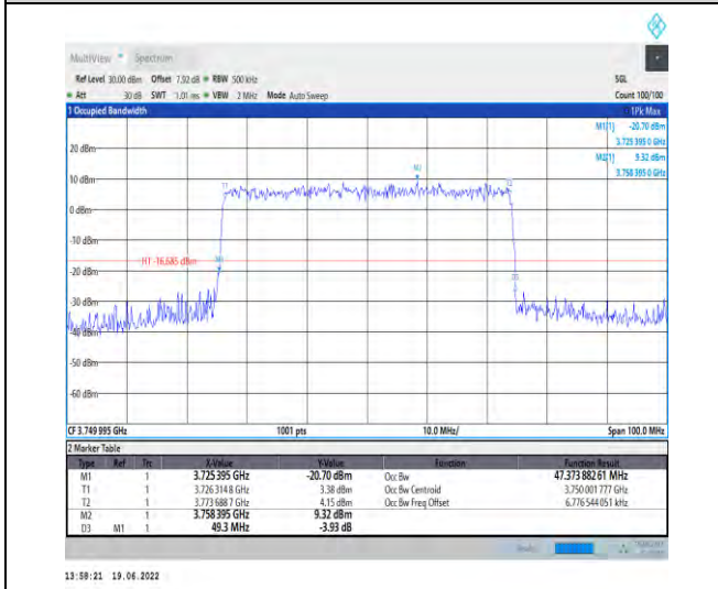
1-N78-3700-3800-PC2-30-50-M-9-CP-256QAM-Outer_Full-133@0-Ant1-47.374-49.300-≤50-PASS
