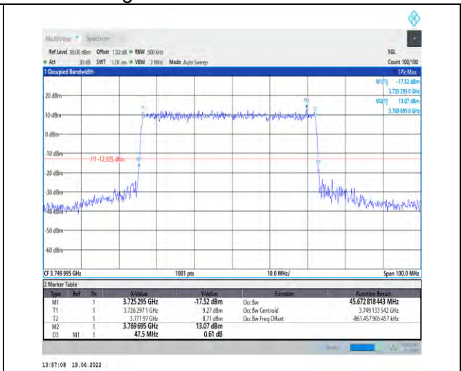
1-N78-3700-3800-PC2-30-50-M-4-DFT-64QAM-Out_r_Full-128@0-Ant1-45.673-47.500-≤50-PASS
