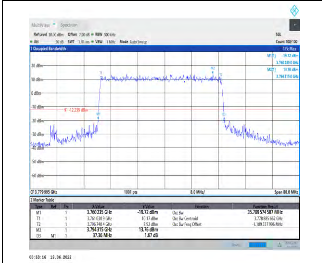
1-N78-3700-3800-PC2-30-40-H-3-DFT-16QAM-Outer_Full-100@0-Ant1-35.71-37.360-≤40-PASS
