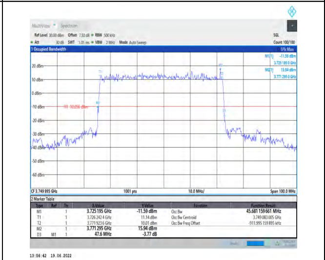
1-N78-3700-3800-PC2-30-50-M-2-DFT-PI2BPSK-Outer _Full-128@0-Ant1-45.681-47.600-≤50-PASS
