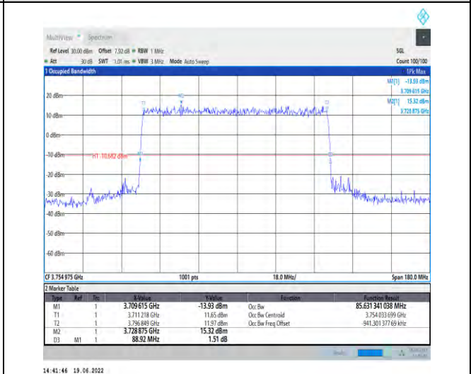
1-N78-3700-3800-PC2-30-90-M-1-DFT-QPSK-Outer_Full-240@0-Ant1-85.631-88.920-≤90-PASS
