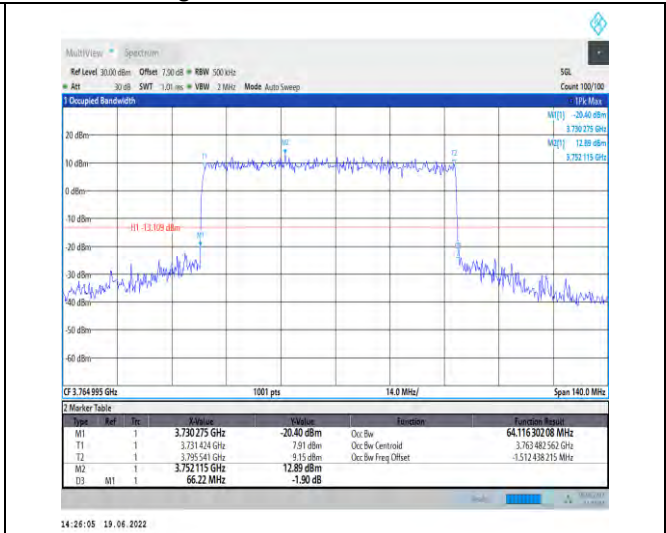
1-N78-3700-3800-PC2-30-70-H-1-DFT-QPSK-Outer_Full-180@0-Ant1-64.116-66.220-≤70-PASS
