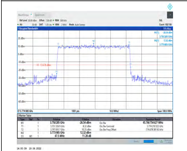
1-N78-3700-3800-PC2-30-50-H-4-DFT-64QAM-Outer_Full-128@0-Ant1-45.767-47.500-≤50-PASS
