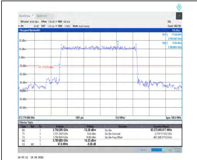
1-N78-3700-3800-PC2-30-50-H-2-DFT-PI2BPSK-Outer_Full-128@0-Ant1-45.573-47.600-≤50-PASS
