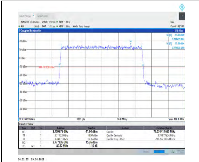
1-N78-3700-3800-PC2-30-80-M-2-DFT-PI2BPSK-Outer_Full-216@0-Ant1-77.074-80.320-≤80-PASS
