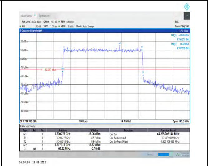
1-N78-3700-3800-PC2-30-70-L-1-DFT-QPSK-Outer_Full-180@0-Ant1-64.236-66.220-≤70-PASS
