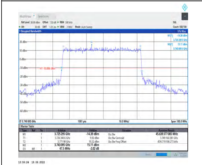
1-N78-3700-3800-PC2-30-50-M-1-DFT-QPSK-Outer _Full-128@0-Ant1-45.639-47.500-≤50-PASS
