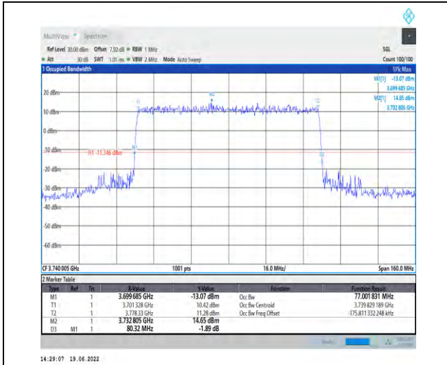
1-N78-3700-3800-PC2-30-80-L-3-DFT-16QAM-Outer_Full-216@0-Ant1-77.002-80.320-≤80-PASS
