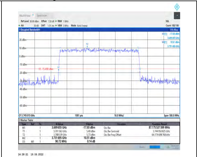
1-N78-3700-3800-PC2-30-90-L-9-CP-256QAM-Outer _Full-245@0-Ant1-87.176-90.720-≤90-PASS
