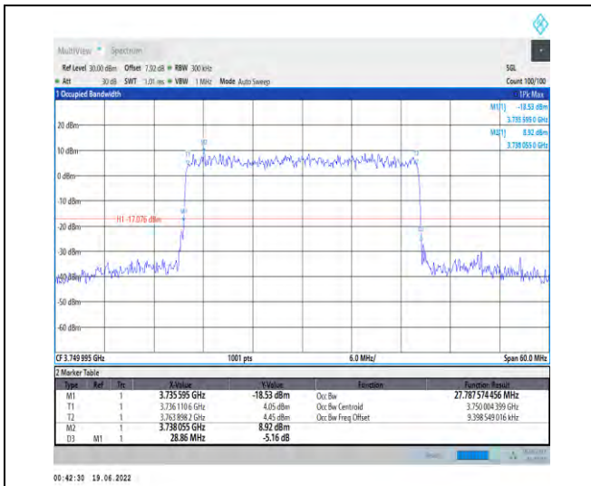
1-N78-3700-3800-PC2-30-30-M-9-CP-256QAM-Out er_Full-78@0-Ant1-27.788-28.860-≤30-PASS
