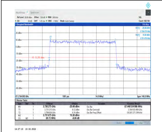
1-N78-3700-3800-PC2-30-70-H-6-CP-QPSK-Outer_Full-189@0-Ant1-67.441-69.720-≤70-PASS
