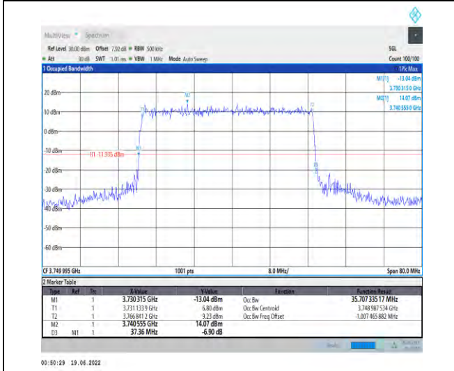
1-N78-3700-3800-PC2-30-40-M-4-DFT-64QAM-Outer_Full-100@0-Ant1-35.707-37.360-≤40-PASS
