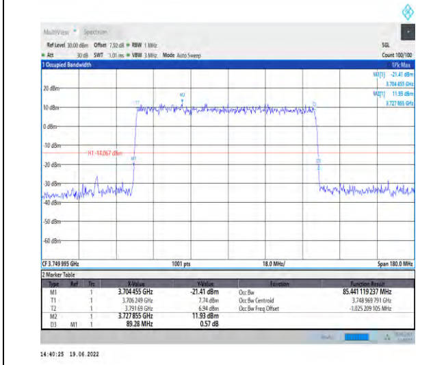
1-N78-3700-3800-PC2-30-90-M-5-DFT-256QAM-Out er_Full-240@0-Ant1-85.441-89.280-≤90-PASS
