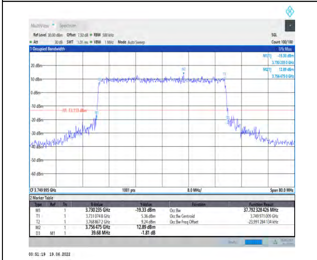
1-N78-3700-3800-PC2-30-40-M-8-CP-64QAM-Outer_Full-106@0-Ant1-37.792-39.680-≤40-PASS
