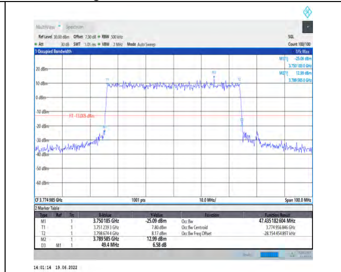
1-N78-3700-3800-PC2-30-50-H-7-CP-16QAM-Outer_Full-133@0-Ant1-47.435-49.400-≤50-PASS
