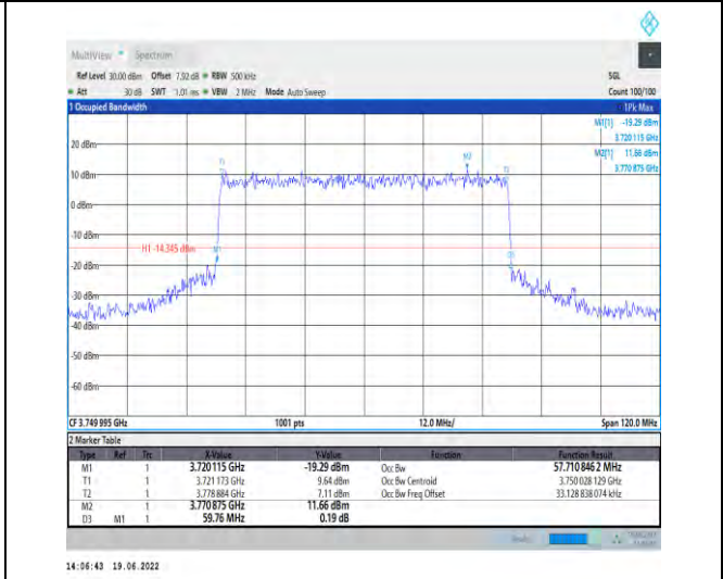
1-N78-3700-3800-PC2-30-60-M-7-CP-16QAM-Outer_Full-162@0-Ant1-57.711-59.760-≤60-PASS
