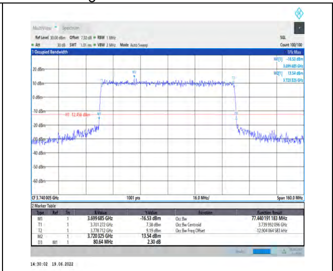
1-N78-3700-3800-PC2-30-80-L-8-CP-64QAM-Outer_Full-217@0-Ant1-77.44-80.640-≤80-PASS
