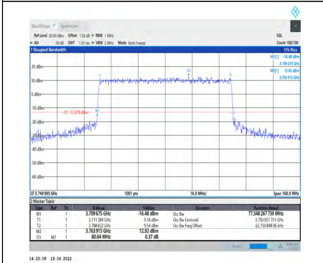
1-N78-3700-3800-PC2-30-80-M-8-CP-64QAM-Outer_Full-217@0-Ant1-77.548-80.640-≤80-PASS
