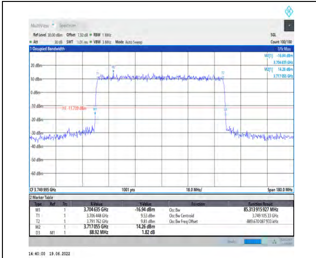
1-N78-3700-3800-PC2-30-90-M-3-DFT-16QAM-Out er_Full-240@0-Ant1-85.314-88.920-≤90-PASS
