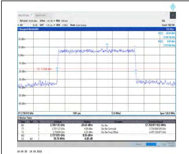
1-N78-3700-3800-PC2-30-60-L-9-CP-256QAM-Outer_Full-162@0-Ant1-57.764-59.760-≤60-PASS
