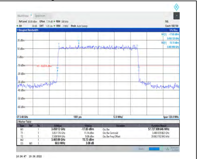
1-N78-3450-3550-PC2-30-60-L-2-DFT-PI2BPSK-Out er_Full-162@0-Ant1-57.727-60.000-≤60-PASS
