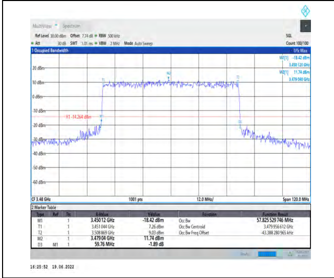
1-N78-3450-3550-PC2-30-60-L-7-CP-16QAM-Outer _Full-162@0-Ant1-57.826-59.760-≤60-PASS
