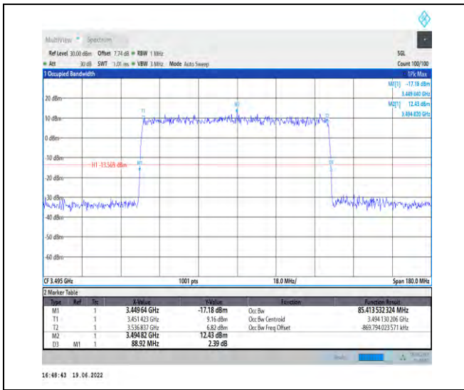
1-N78-3450-3550-PC2-30-90-L-5-DFT-256QAM-Out er_Full-240@0-Ant1-85.414-88.920-<=90-PASS
