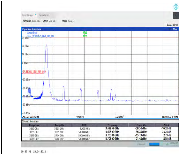
1-N77-3700-3980--30-60-L-1-DFT-PI2BPSK-Edge_1R_B_Left-1@0-Ant1-PASS-see graph
