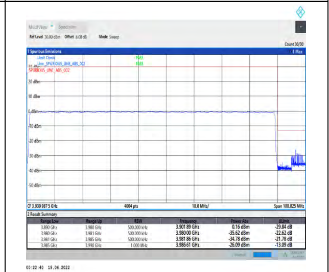
1-N77-3700-3980--30-90-H-6-CP-QPSK-Outer_Full-245@0-Ant1-PASS-see graph
