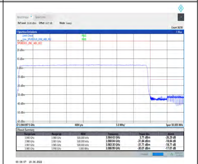
1-N77-3700-3980--30-40-H-6-CP-QPSK-Outer_Full-106@0-Ant1-PASS-see graph
