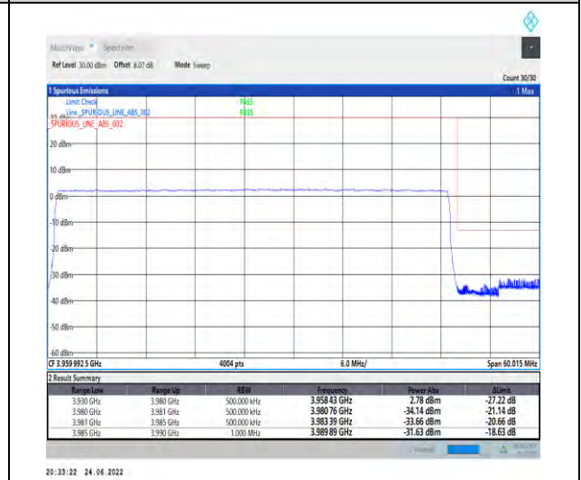
1-N77-3700-3980--30-50-H-6-CP-QPSK-Outer_Full-133@0-Ant1-PASS-see graph
