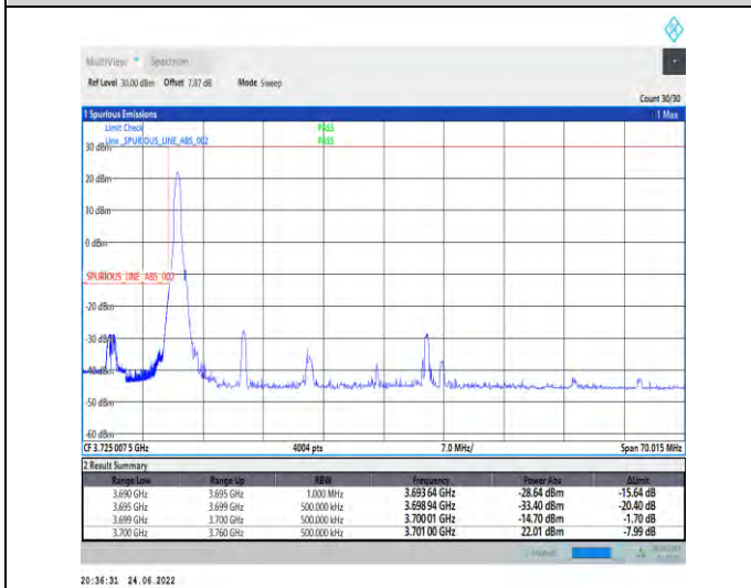
1-N77-3700-3980--30-60-L-4-CP-QPSK-Edge_1RB_L_eff-1@0-Ant1-PASS-see graph
