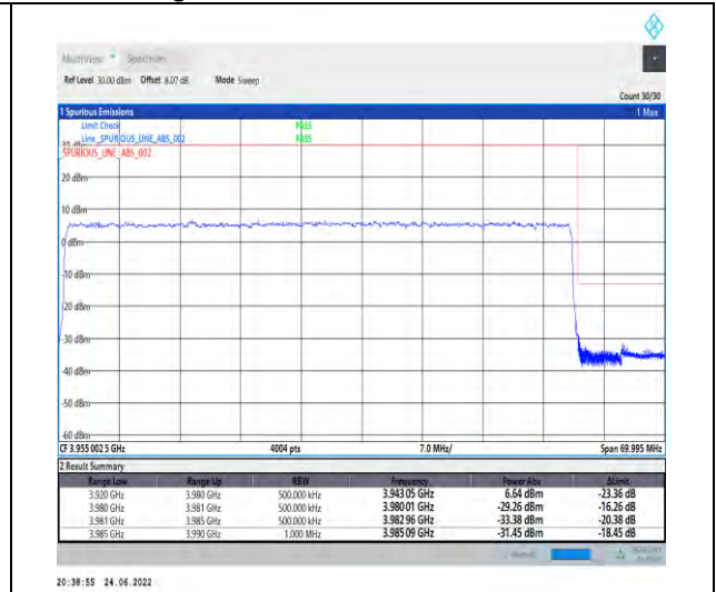
1-N77-3700-3980--30-60-H-3-DFT-PI2BPSK-Outer_Full-162@0-Ant1-PASS-see graph
