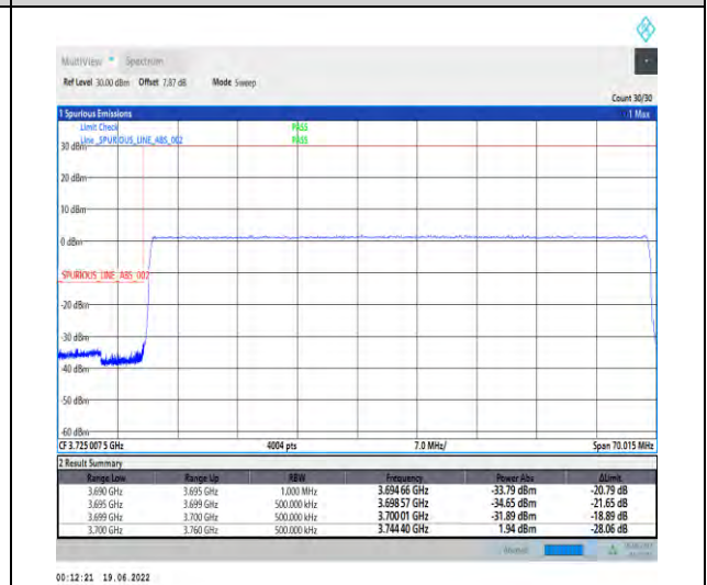
1-N77-3700-3980--30-60-L-6-CP-QPSK-Outer_Ful I-162@0-Ant1-PASS-see graph
