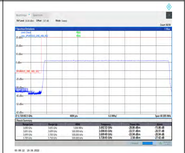
1-N77-3700-3980--30-50-L-6-CP-QPSK-Outer_Ful I-133@0-Ant1-PASS-see graph
