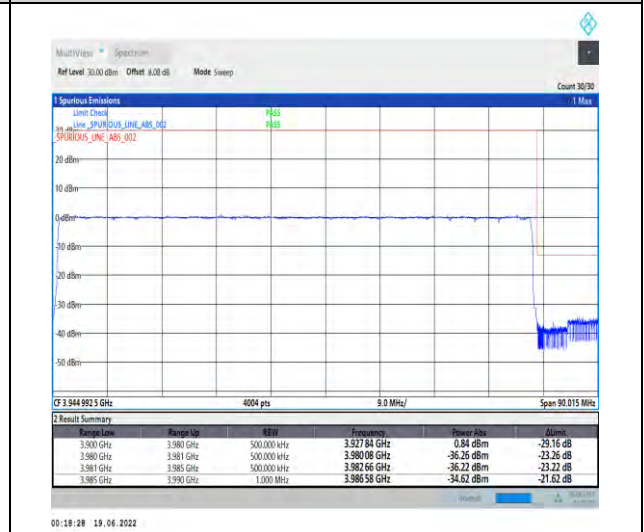
1-N77-3700-3980--30-80-H-6-CP-QPSK-Outer_Full-217@0-Ant1-PASS-see graph
