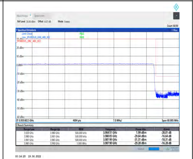
1-N77-3700-3980--30-60-H-6-CP-QPSK-Outer_Full-162@0-Ant1-PASS-see graph
