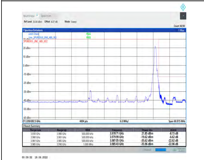
1-N77-3700-3980--30-50-H-5-CP-QPSK-Edge_1RB_Right-1@132-Ant1-PASS-see graph
