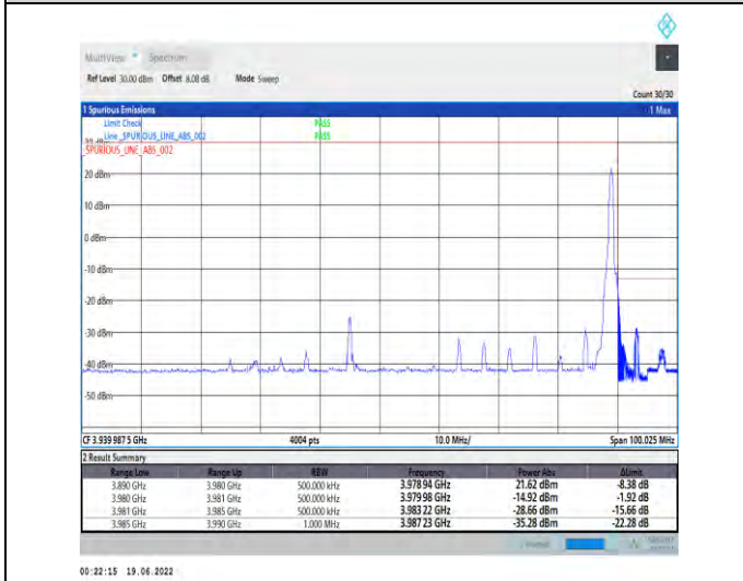
1-N77-3700-3980--30-90-H-5-CP-QPSK-Edge_1RB_Right-1@244-Ant1-PASS-see graph
