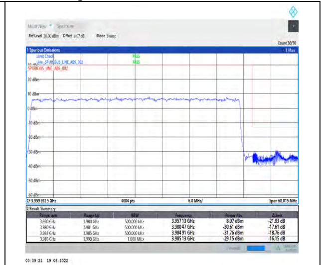
1-N77-3700-3980--30-50-H-3-DFT-PI2BPSK-Outer_Full-128@0-Ant1-PASS-see graph
