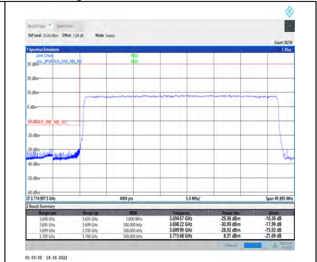
1-N77-3700-3980--30-40-L-3-DFT-PI2BPSK-Outer_Full-100@0-Ant1-PASS-see graph
