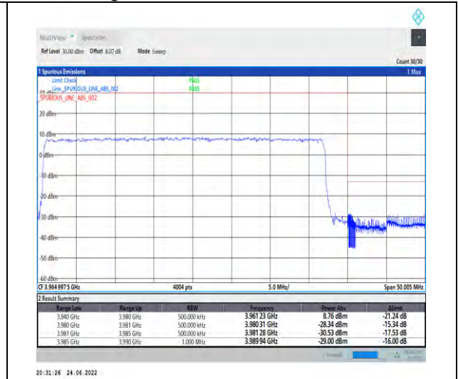
1-N77-3700-3980--30-40-H-3-DFT-PI2BPSK-Outer_Full-100@0-Ant1-PASS-see graph
