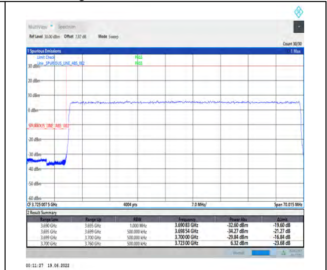
1-N77-3700-3980--30-60-L-3-DFT-PI2BPSK-Outer_Full-162@0-Ant1-PASS-see graph
