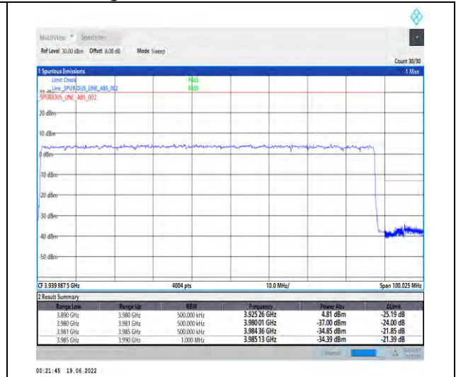
1-N77-3700-3980--30-90-H-3-DFT-PI2BPSK-Outer_Full-240@0-Ant1-PASS-see graph
