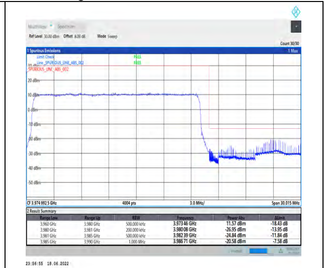
1-N77-3700-3980--30-20-H-3-DFT-PI2BPSK-Outer_Full-50@0-Ant1-PASS-see graph
