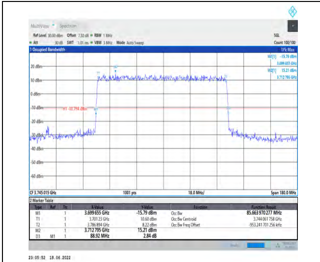
1-N77-3700-3980--30-90-L-3-DFT-16QAM-Outer_Fu II-240@0-Ant1-85.664-88.920-<=90-PASS
