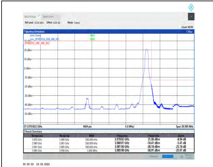
1-N77-3700-3980--30-30-H-2-DFT-PI2BPSK-Edge_1R_B_Right-1@77-Ant1-PASS-see graph
