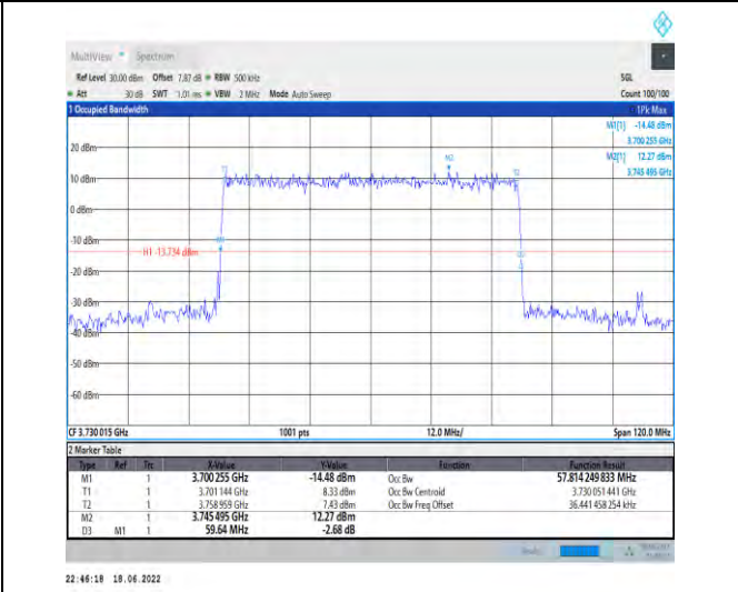
1-N77-3700-3980--30-60-L-4-DFT-64QAM-Outer_Full-162@0-Ant1-57.814-59.640-≤60-PASS
