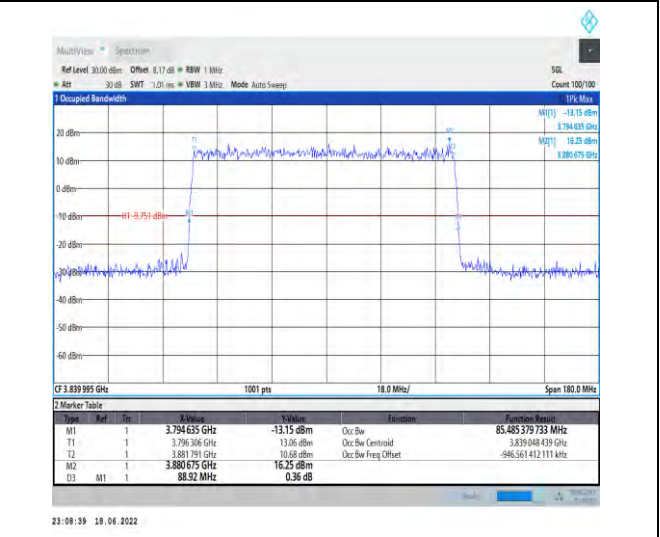
1-N77-3700-3980--30-90-M-1-DFT-QPSK-Outer_Full -240@0-Ant1-85.485-88.920-≤90-PASS
