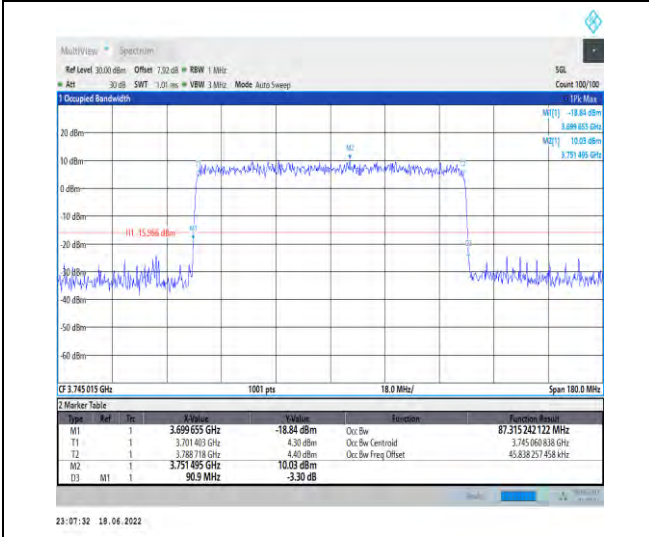
1-N77-3700-3980--30-90-L-9-CP-256QAM-Outer_Full -245@0-Ant1-87.315-90.900-≤90-PASS
