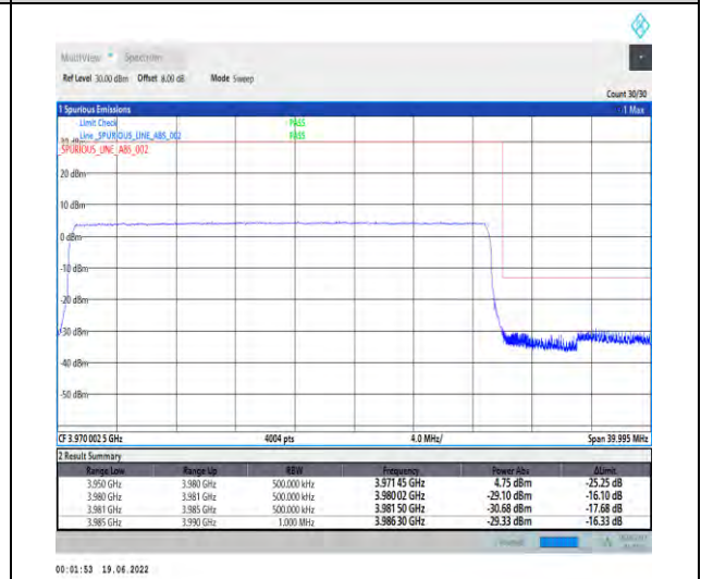
1-N77-3700-3980--30-30-H-6-CP-QPSK-Outer_Full-78@0-Ant1-PASS-see graph
