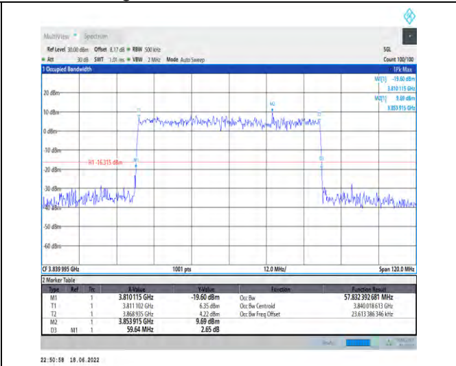
1-N77-3700-3980--30-60-M-9-CP-256QAM-Outer_Fu ll-162@0-Ant1-57.832-59.640-≤60-PASS
