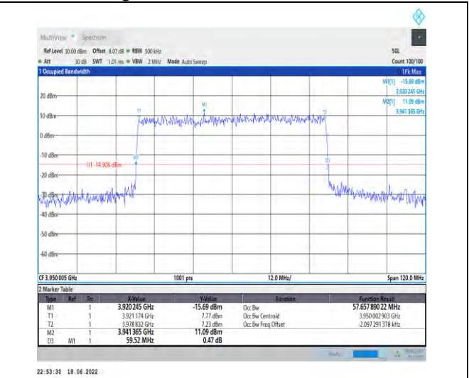
1-N77-3700-3980--30-60-H-8-CP-64QAM-Outer_Full -162@0-Ant1-57.658-59.520-≤60-PASS
