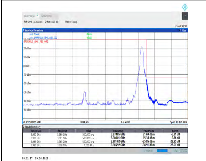
1-N77-3700-3980--30-30-H-5-CP-QPSK-Edge_1RB_Right-1@77-Ant1-PASS-see graph
