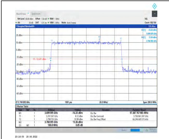
1-N77-3700-3980--30-100-L-8-CP-64QAM-Outer_F ull-273@0-Ant1-97.388-100.800-≤100-PASS
