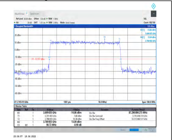
1-N77-3700-3980--30-90-L-8-CP-64QAM-Outer_Full -245@0-Ant1-87.29-90.720-≤90-PASS
