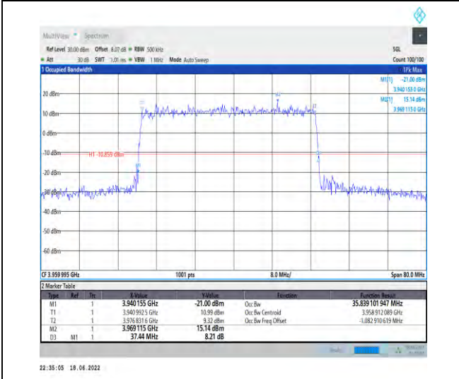
1-N77-3700-3980--30-40-H-3-DFT-16QAM-Outer_Full -100@0-Ant1-35.839-37.440-≤40-PASS
