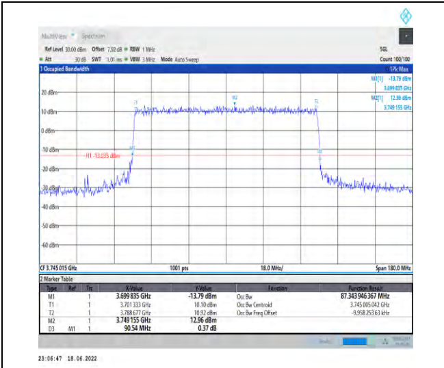
1-N77-3700-3980--30-90-L-7-CP-16QAM-Outer_Full -245@0-Ant1-87.344-90.540-≤90-PASS
