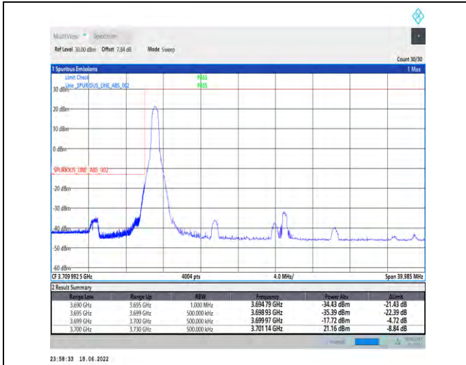
1-N77-3700-3980--30-30-L-1-DFT-PI2BPSK-Edge_1R_B_Left-1@0-Ant1-PASS-see graph
