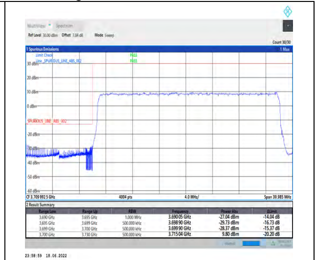
1-N77-3700-3980--30-30-L-3-DFT-PI2BPSK-Outer_Full-75@0-Ant1-PASS-see graph
