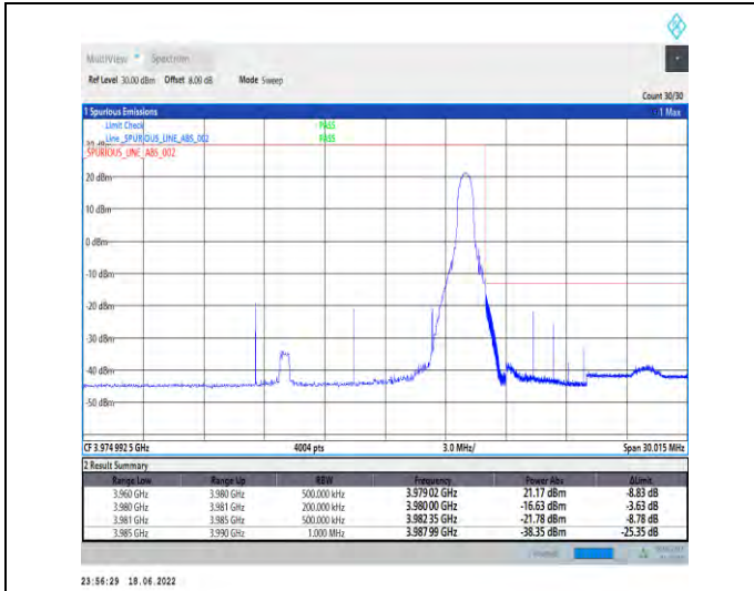
1-N77-3700-3980--30-20-H-2-DFT-PI2BPSK-Edge_1R_B_Right-1@50-Ant1-PASS-see graph
