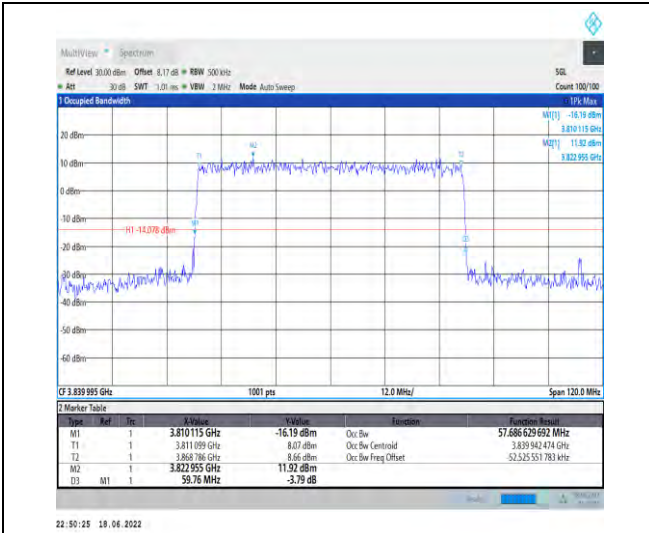
1-N77-3700-3980--30-60-M-8-CP-64QAM-Outer_Ful I-162@0-Ant1-57.687-59.760-≤60-PASS
