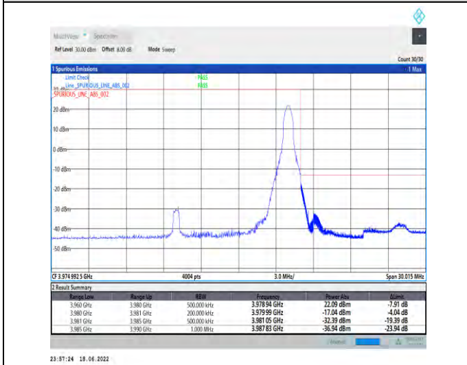
1-N77-3700-3980--30-20-H-5-CP-QPSK-Edge_1RB_Right-1@50-Ant1-PASS-see graph
