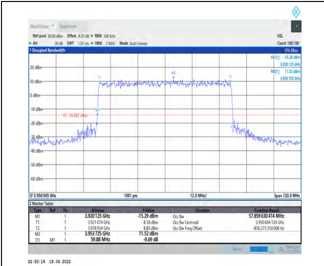
1-N77-3700-3980--30-60-H-7-CP-16QAM-Outer_Full I-162@0-Ant1-57.86-59.880-≤60-PASS
