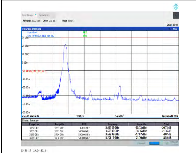
1-N77-3700-3980--30-30-L-4-CP-QPSK-Edge_1RB_L_eff-1@0-Ant1-PASS-see graph
