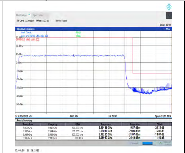
1-N77-3700-3980--30-30-H-3-DFT-PI2BPSK-Outer_Full-75@0-Ant1-PASS-see graph
