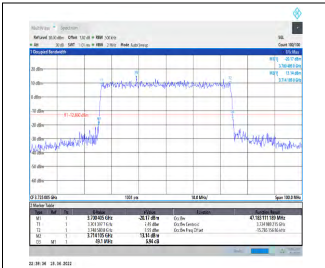
1-N77-3700-3980--30-50-L-8-CP-64QAM-Outer_Full -133@0-Ant1-47.183-49.100-≤50-PASS
