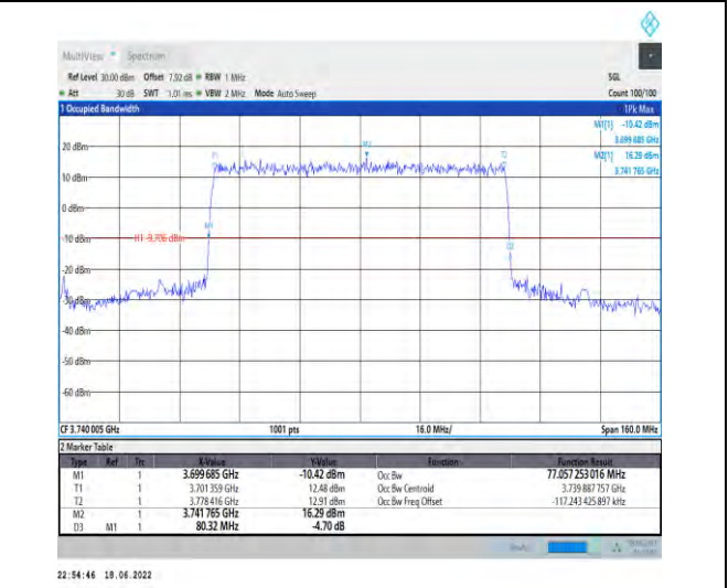
1-N77-3700-3980--30-80-L-1-DFT-QPSK-Outer_Full- 216@0-Ant1-77.057-80.320-≤80-PASS
