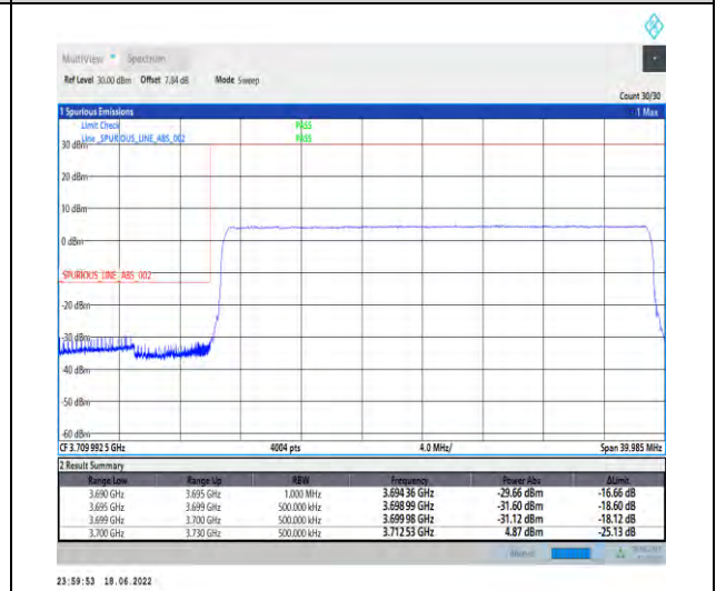
1-N77-3700-3980--30-30-L-6-CP-QPSK-Outer_Ful l-78@0-Ant1-PASS-see graph
