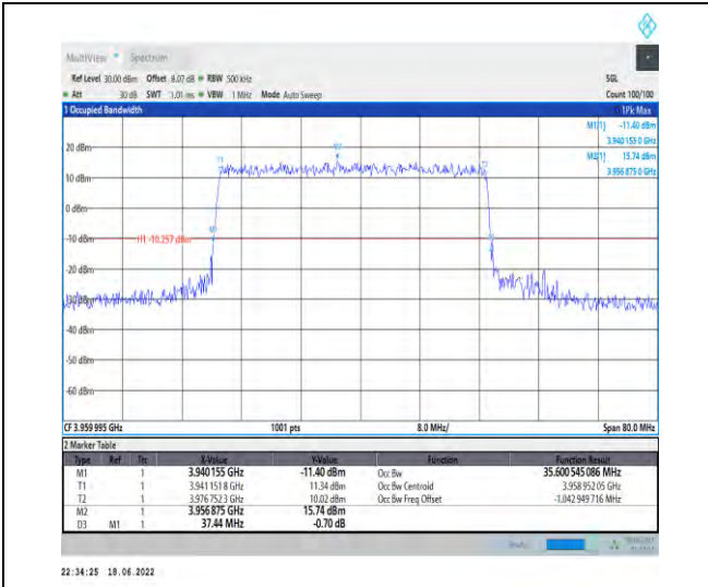
1-N77-3700-3980--30-40-H-1-DFT-QPSK-Outer_Full -100@0-Ant1-35.601-37.440-≤40-PASS
