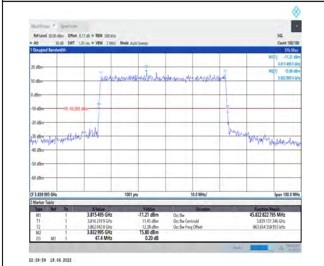
1-N77-3700-3980--30-50-M-1-DFT-QPSK-Outer_Ful I-128@0-Ant1-45.823-47.400-≤50-PASS
