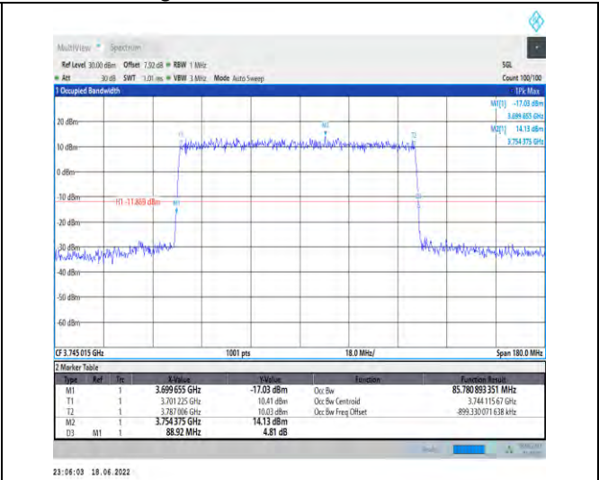
1-N77-3700-3980--30-90-L-4-DFT-64QAM-Outer_Ful I-240@0-Ant1-85.781-88.920-<=90-PASS
