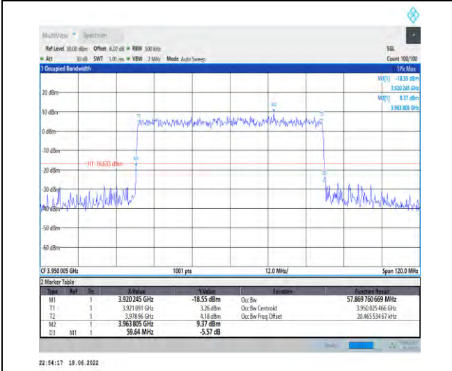
1-N77-3700-3980--30-60-H-9-CP-256QAM-Outer_F ull-162@0-Ant1-57.87-59.640-≤60-PASS
