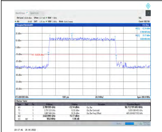
1-N77-3700-3980--30-100-M-1-DFT-QPSK-Outer_F ull-270@0-Ant1-96.112-99.800-≤100-PASS
