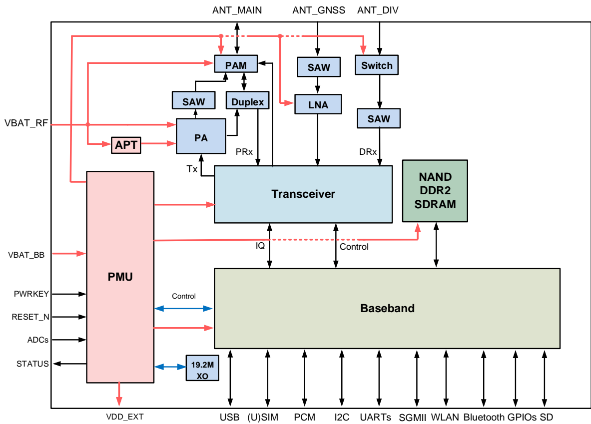
Figure 1: Functional Diagram
