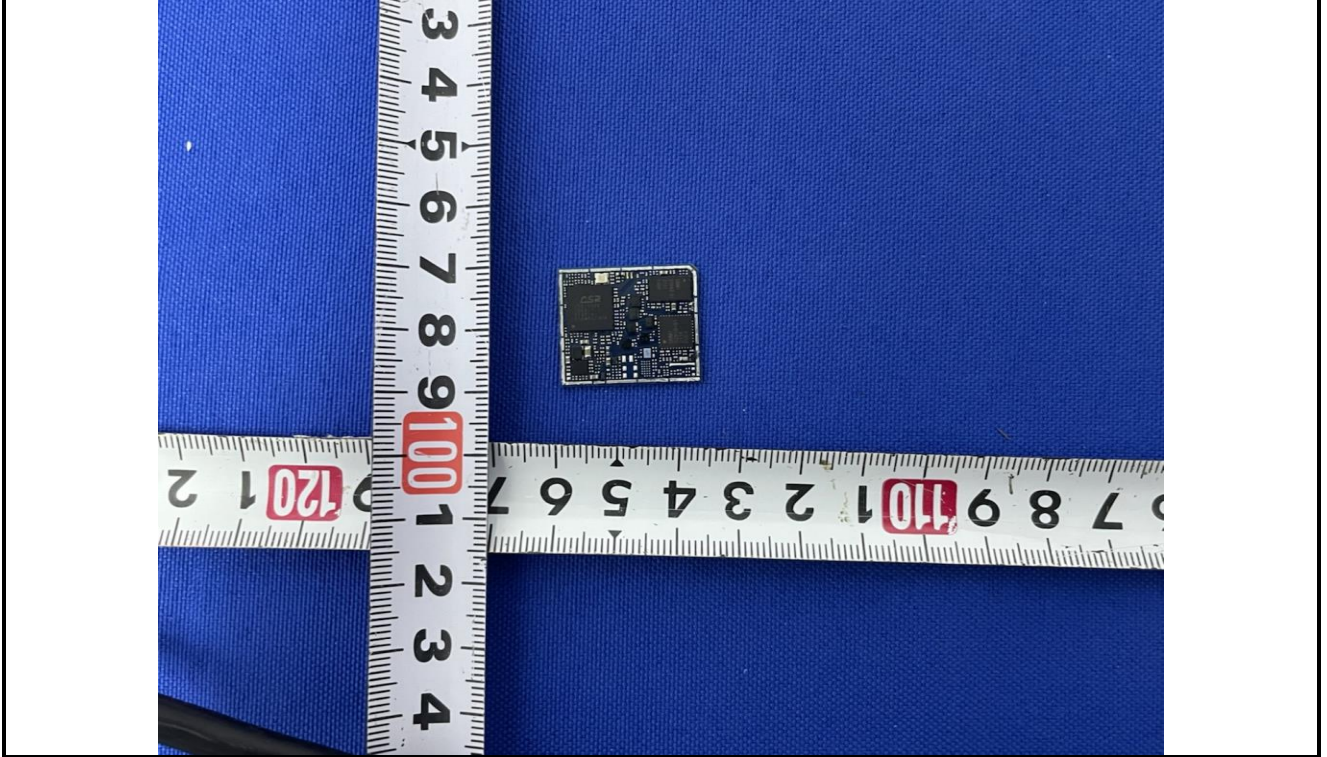
EUT Photo(without GPS)
