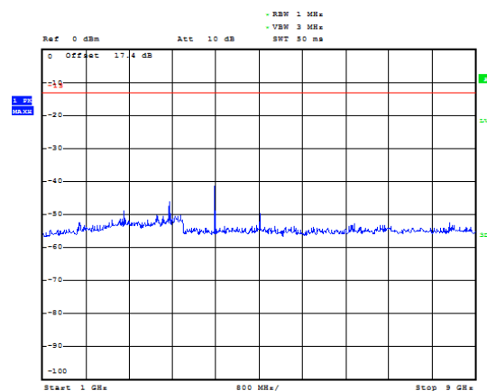
LTE Band 5 3MHz CH-Middle 1GHz~9GHz
