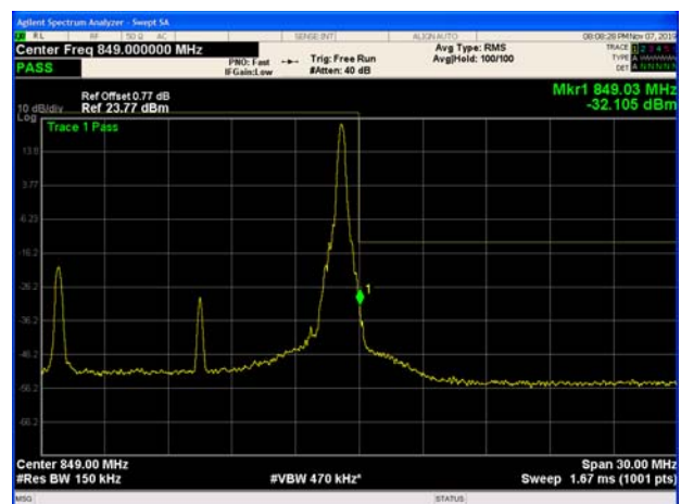
LTE Band 26 QPSK 15MHz CH-High 1RB
