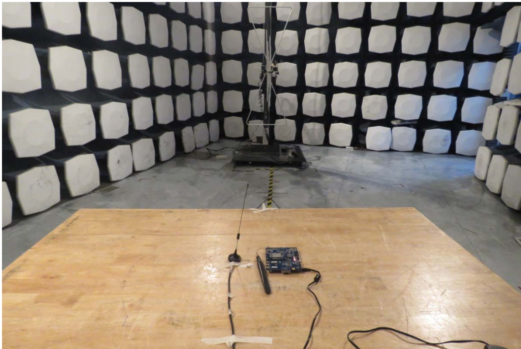
30MHz-1GHz
