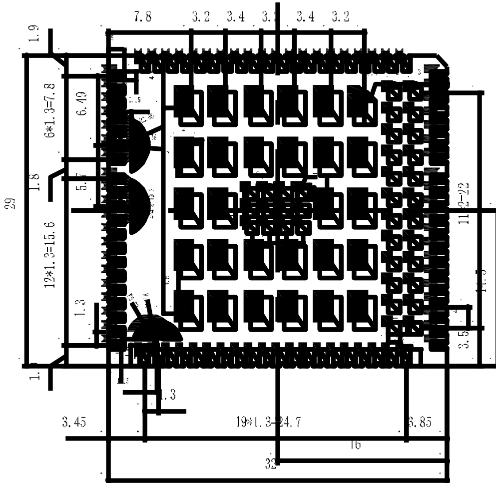
Figure 45: Module Bottom Dimensions (Bottom View)
