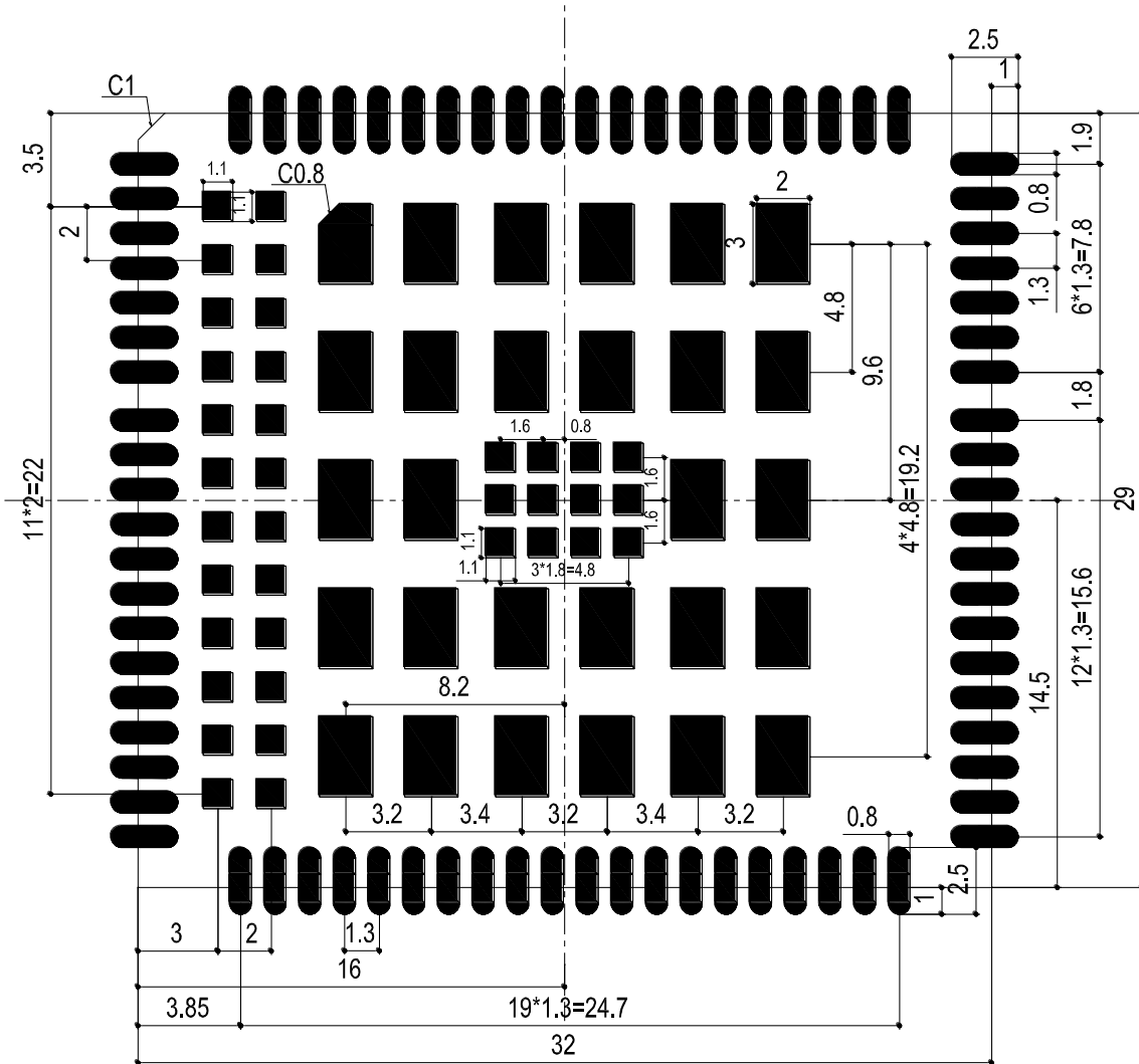
Figure 46: Recommended Footprint (Top View)
