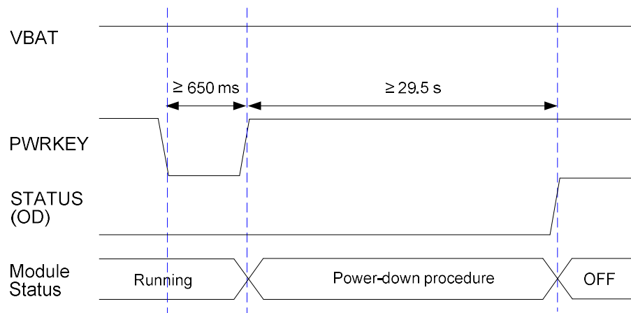
Figure 13: Power-down Timing
