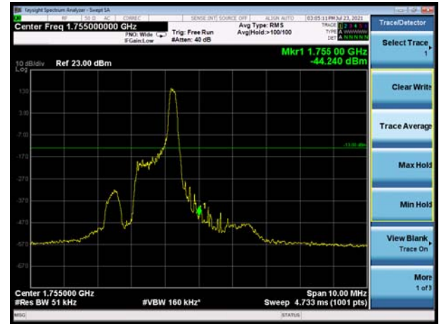
LTE eMTC Band 4 QPSK 10MHz CH-High, 100%RB
