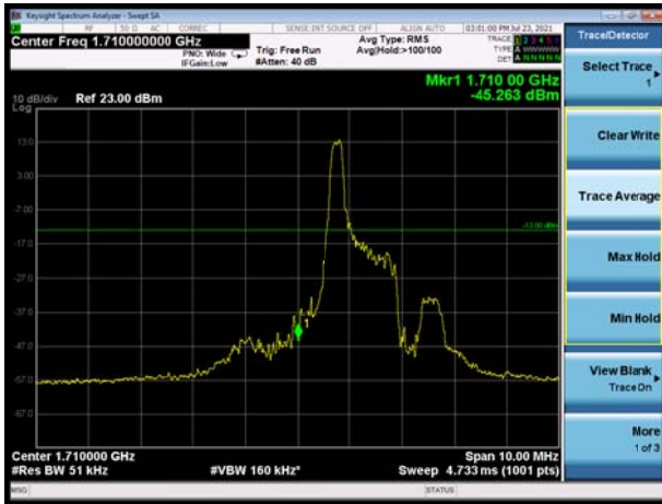
LTE eMTC Band 4 QPSK 10MHz CH-Low, 100%RB
