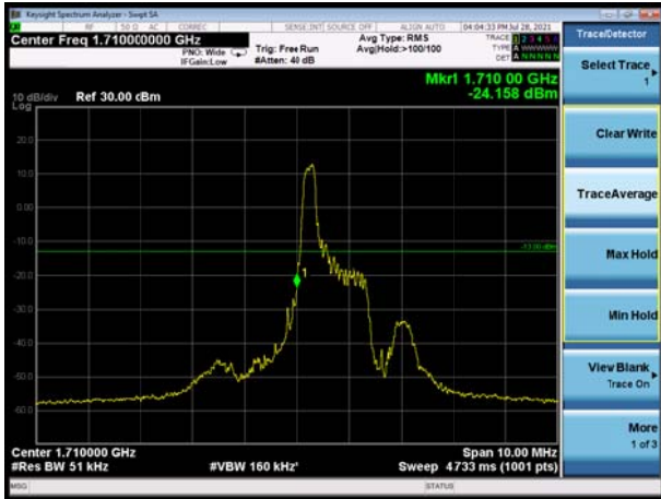
LTE eMTC Band 66 QPSK 1.4MHz CH-Low, 100%RB
