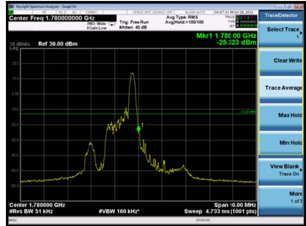
LTE eMTC Band 66 16QAM 1.4MHz CH-High, 100%RB
