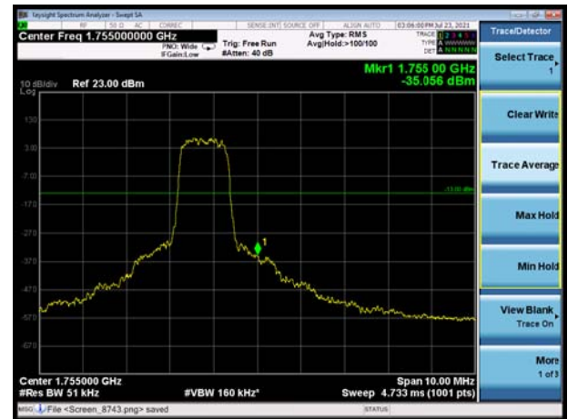
LTE eMTC Band 4 QPSK 15MHz CH-High, 1 RB
