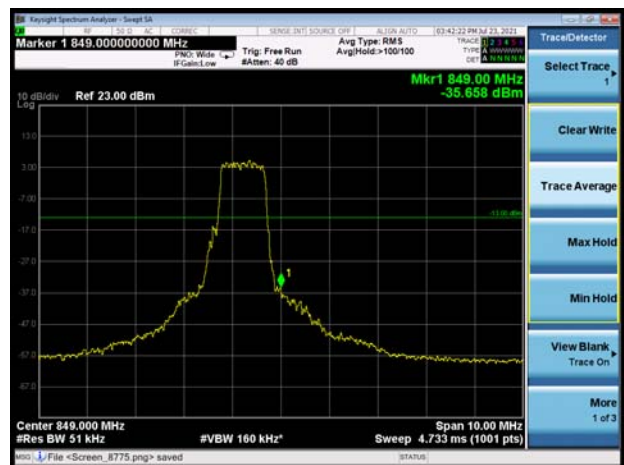
LTE eMTC Band 5 16QAM 3MHz CH-High 100%RB
