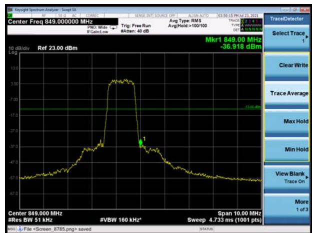
LTE eMTC Band 5 QPSK 5MHz CH-High 100%RB
