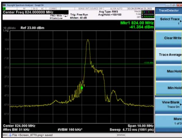
LTE eMTC Band 5 16QAM 3MHz CH-Low 100%RB
