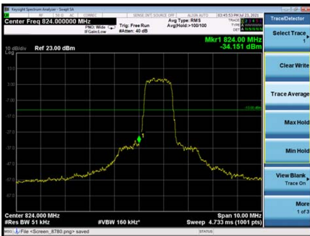
LTE eMTC Band 5 QPSK 5MHz CH-Low 100%RB
