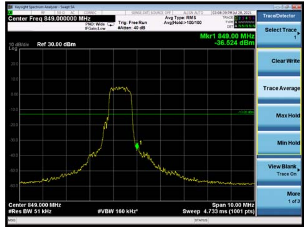
LTE eMTC Band 26 16QAM 10MHz CH-High 1RB
