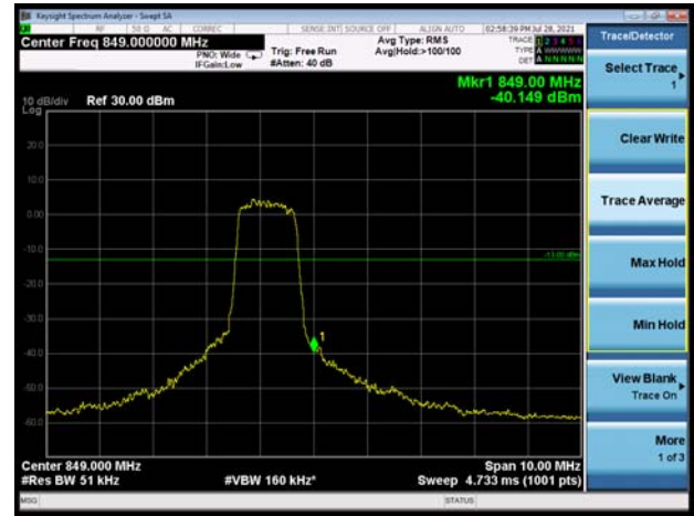
LTE eMTC Band 26 QPSK 5MHz CH-High 1RB
