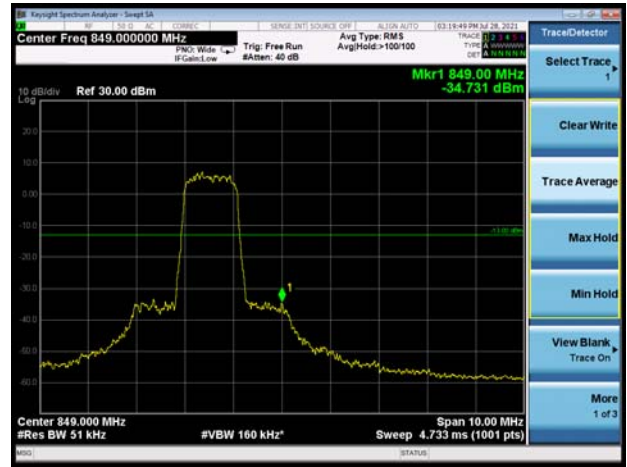
LTE eMTC Band 26 16QAM 1.4MHz CH-High 1RB
