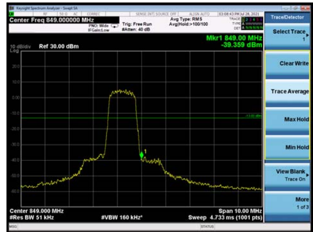
LTE eMTC Band 26 QPSK 5MHz CH-High 100%RB
