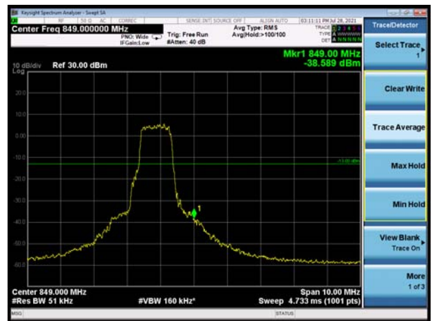
LTE eMTC Band 26 16QAM 10MHz CH-High 100%RB
