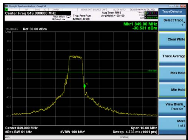
LTE eMTC Band 26 16QAM 1.4MHz CH-High 100%RB
