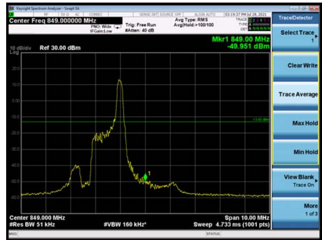
LTE eMTC Band 26 16QAM 15MHz CH-High 100%RB
