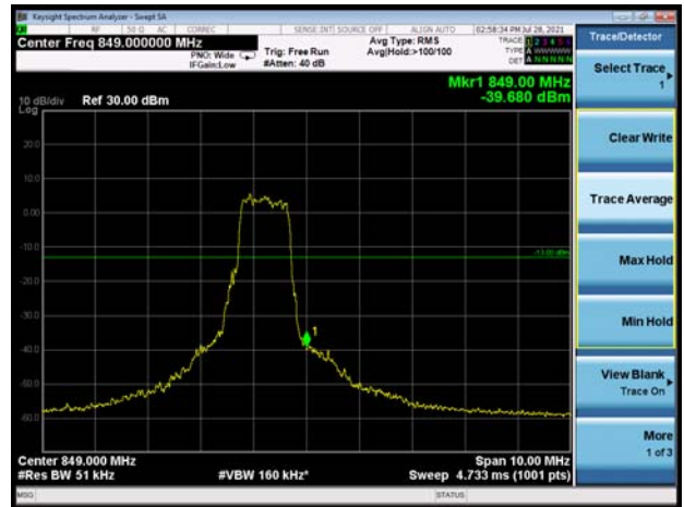
LTE eMTC Band 26 16QAM 5MHz CH-High 1RB
