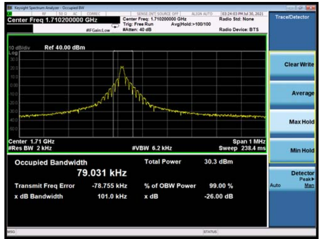
NB-IoT Band 4 BPSK 15KHz 1@0 CH-Middle
