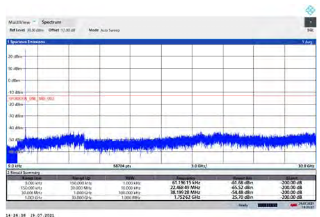
LTE Band 4 3MHz CH-High 9kHz~30GHz
