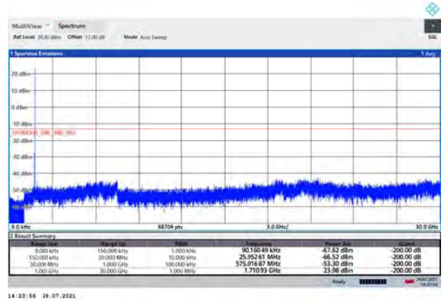
LTE Band 4 3MHz CH-Middle 9kHz~30GHz
