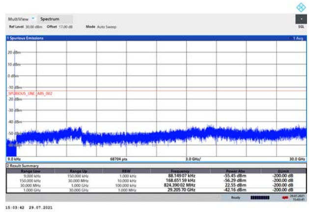
LTE Band 5 3MHz CH-Middle 9kHz~30GHz
