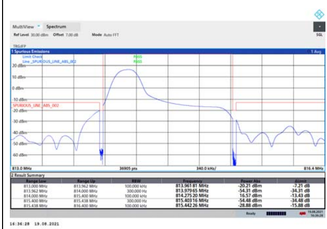
LTE Band 26 QPSK 1.4MHz CH-Low 100%RB
