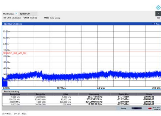
LTE Band 26 1.4MHz CH-Middle 9kHz~30GHz
