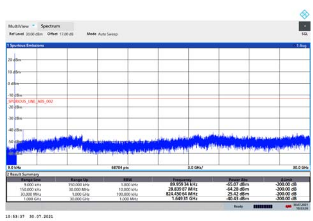
LTE Band 26 3MHz CH-Middle 9kHz~30GHz
