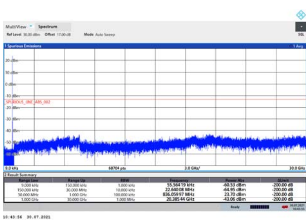
LTE Band 26 1.4MHz CH-High 9kHz~30GHz
