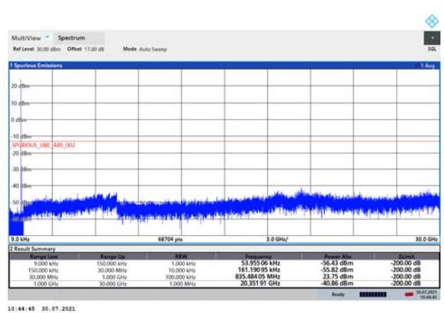
LTE Band 26 3MHz CH-High 9kHz~30GHz
