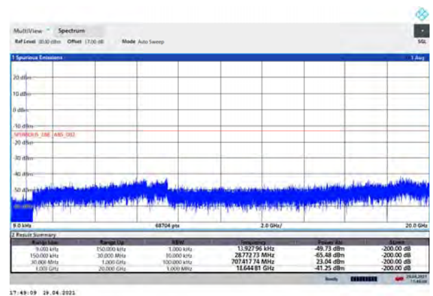
NB-IoT Band 12 CH-High 9kHz~20GHz
