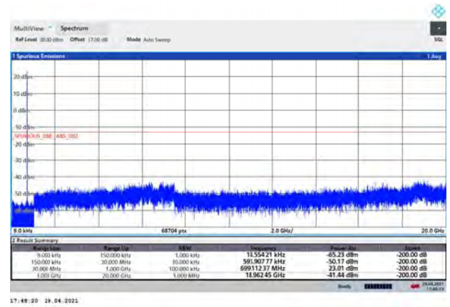
NB-IoT Band 12 CH-Middle 9kHz~20GHz
