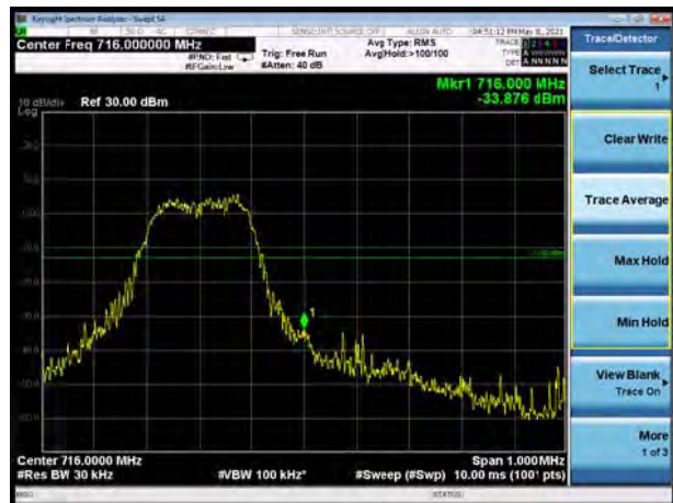
NB-IoT Band 17 QPSK 15KHz 12@0 CH- High
