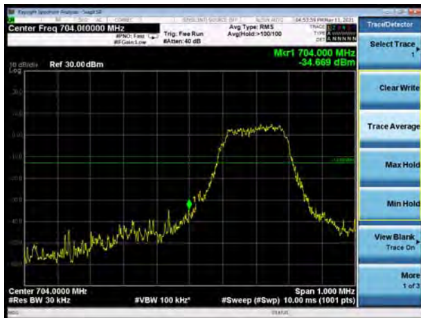
NB-IoT Band 17 QPSK 15KHz 12@0 CH-Low
