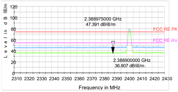
Bluetooth LE Channel 0 Peak+ Average
