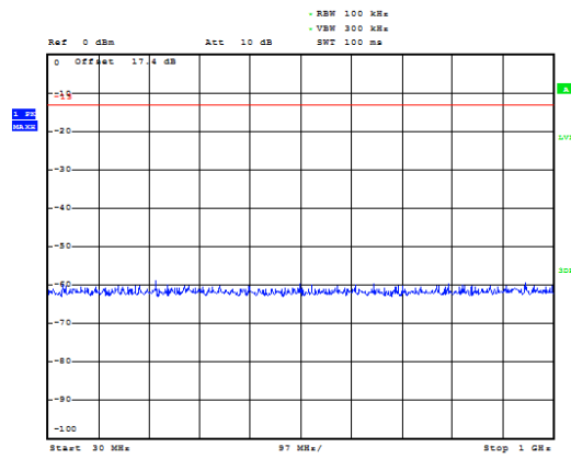
LTE Band 2 1.4MHz CH-Middle 30MHz~1GHz
