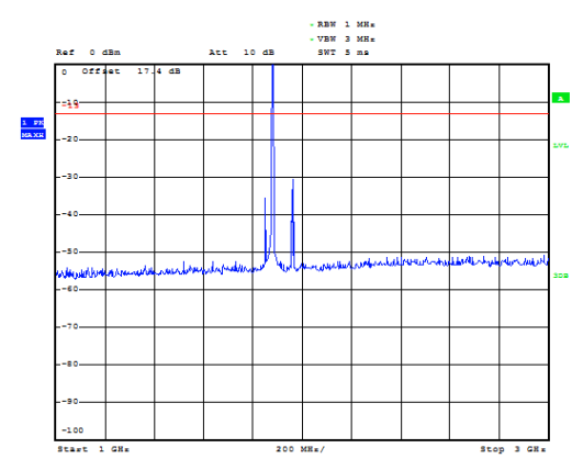
LTE Band 2 1.4MHz CH-Middle 1GHz~3GHz
