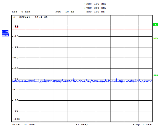
LTE Band 2 1.4MHz CH-Low 30MHz~1GHz
