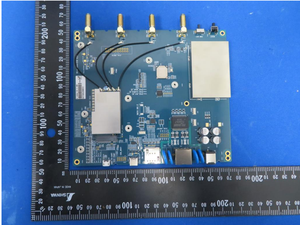
(1) EUT & Test Fixture Photo
