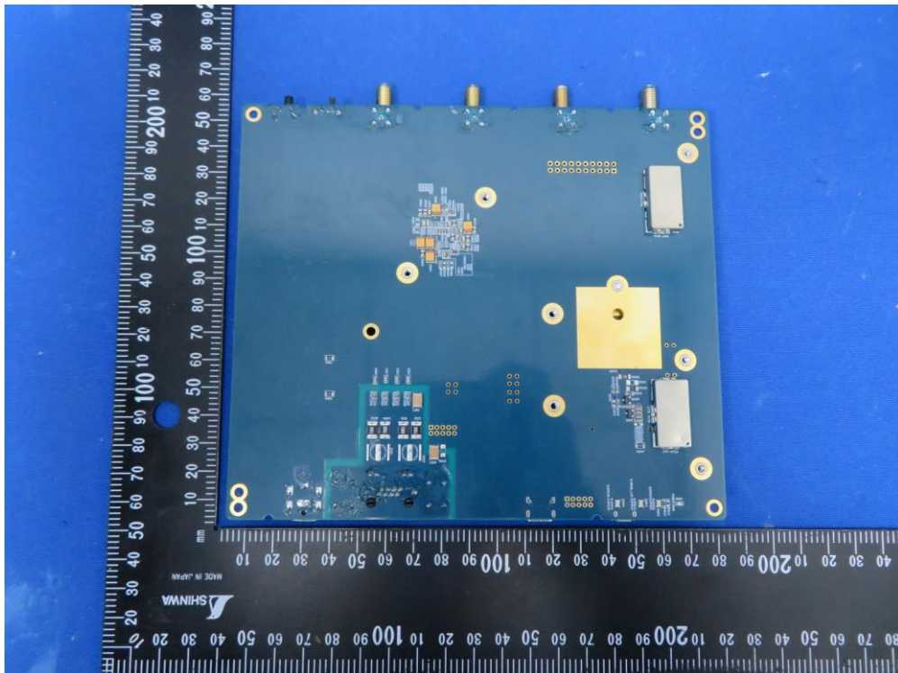
(2) EUT & Test Fixture Photo
