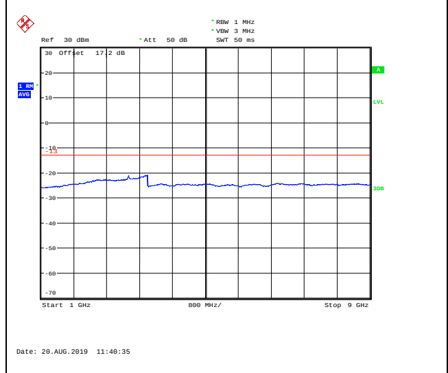
LTE Band 26 5MHz CH-High 1GHz~9GHz
