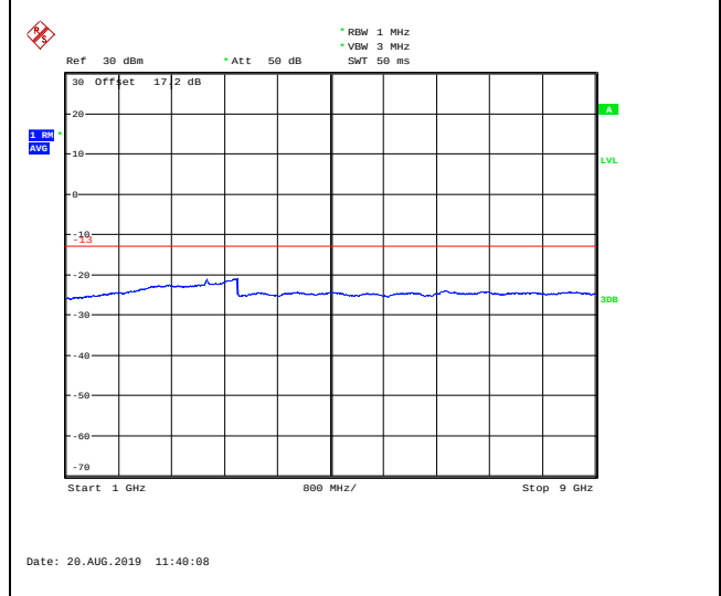
LTE Band 26 5MHz CH-Middle 1GHz~9GHz
