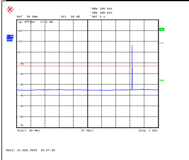
LTE Band 26 5MHz CH-Low 30MHz~1GHz
