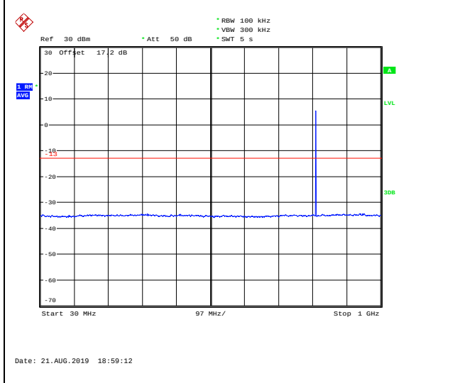
LTE Band 26 5MHz CH-Middle 30MHz~1GHz
