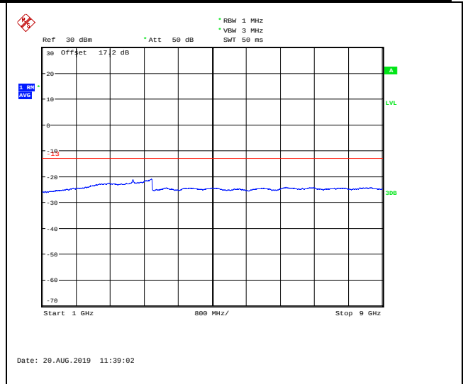
LTE Band 26 5MHz CH-Low 1GHz~9GHz
