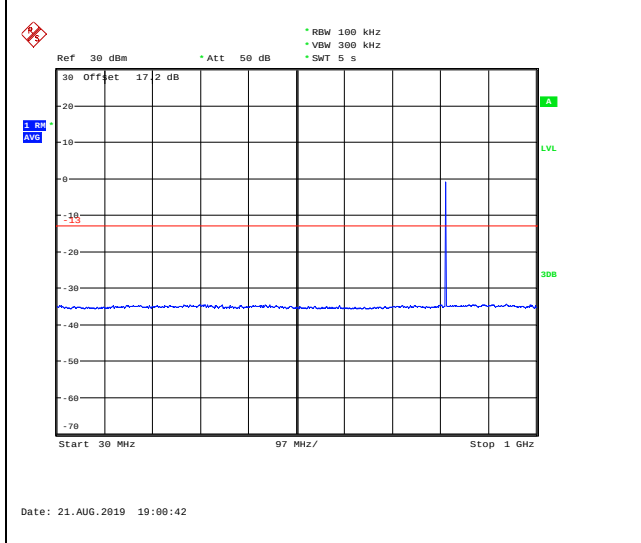
LTE Band 26 5MHz CH-High 30MHz~1GHz
