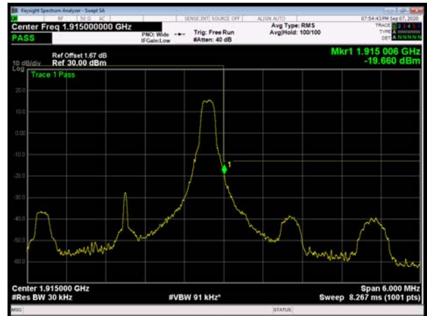
LTE Band 25 3MHz 16QAM 100%RB CH-High
