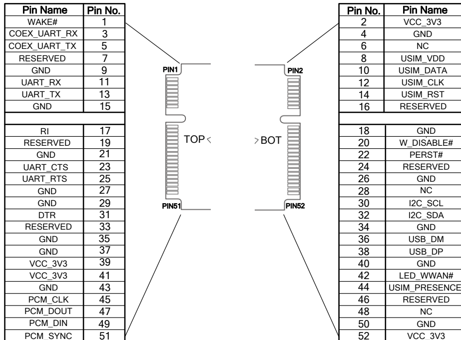
Figure 1: Pin Assignment
