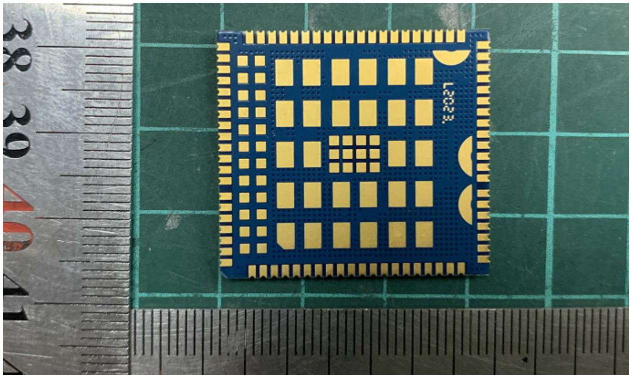
EC200T-AU
