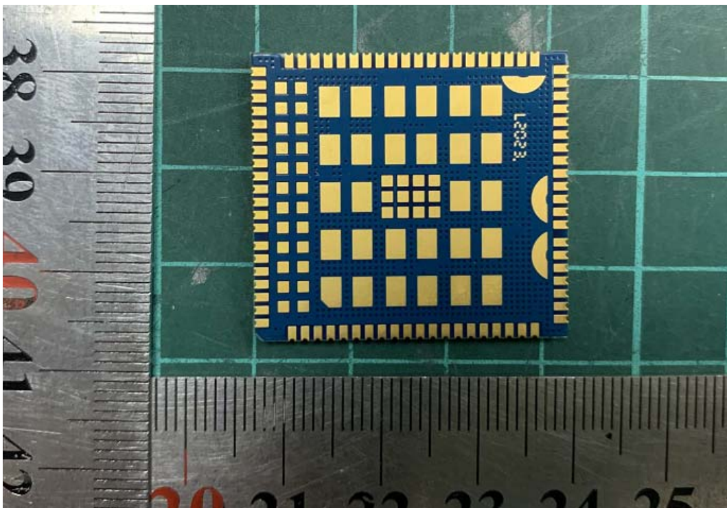
EC200T-AU
