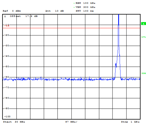
WCDMA Band V CH-High 30MHz ~ 1GHz
