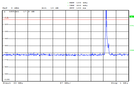
WCDMA Band V CH-Low 30MHz ~ 1GHz
