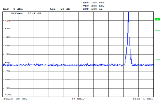
WCDMA Band V CH-Middle 30MHz ~ 1GHz
