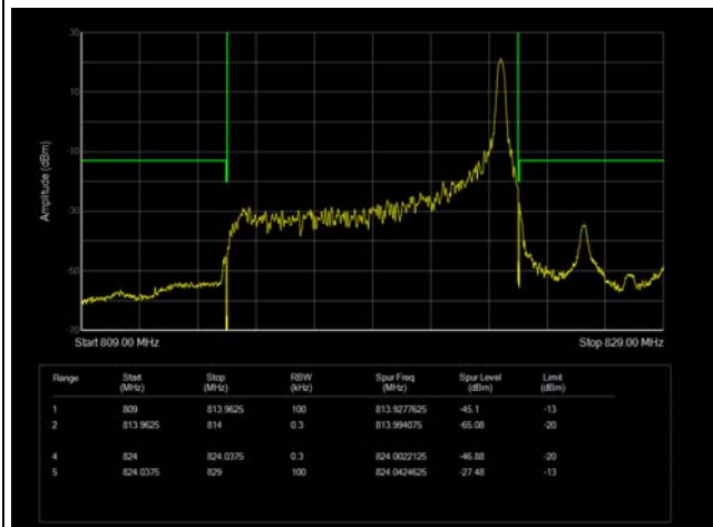
LTE Band 26 16QAM 10MHz CH-High 1RB
