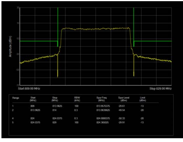
LTE Band 26 16QAM 10MHz CH-Low 100%RB
